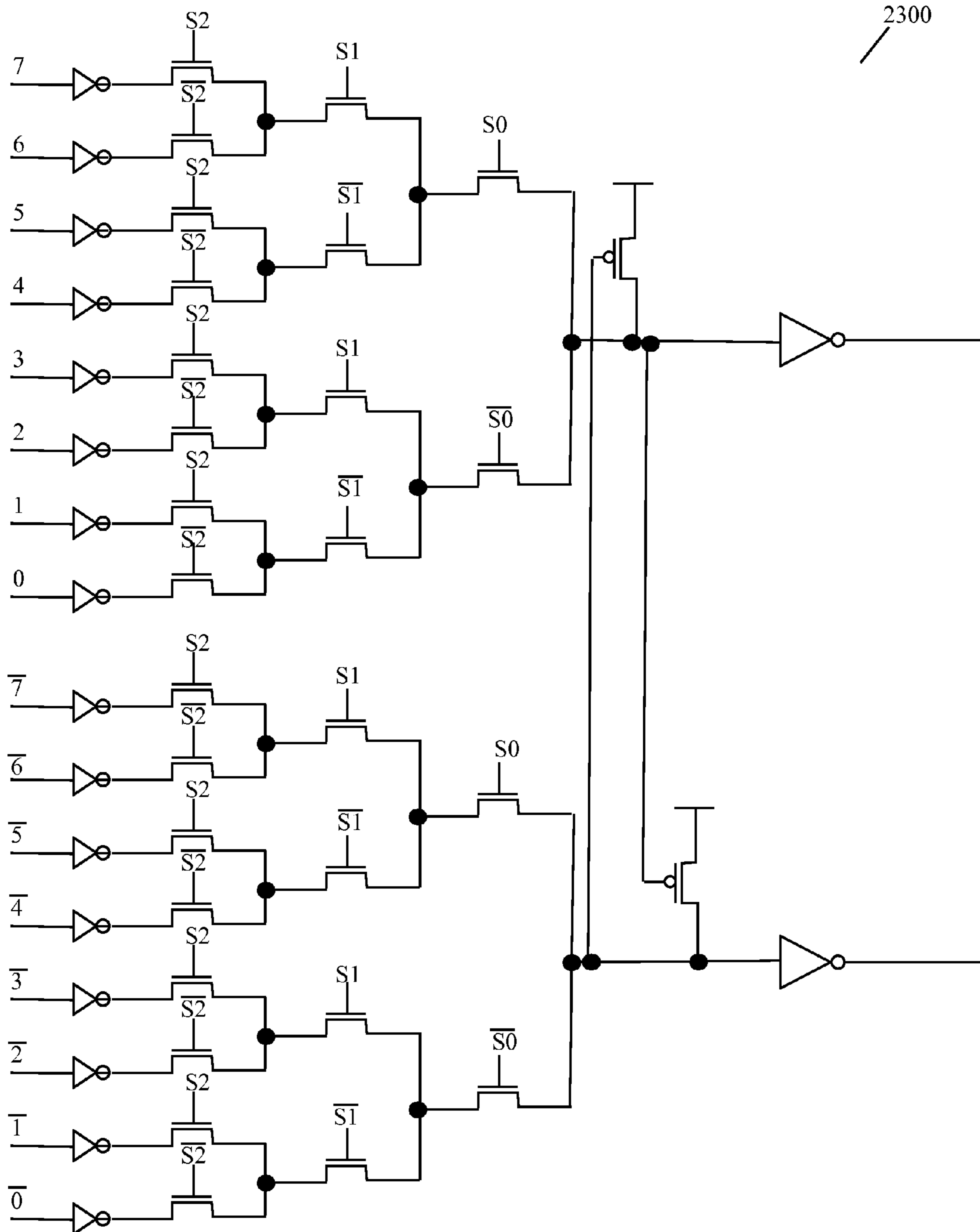
Figure 23 Prior Art
