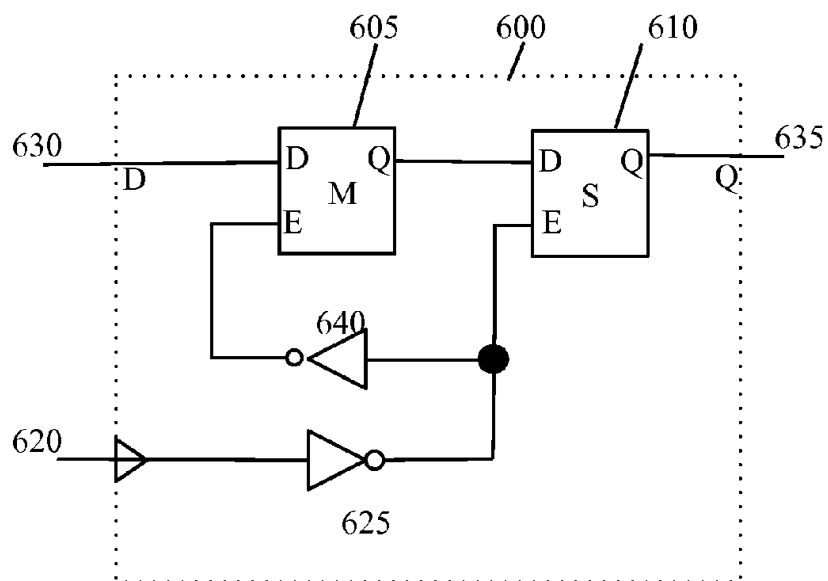
Figure 6 Prior Art
