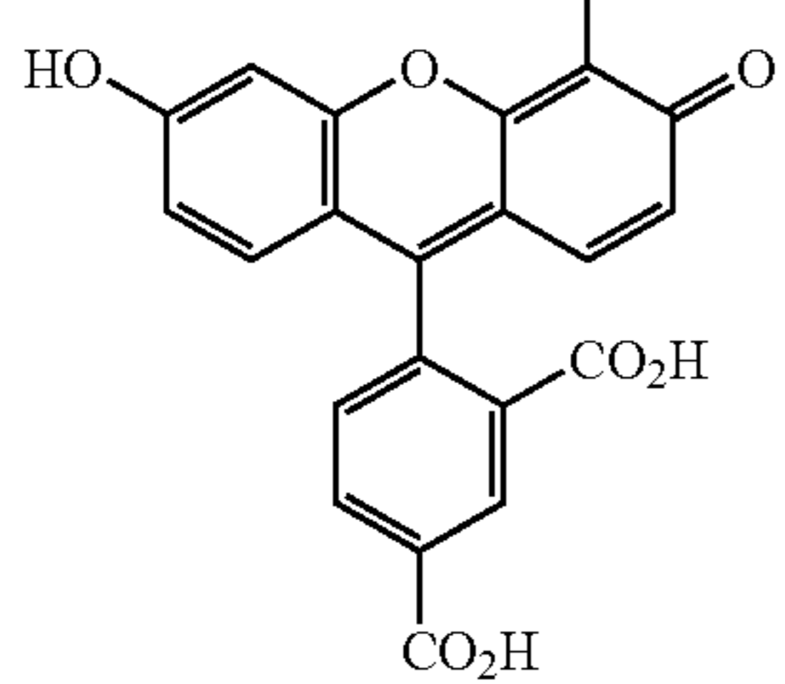
5-TMR-F-CF
