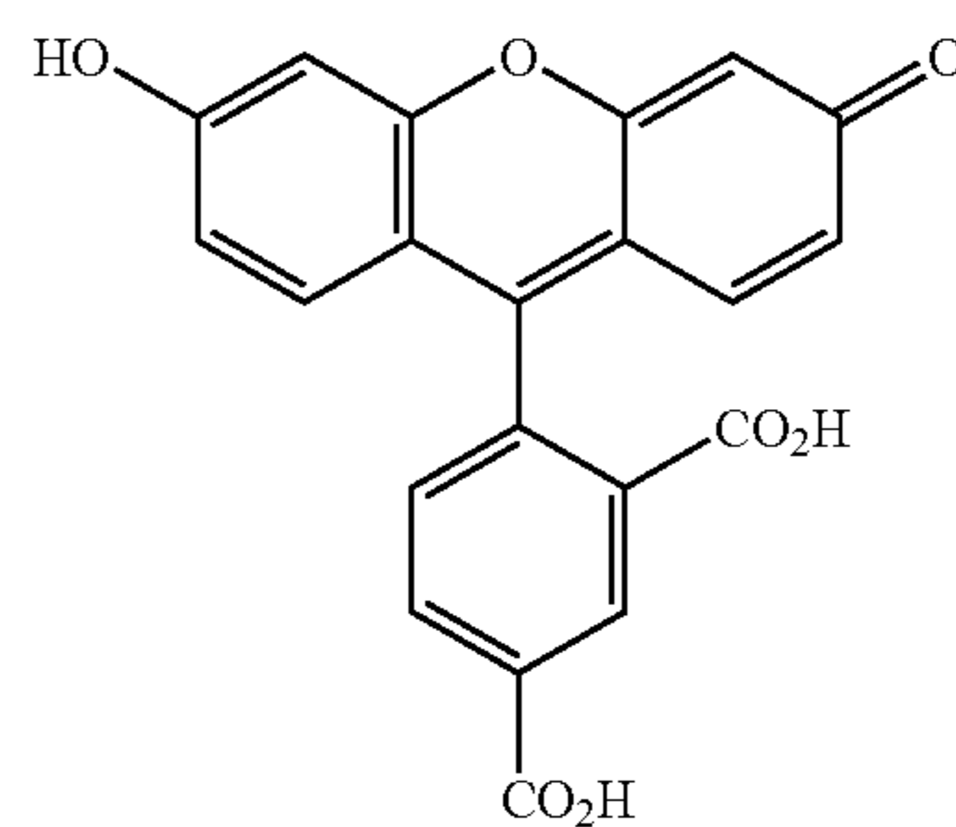
5-carboxyfluorescein
