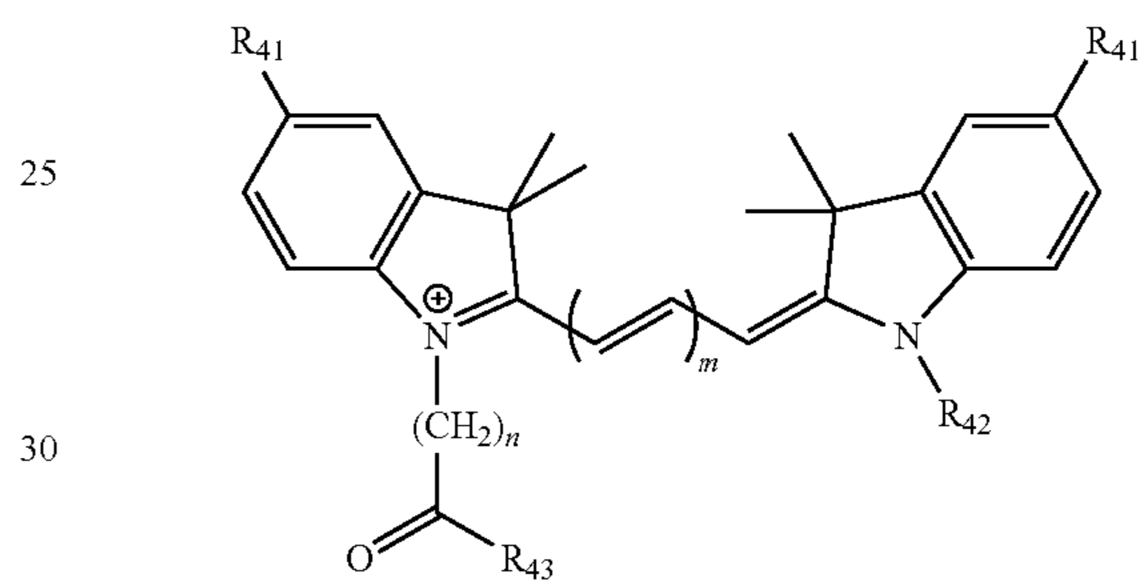
CYANINE
