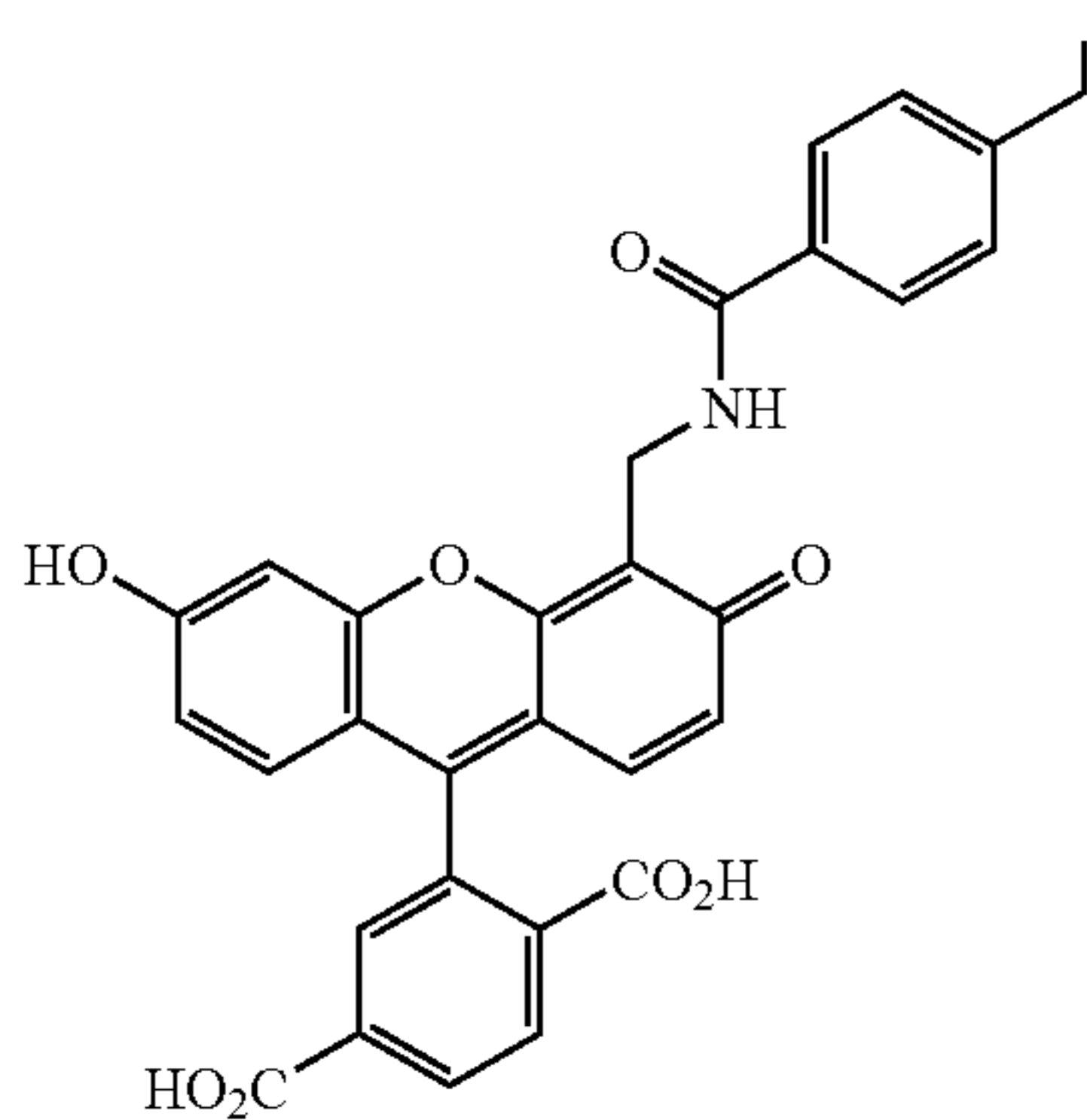
6-CFB-DR110-2
