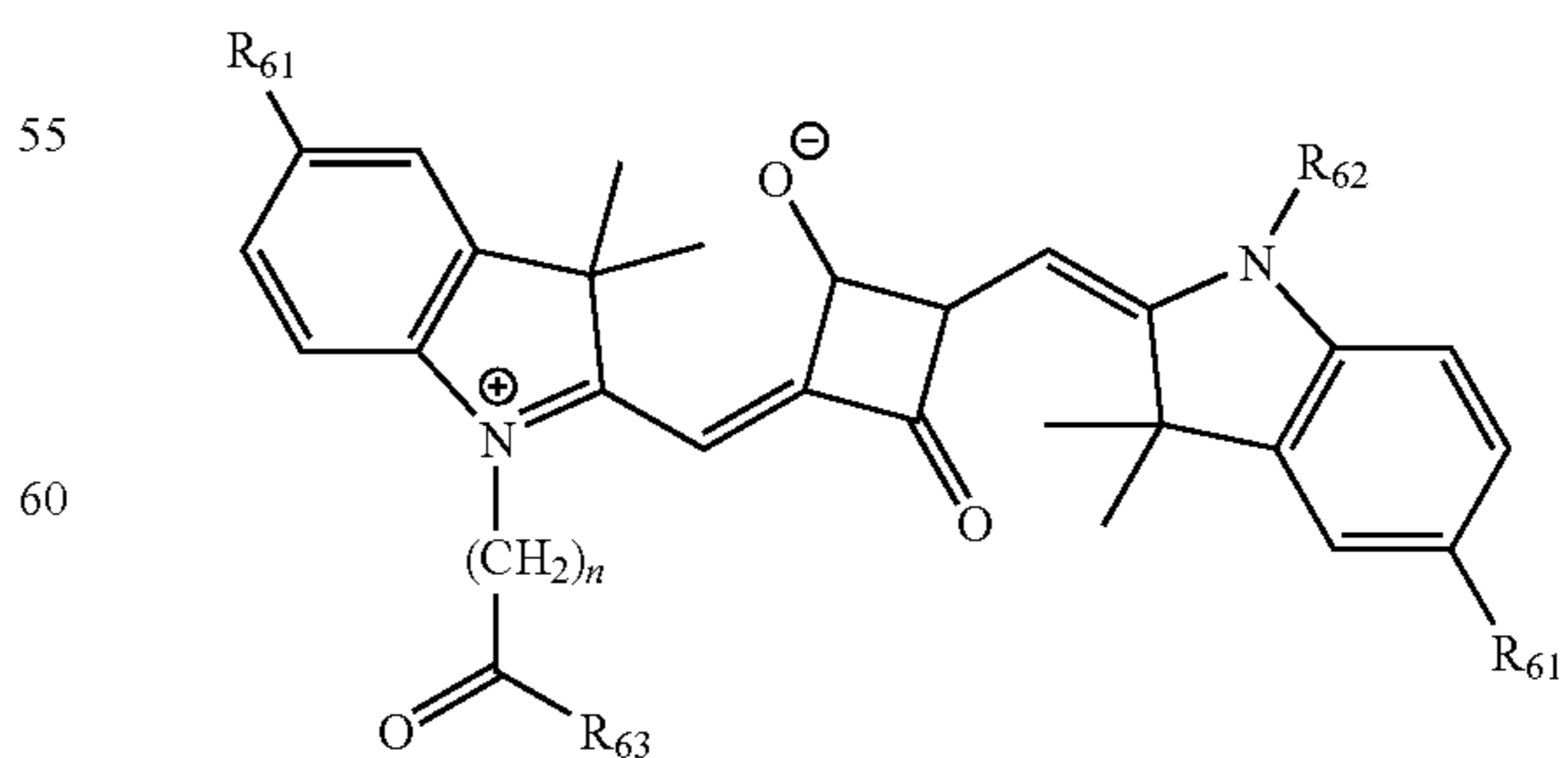
SQUARINE
