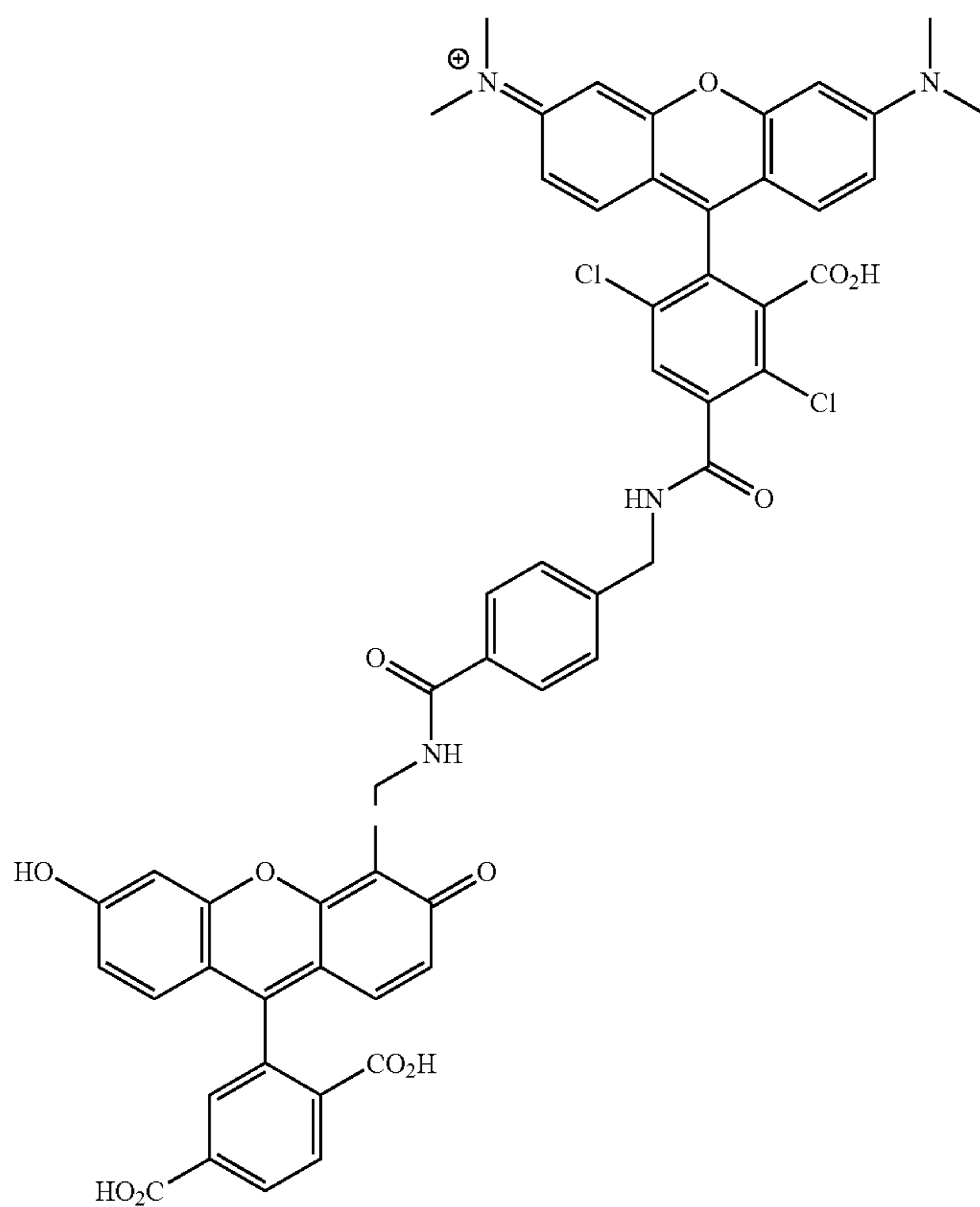
6-CF-B-DTMR-2
