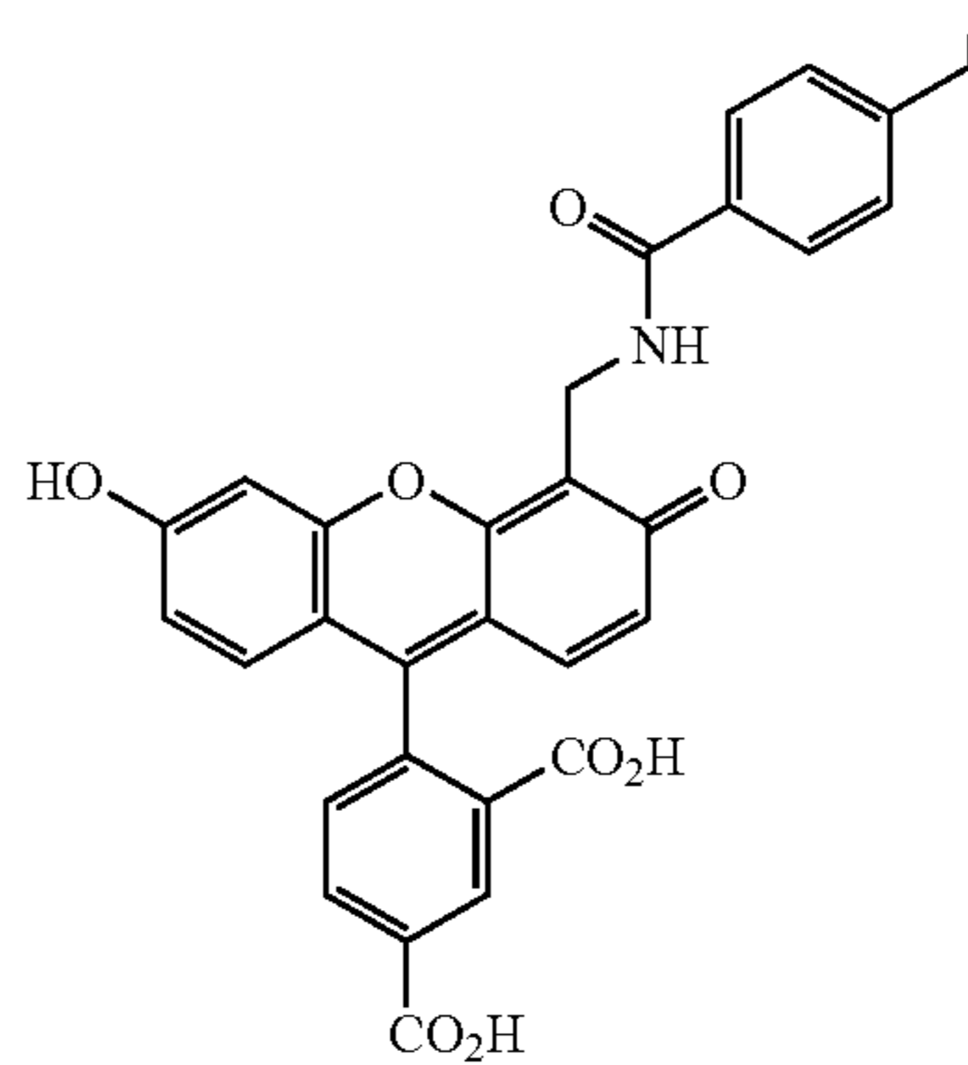
5-CFB-DTMR-2
