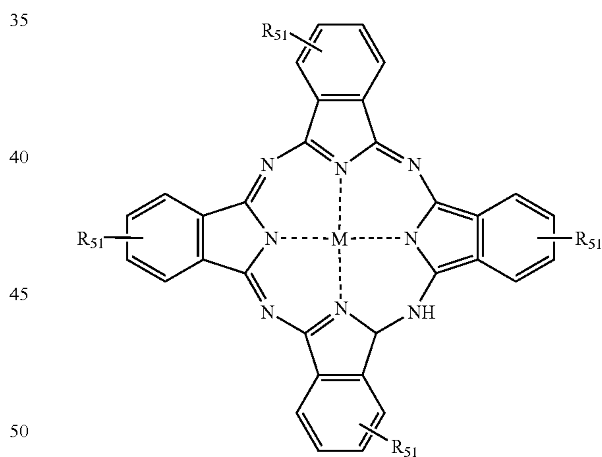
PHTHALOCYANINE
