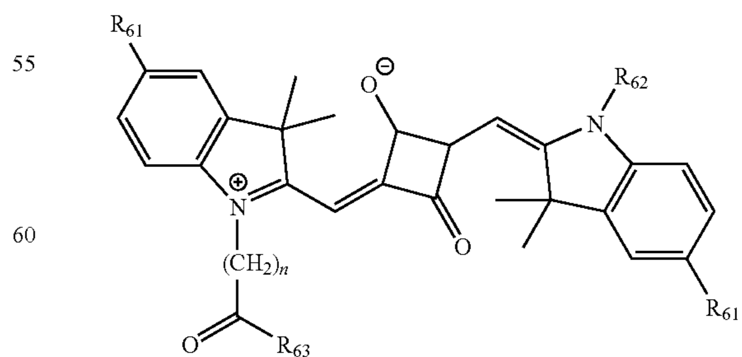
SQUARINE
