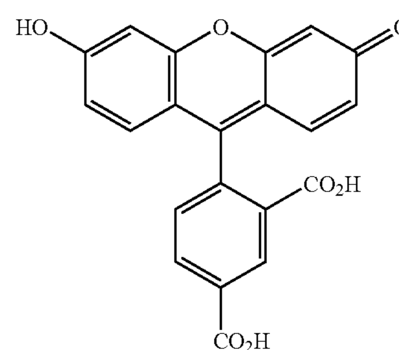
5-carboxyfluorescein
