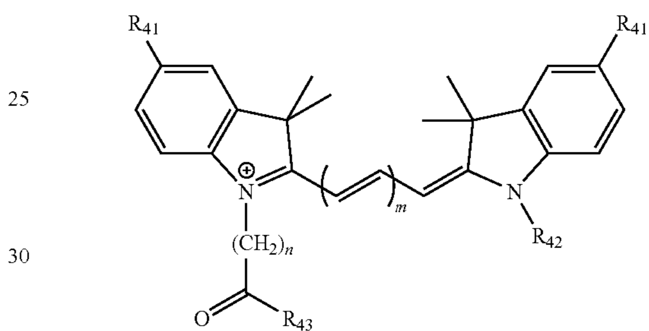
CYANINE
