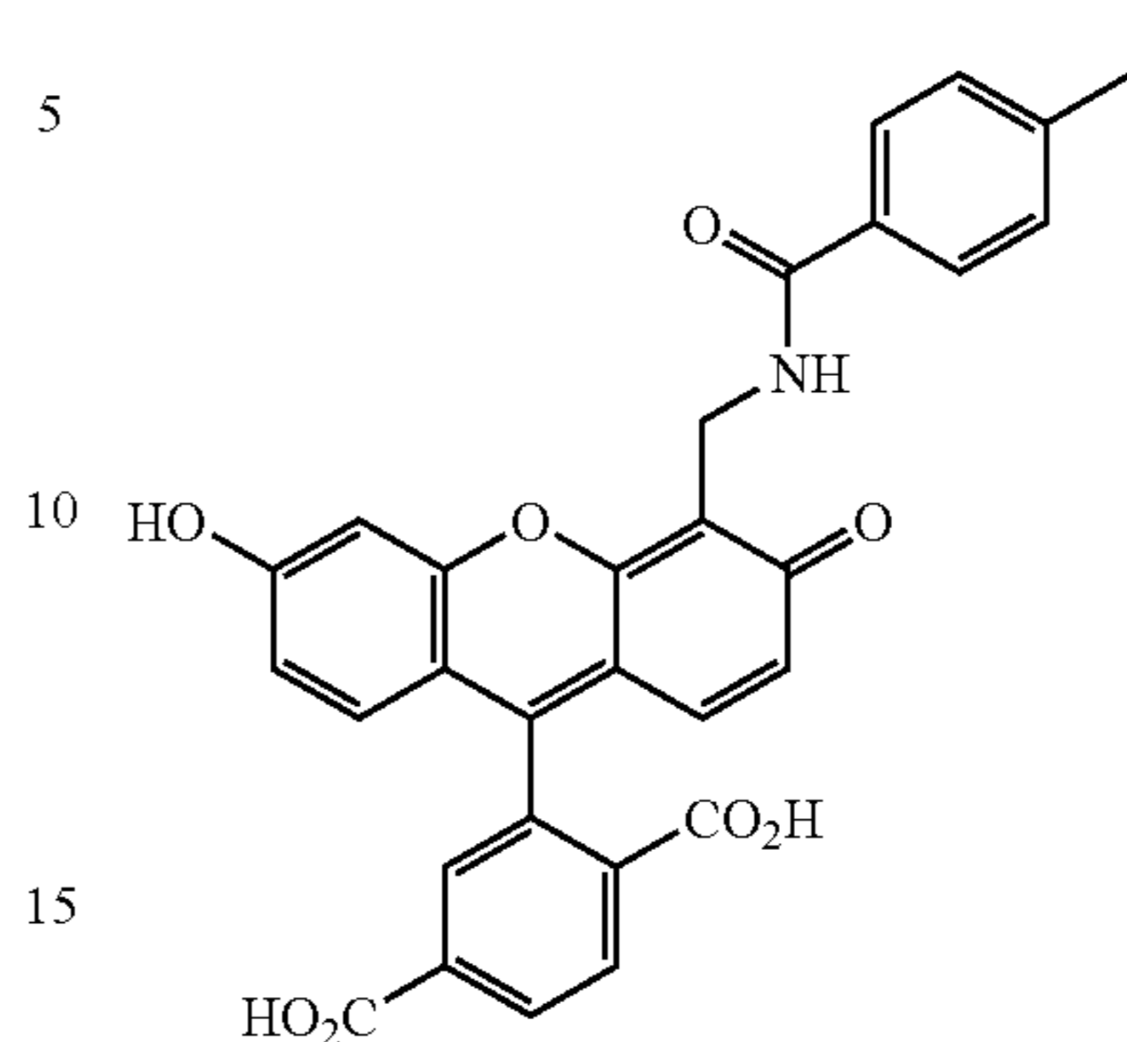
6-CFB-DR6G-2
