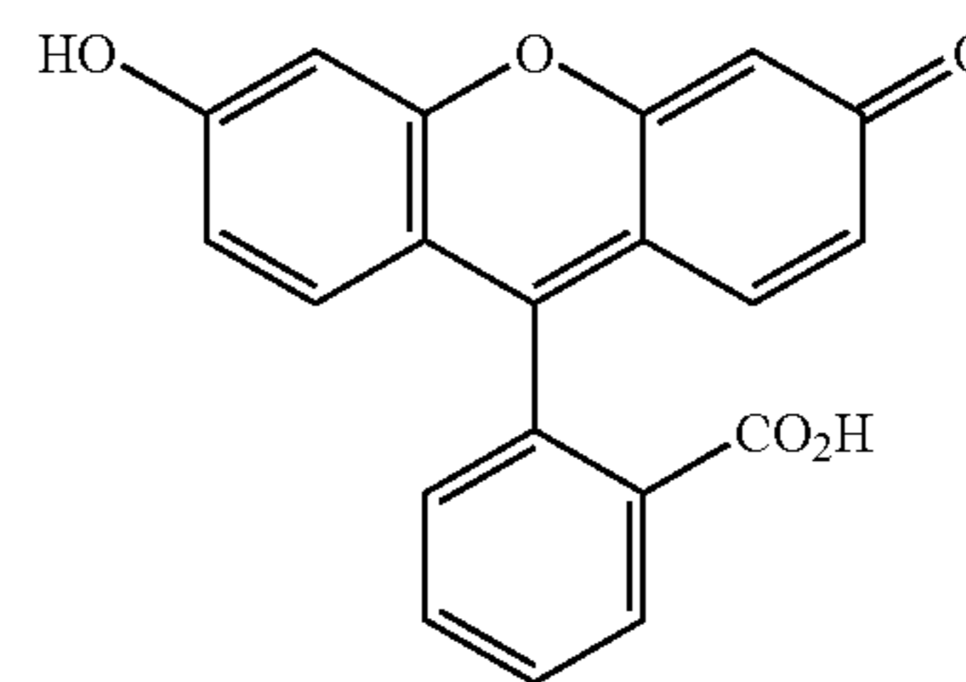
Fluorescein
