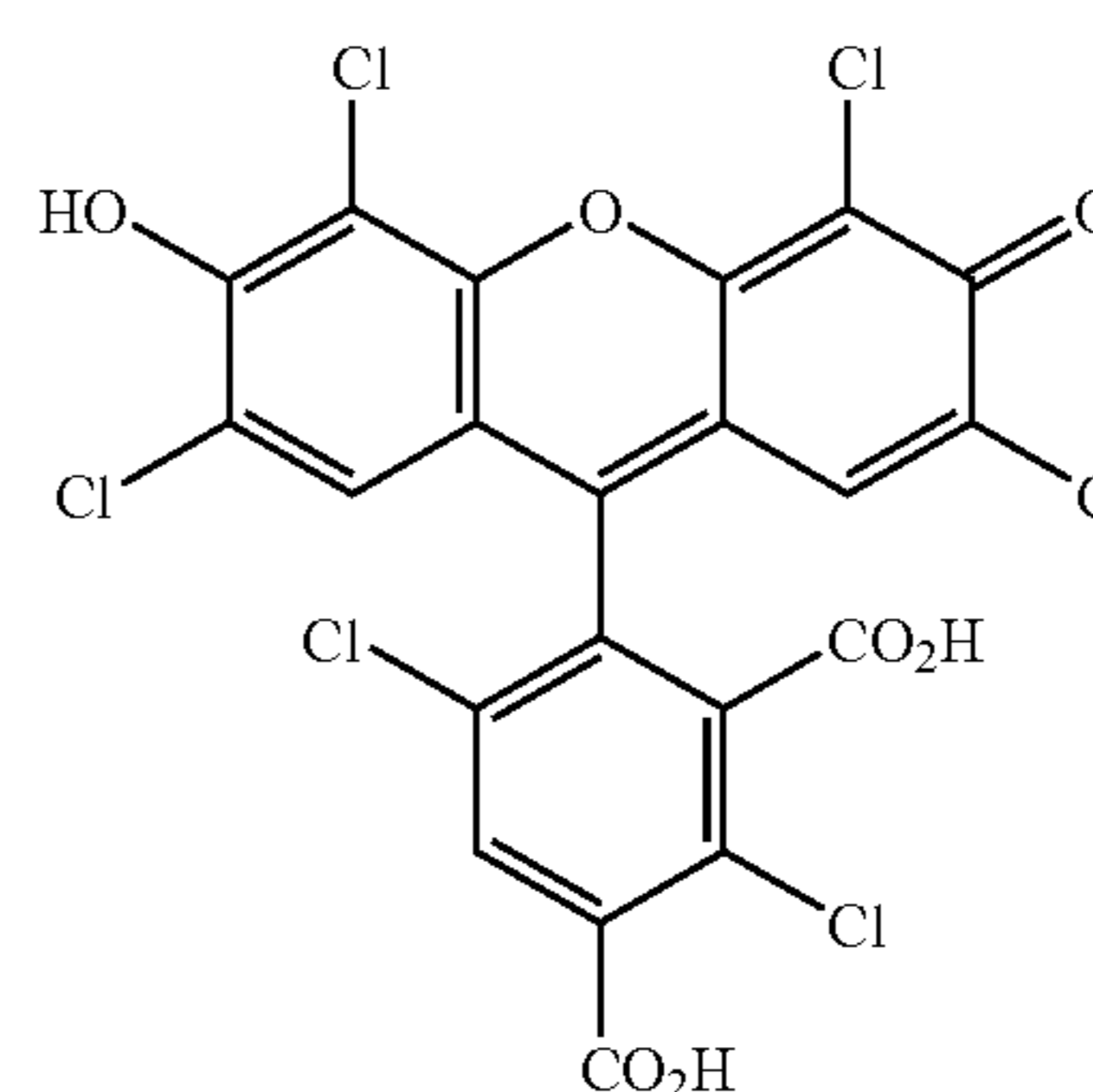
5-carboxy-HEX
