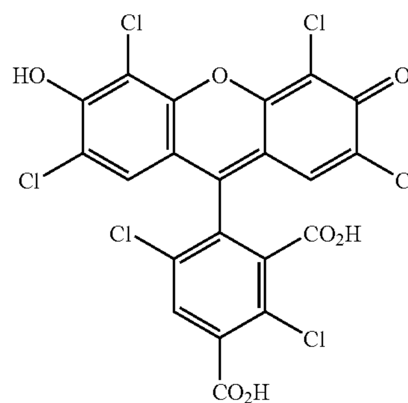
5-carboxy-HEX
