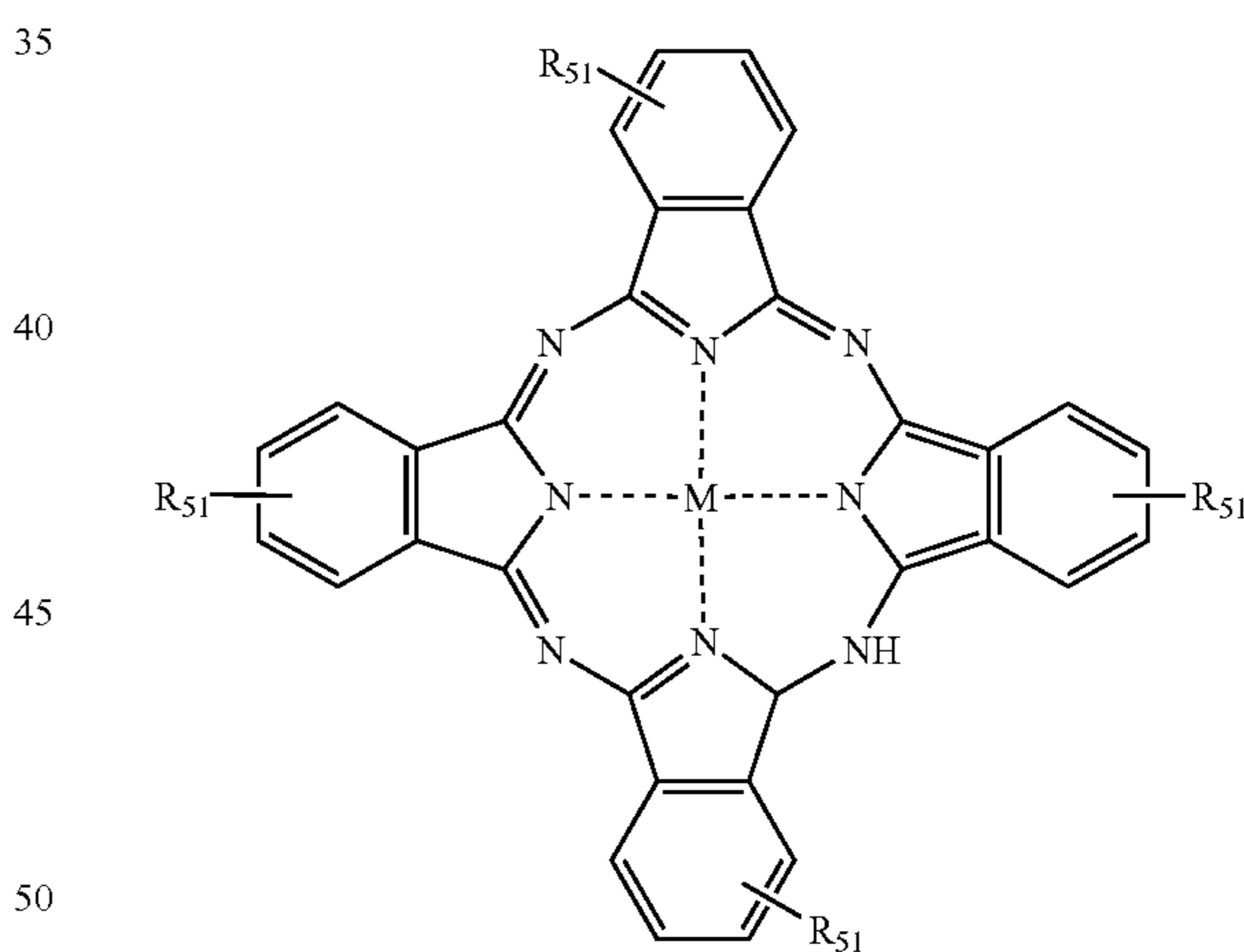
PHTHALOCYANINE
