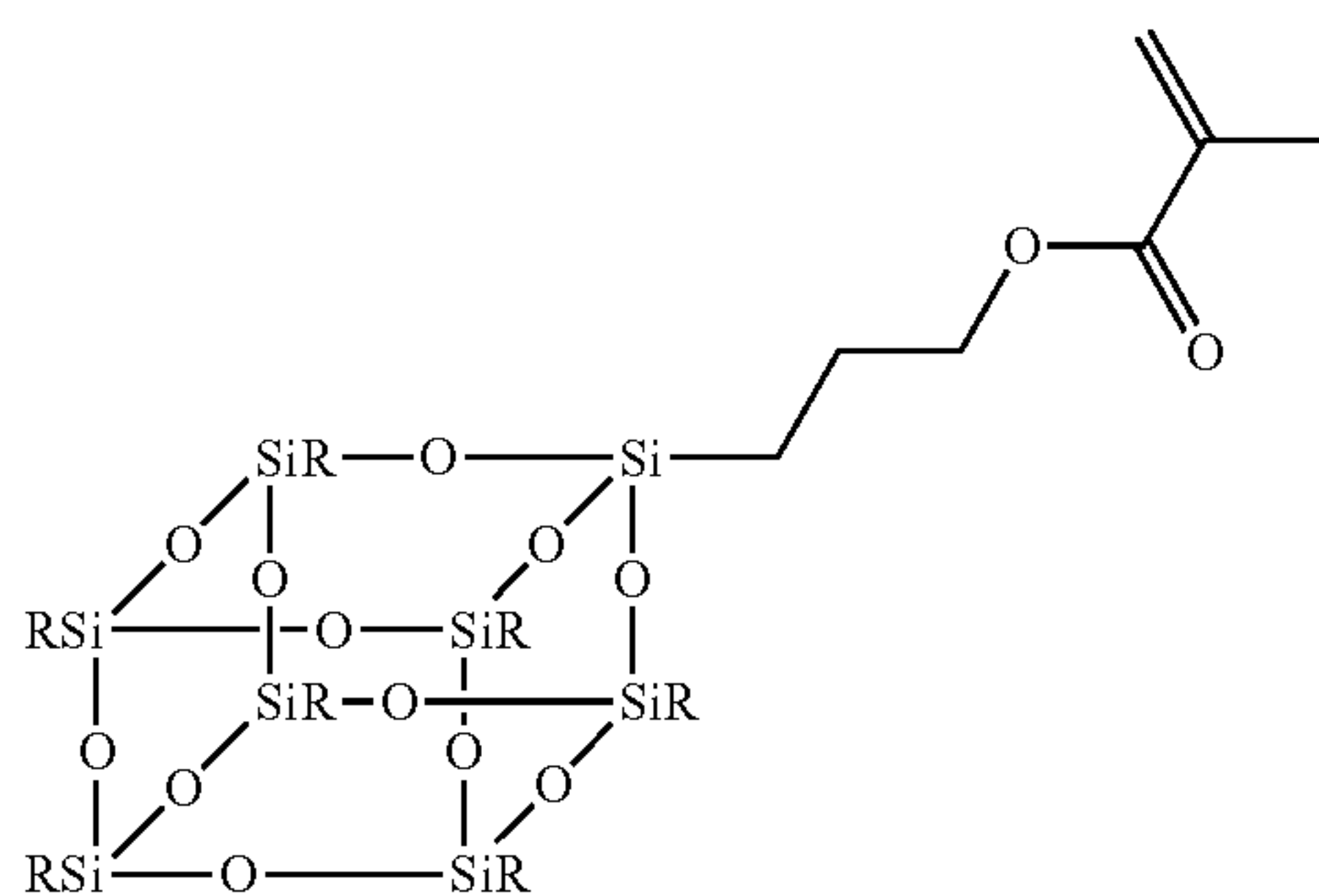
Scheme 10: POSS Monomers for ATRP
