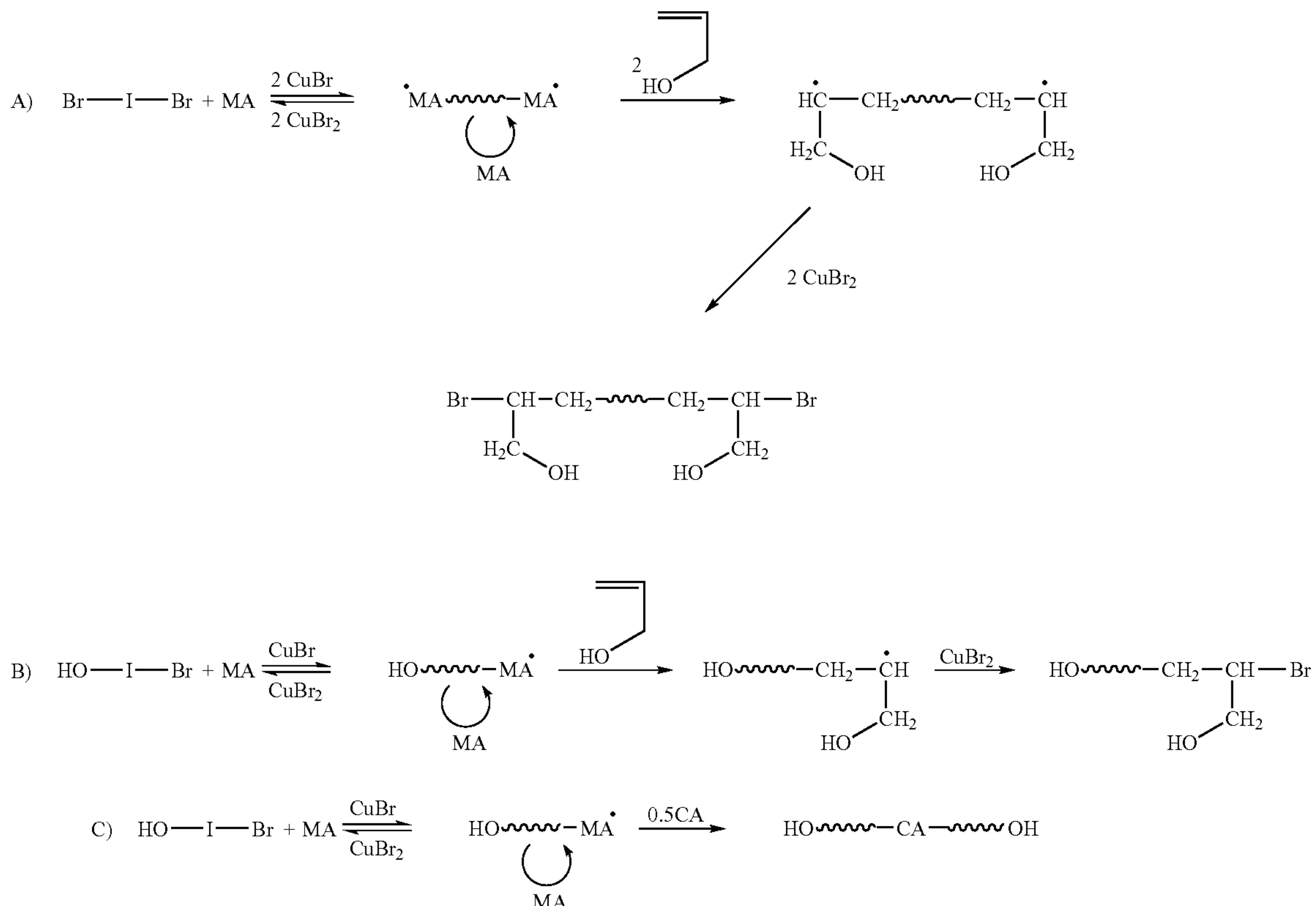
Scheme 4. Formation of telechelic diols
