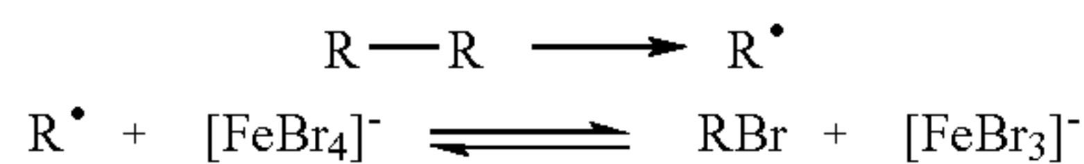
Scheme 2 “Reverse” ATRP with transition metal salts
