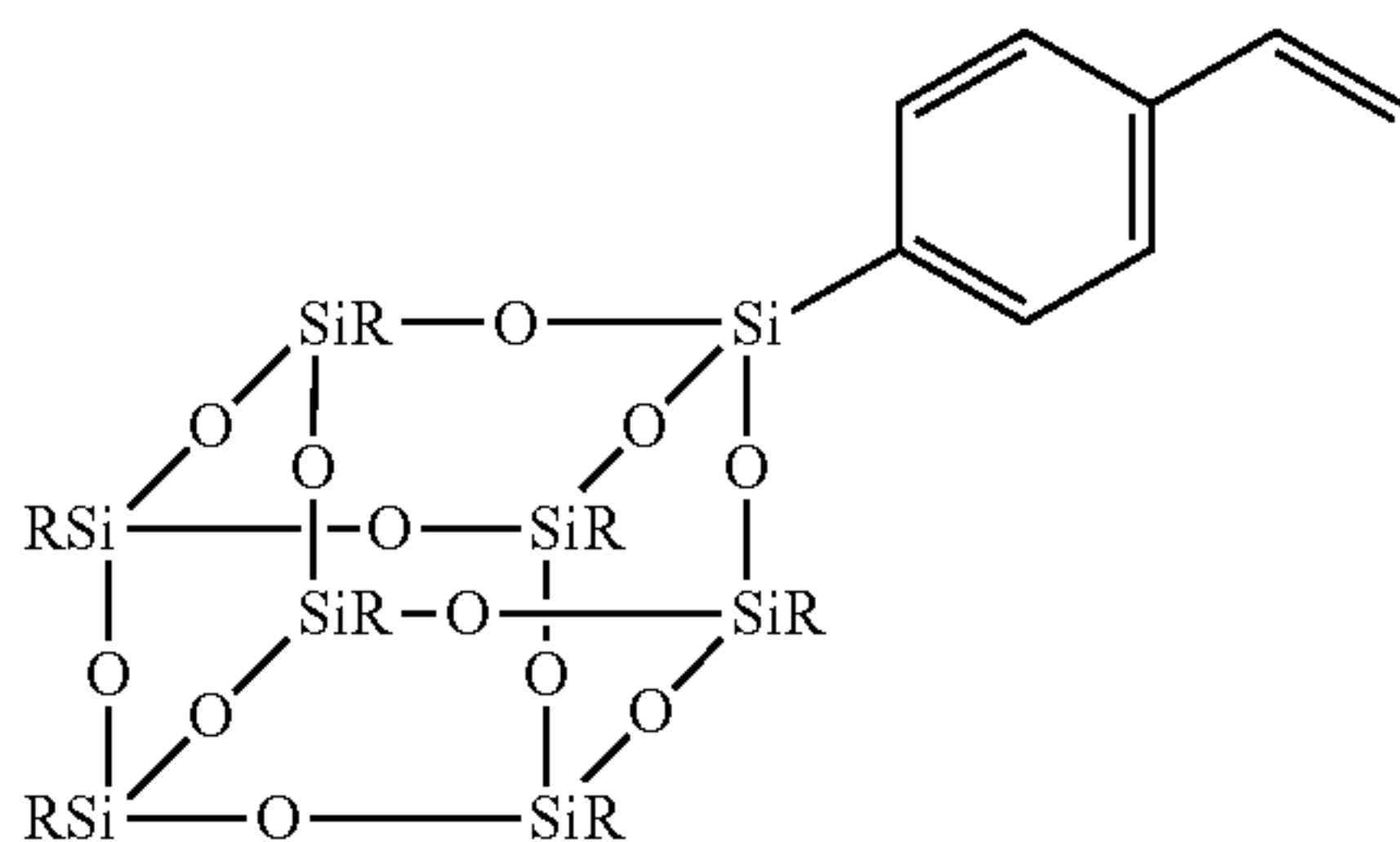
Styryl-POSS (Sty-POSS)
