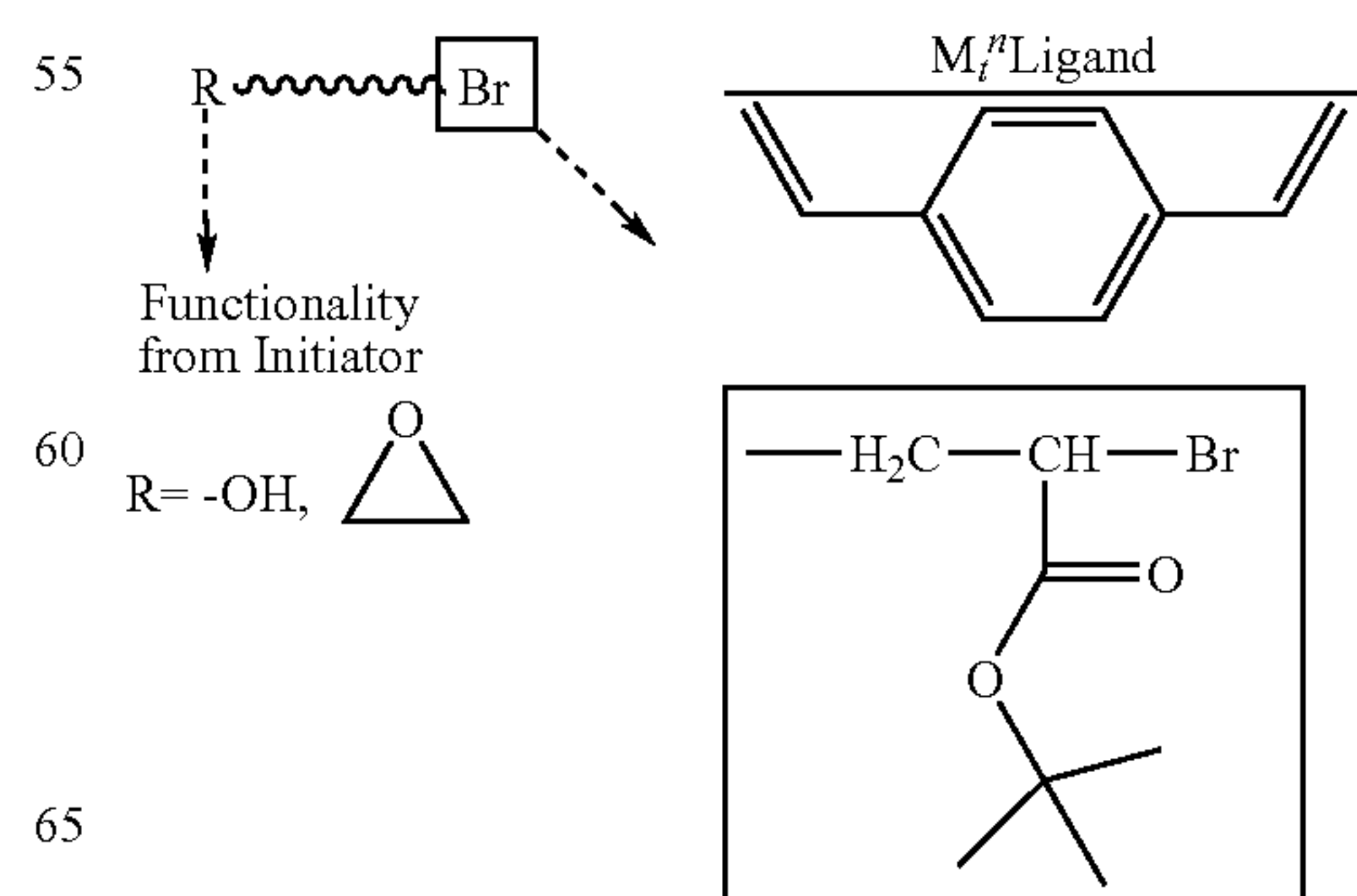
Scheme 7: Functional Stars from ATRP
