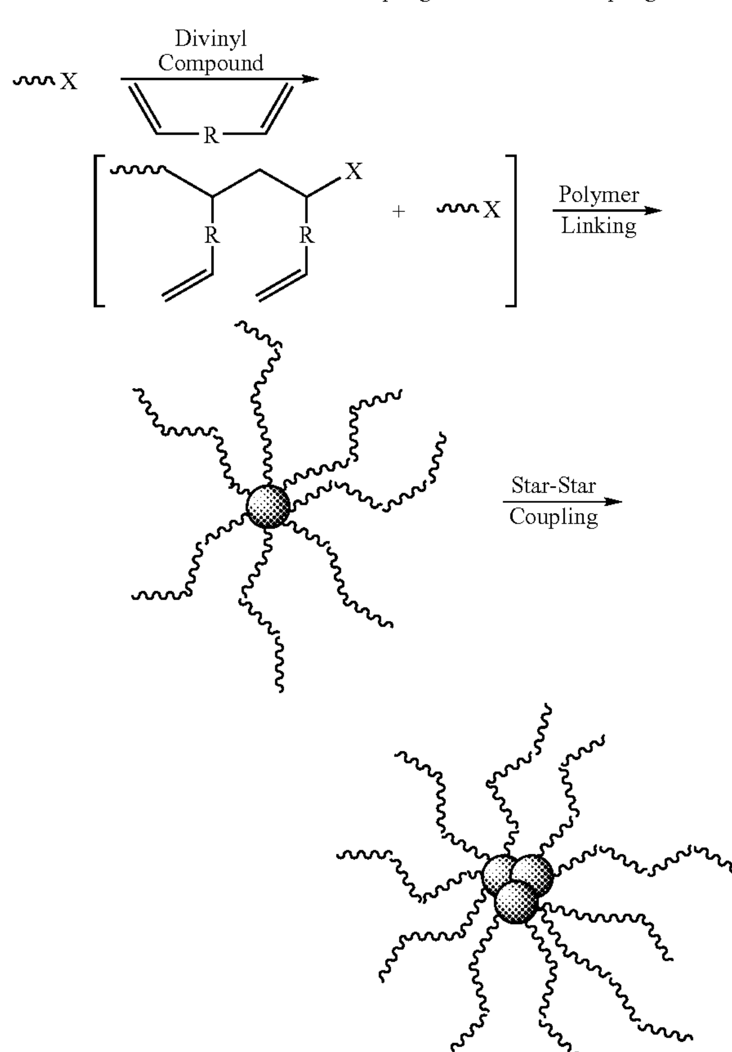
Scheme 5 Arm First Star Coupling and Star-Star Coupling.
