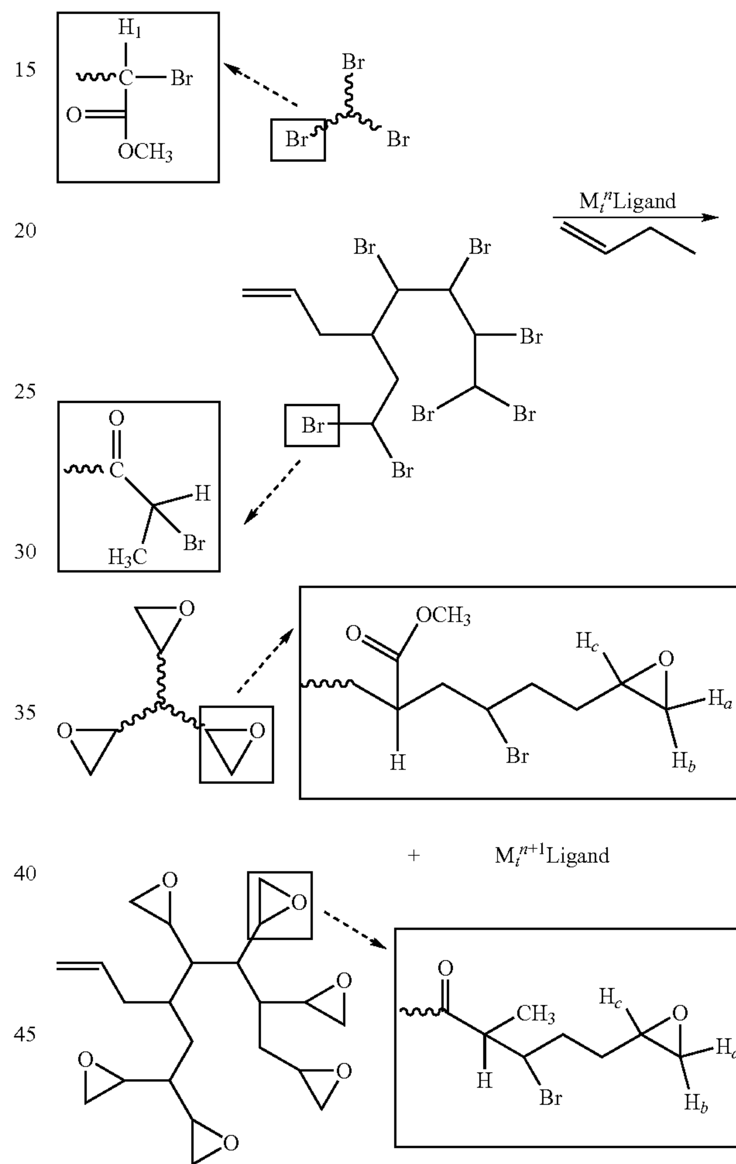
Scheme 6: Functionalization of Stars and Hyperbranched Polymers by ATRA
