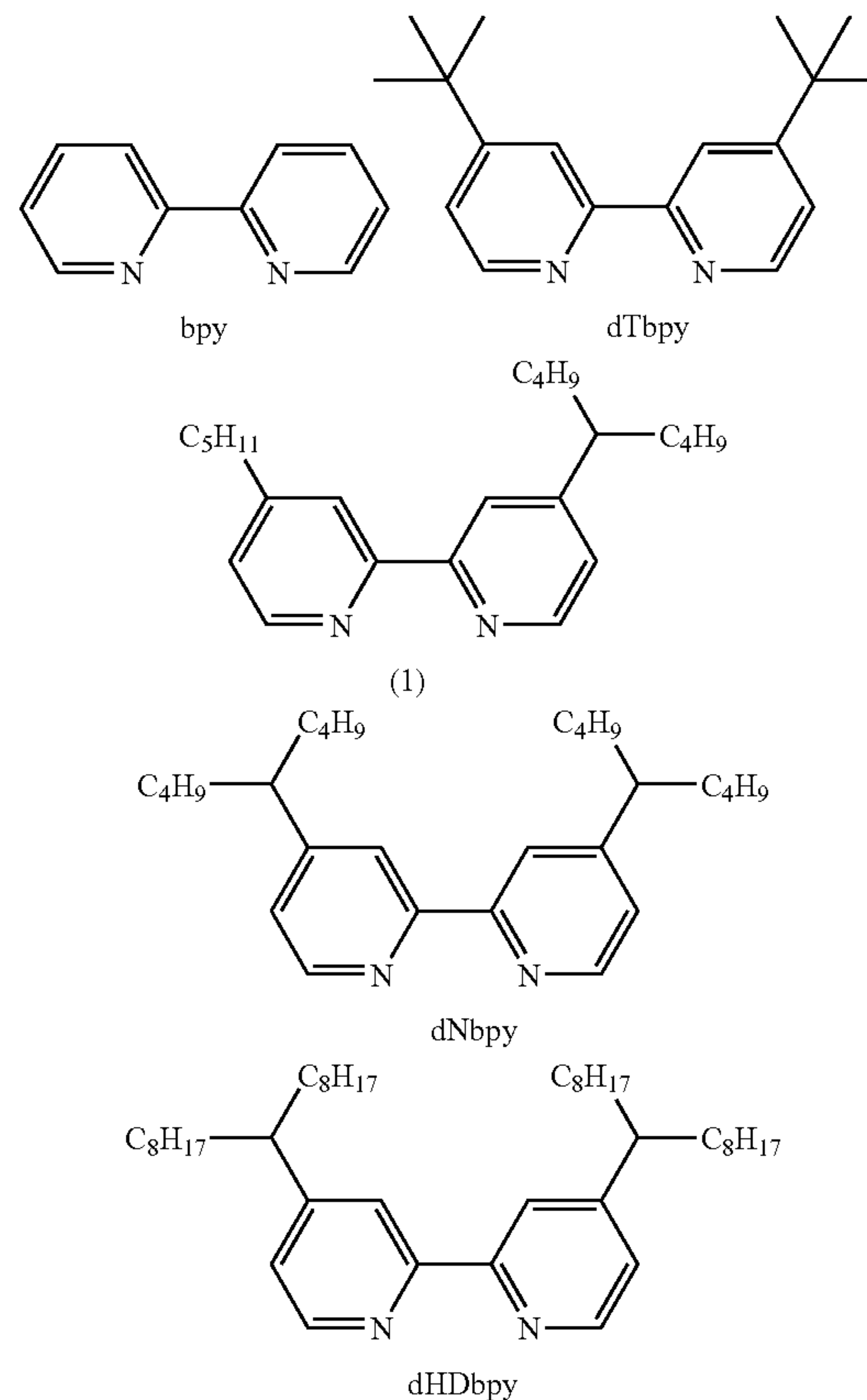
Scheme 8: Bipyridene based ligands
