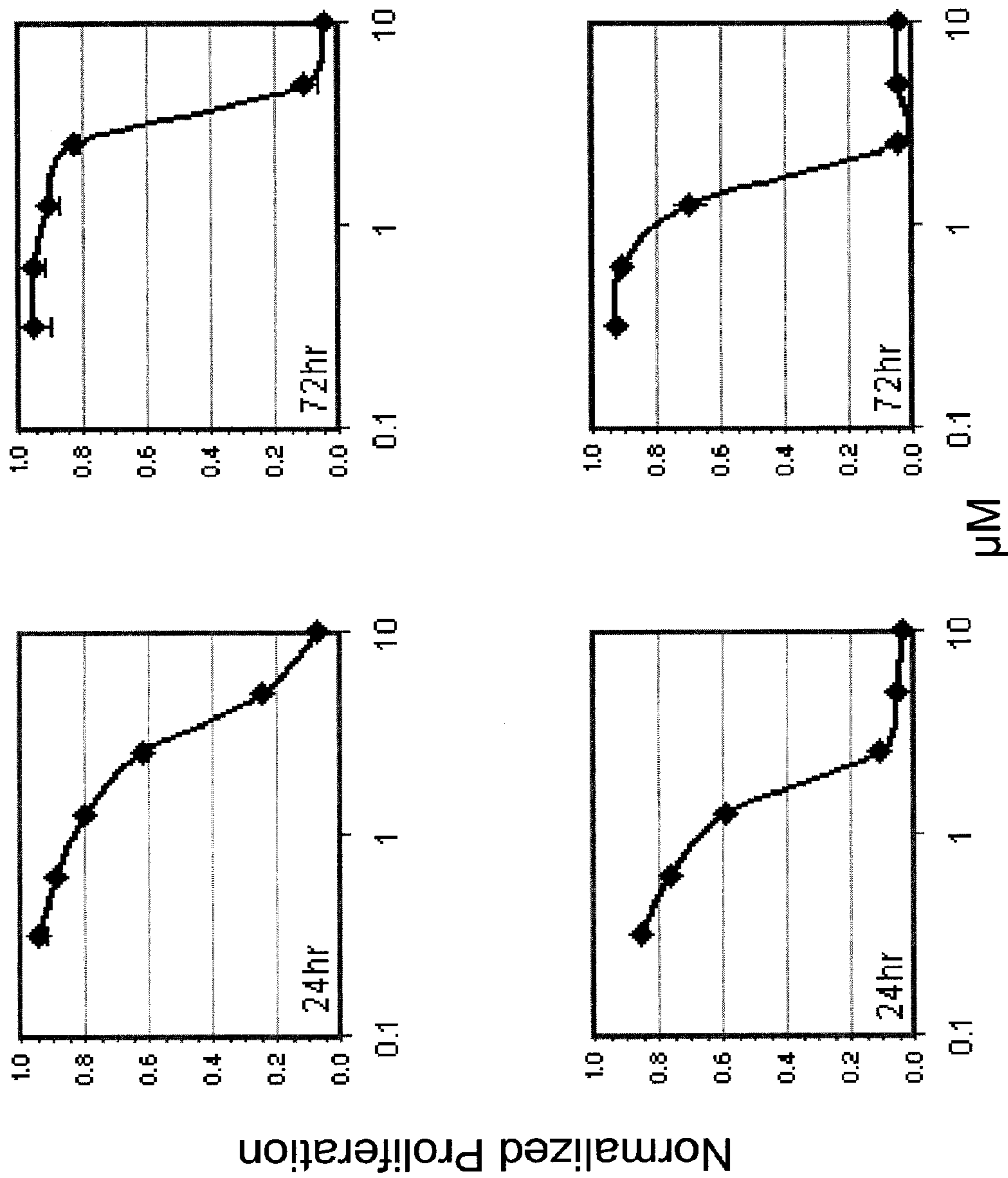
Compound 15
