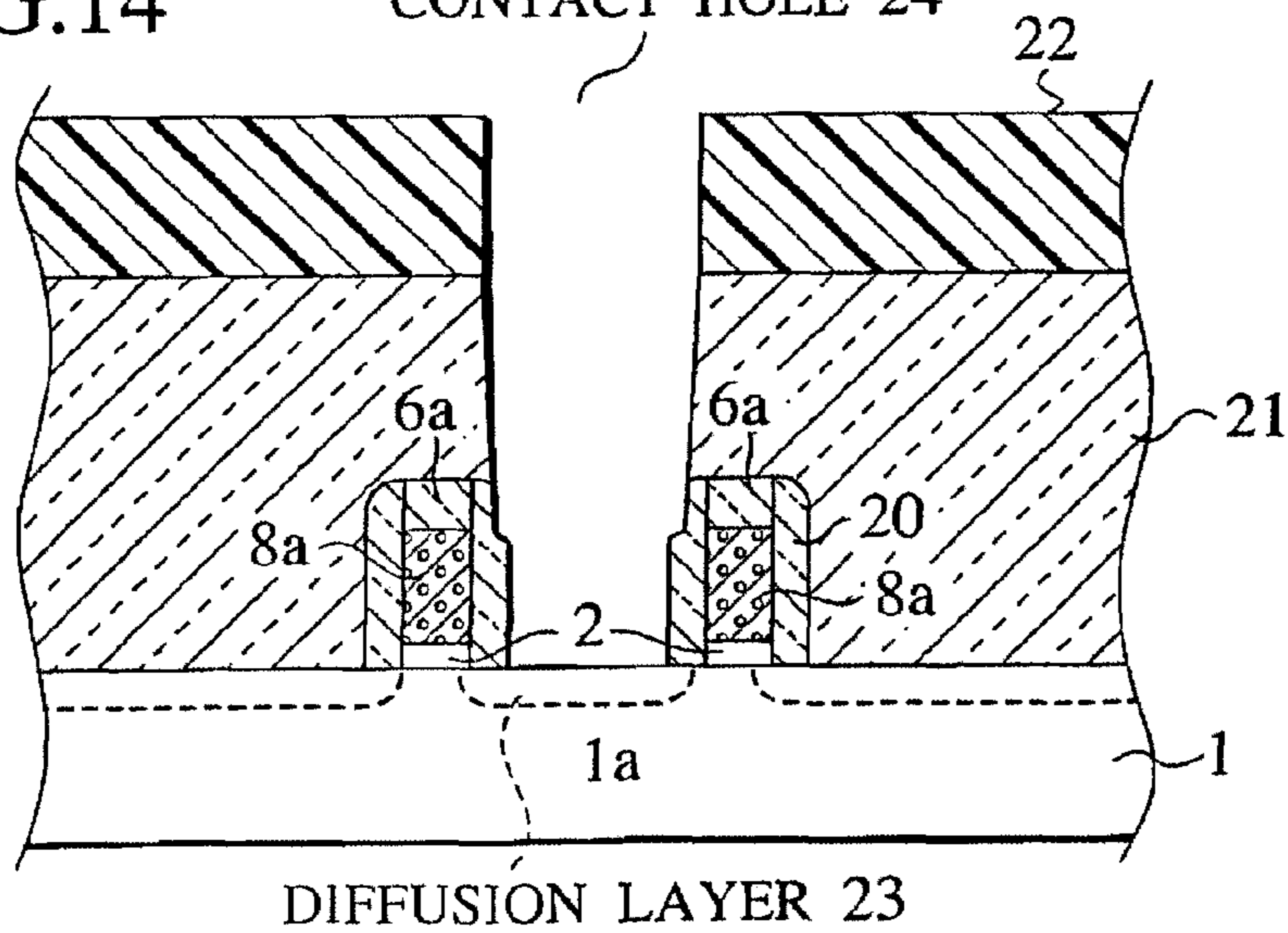
CONTACT HOLE 24
