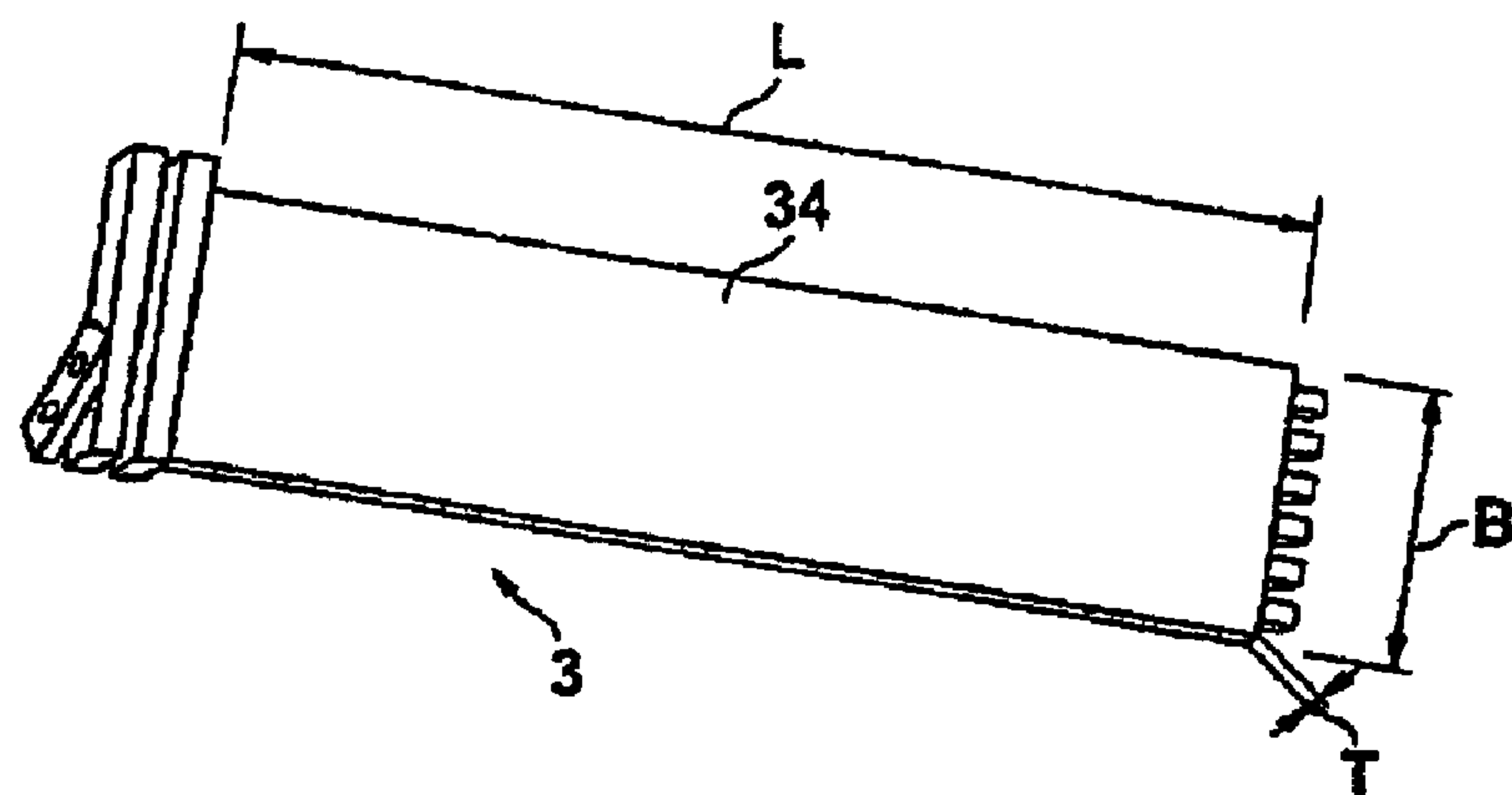
FIG. 5c (Conventional Art)
