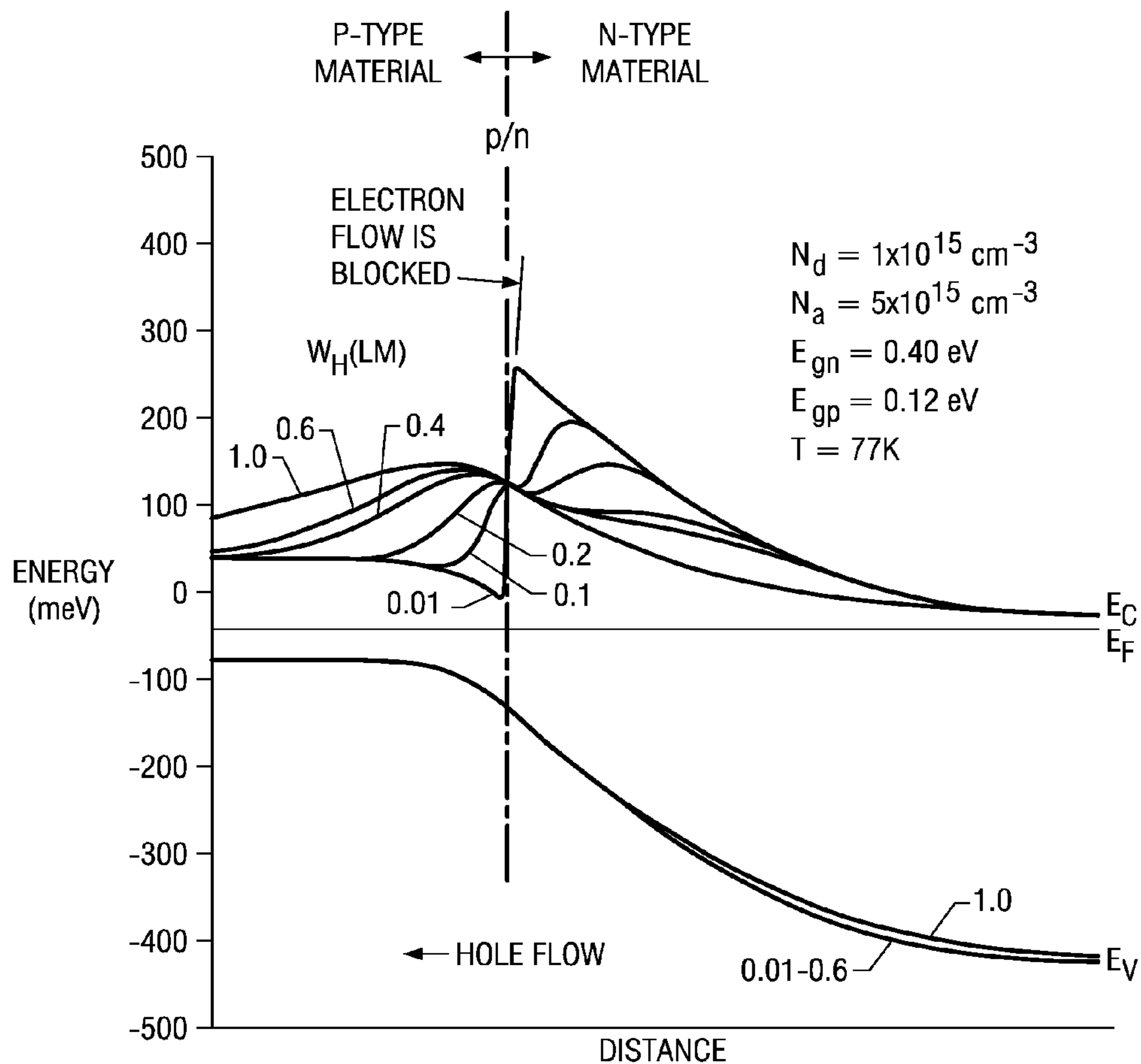
FIG. 3 (PRIOR ART)
