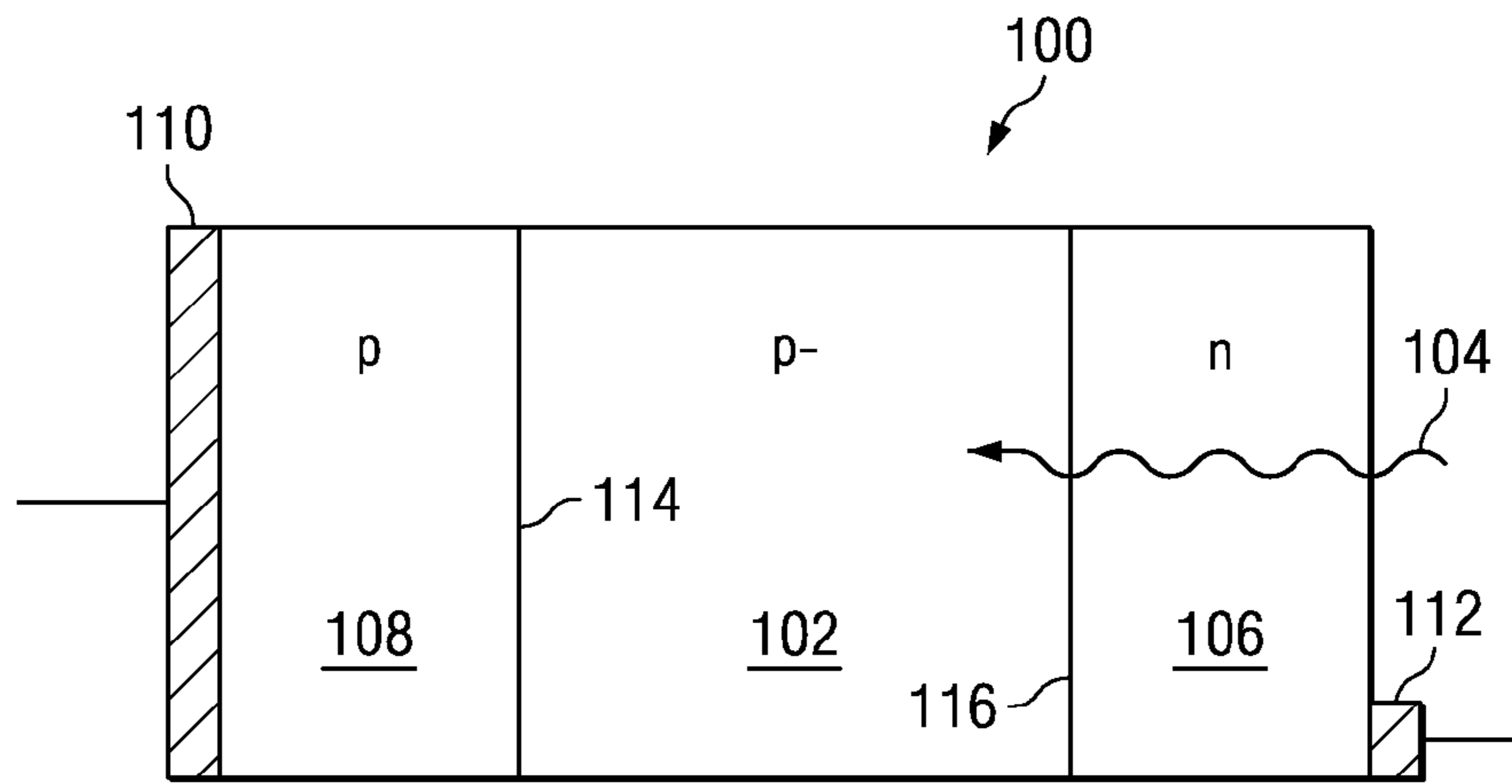
FIG. 1 (PRIOR ART)
