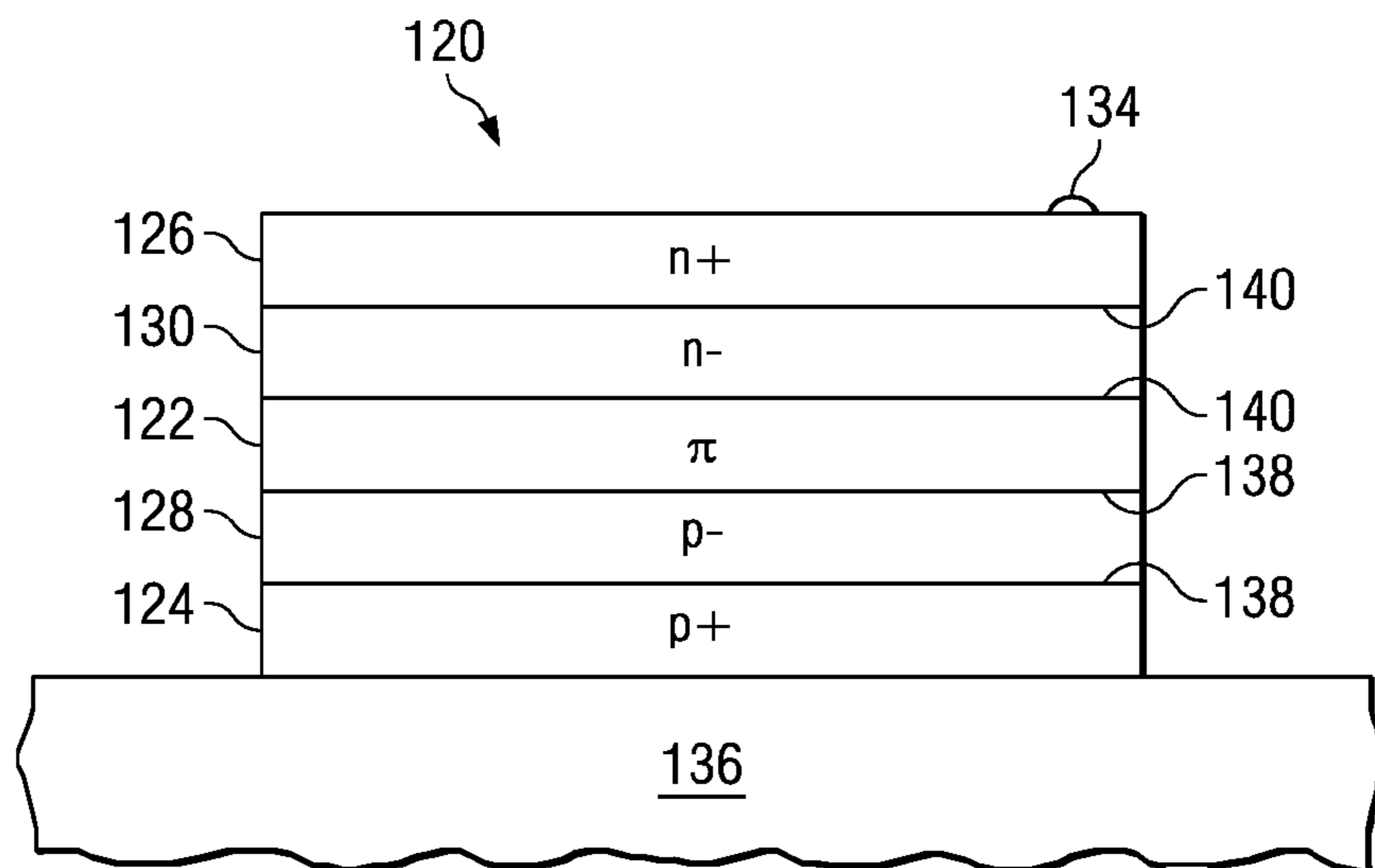
FIG. 2 (PRIOR ART)
