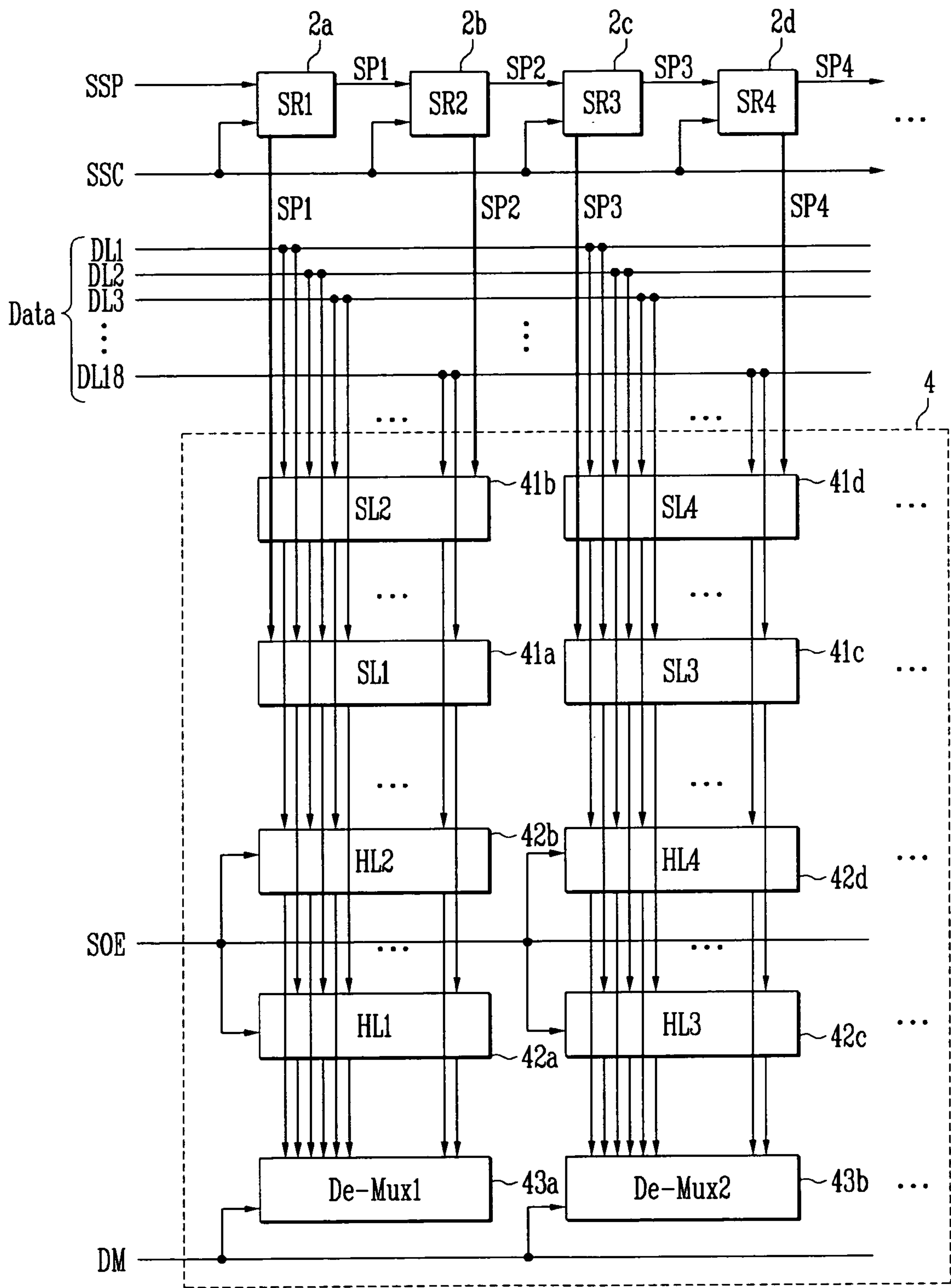
FIG. 2 (PRIOR ART)
