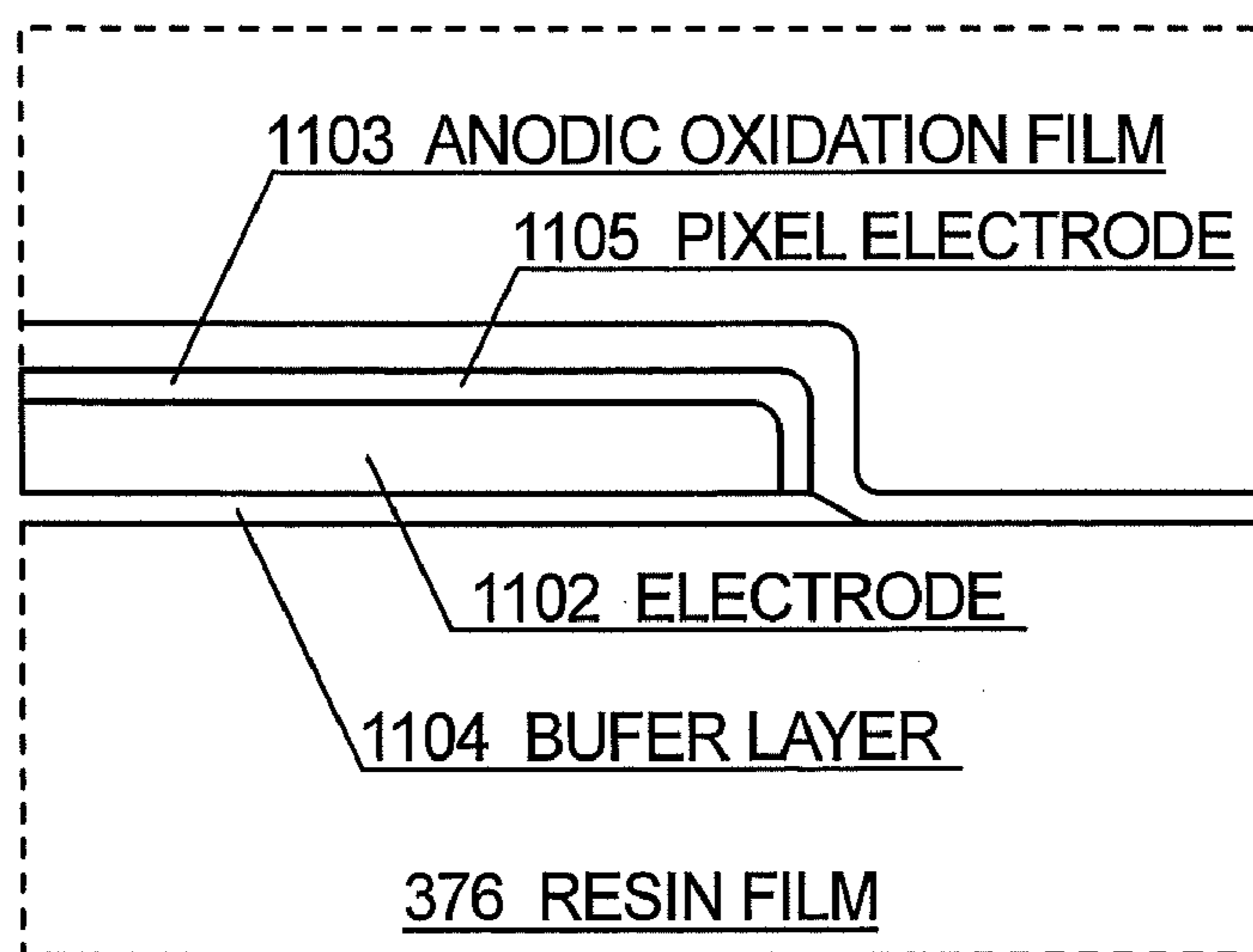
SCHEMATIC DIAGRAM OF ENLARGED ELECTRODE EDGE PORTION
