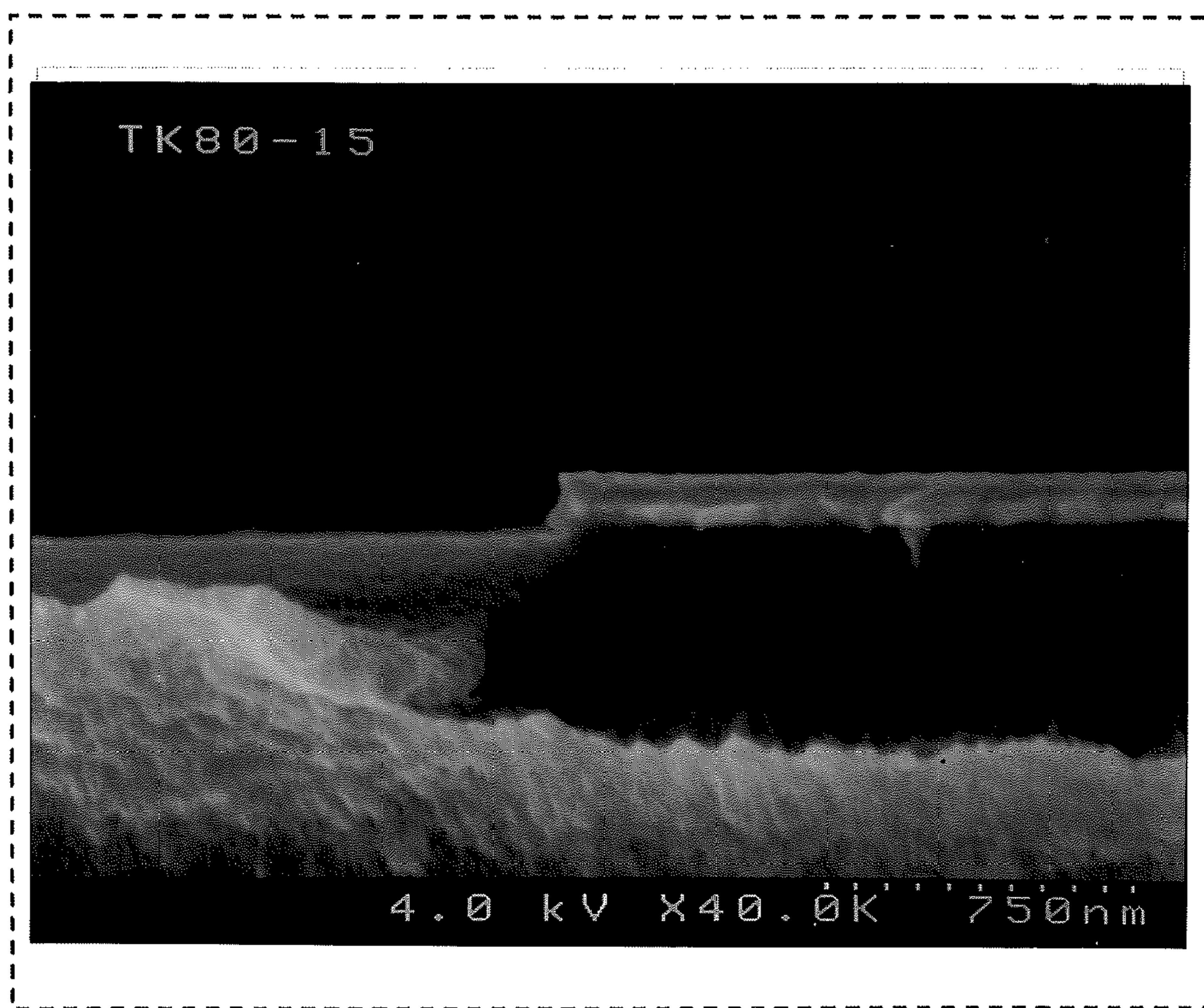
FIG. 1A SEM PHOTOGRAPH (CROSS SECTION)
