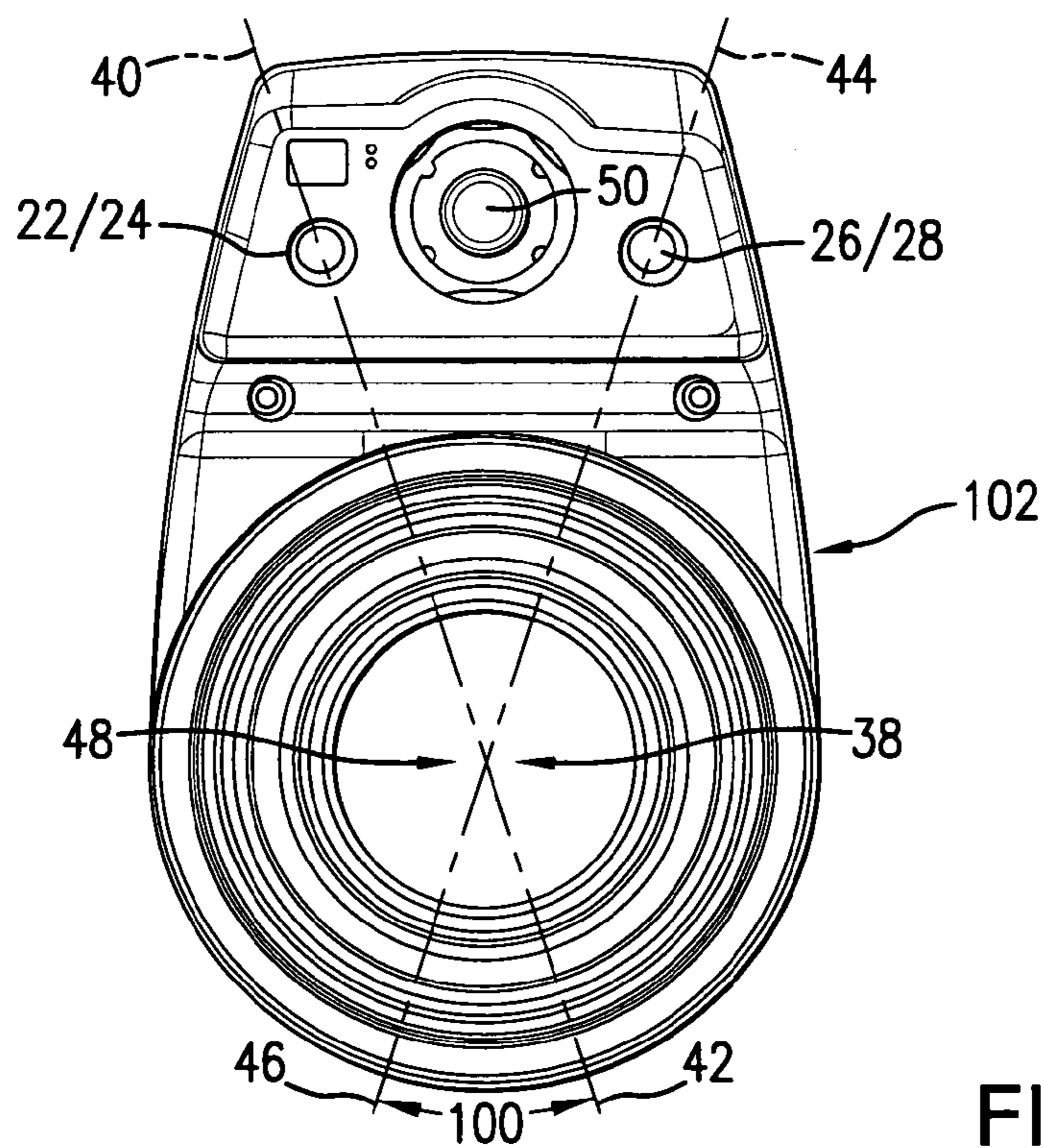
Front View of Camera
