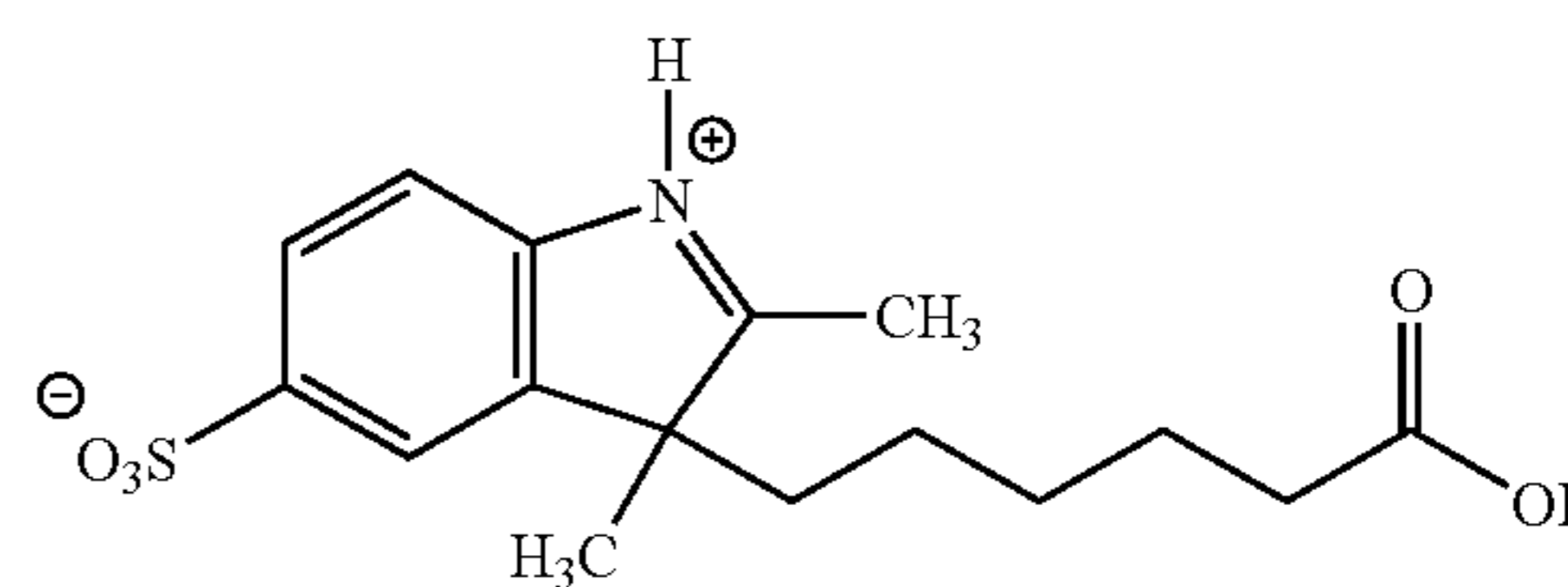
Compound 1
