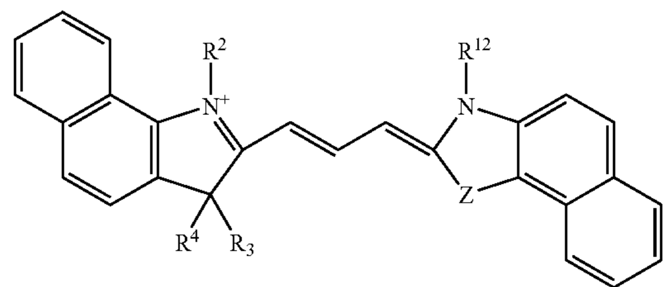
Formula XX
