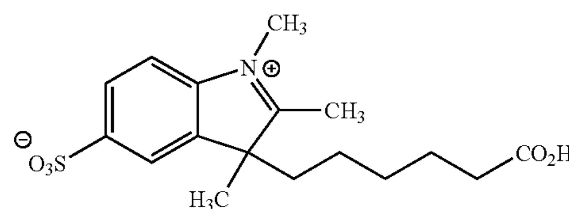
Compound 7
