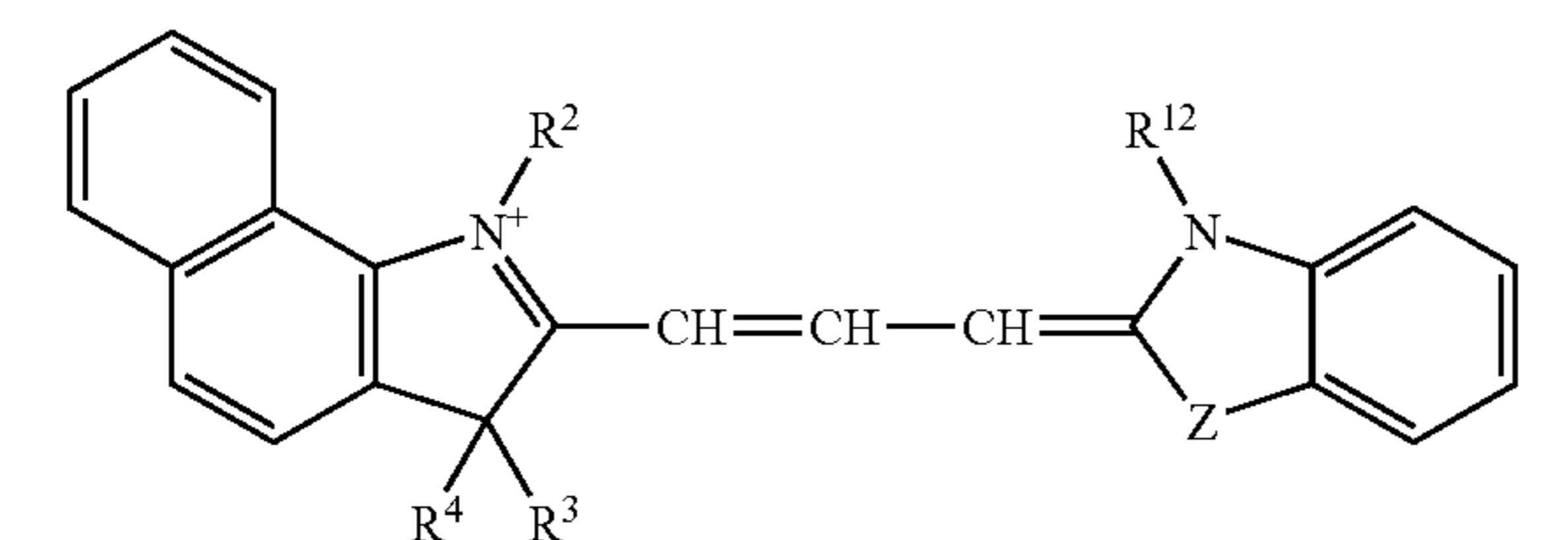
Formula XVI
