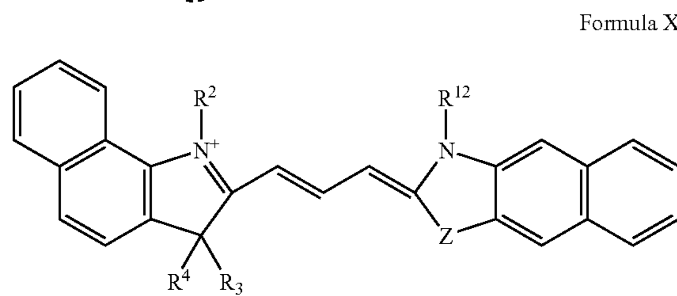
Formula XX
