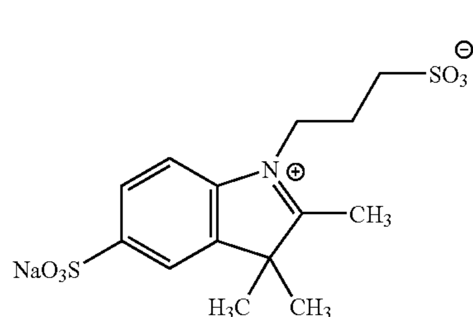
Compound 3A
