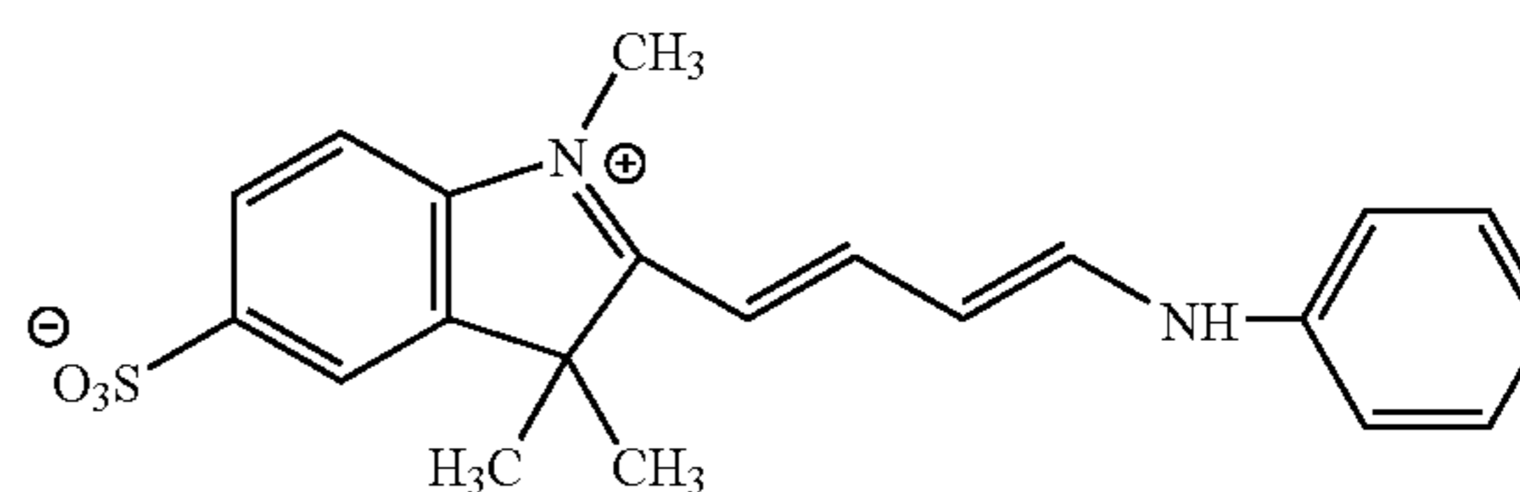
Compound 6
