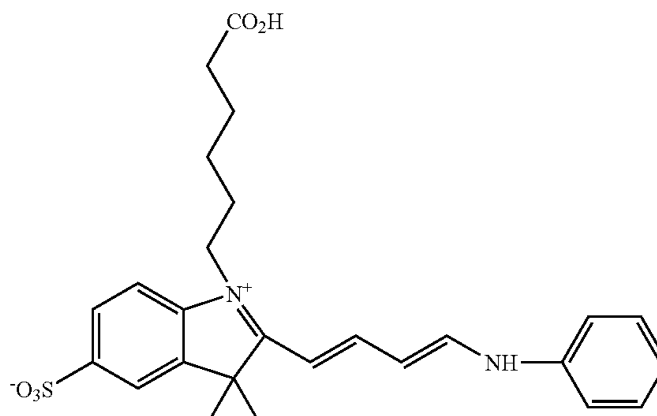
Compound 54
