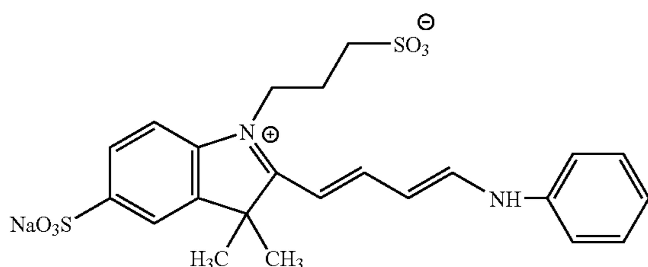
Compound 4
