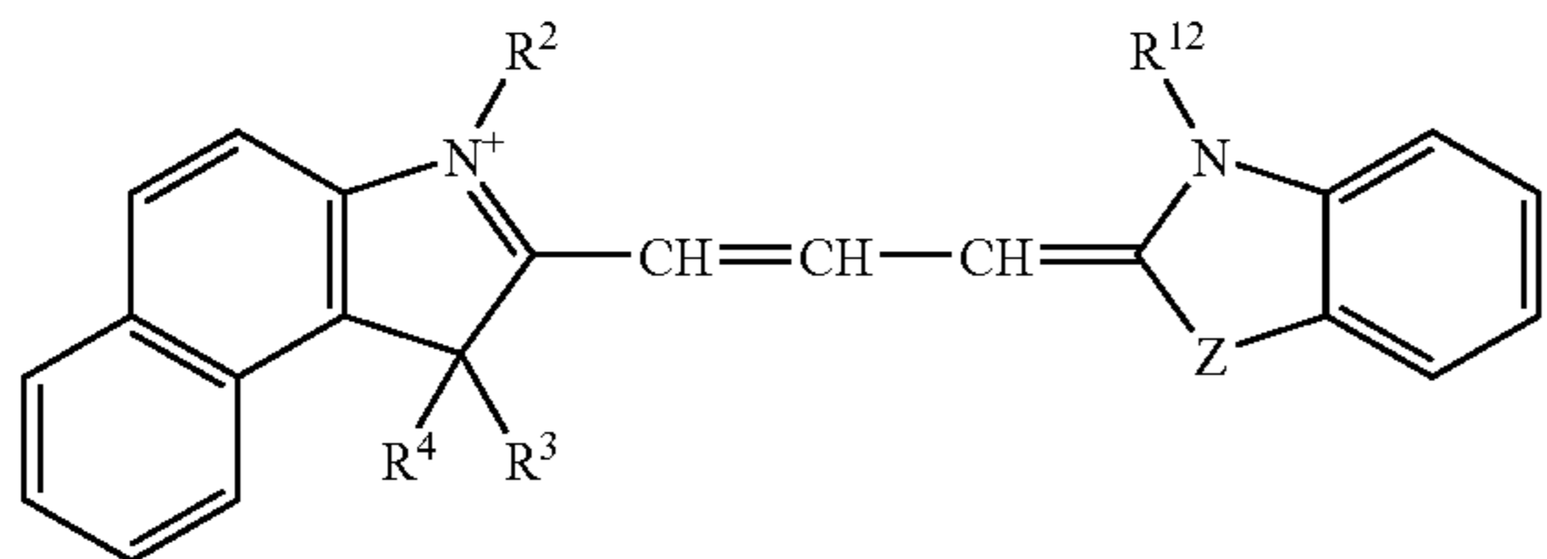
Formula XIII
