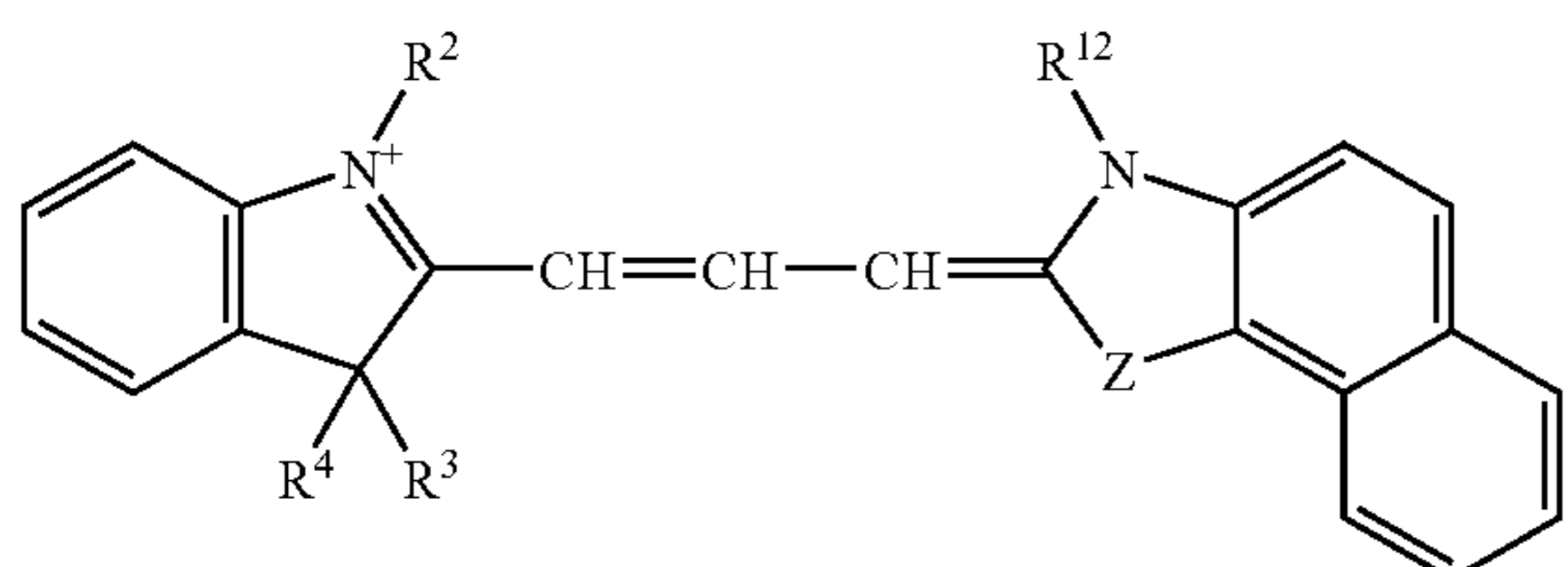
Formula XIV
