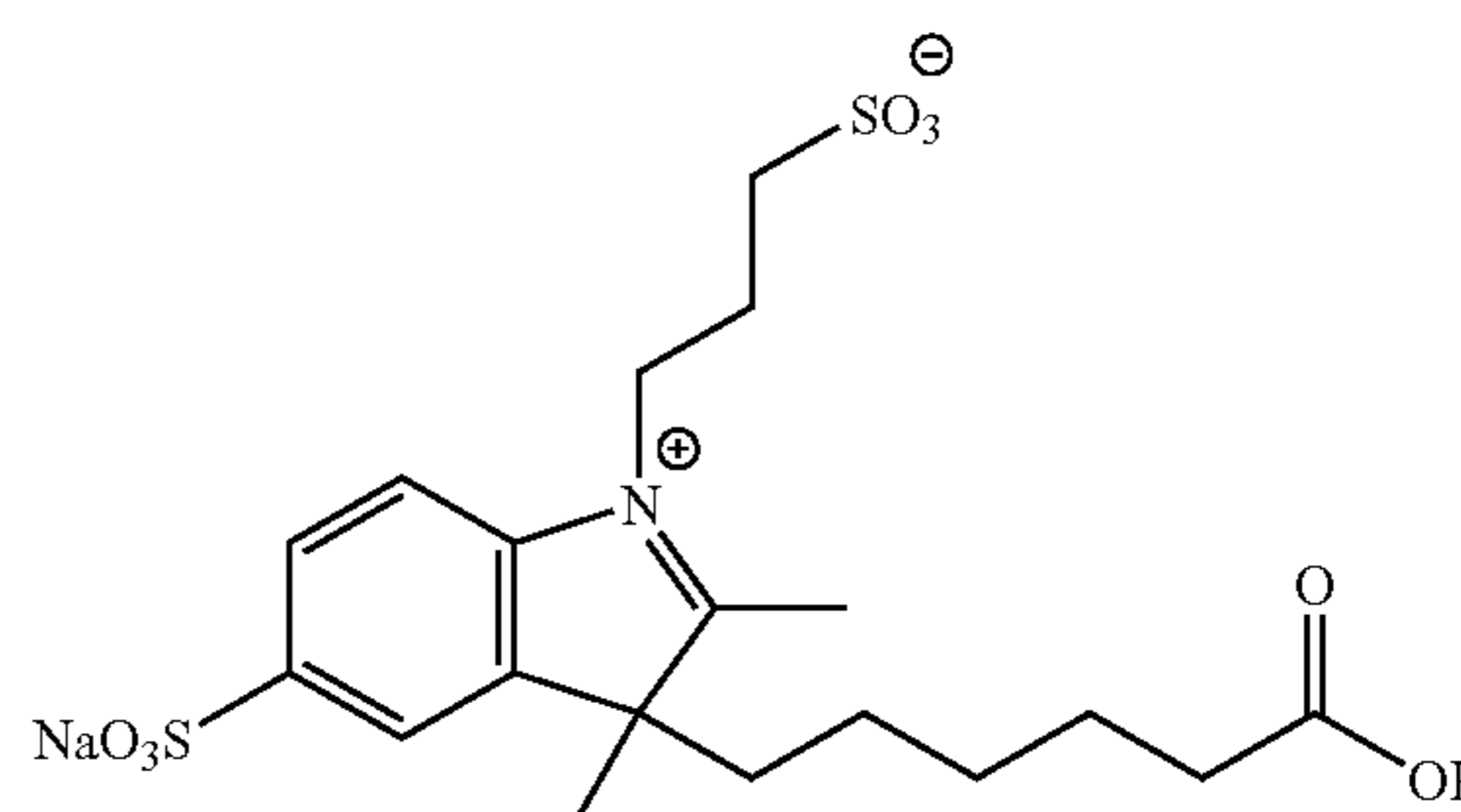
Compound 2
