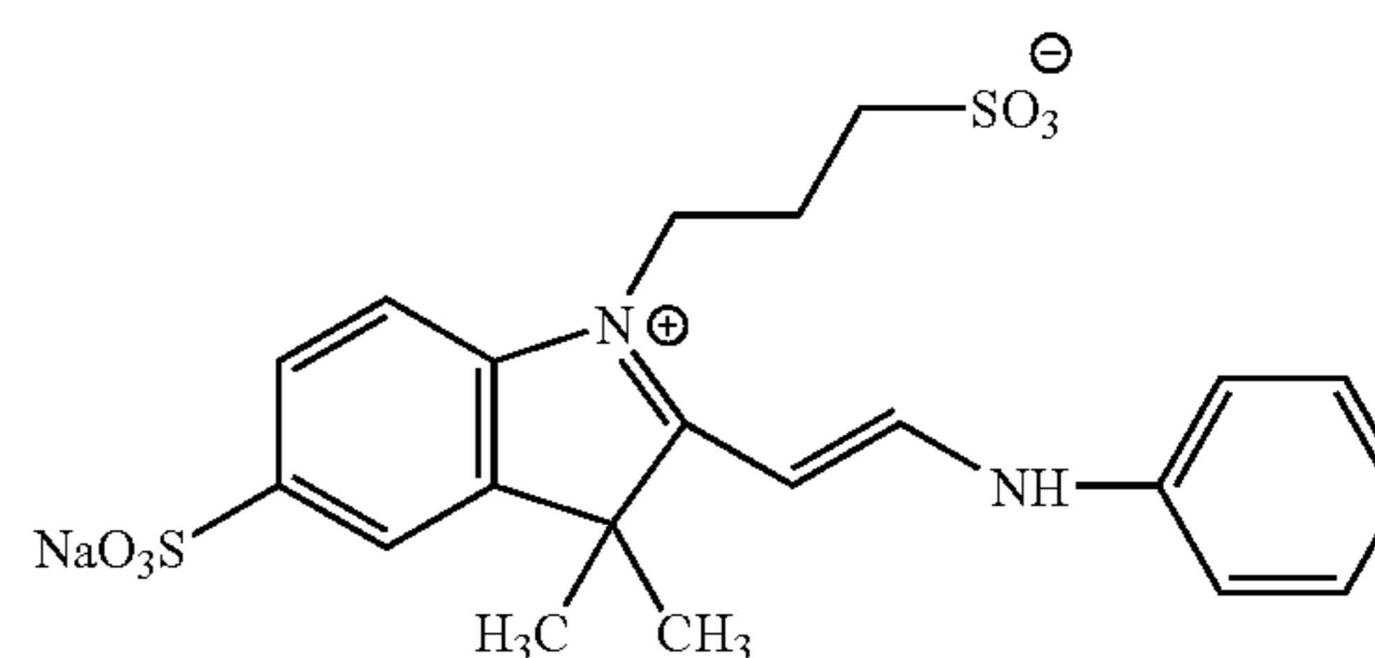
Compound 5
