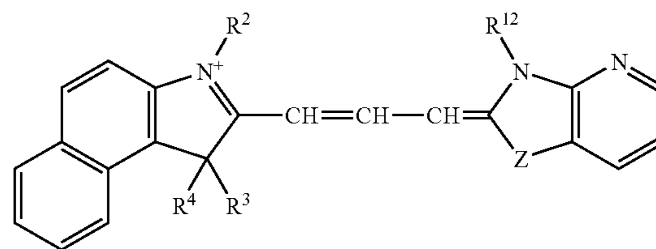
Formula XXIII
