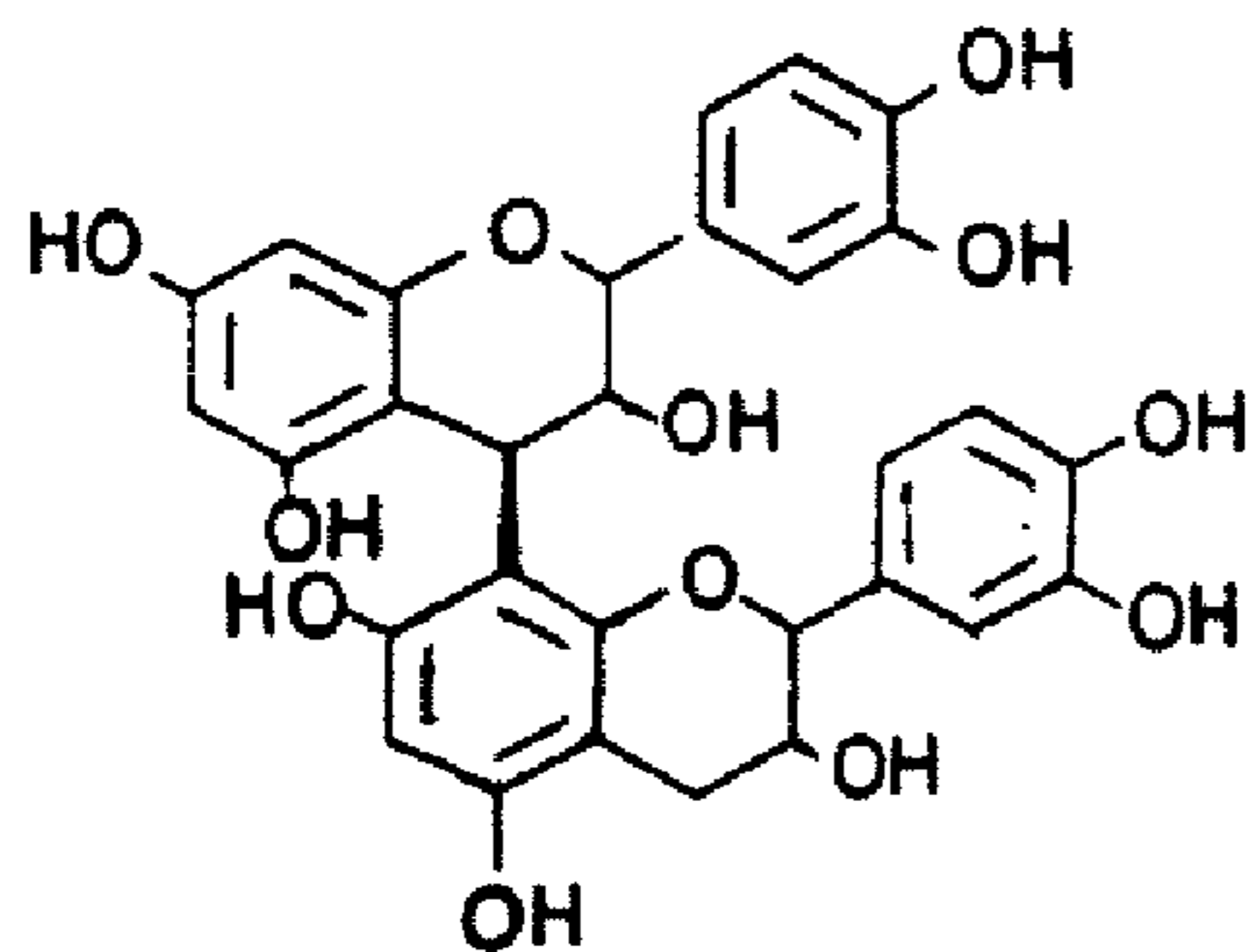
PROCYANIDIN B-2
