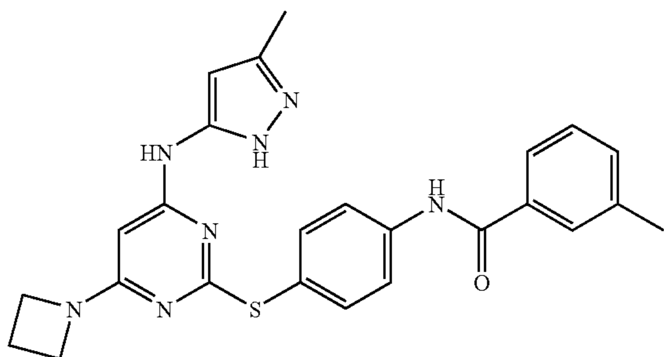
N-(4-(4-(3-methyl-1H-pyrazol-5-ylamino)-6-(azetidin-1-yl)pyrimidin-2-ylthio)phenyl)-3-methylbenzamide (I-4)
