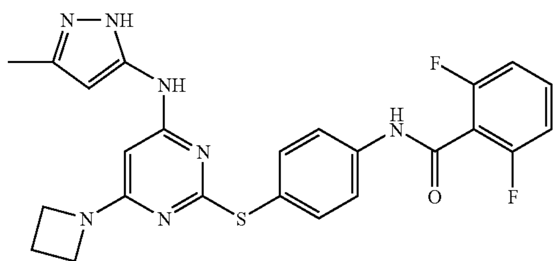
N-{4-[4-Azetidin-1-yl-6-(5-methyl-2H-pyrazol-3-ylamino)-pyrimidin-2-ylsulfanyl]-phenyl}-2,6-Difluoro-benzamide
