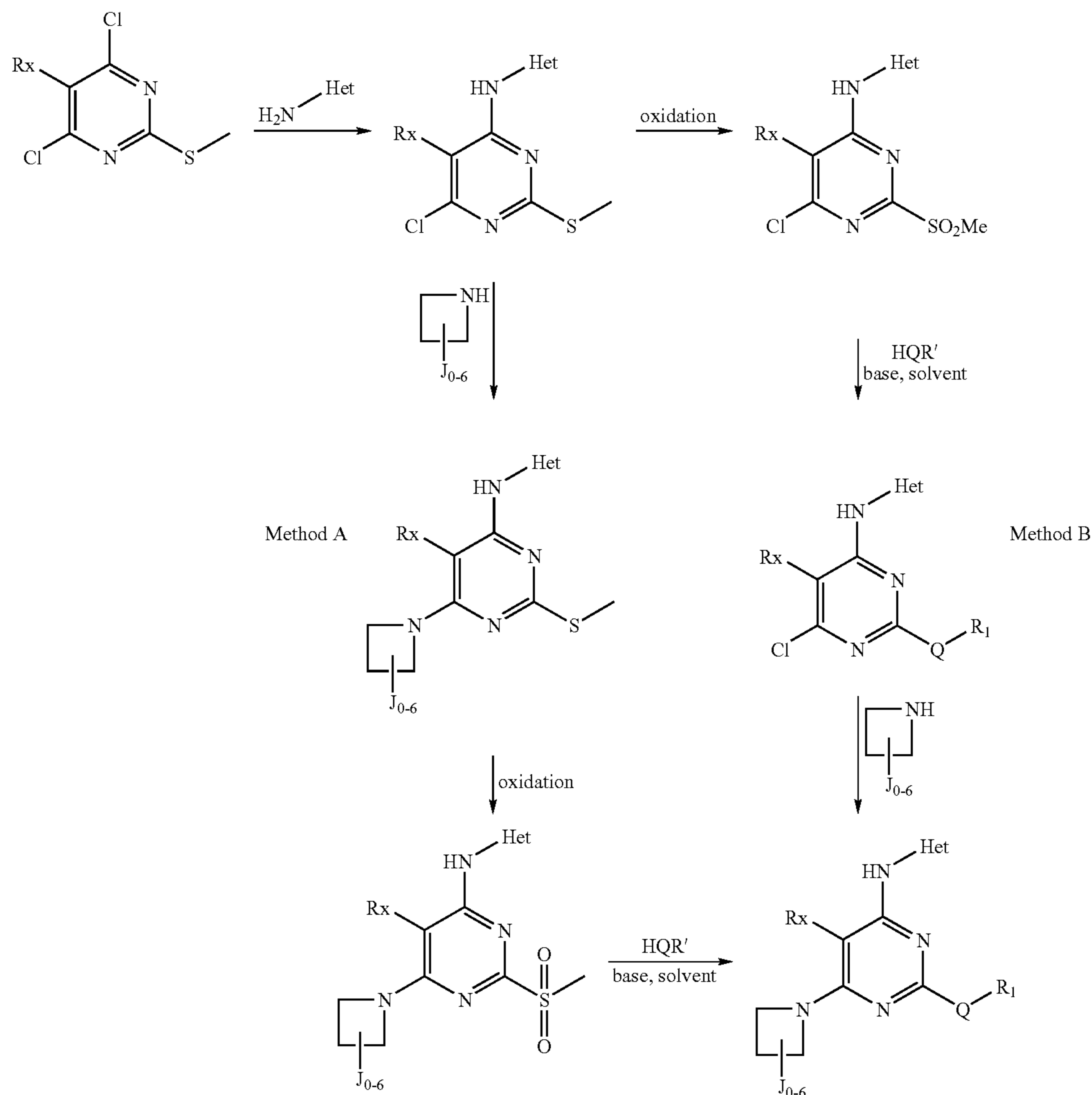
General Scheme
