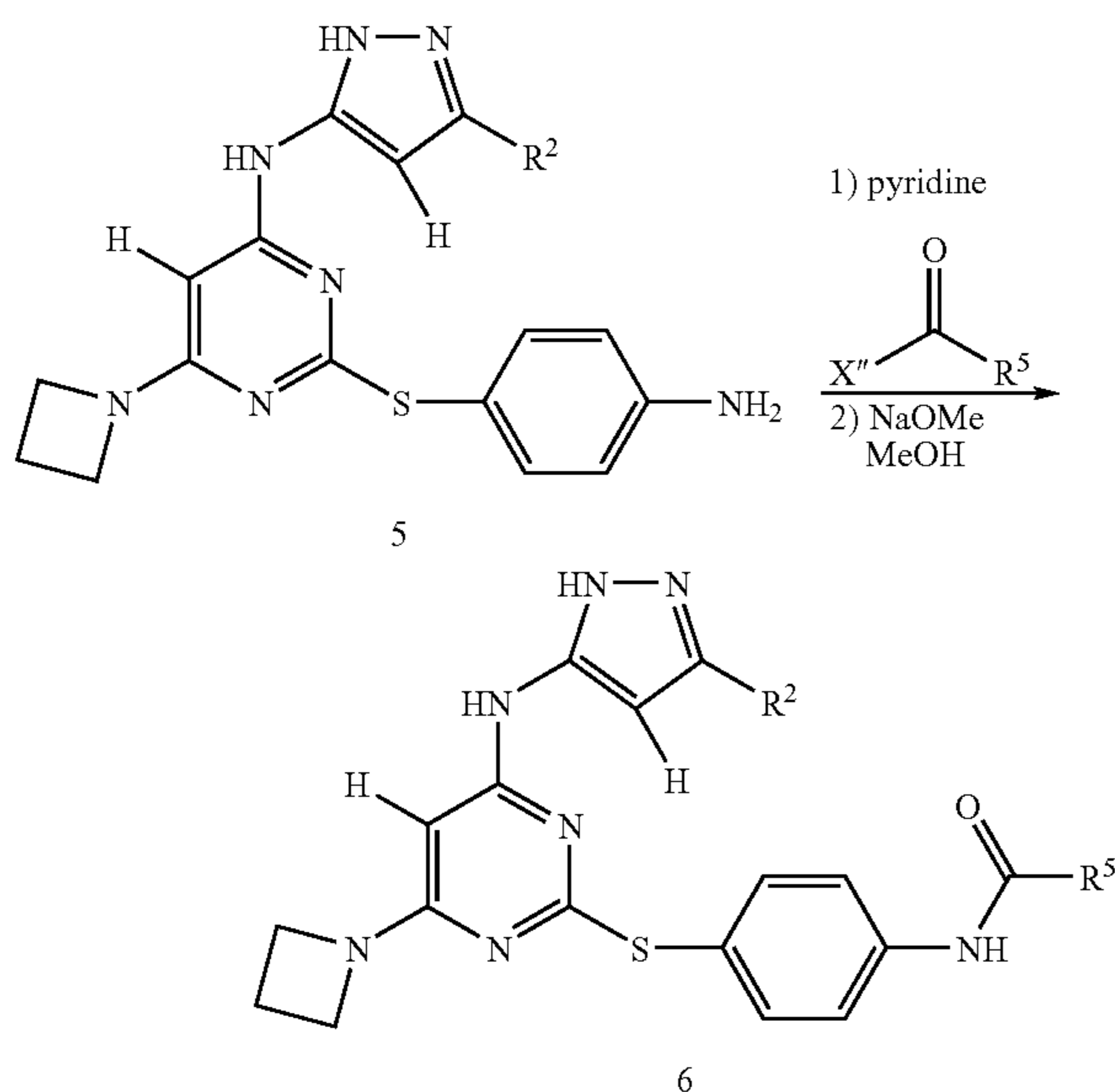
Scheme II
