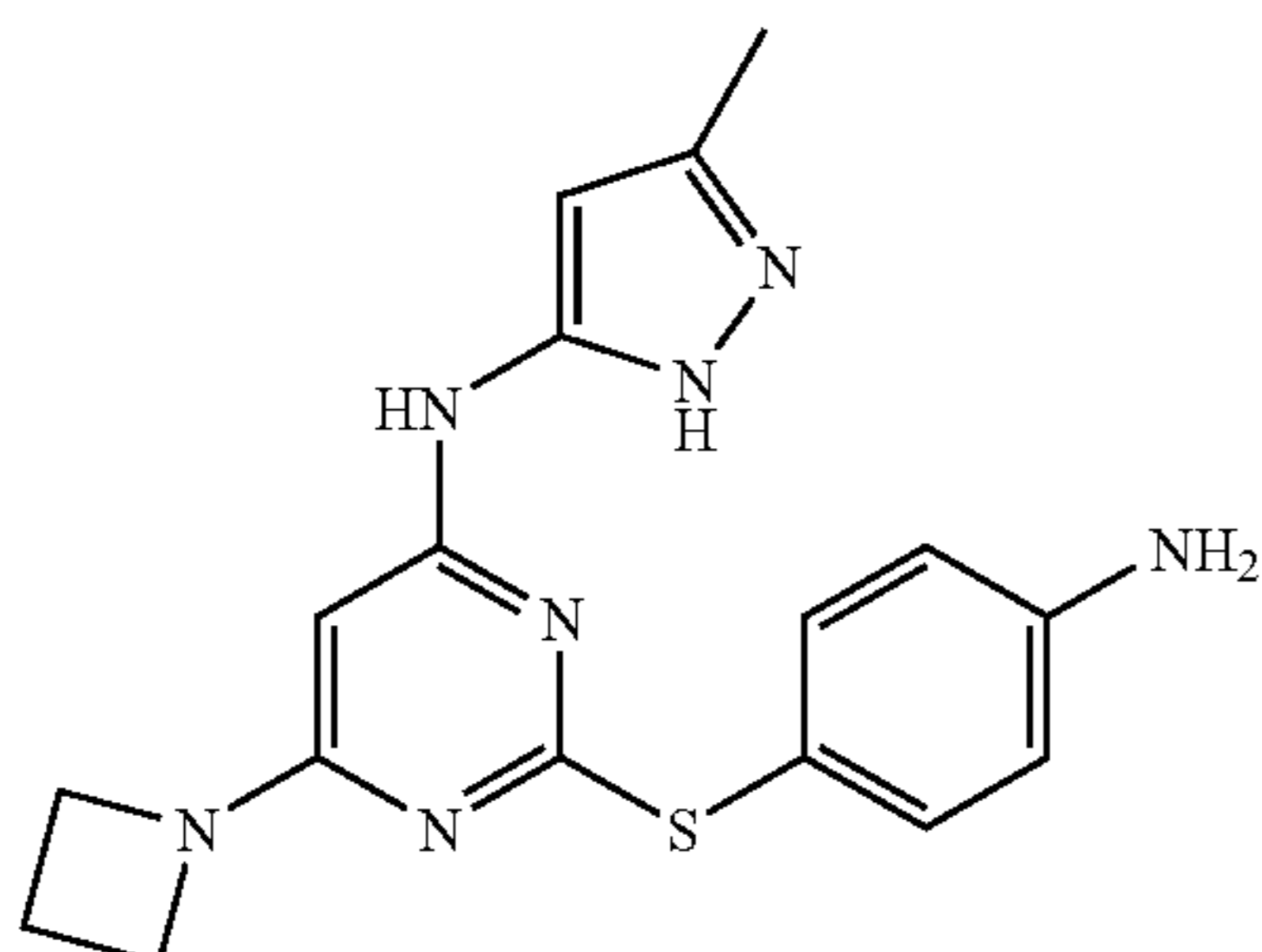
2-(4-aminophenylthio)-6-(azetidin-1-yl)-N-(3-methyl-1H-pyrazol-5-yl)pyrimidin-4-amine
