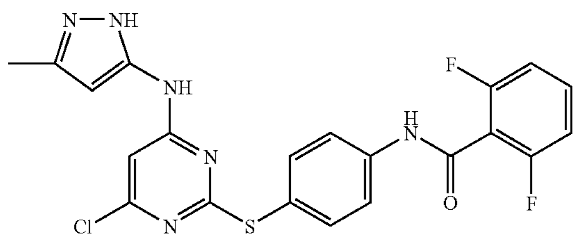
2,6-Difluoro-N-{4-[4-chloro-6-(5-methyl-2H-pyrazol-3-ylamino)-pyrimidin-2-ylsulfanyl]-phenyl}-benzamide
