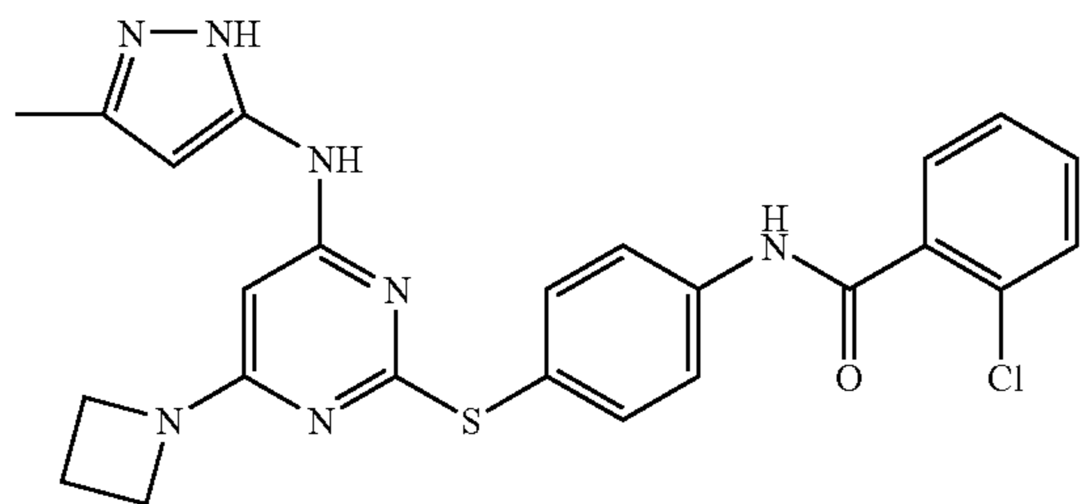
N-{4-[4-Azetidin-1-yl-6-(5-methyl-2H-pyrazol-3-ylamino)-pyrimidin-2-ylsulfanyl]-phenyl}-2-chloro-benzamide: (Compound I-1)
