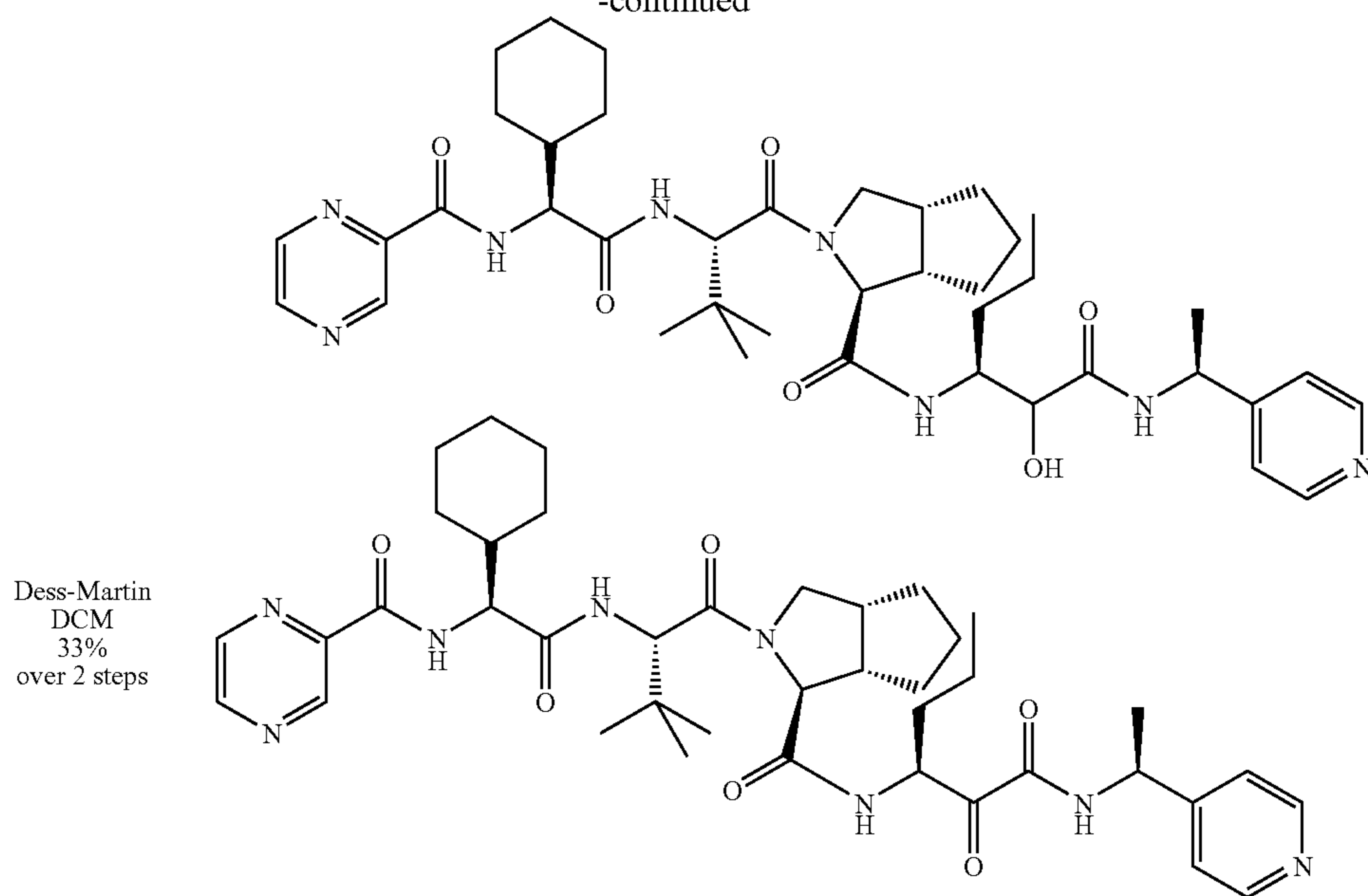
SCHEME 10
