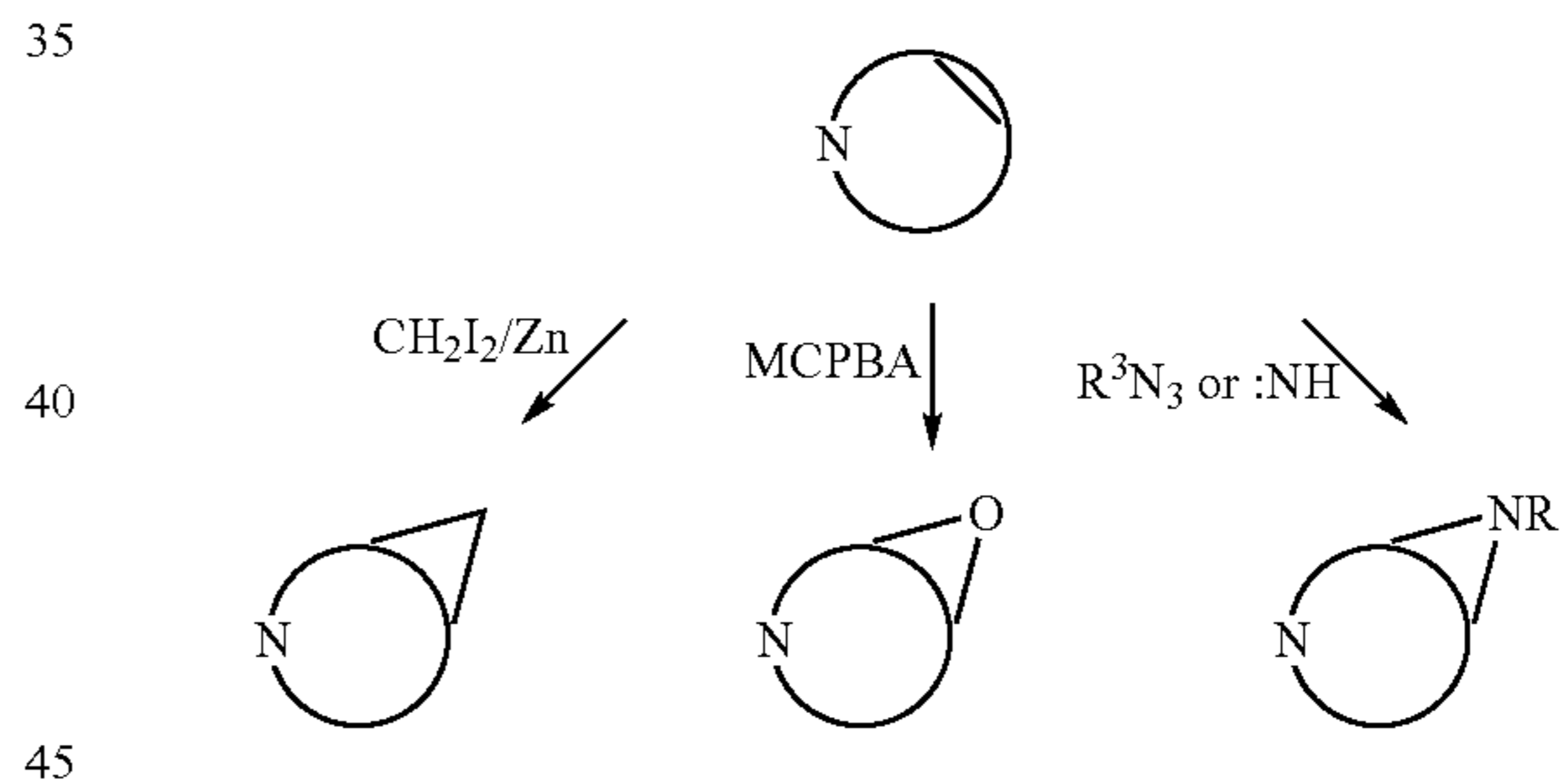
SCHEME 8
