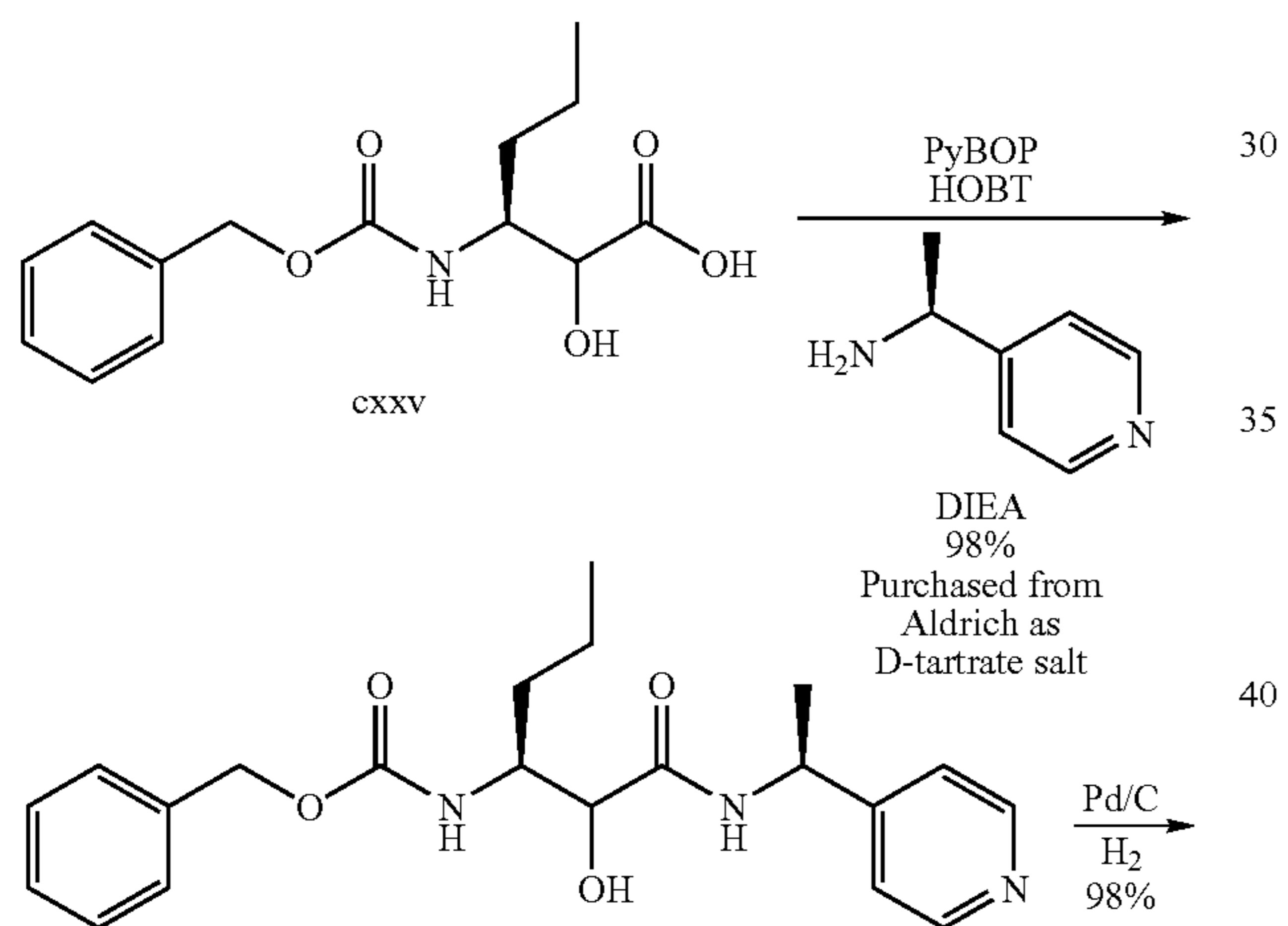
SCHEME 10
