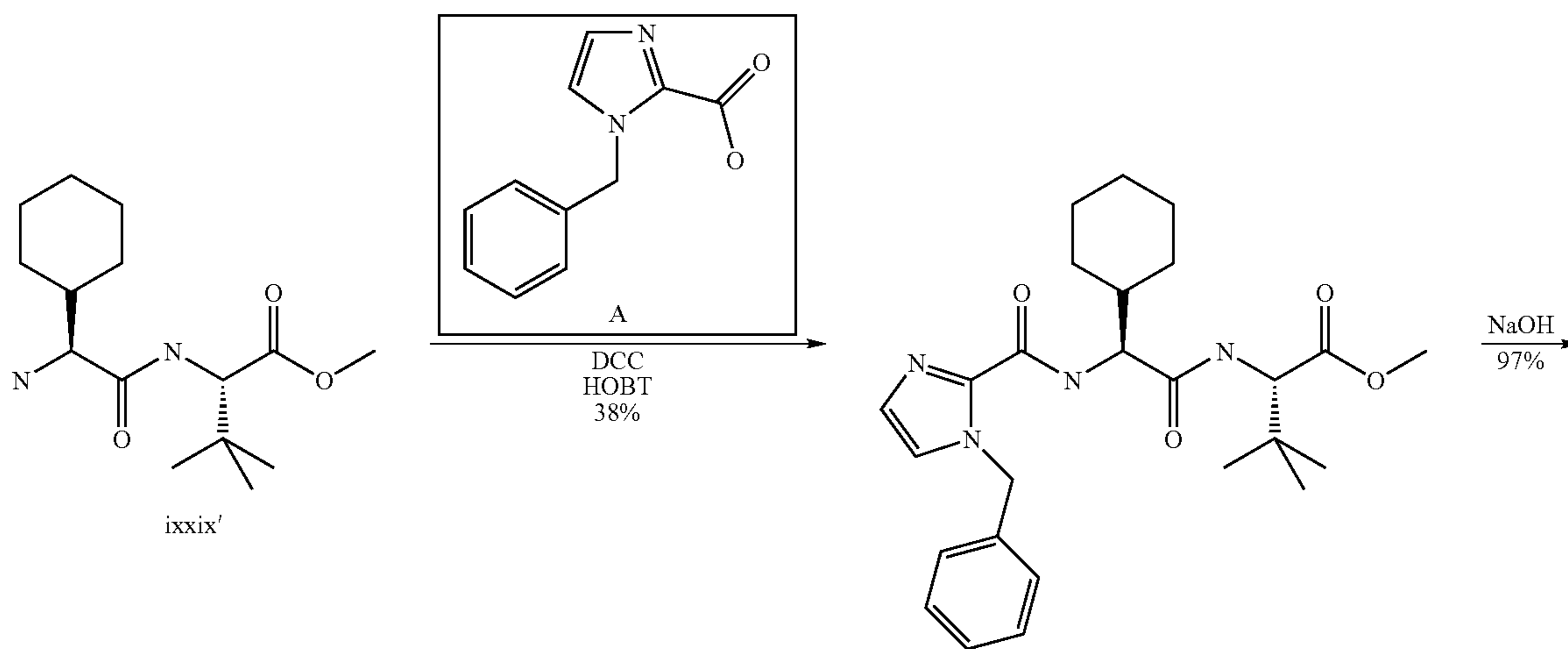
Scheme 11
