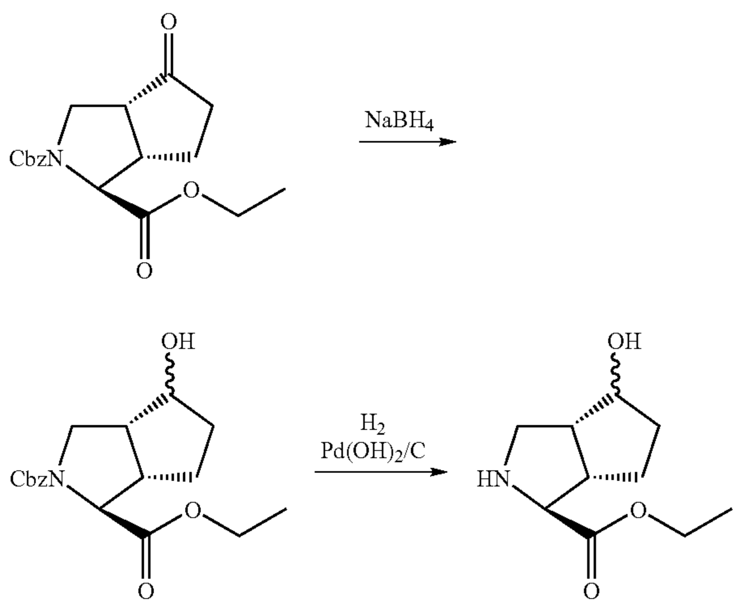
SCHEME 6
