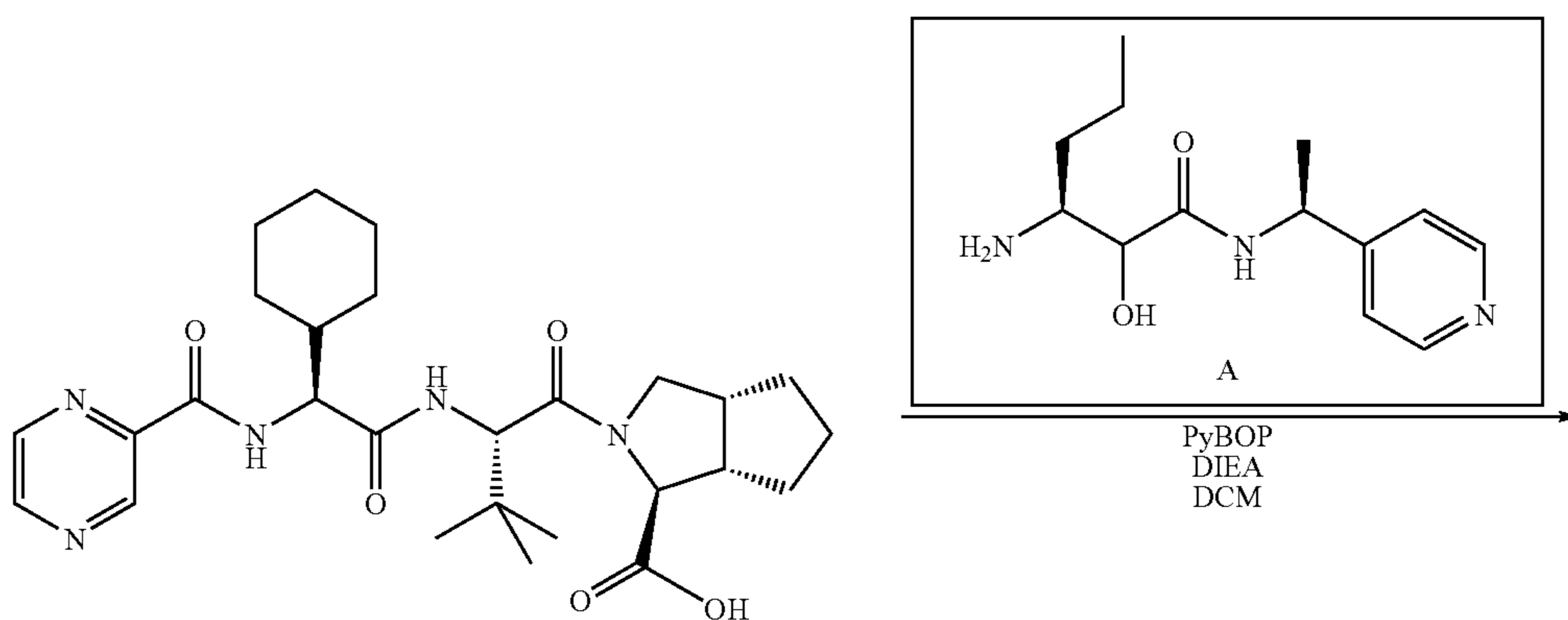
Scheme 9
