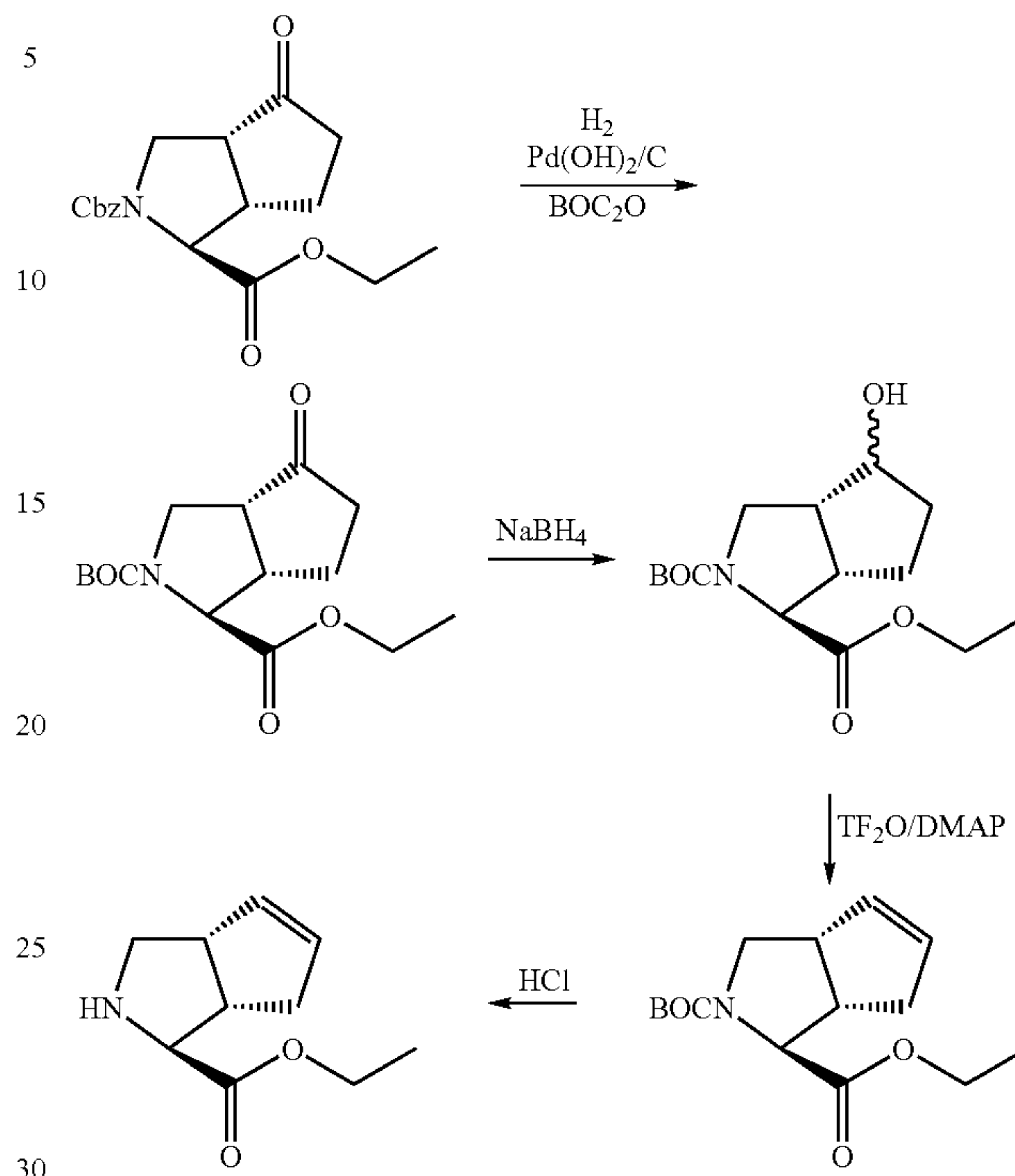
SCHEME 7
