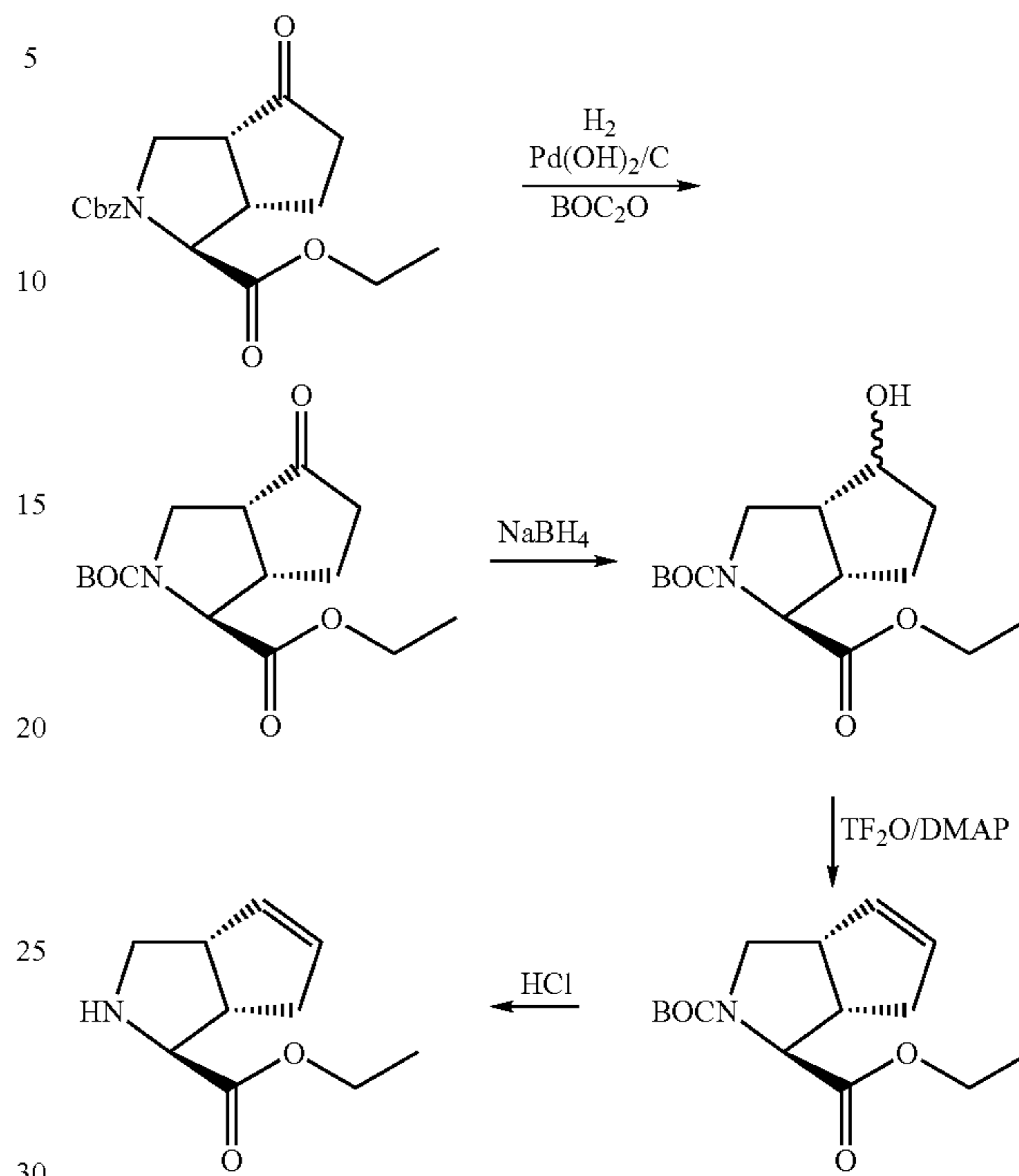
SCHEME 7
