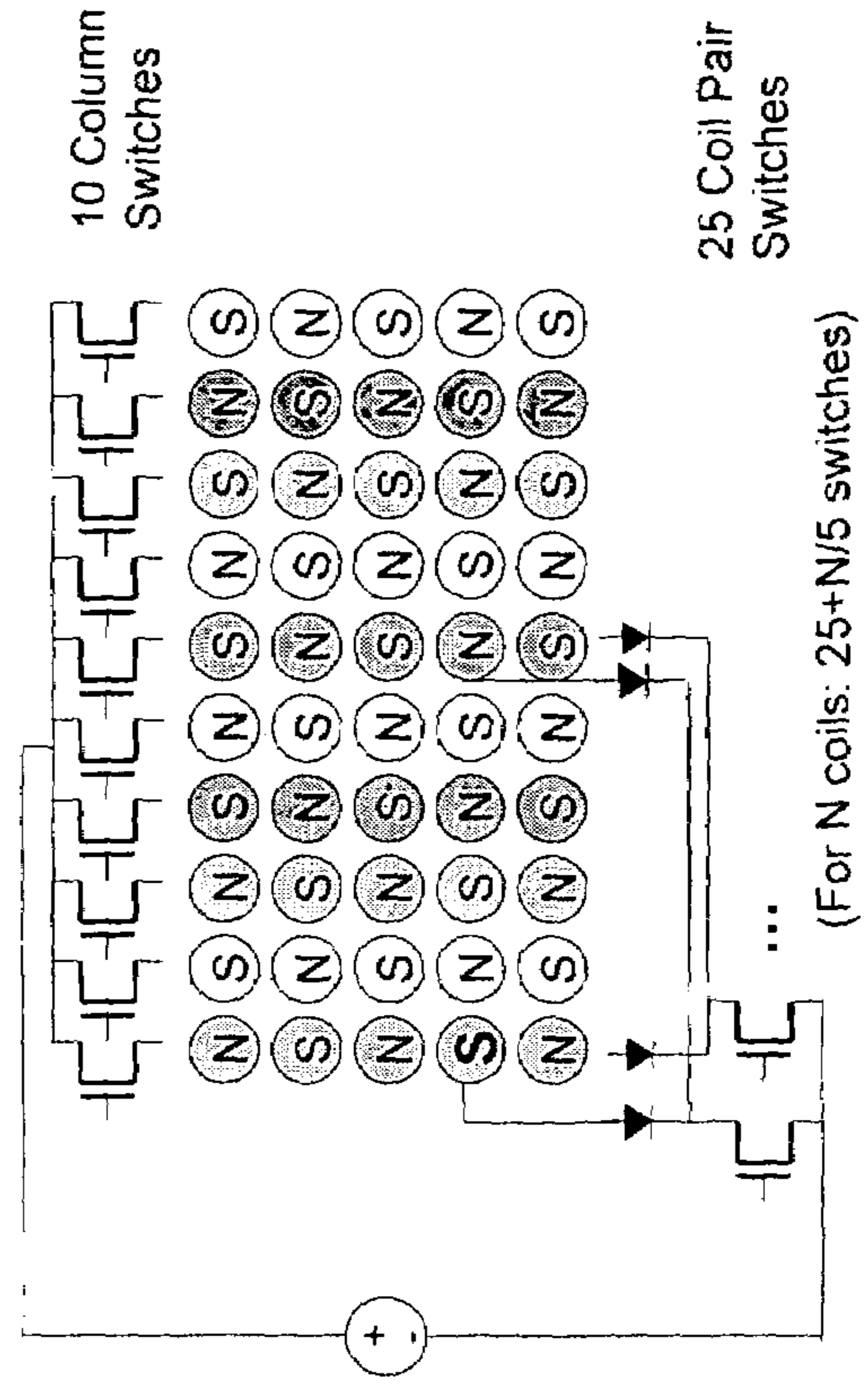
FIG. 9B) Circuit design to reduce # of switches
