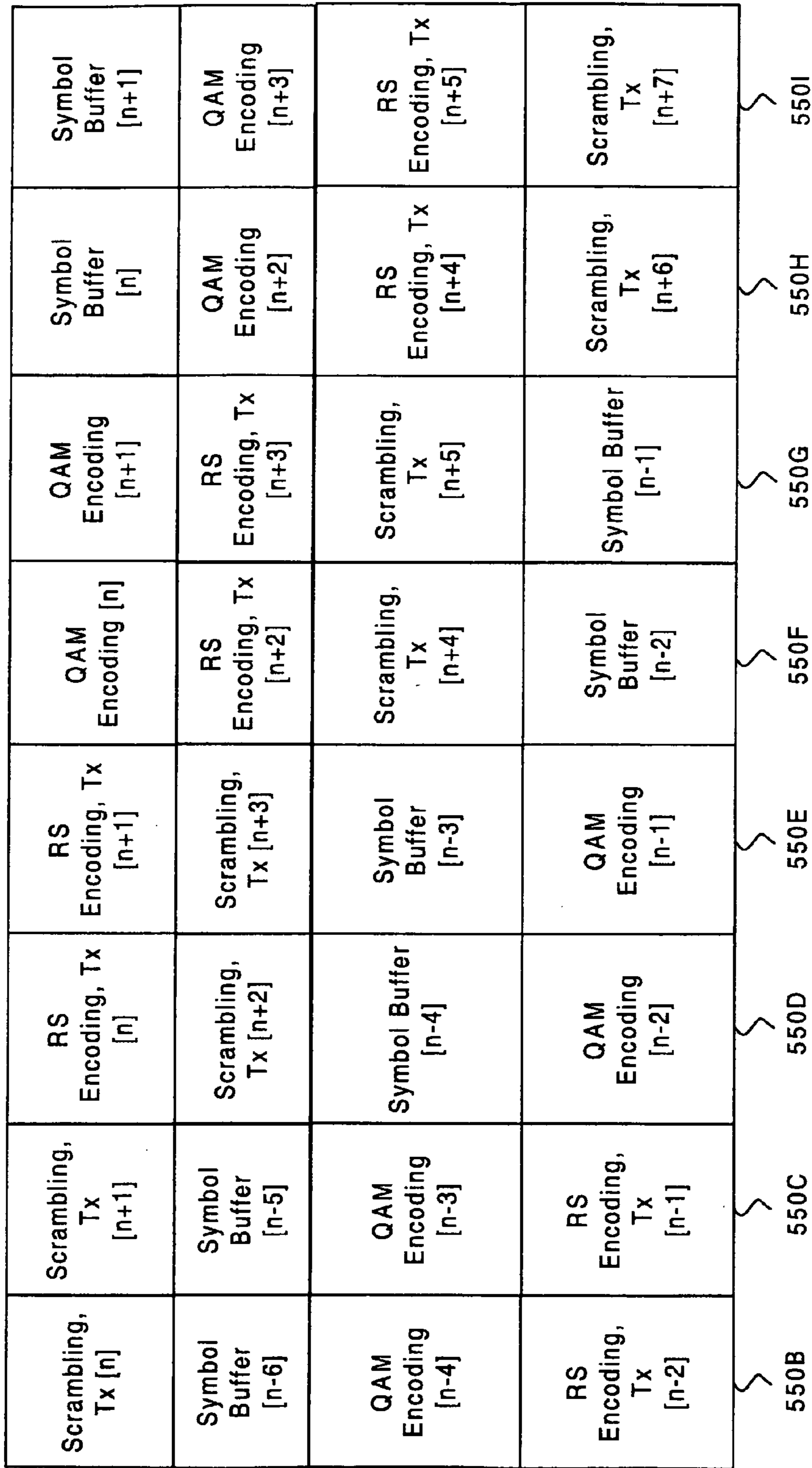
Fig. 5D Timing of symbol tasks and their sequences on hardware side
