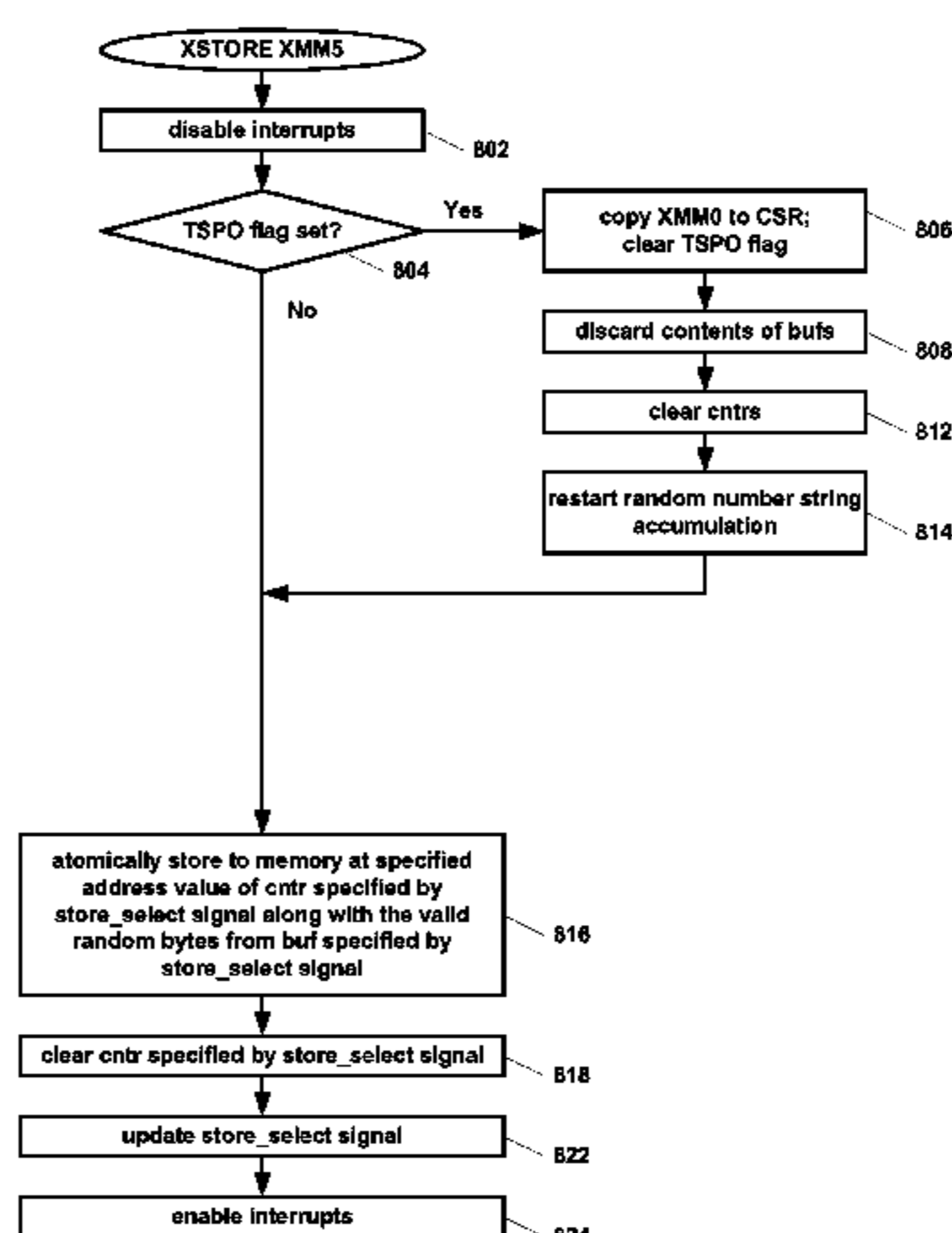
RNG Unit Operation (XSTORE XMM5 instruction)
