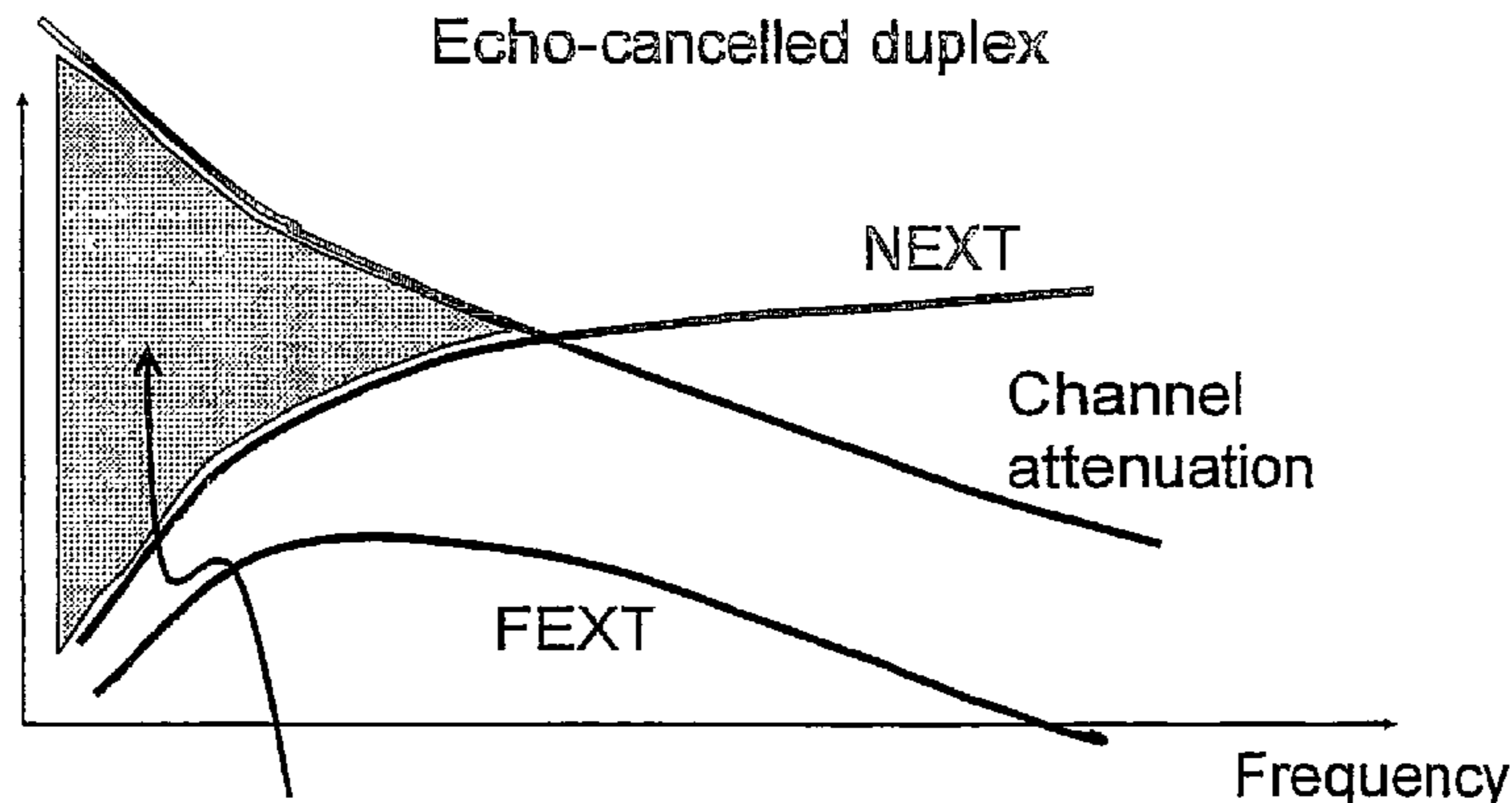
Available SNR in both downstream and upstream direction - full time
