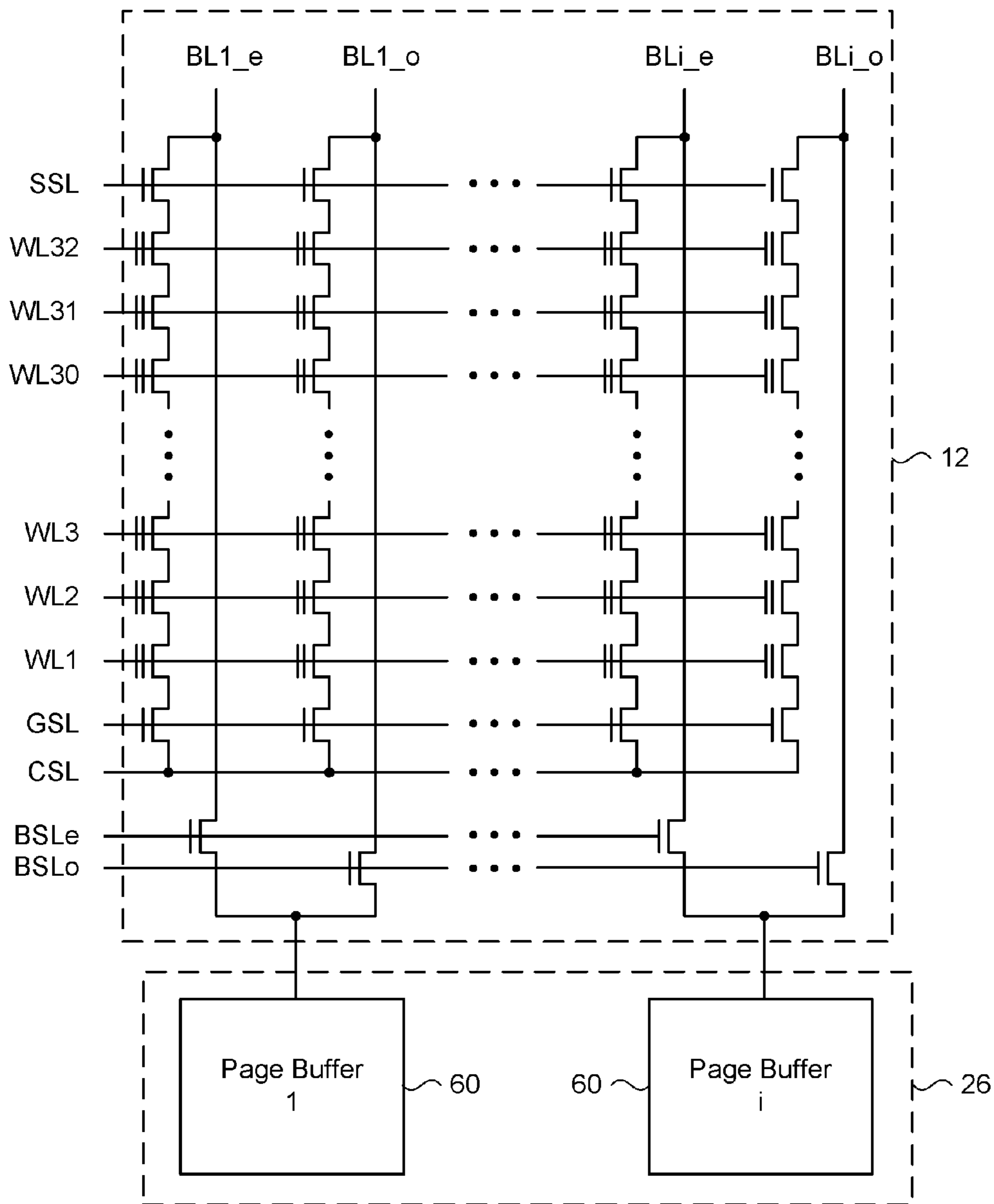
Figure 2 (Prior Art)
