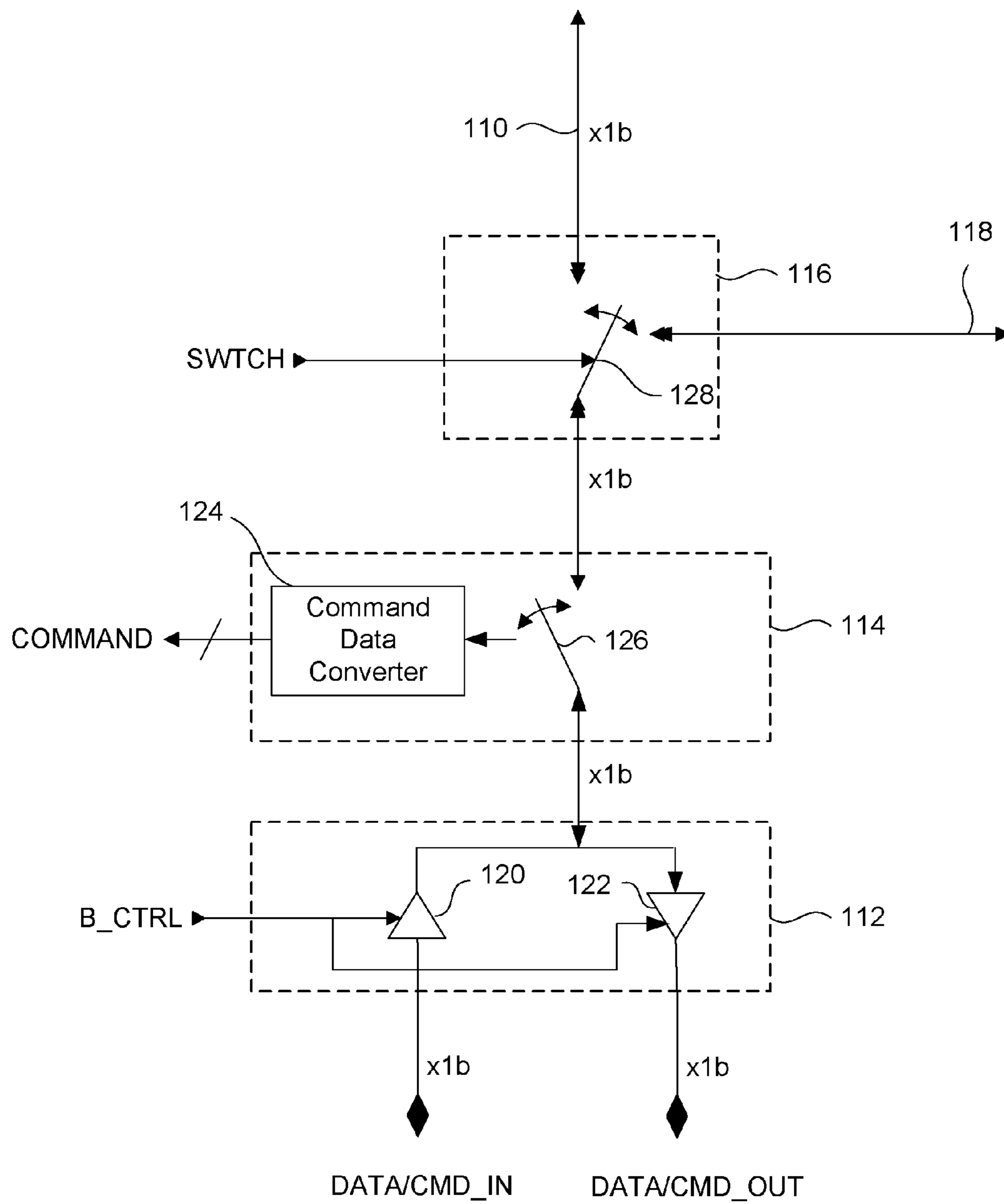
Figure 4B
