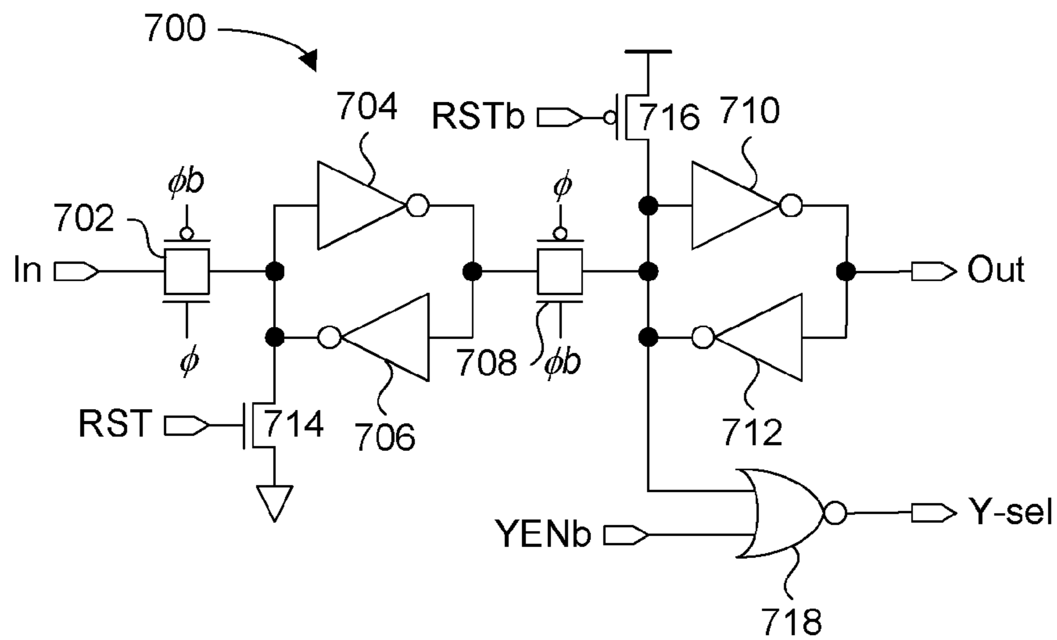
Figure 12
