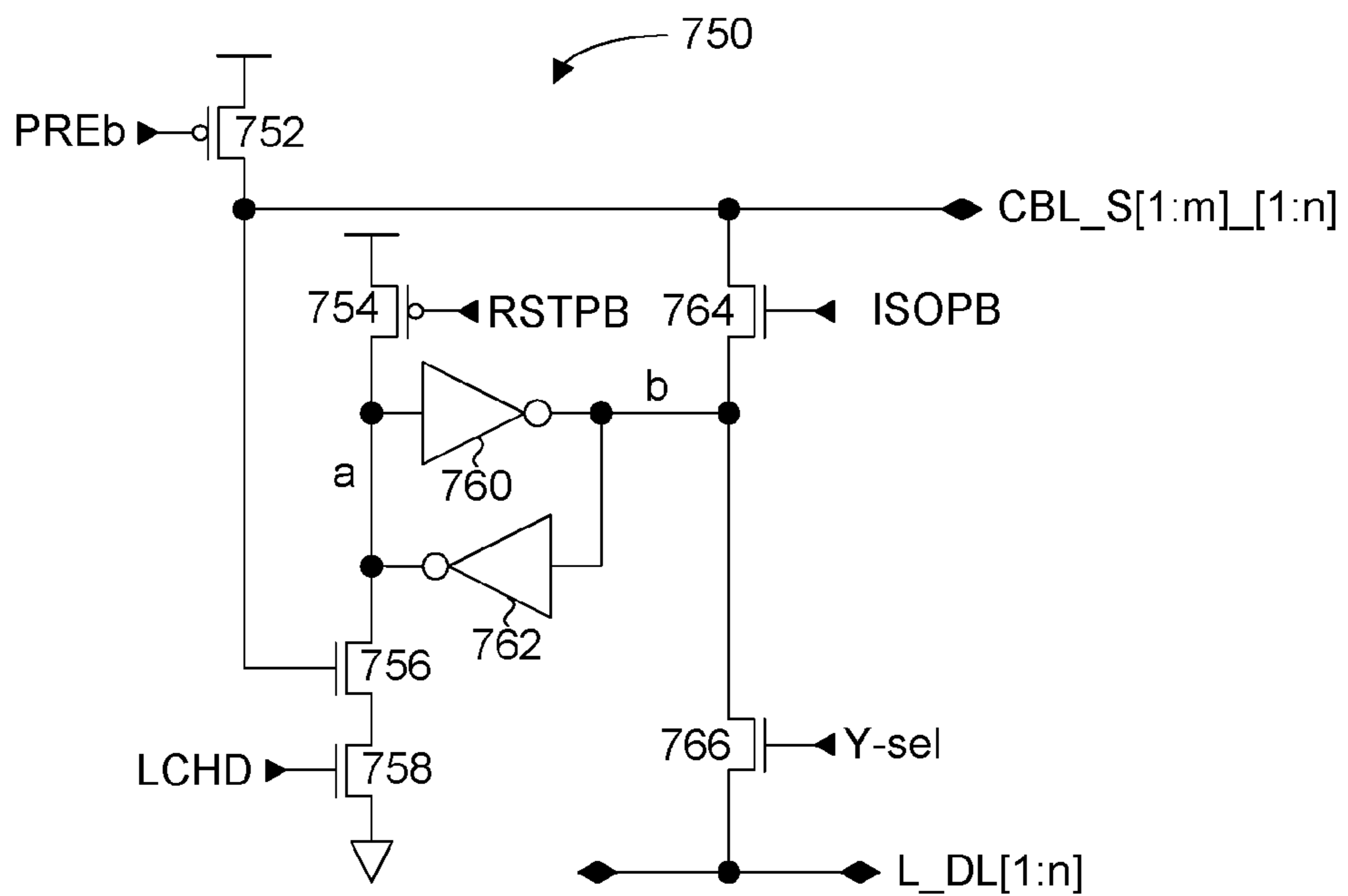
Figure 13
