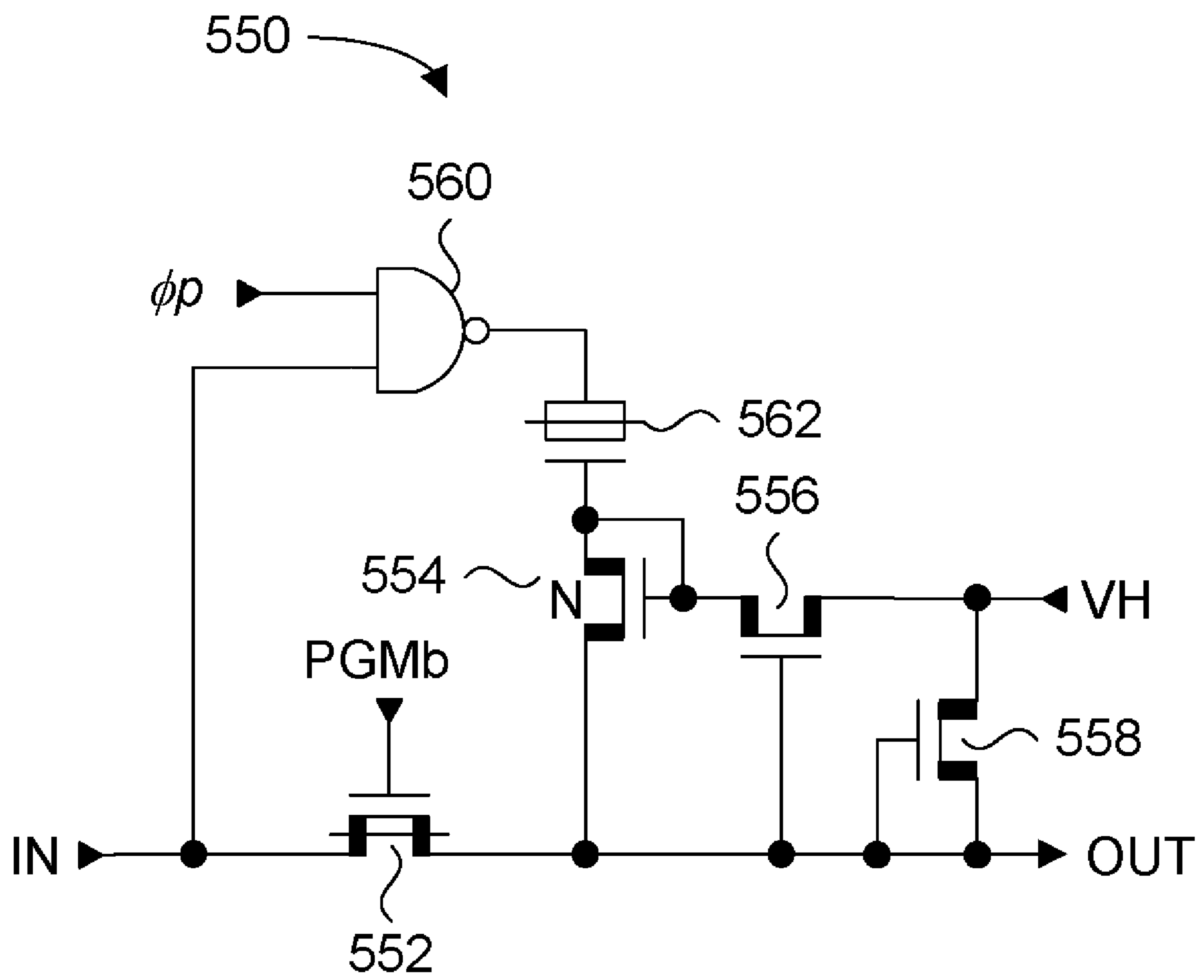
Figure 9
