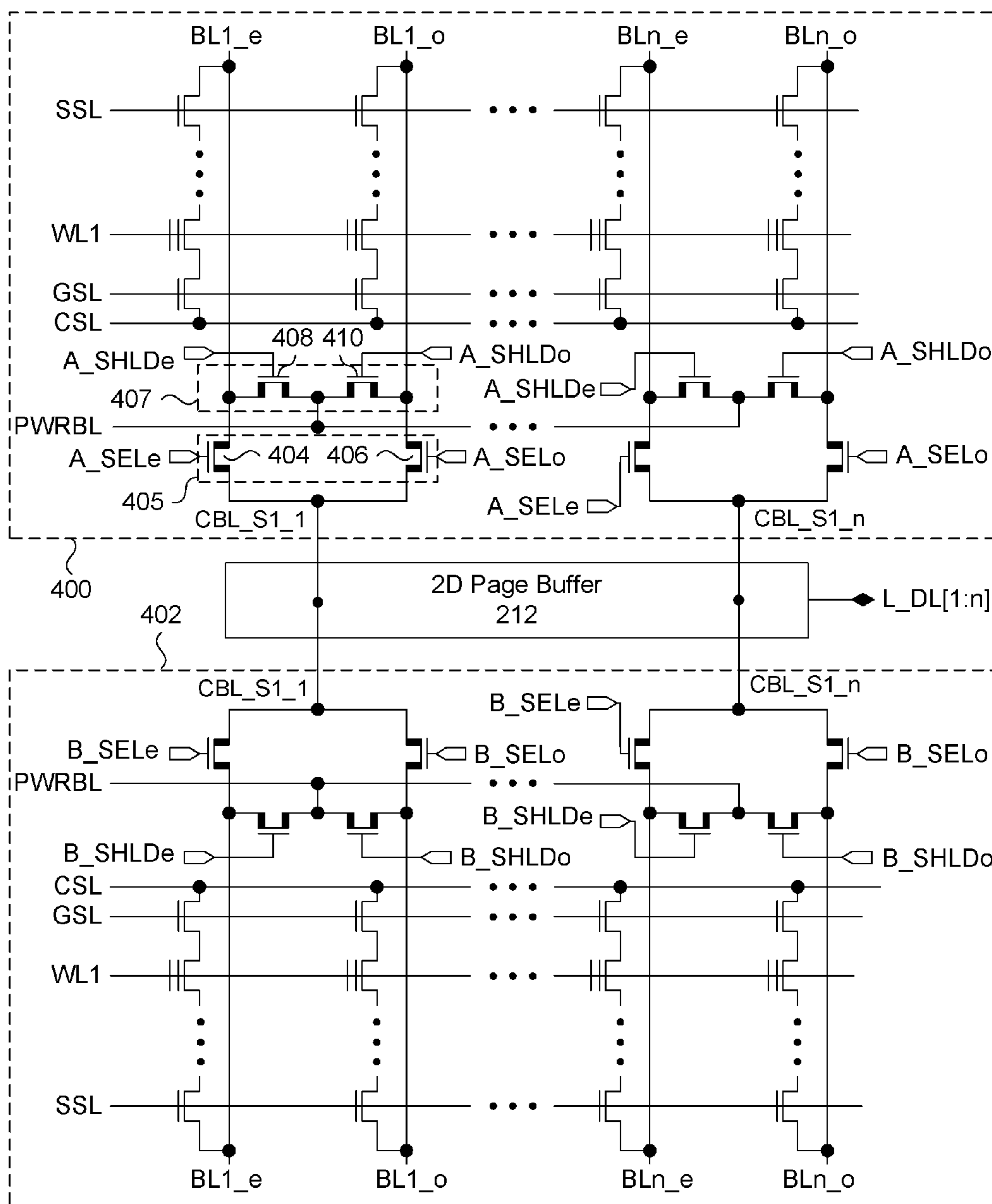
Figure 7B
