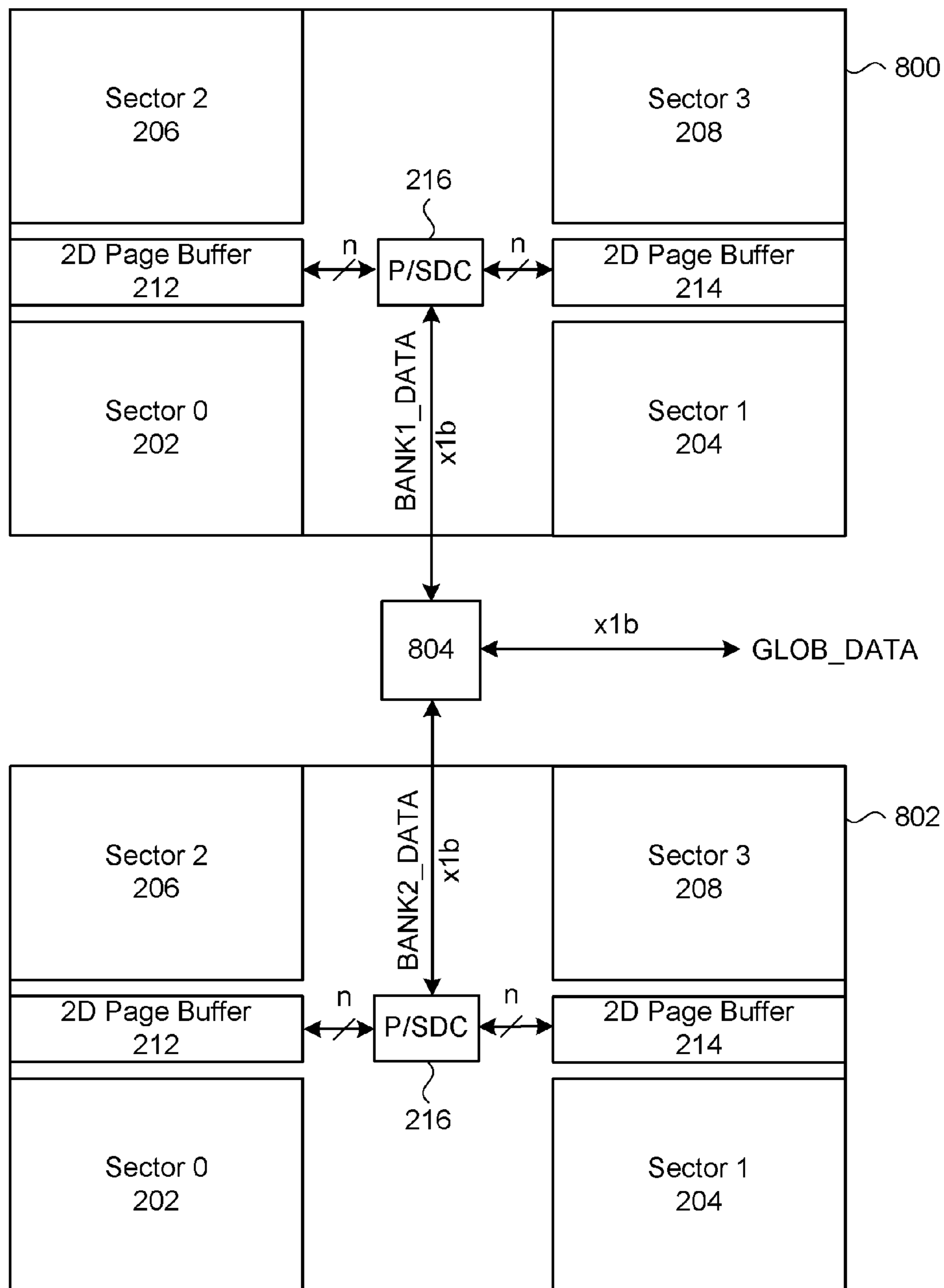
Figure 15
