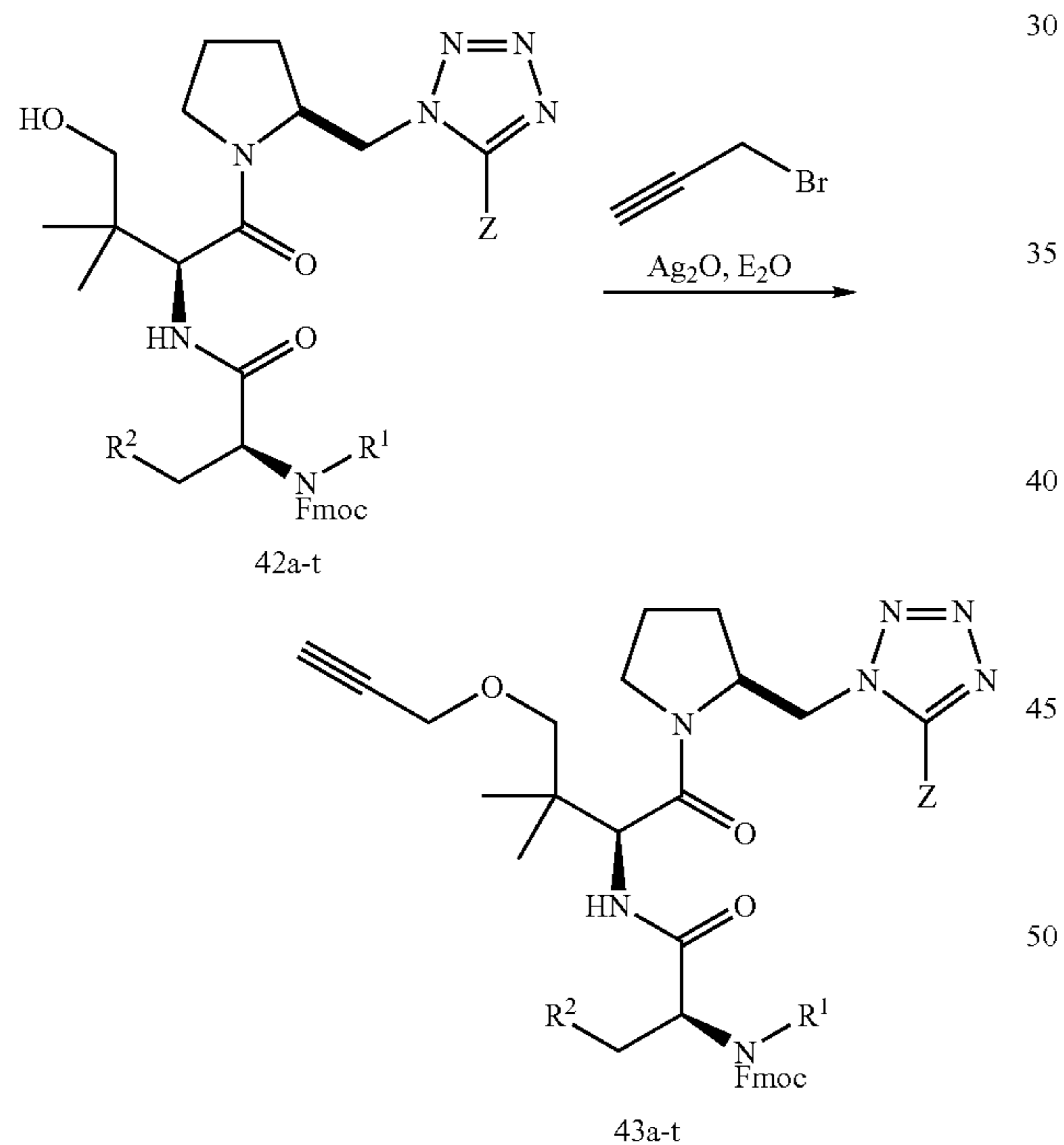
Scheme 15
