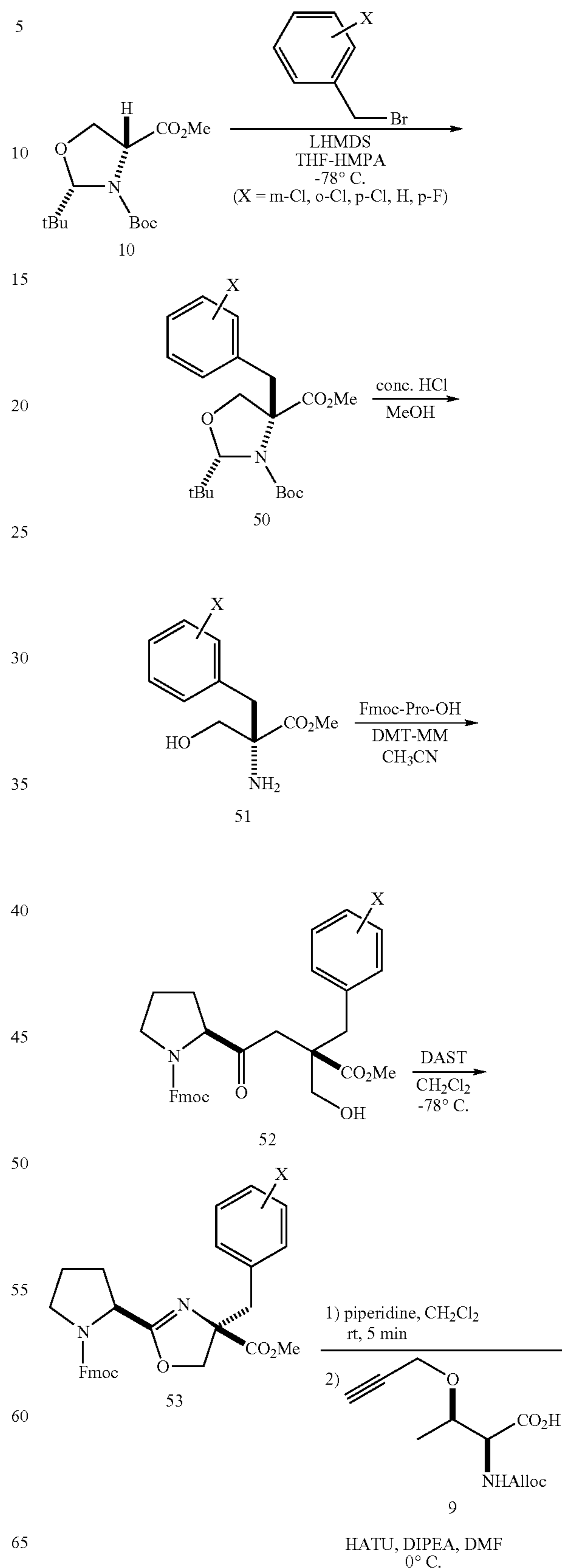
Scheme 10
