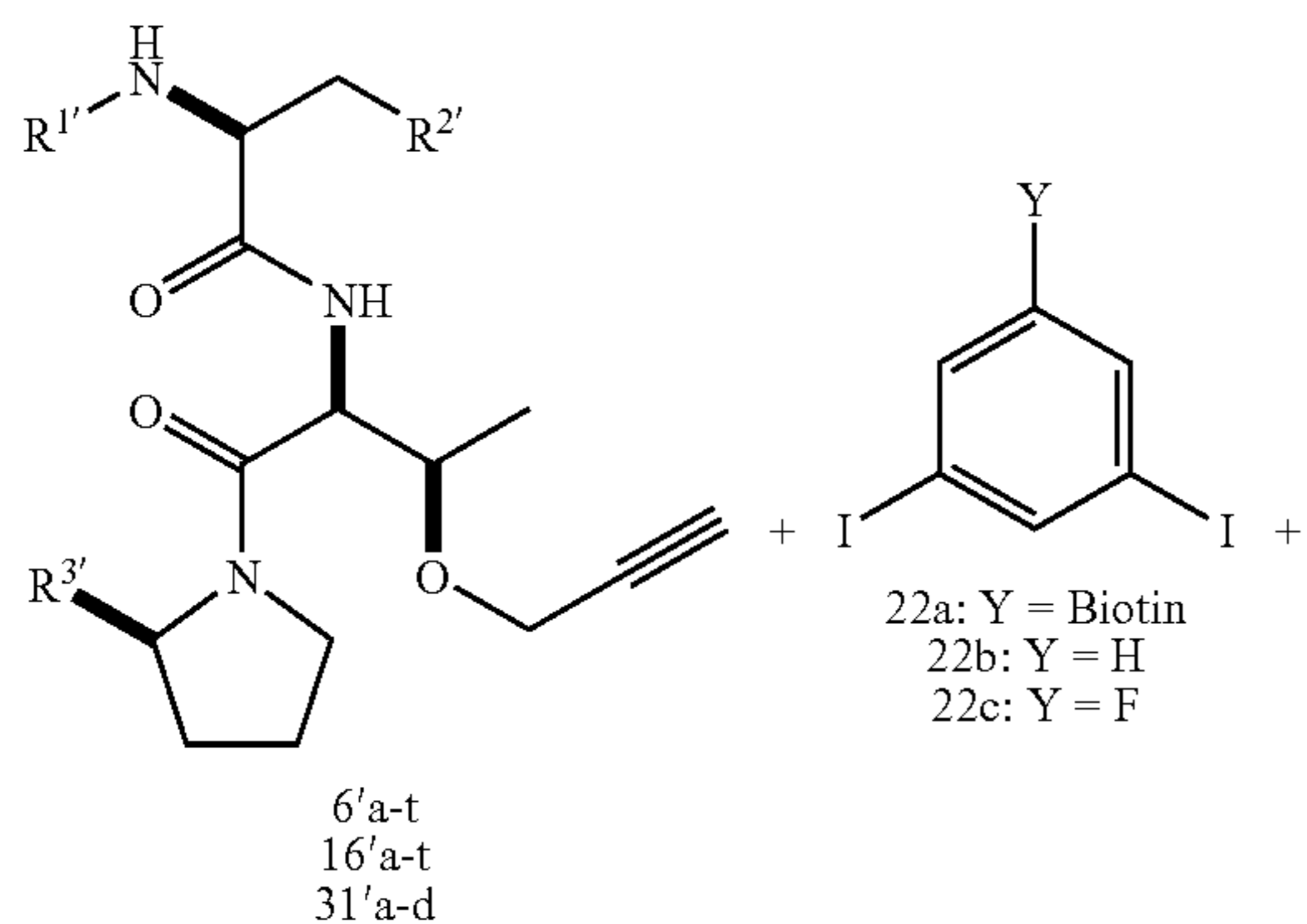
Scheme 13
