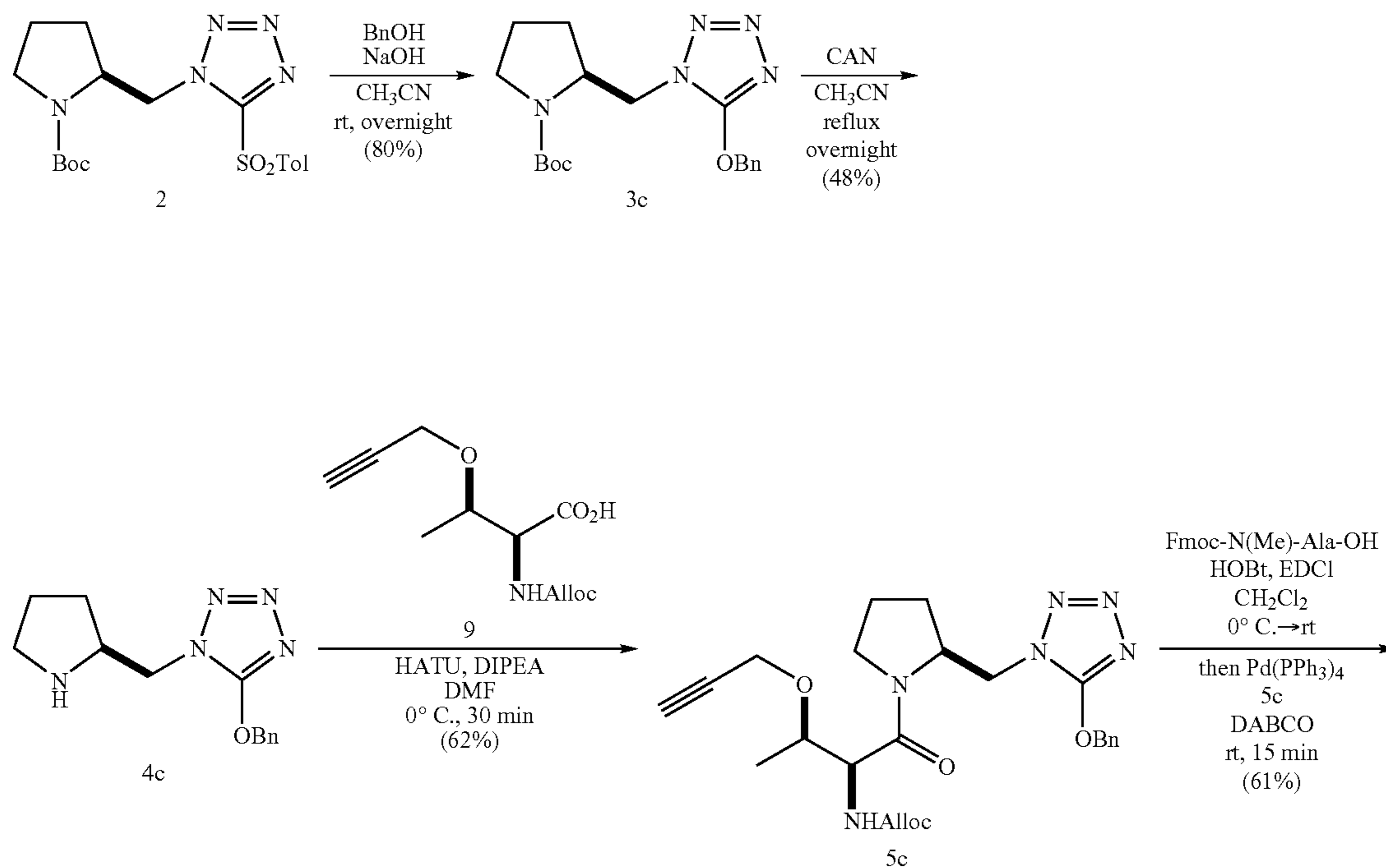
Scheme 3
