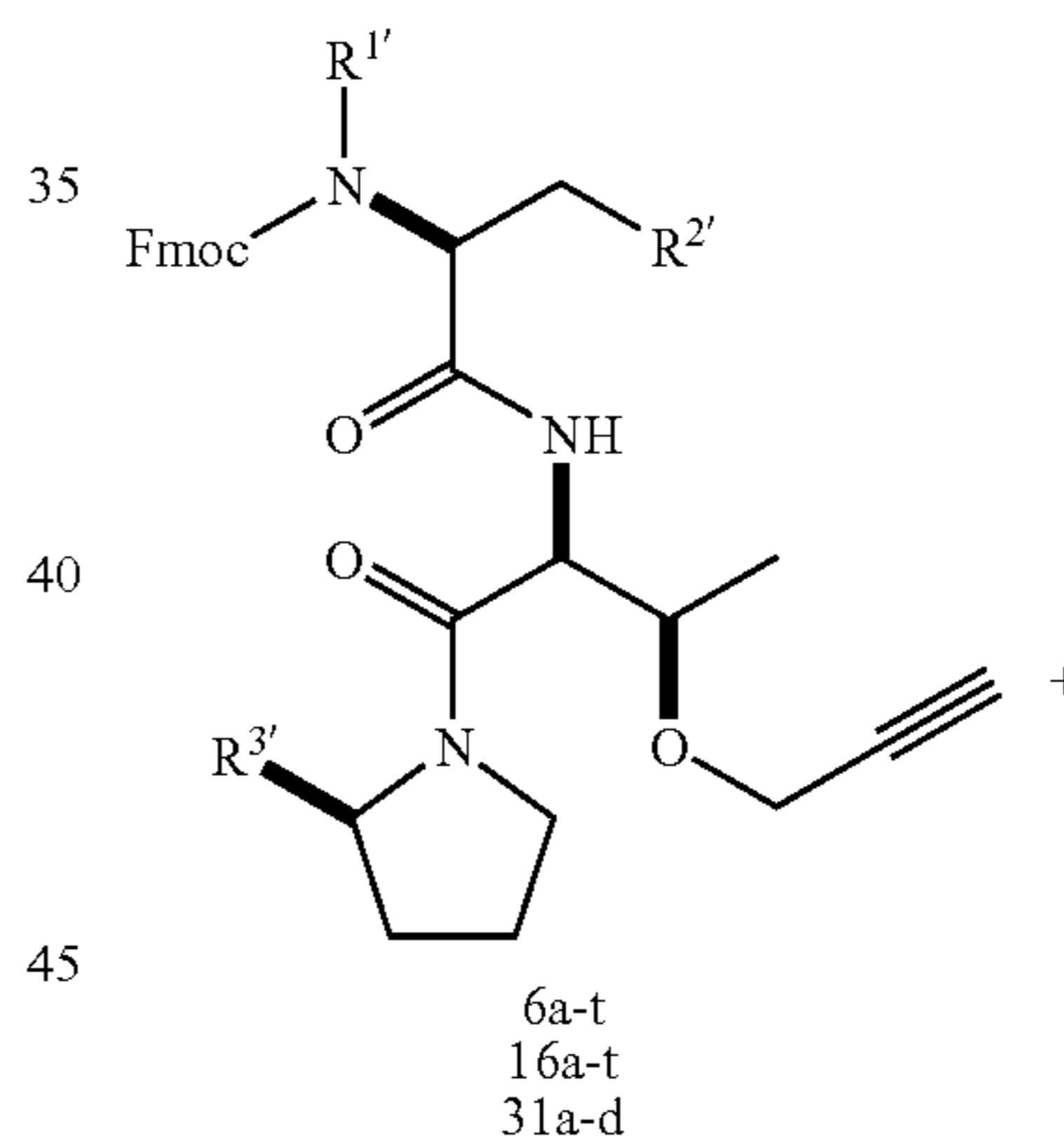
Scheme 12
