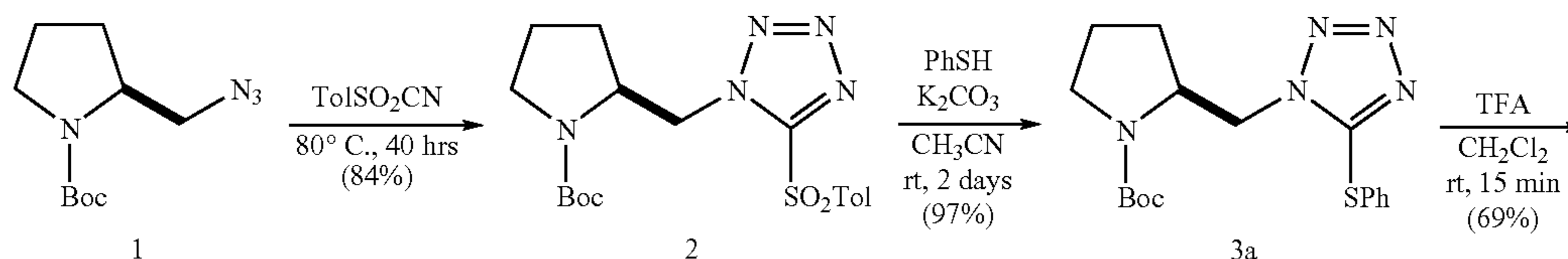
Scheme 1
