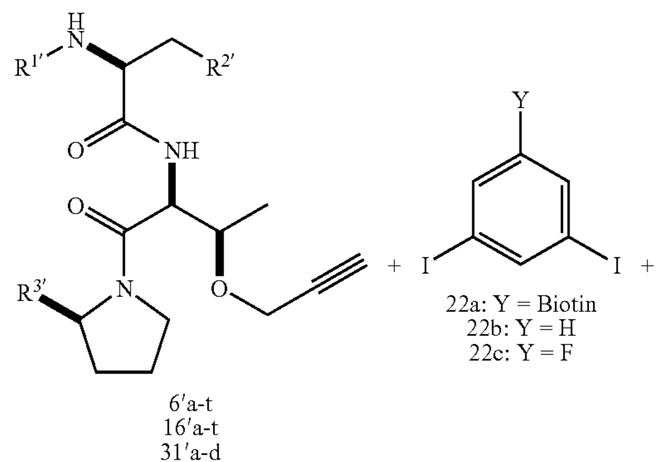
Scheme 13
