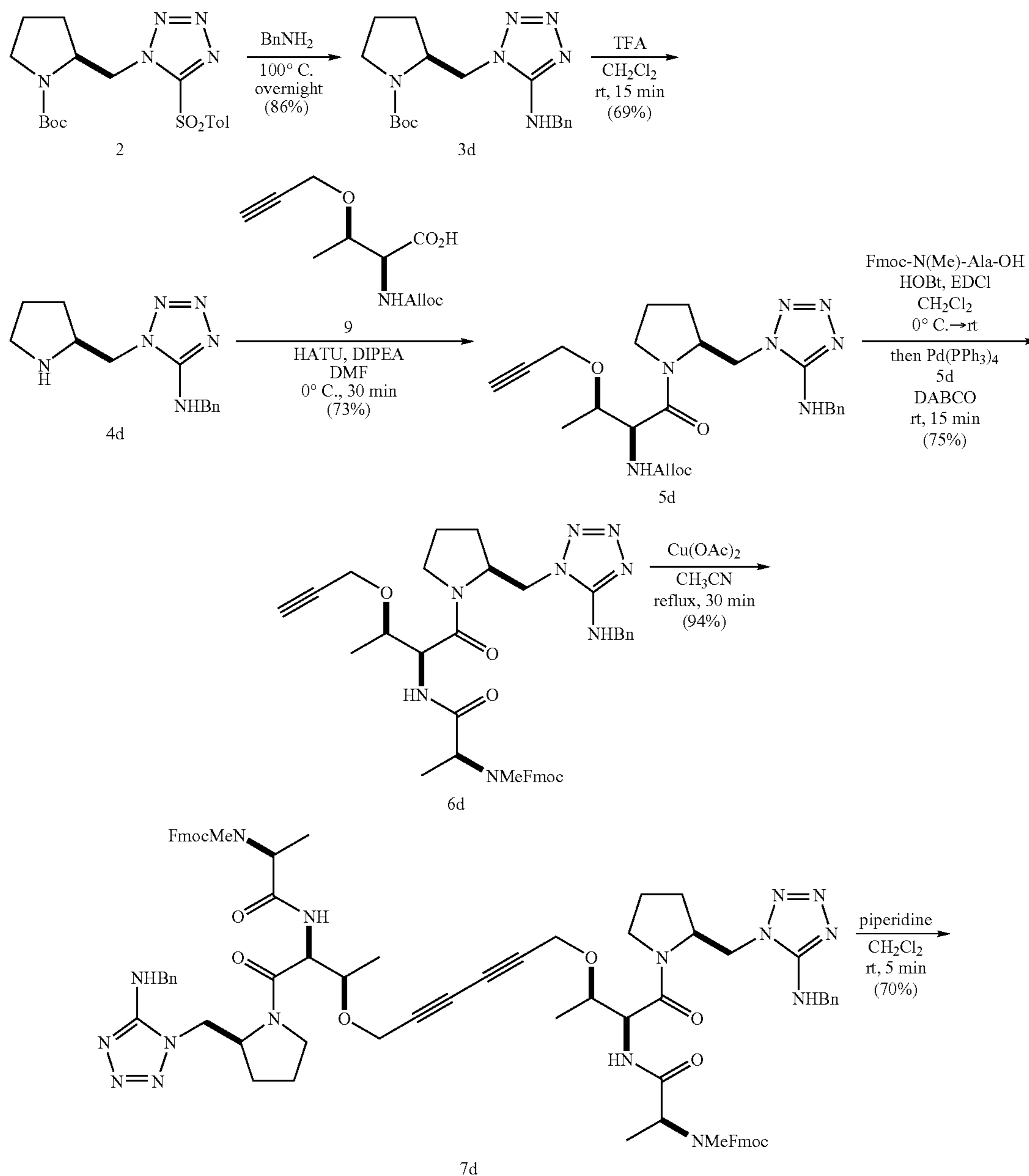
Scheme 4
