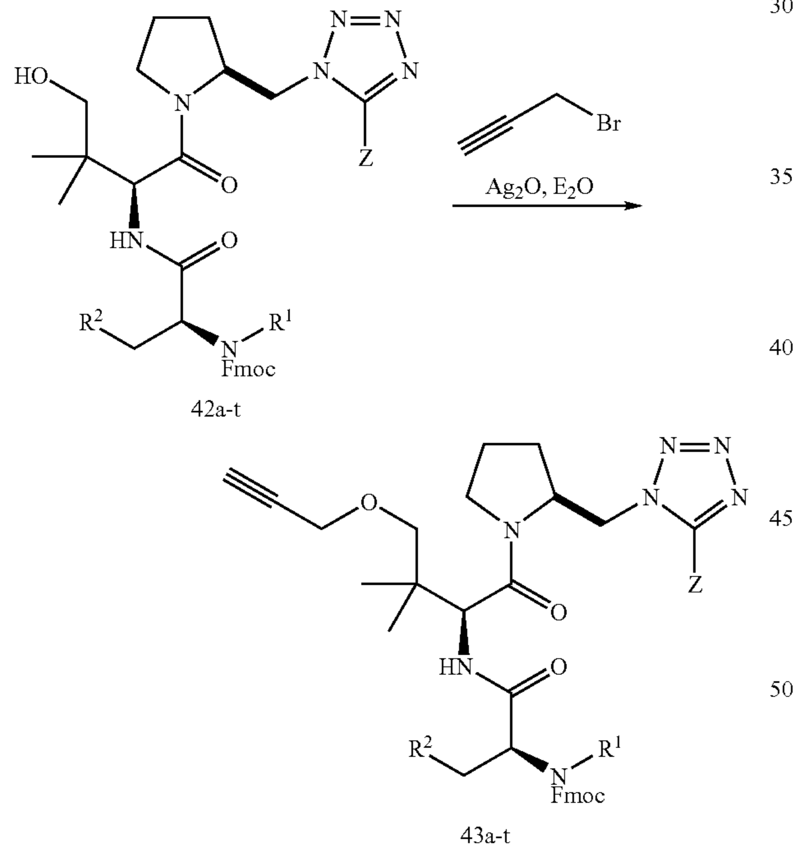
Scheme 15
