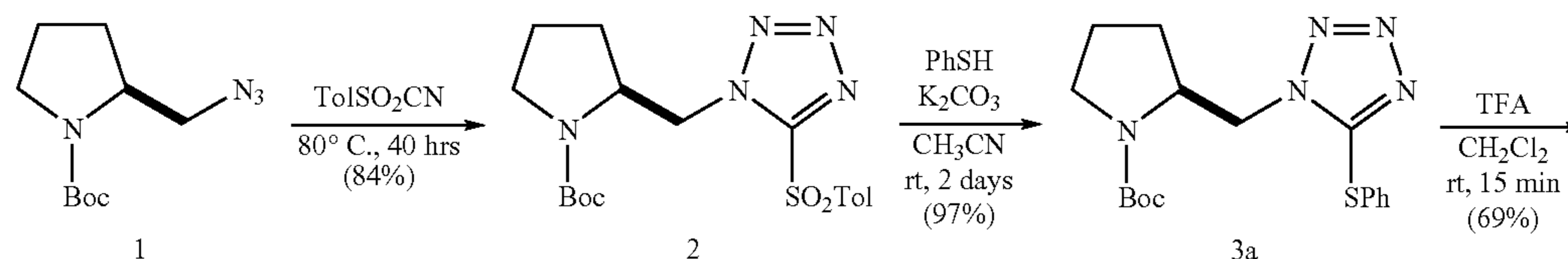
Scheme 1
