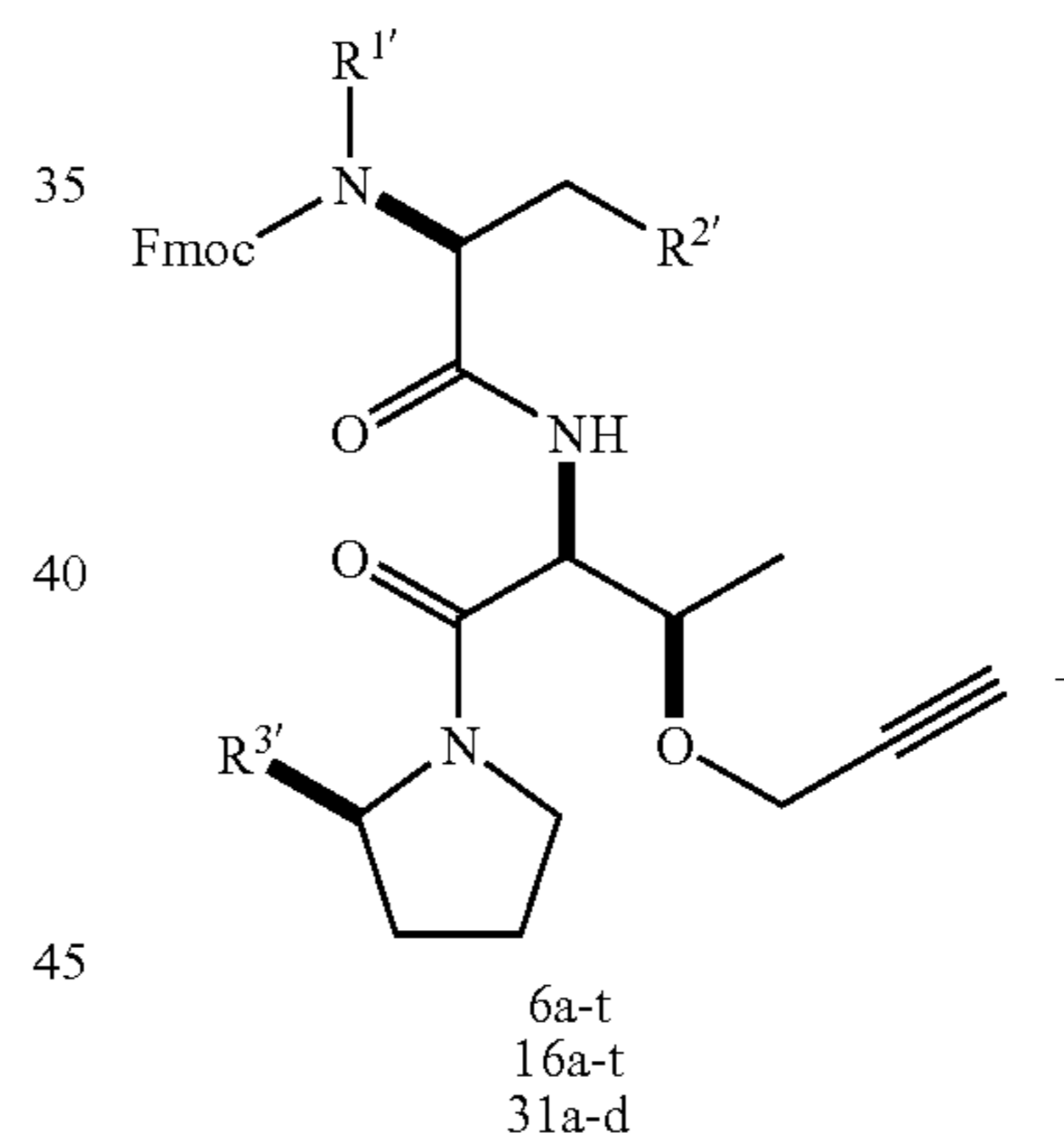
Scheme 12
