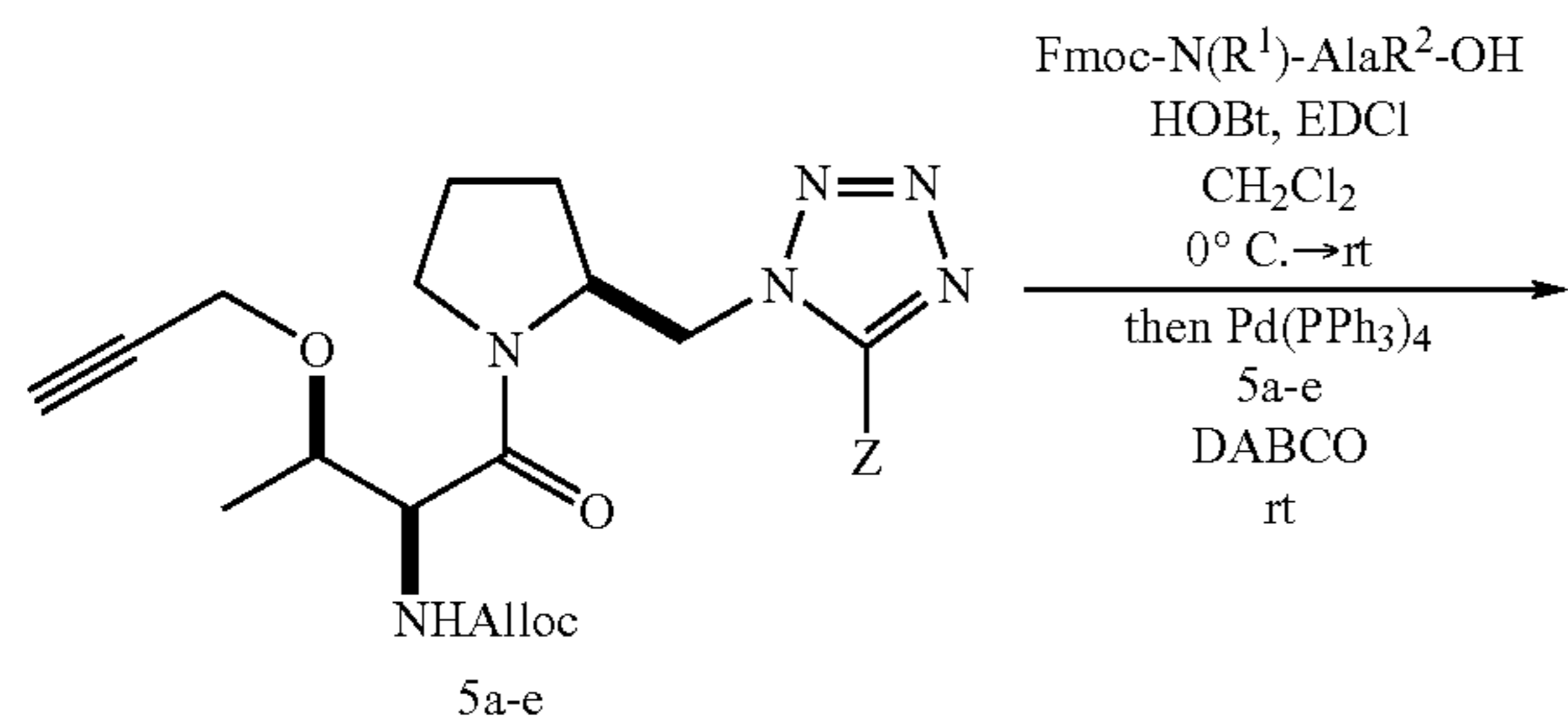
Scheme 9
