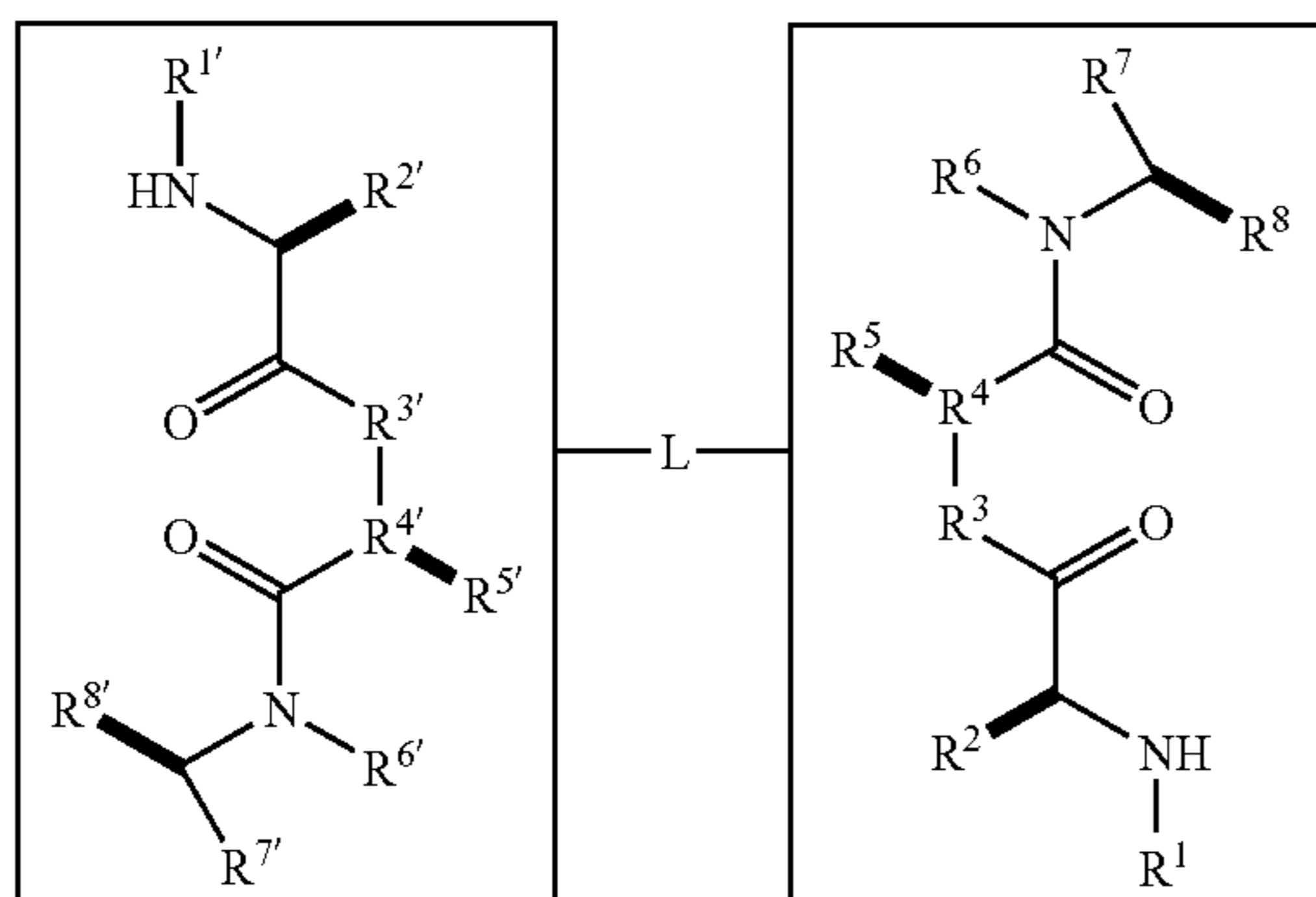
formula II
