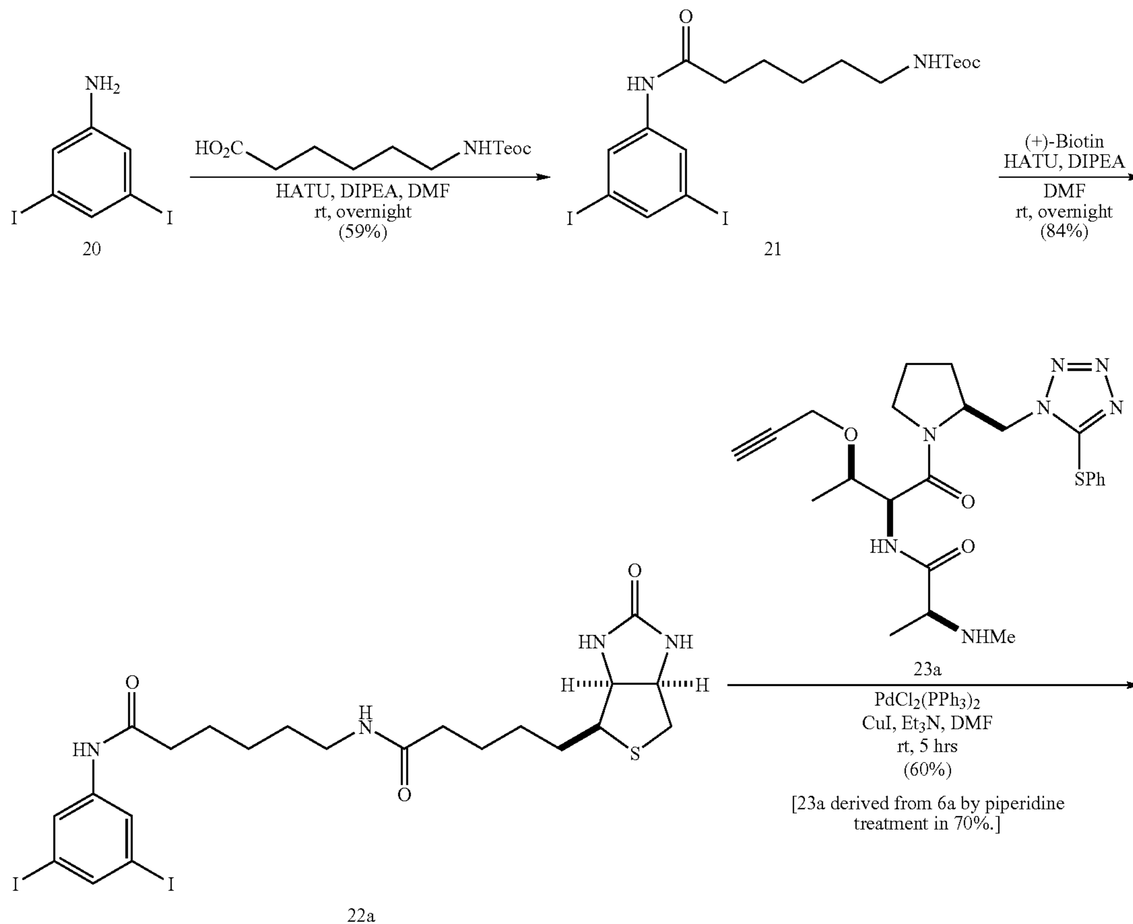
Scheme 7
