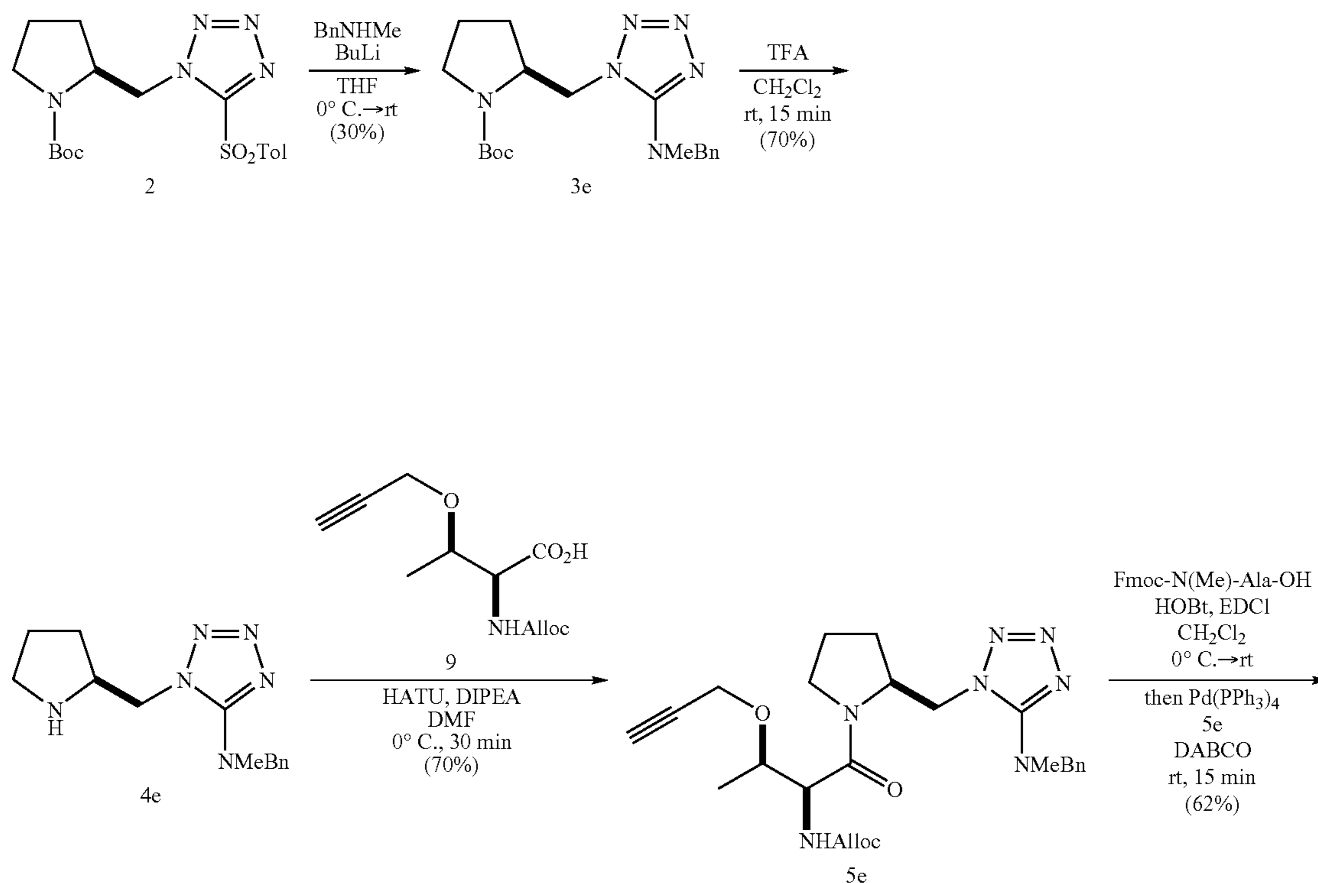
Scheme 5
