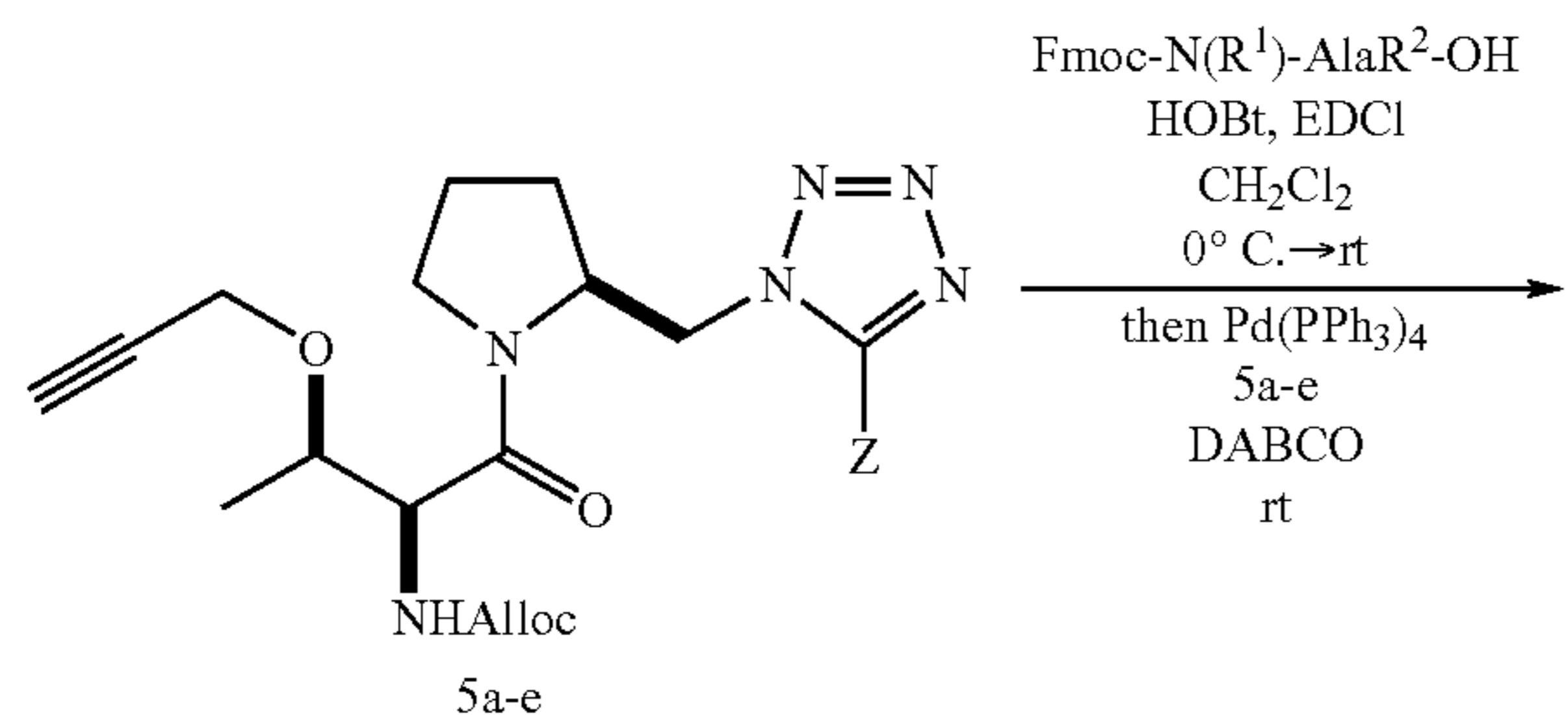
Scheme 9
