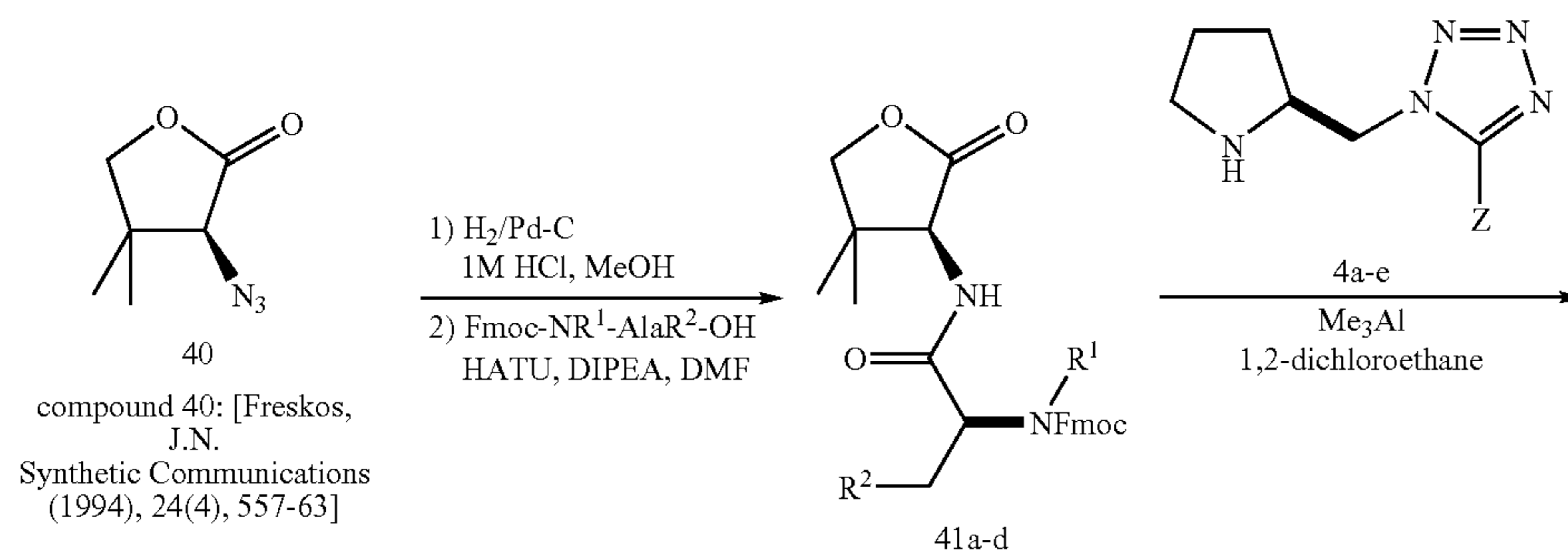
Scheme 14
