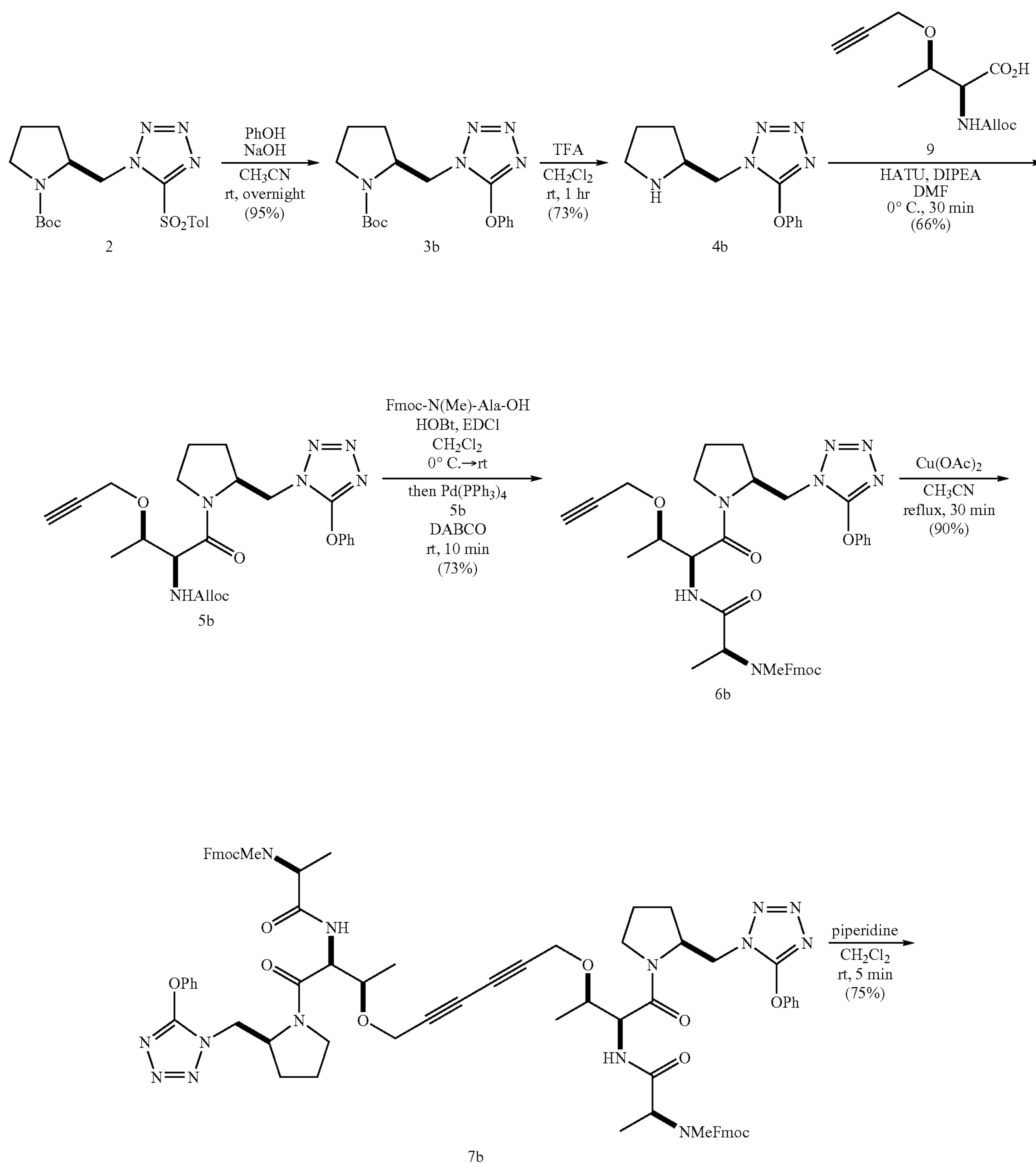
Scheme 2
