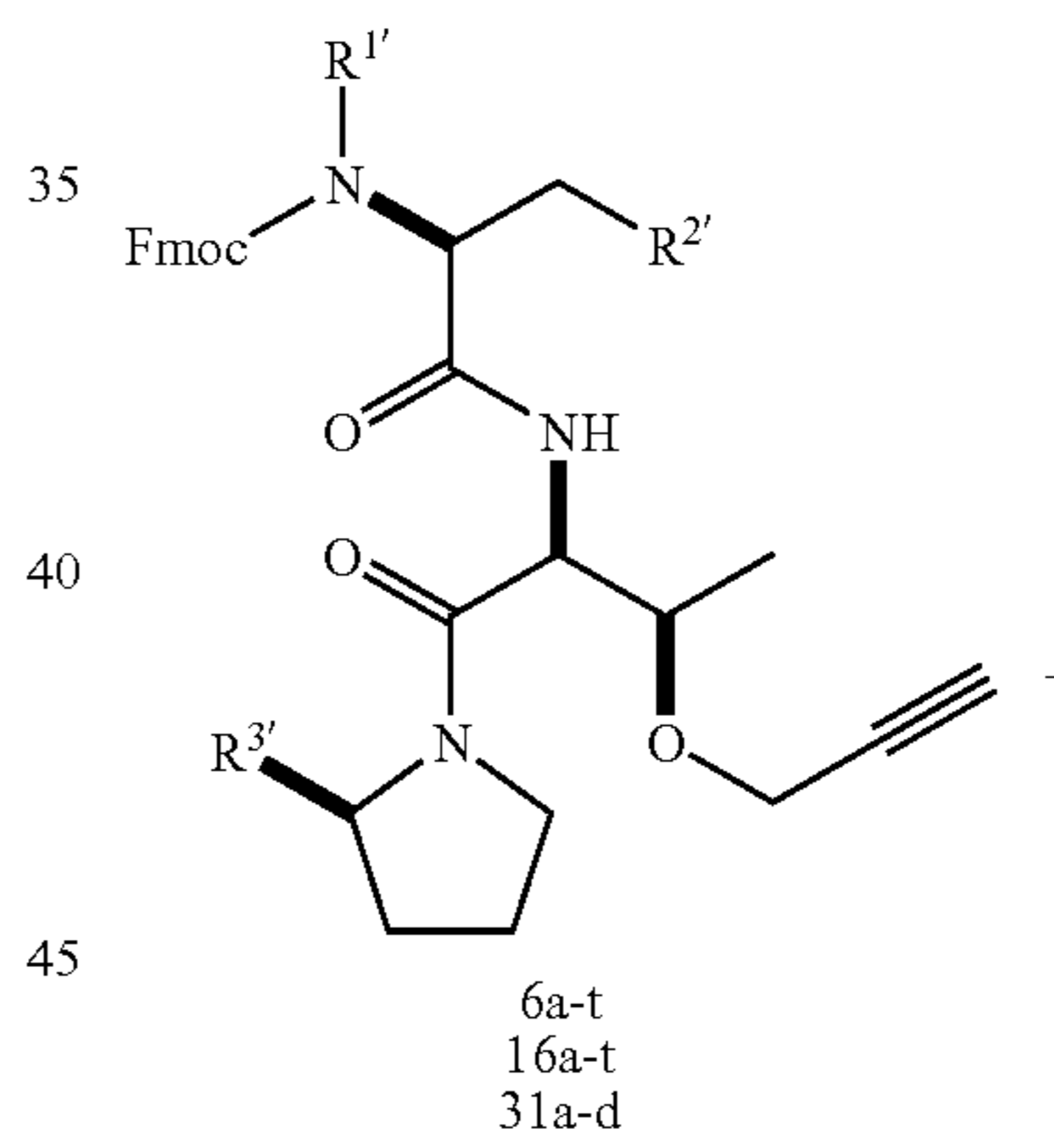
Scheme 12
