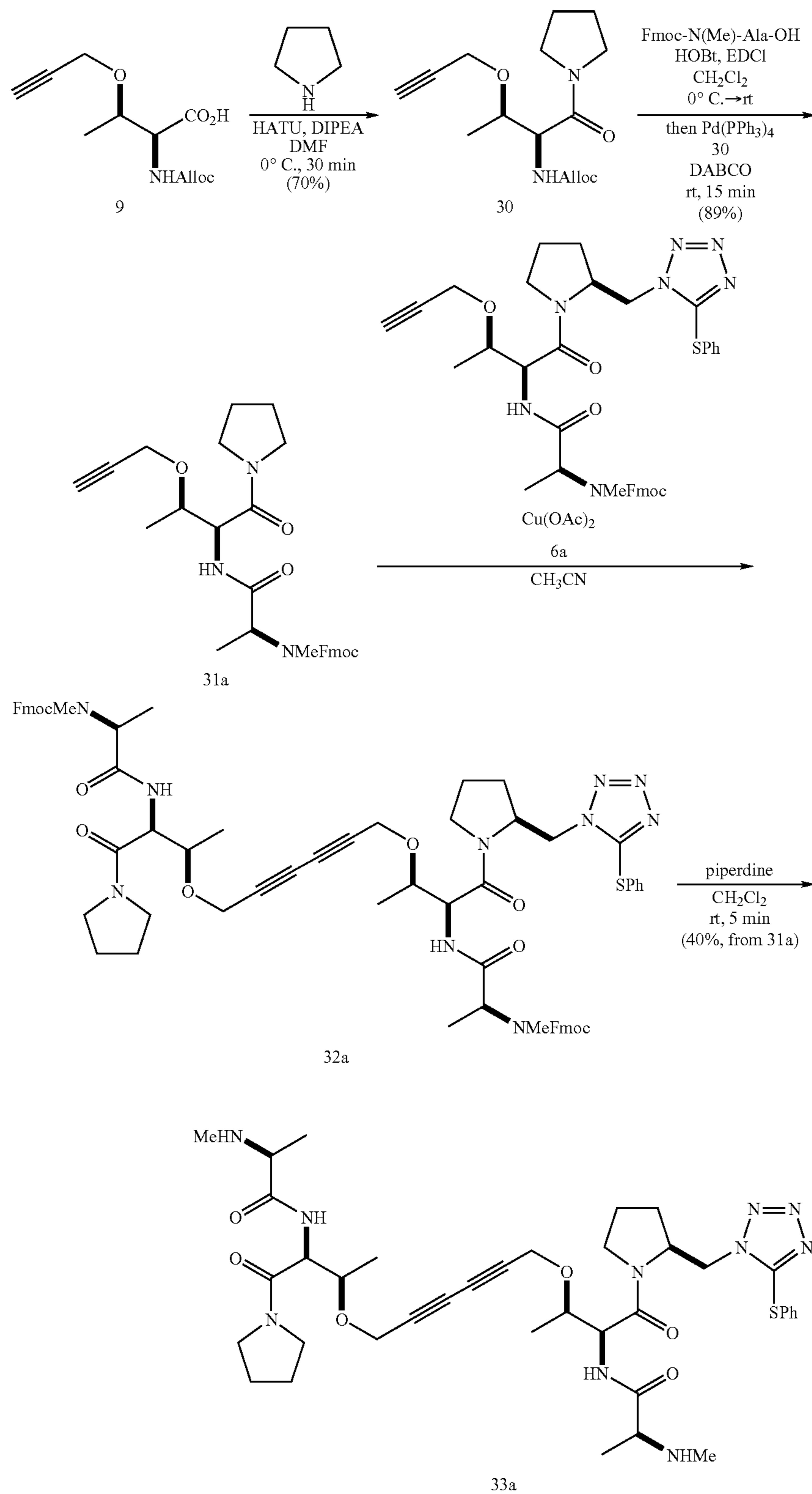
Scheme 8
