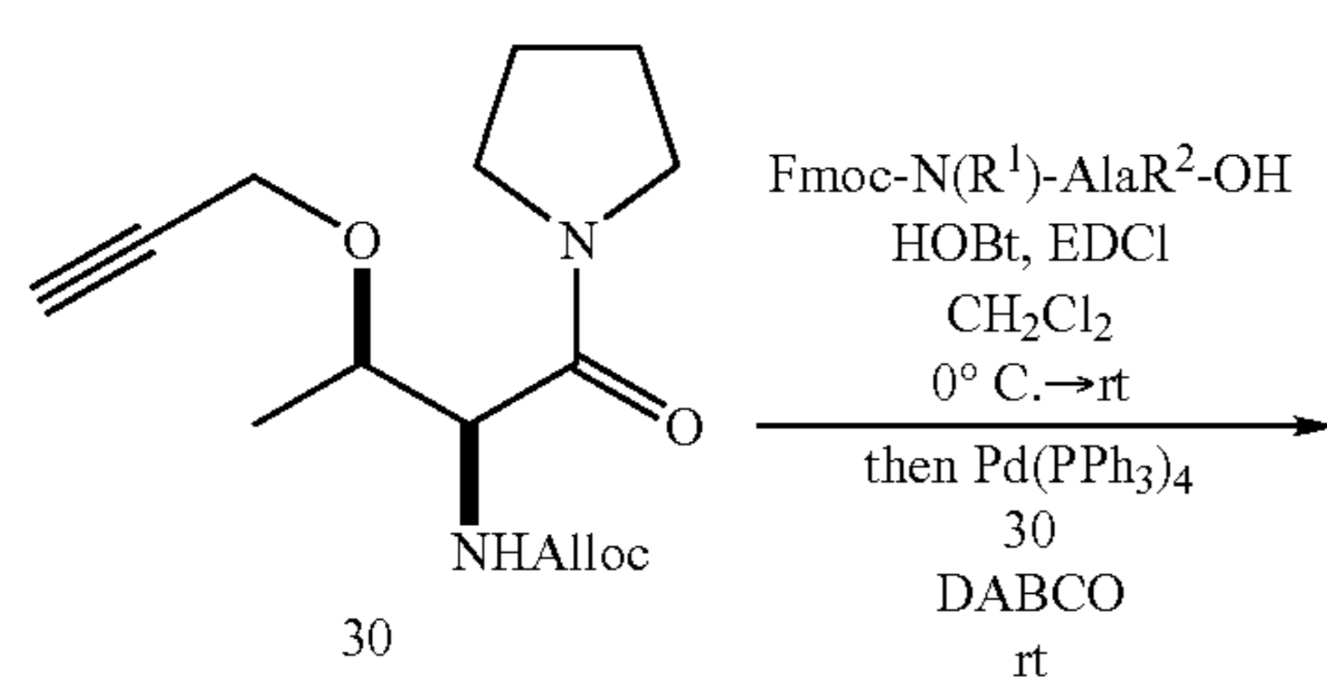
Scheme 11
