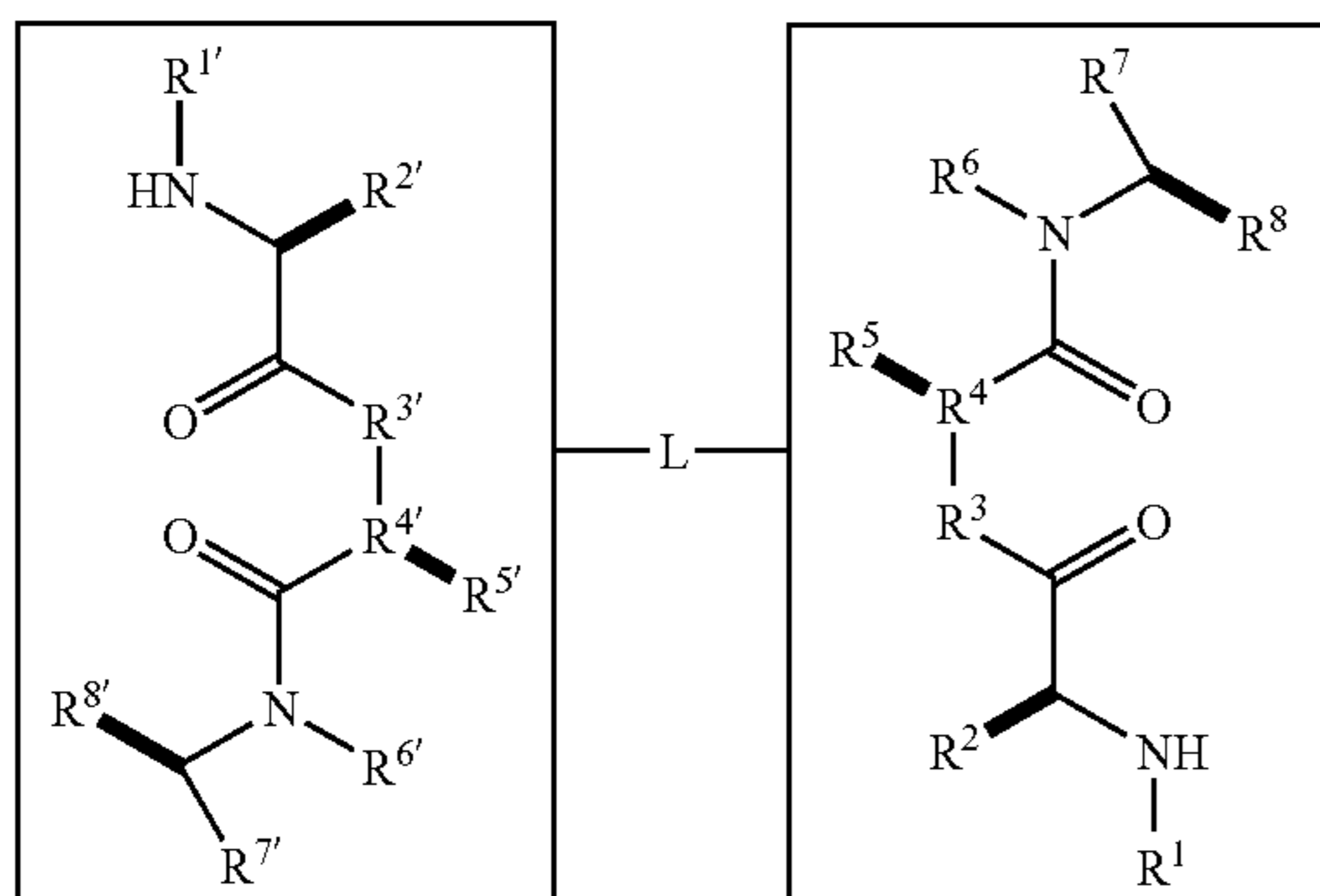
formula II
