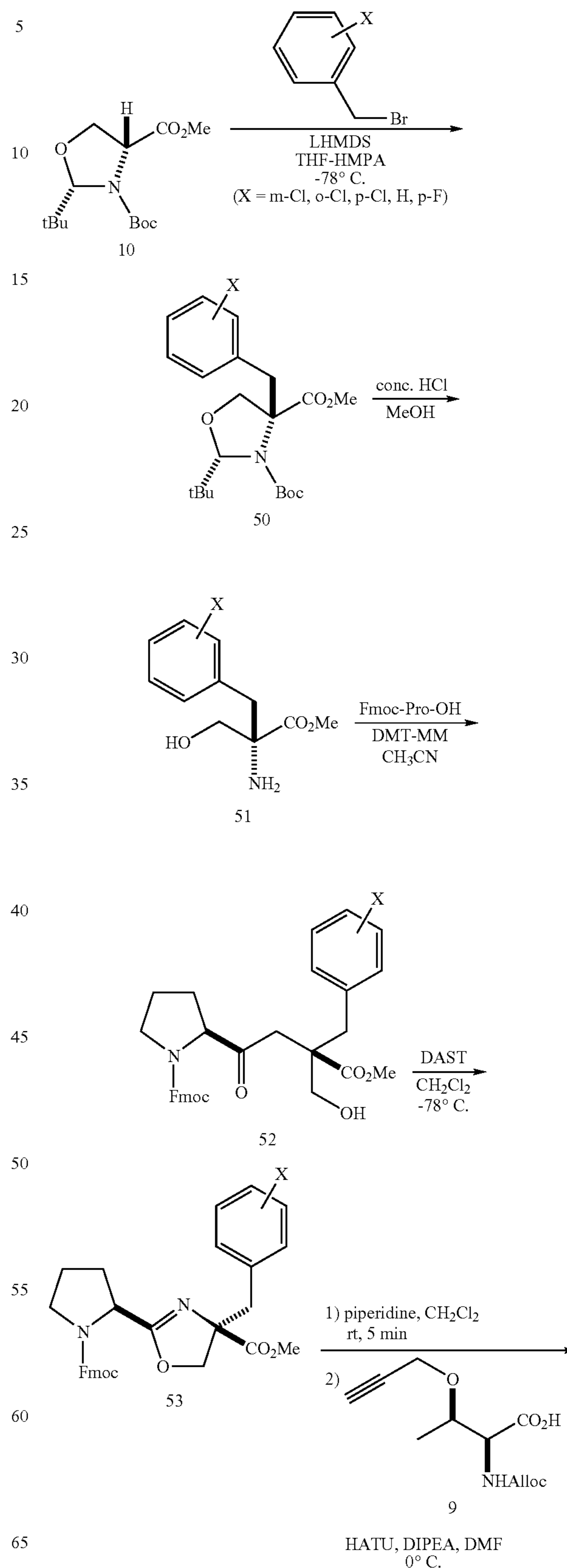
Scheme 10
