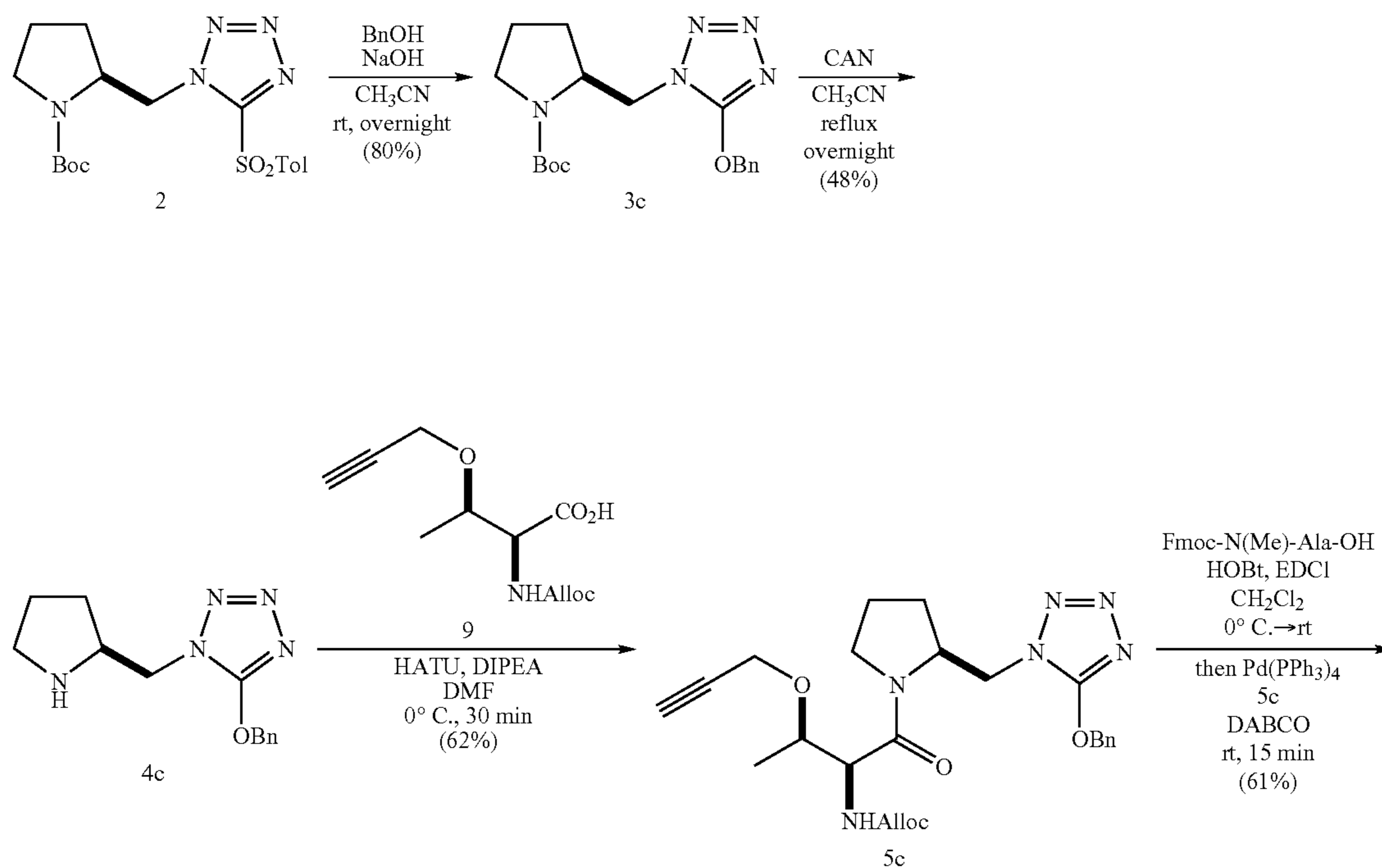
Scheme 3
