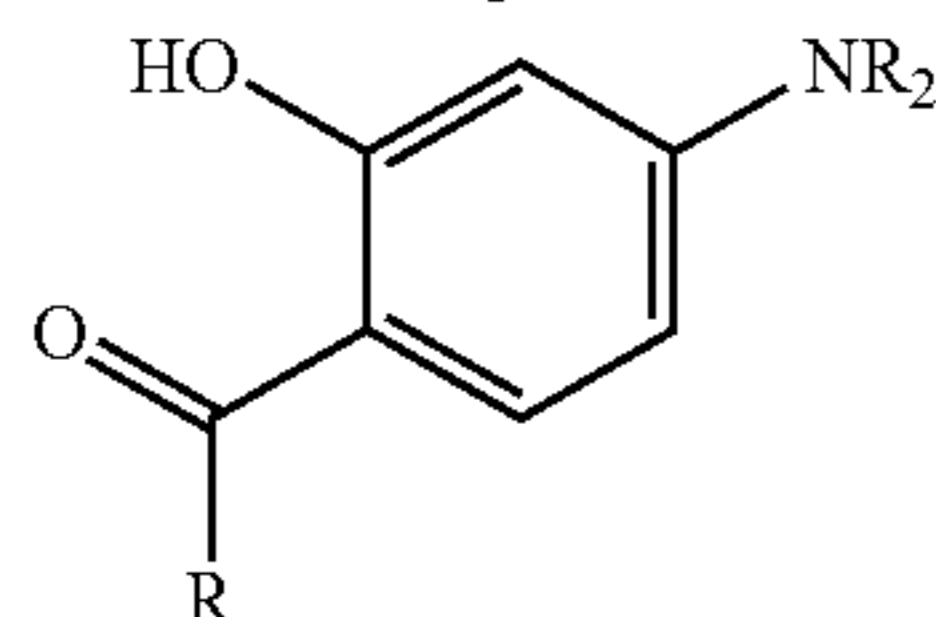
a 6-acyl-3-aminophenol
