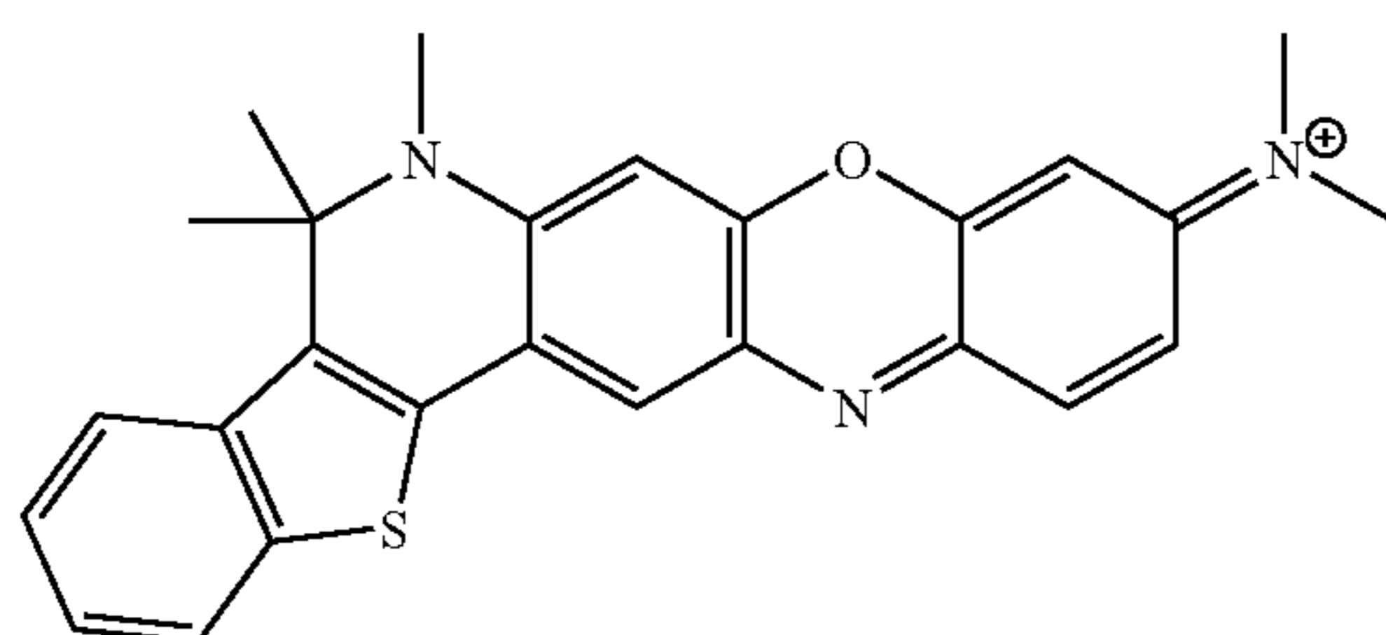
Compound 39
