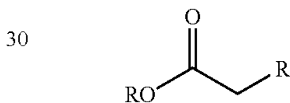
an alpha-methylene ester
