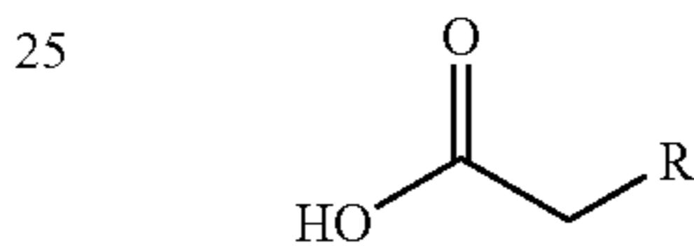
an alpha-methylene acid
