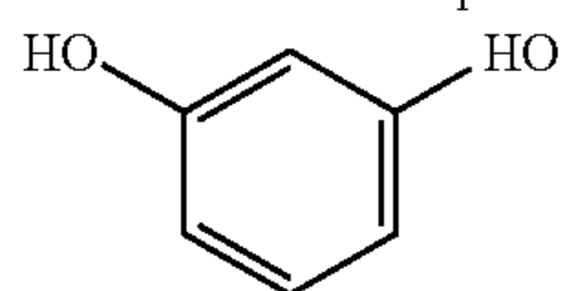
a resorcinol
