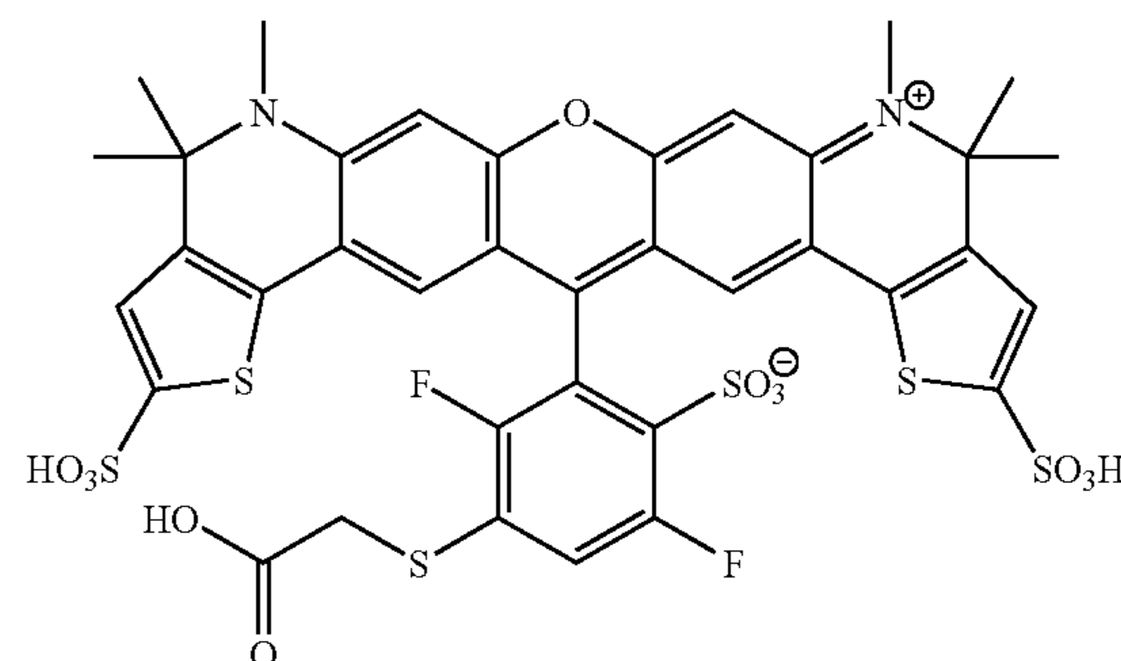
Compound 41
