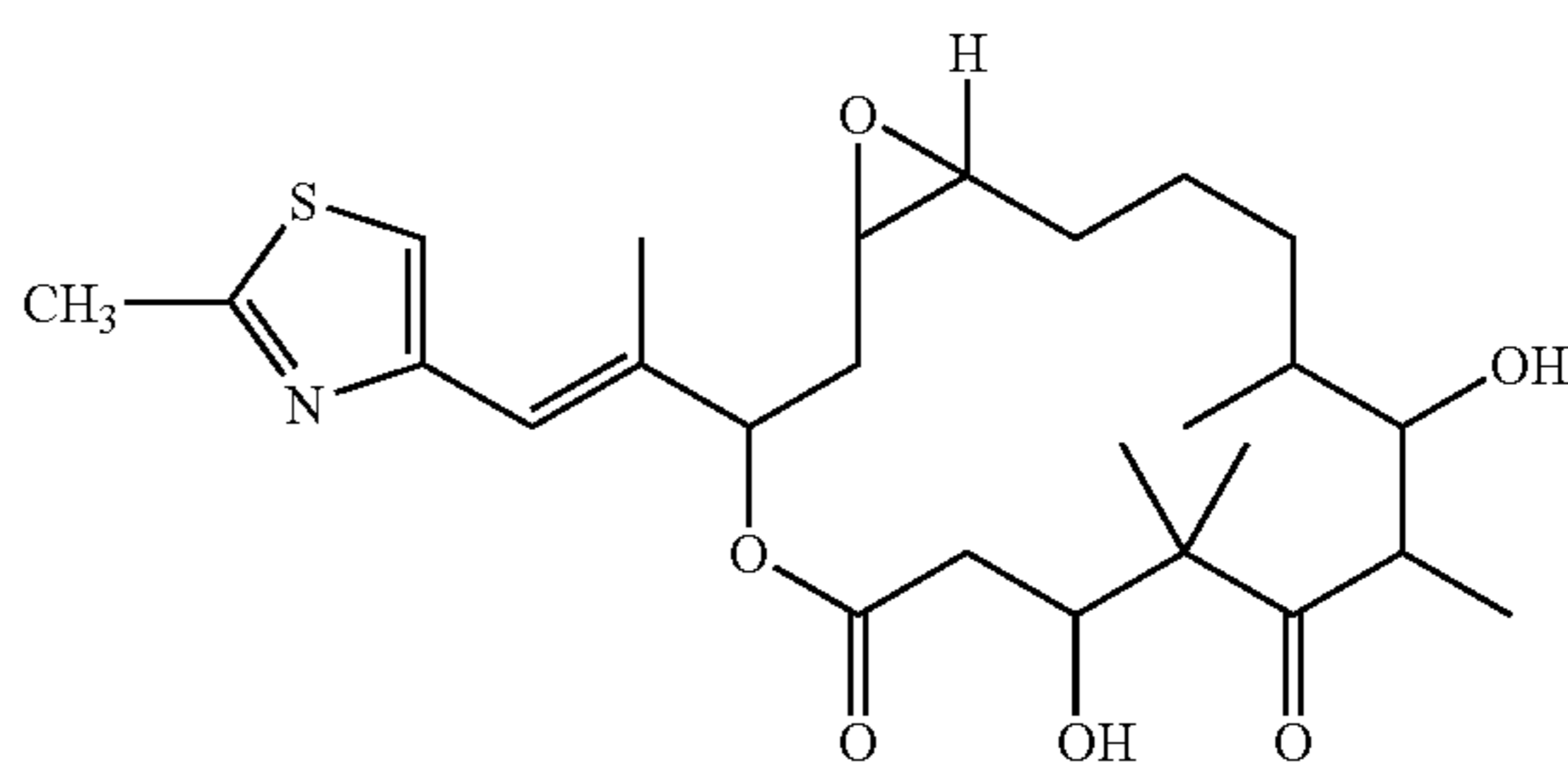
Epothilone B
