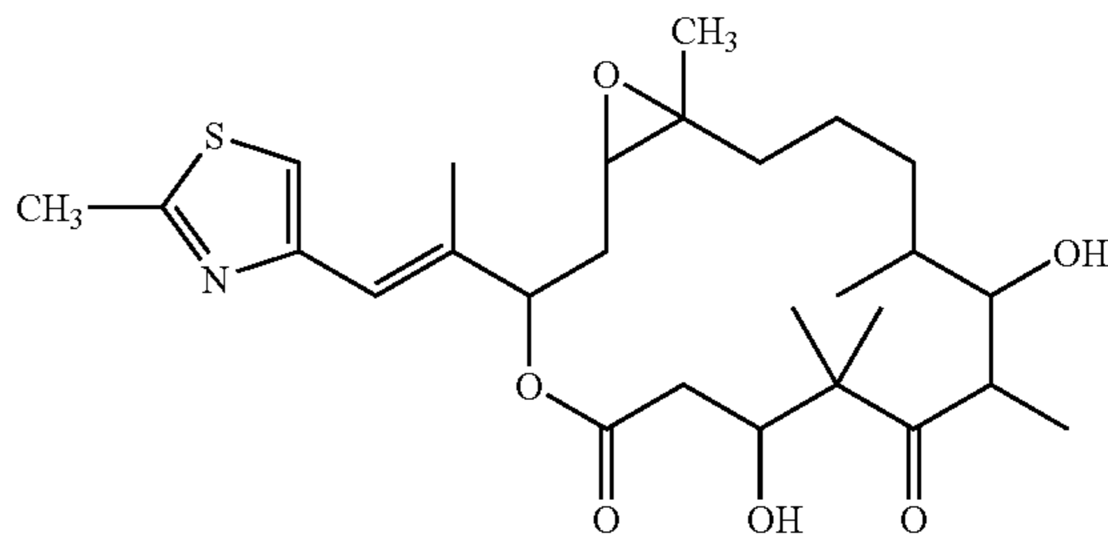
Epothilone B
