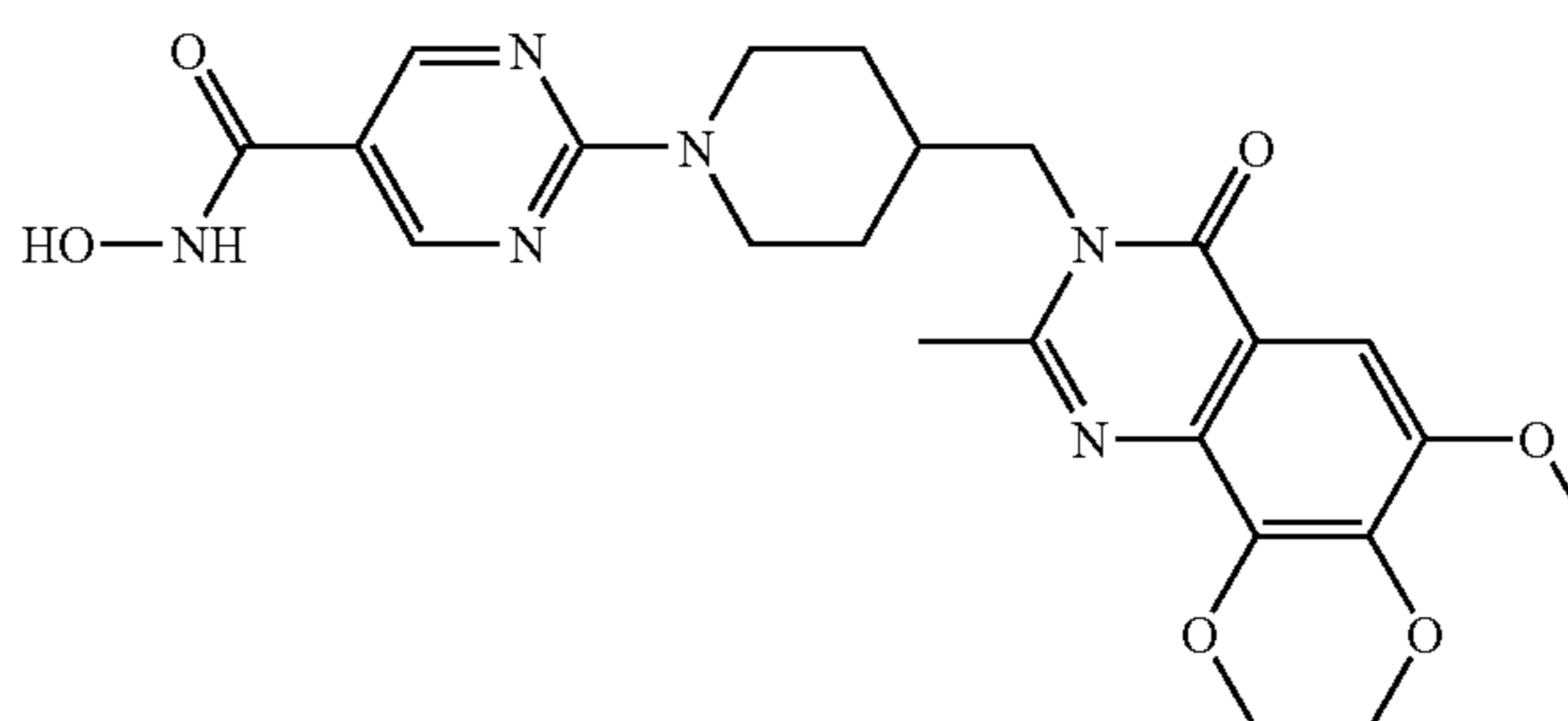
compound 8
