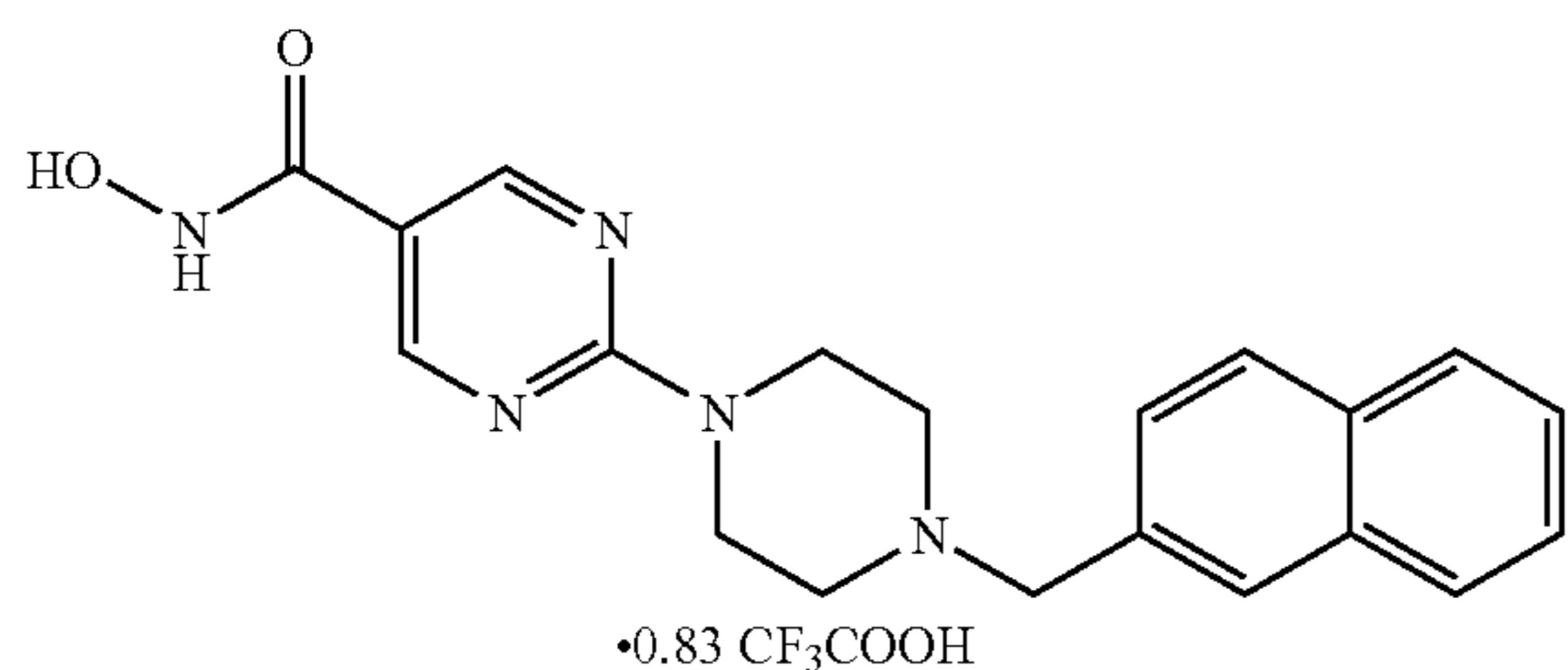
compound 6
