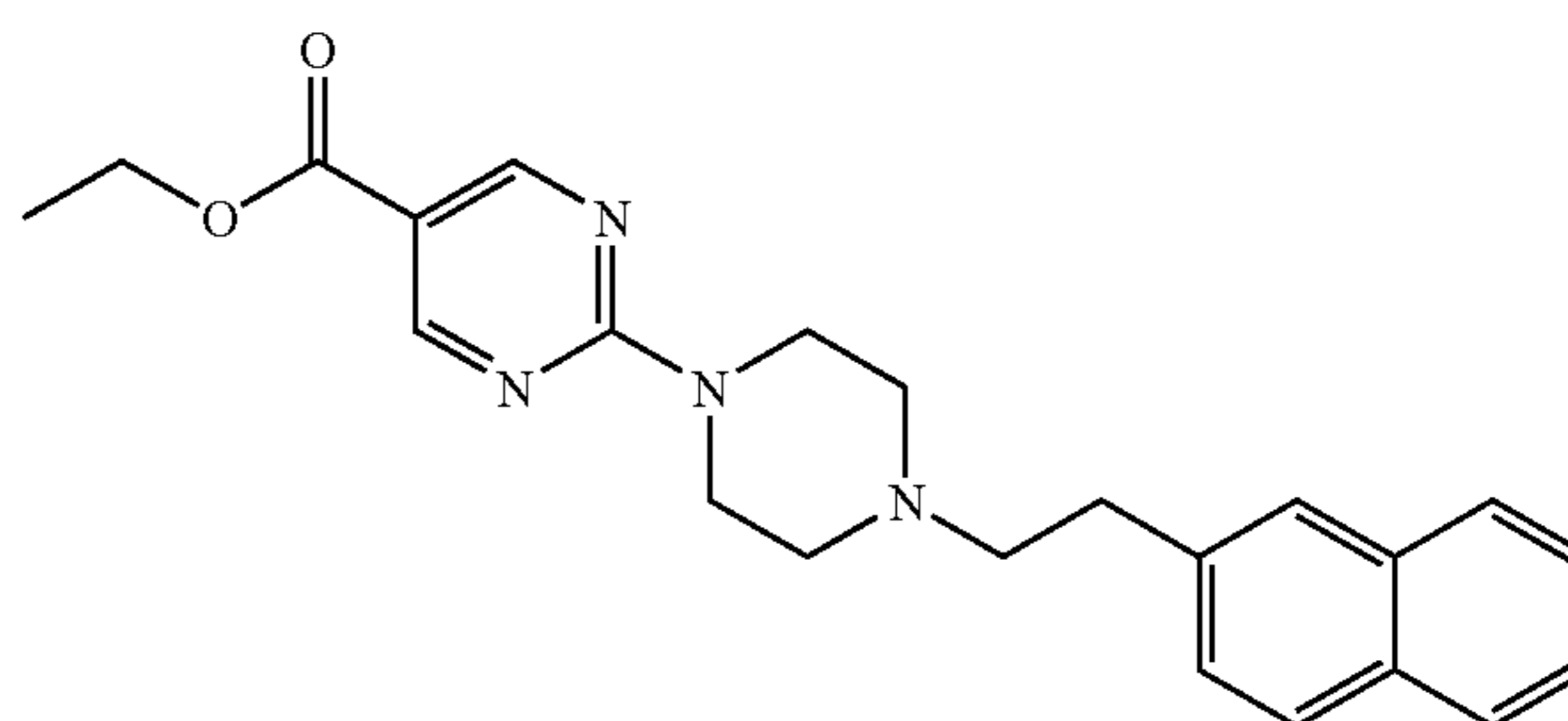
compound 5
