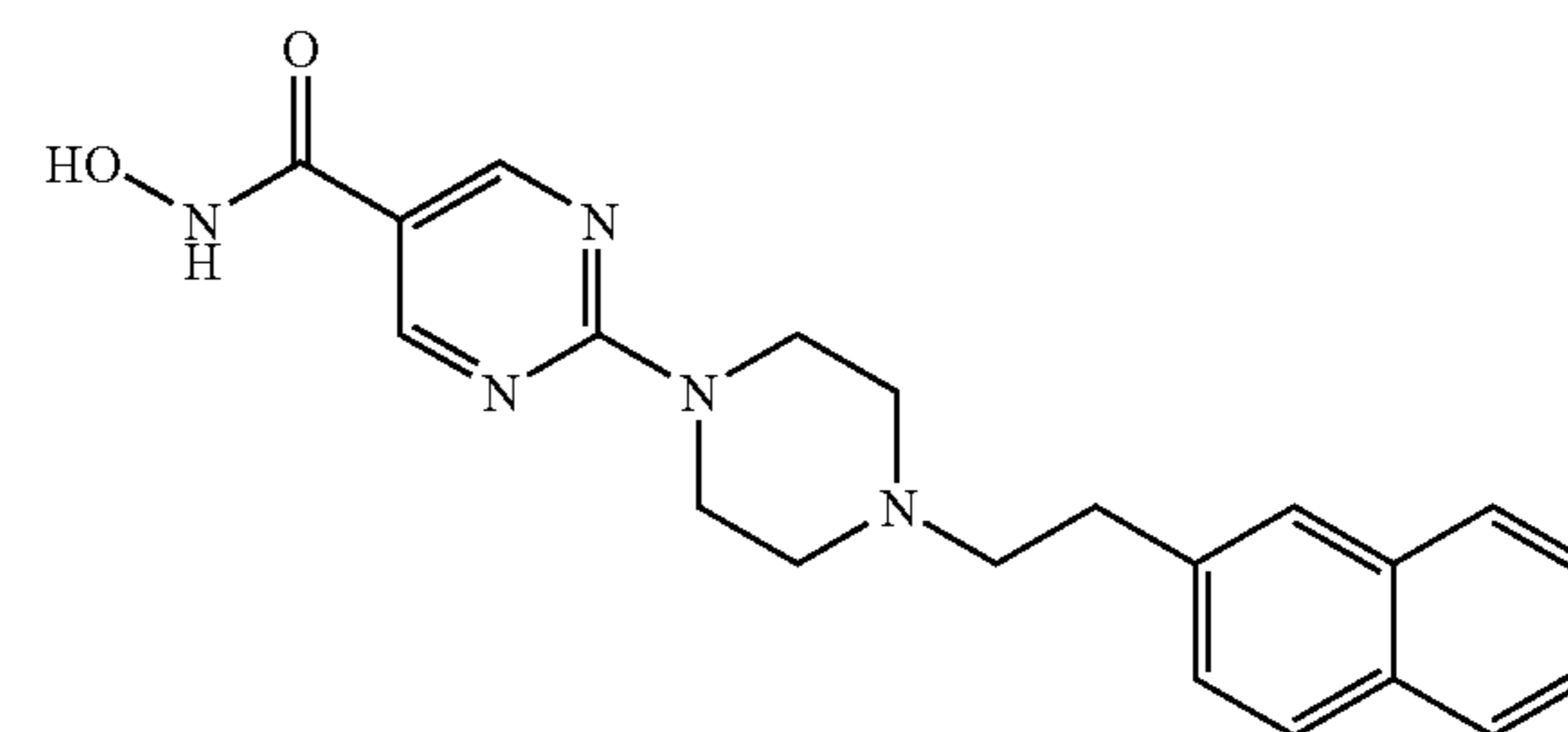
intermediate 28
