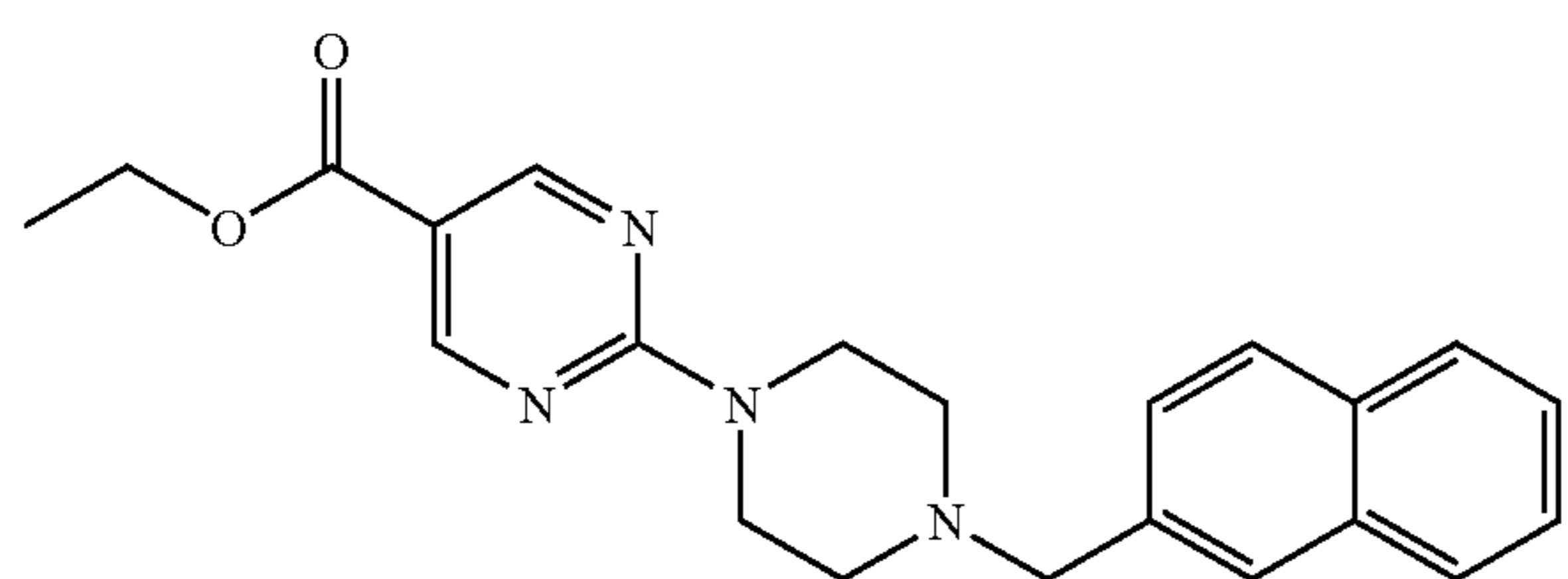
intermediate 28
