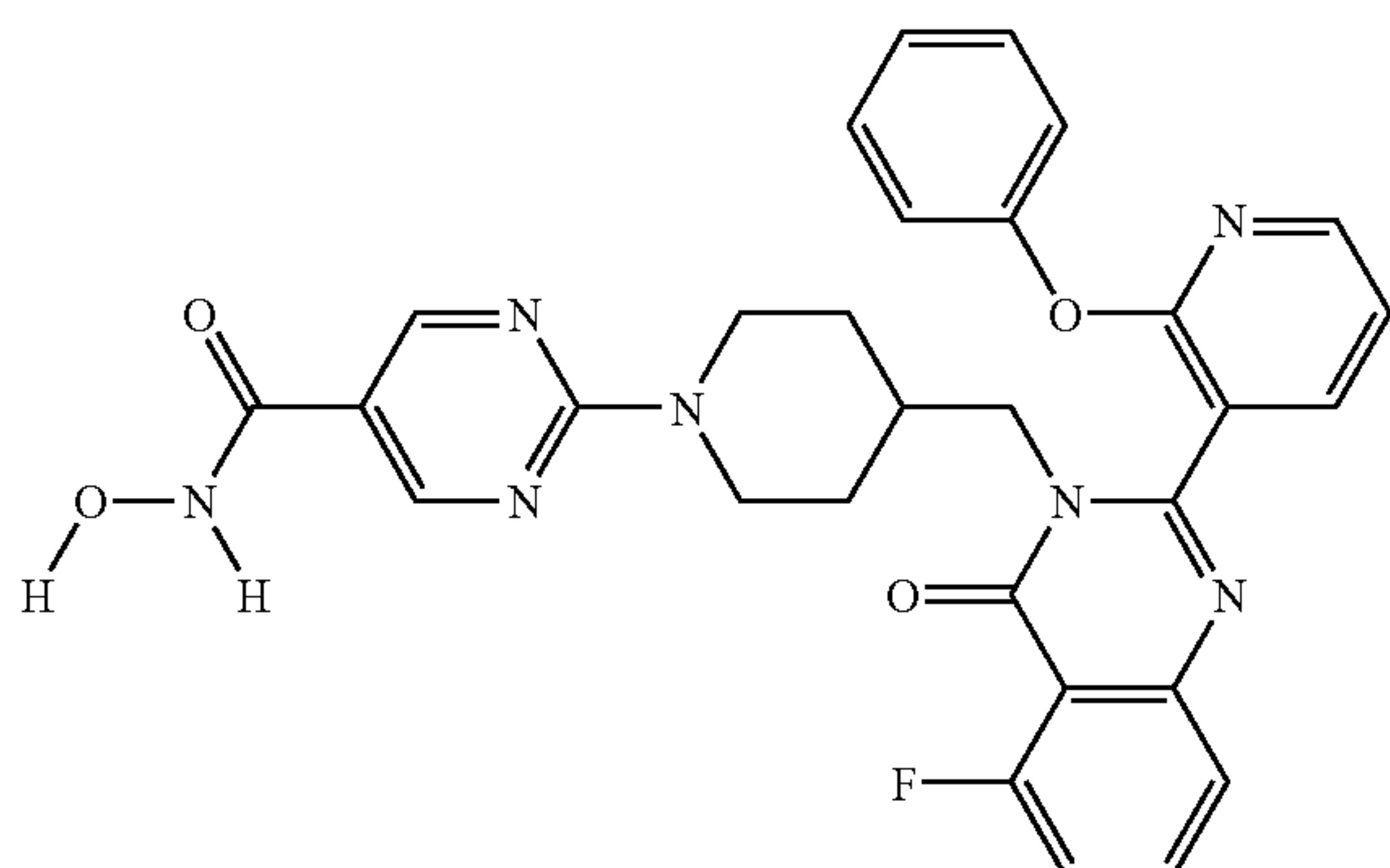
C 2 HF 3 O 2 (1:1); Co. No.53; Ex. [B11]
