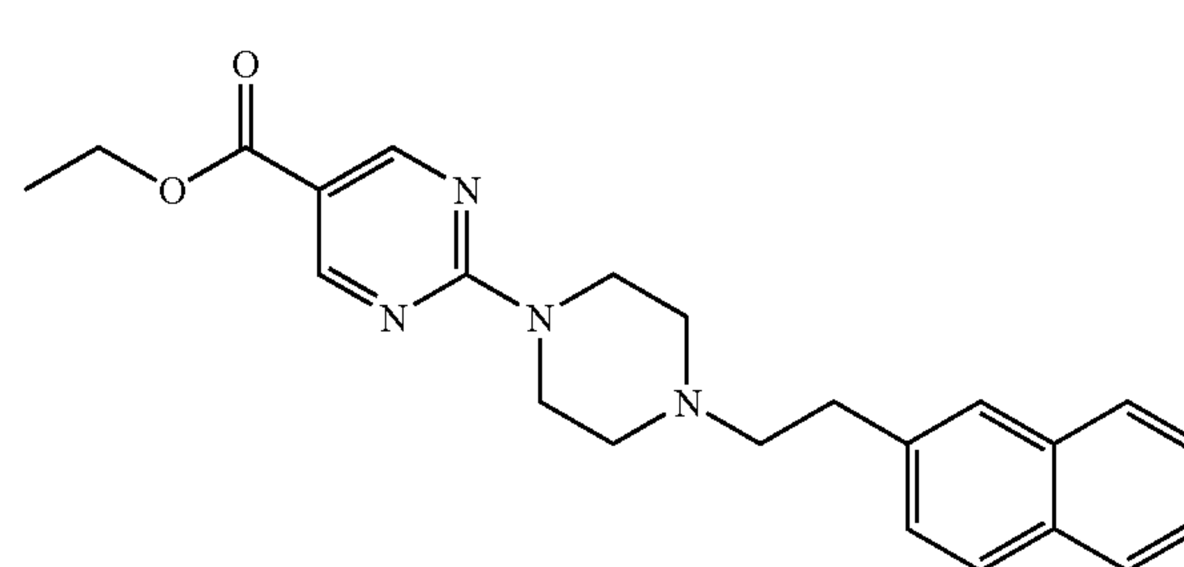
compound 5
