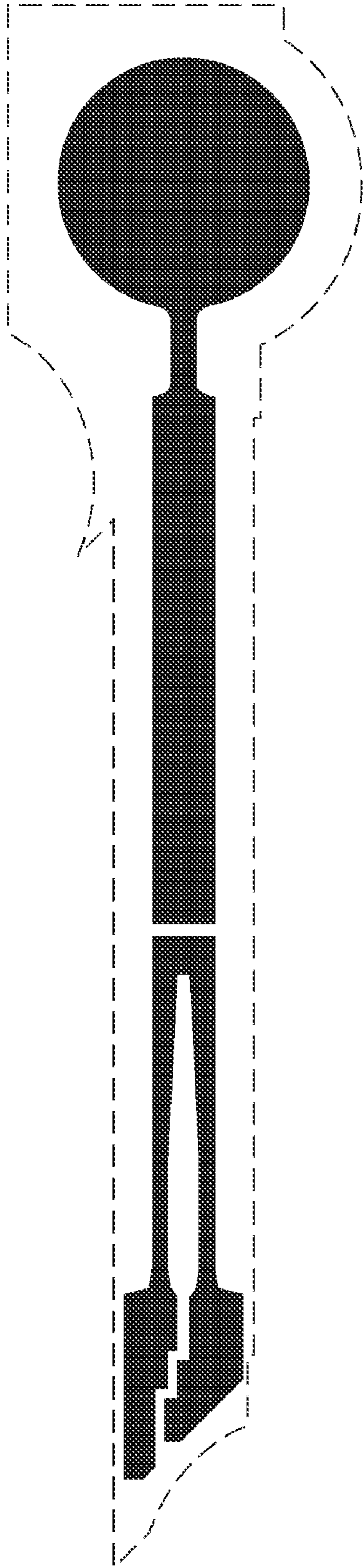
Heater mask
