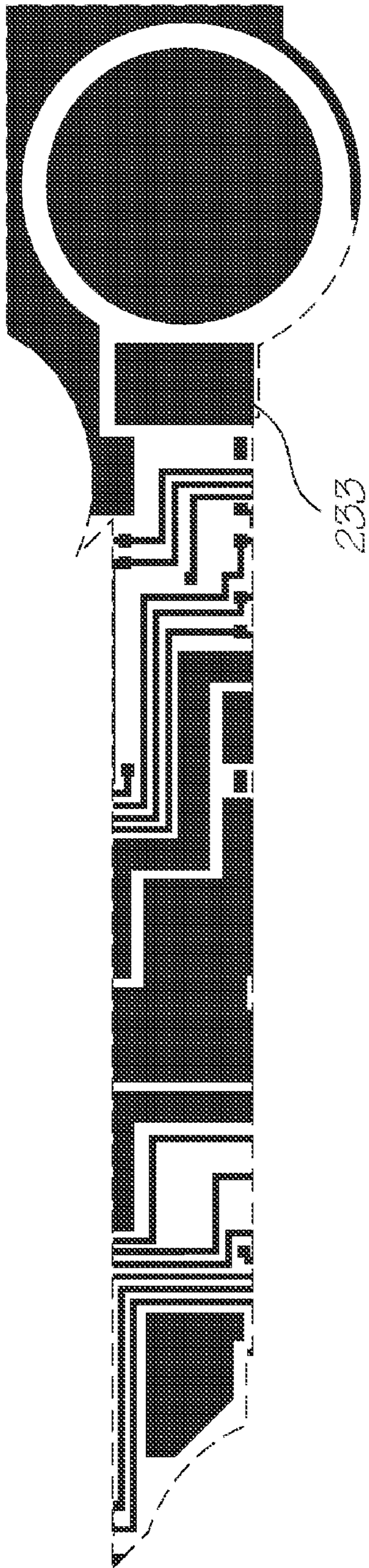
Metal 2 mask
