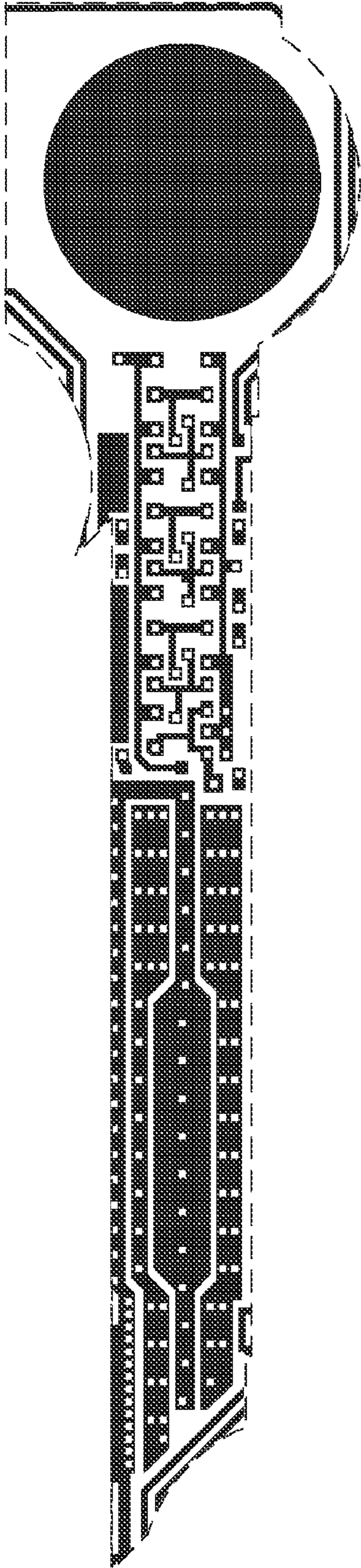
Metal 1 mask
