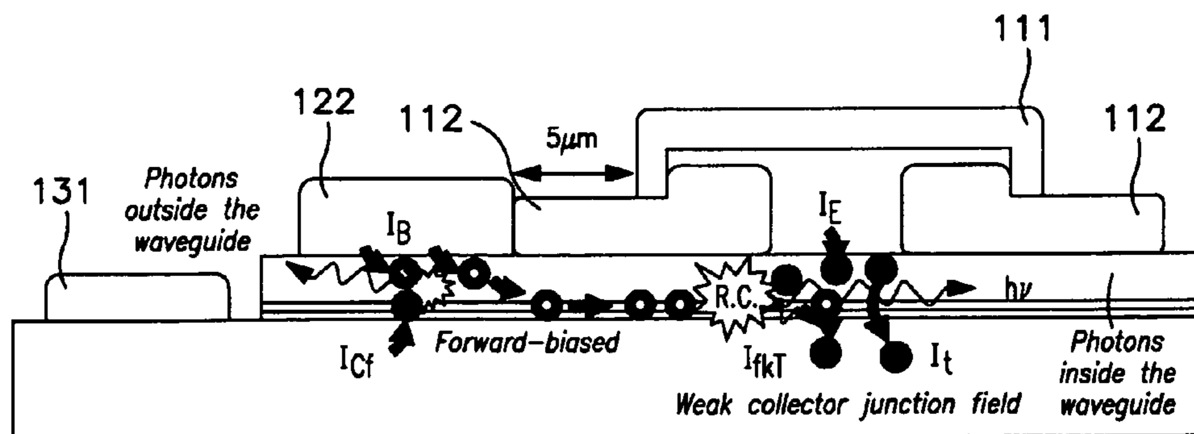
Weak collector junction field in the presence of an optical field
