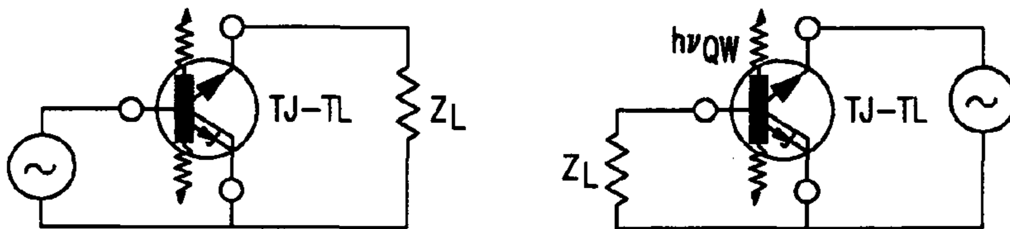
(c) Common-Collector
