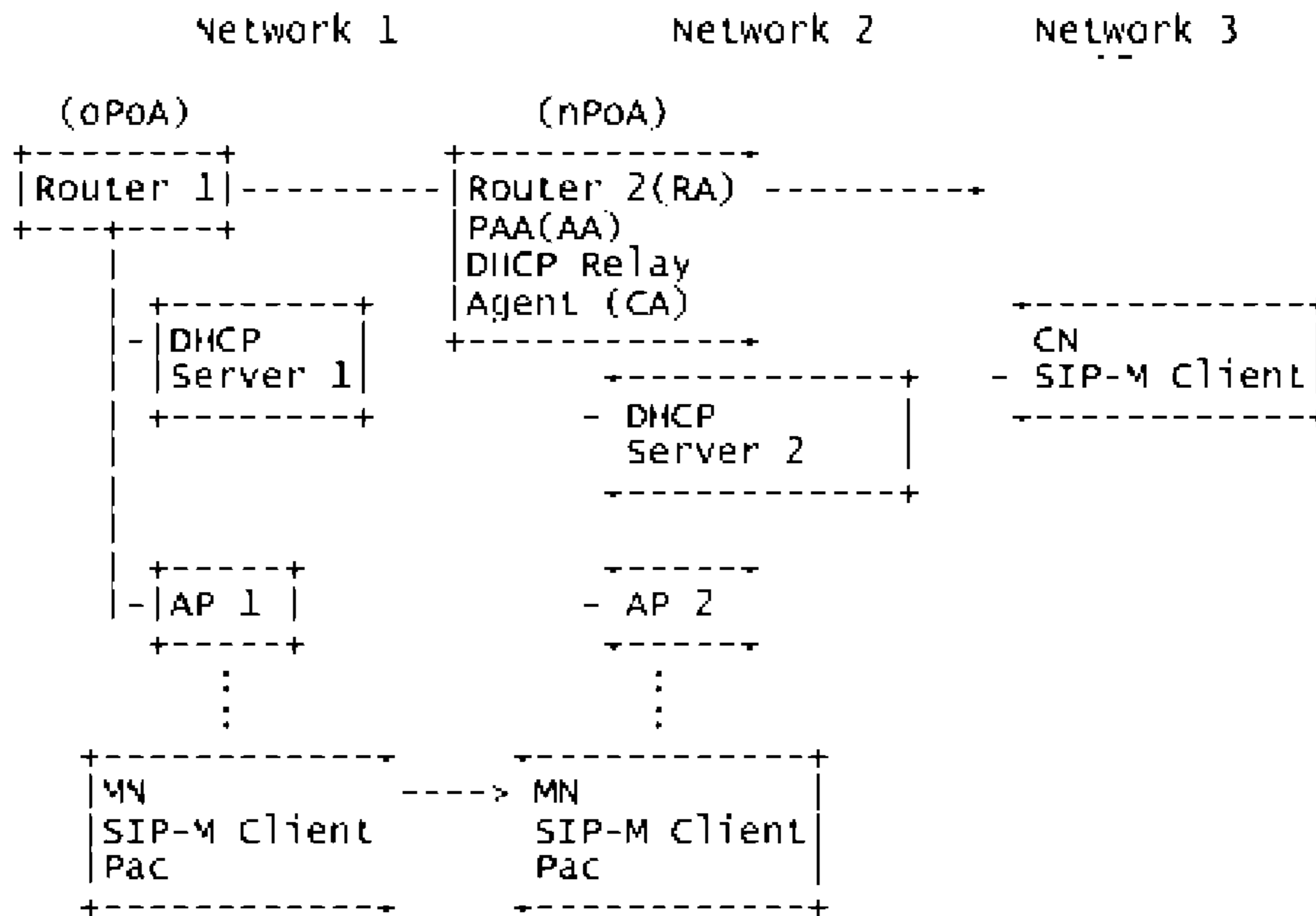
Figure 4: Network Structure
