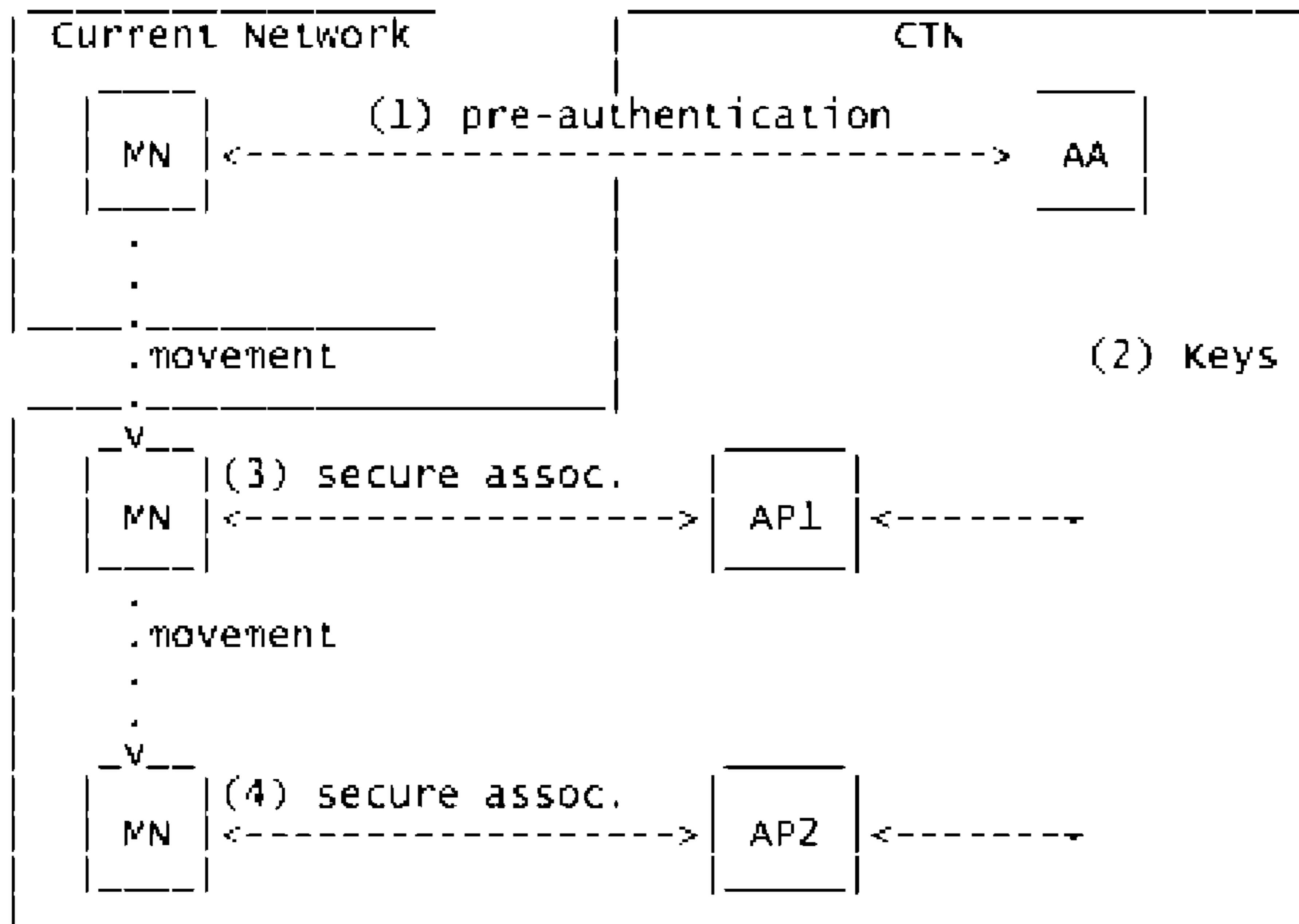
Figure 3: Bootstrapping Link-layer Security
