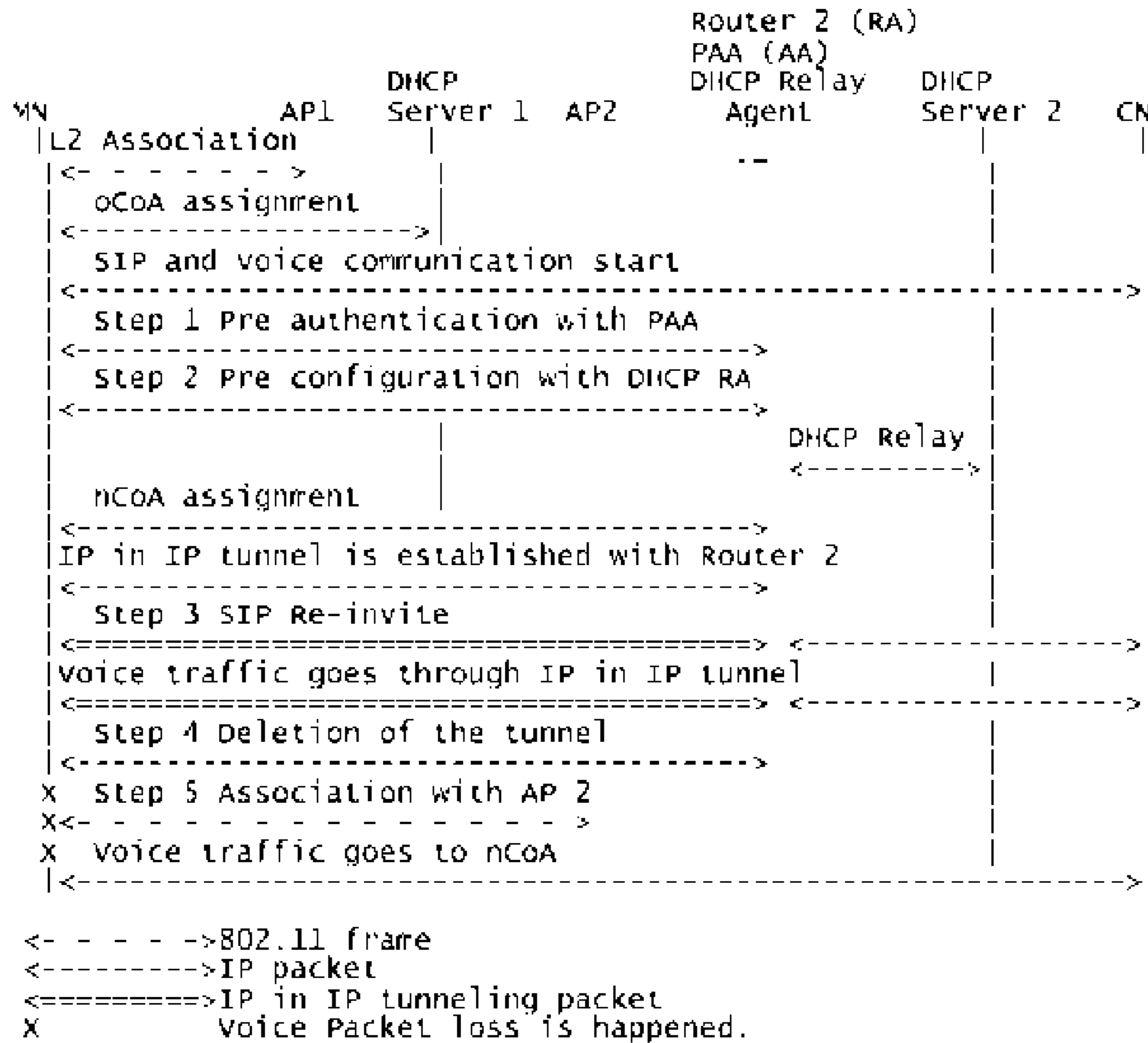
Figure 5: MPA Communication Flow in the implementation environment
