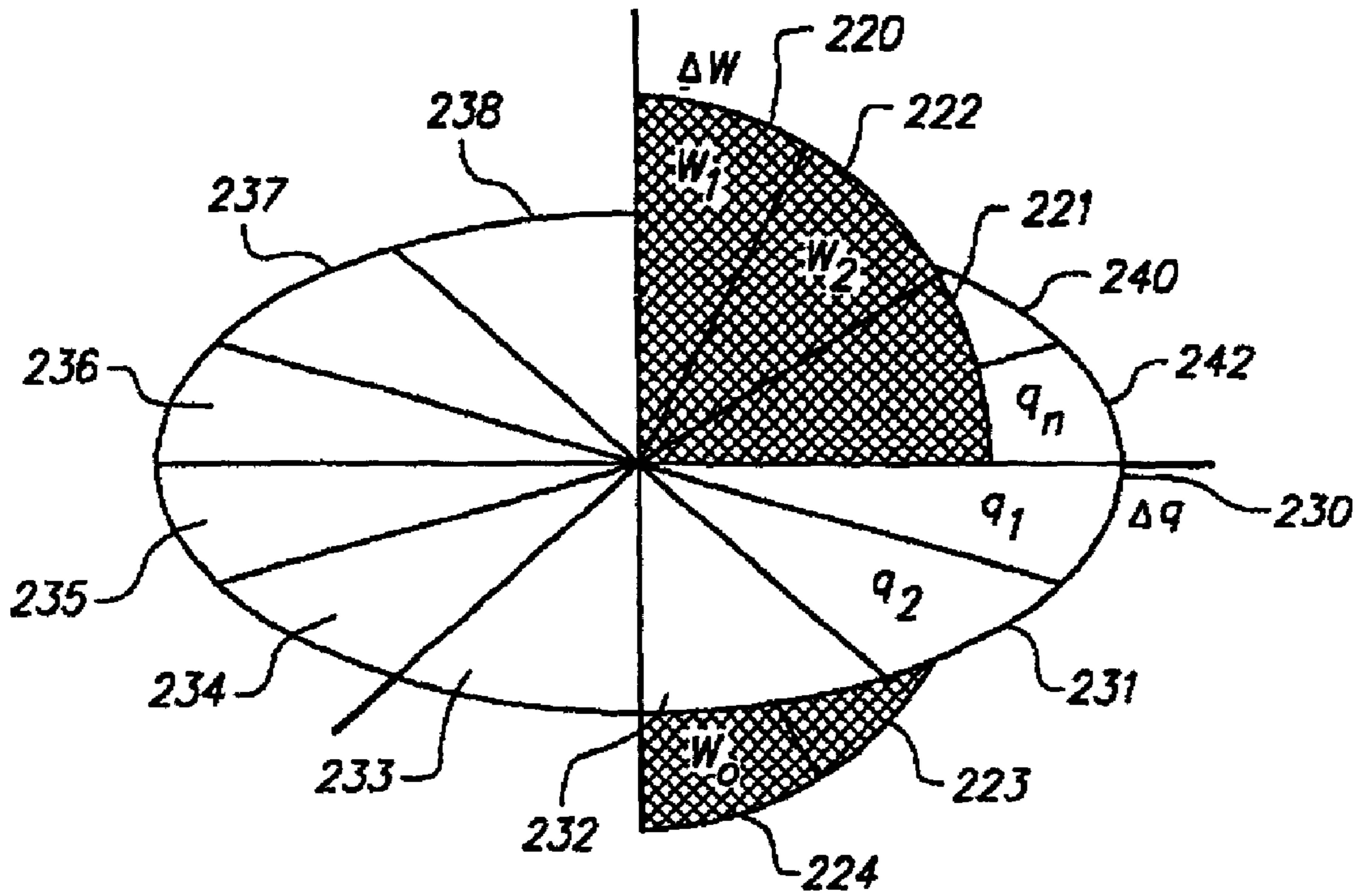
FIG. 12 (Prior Art)
