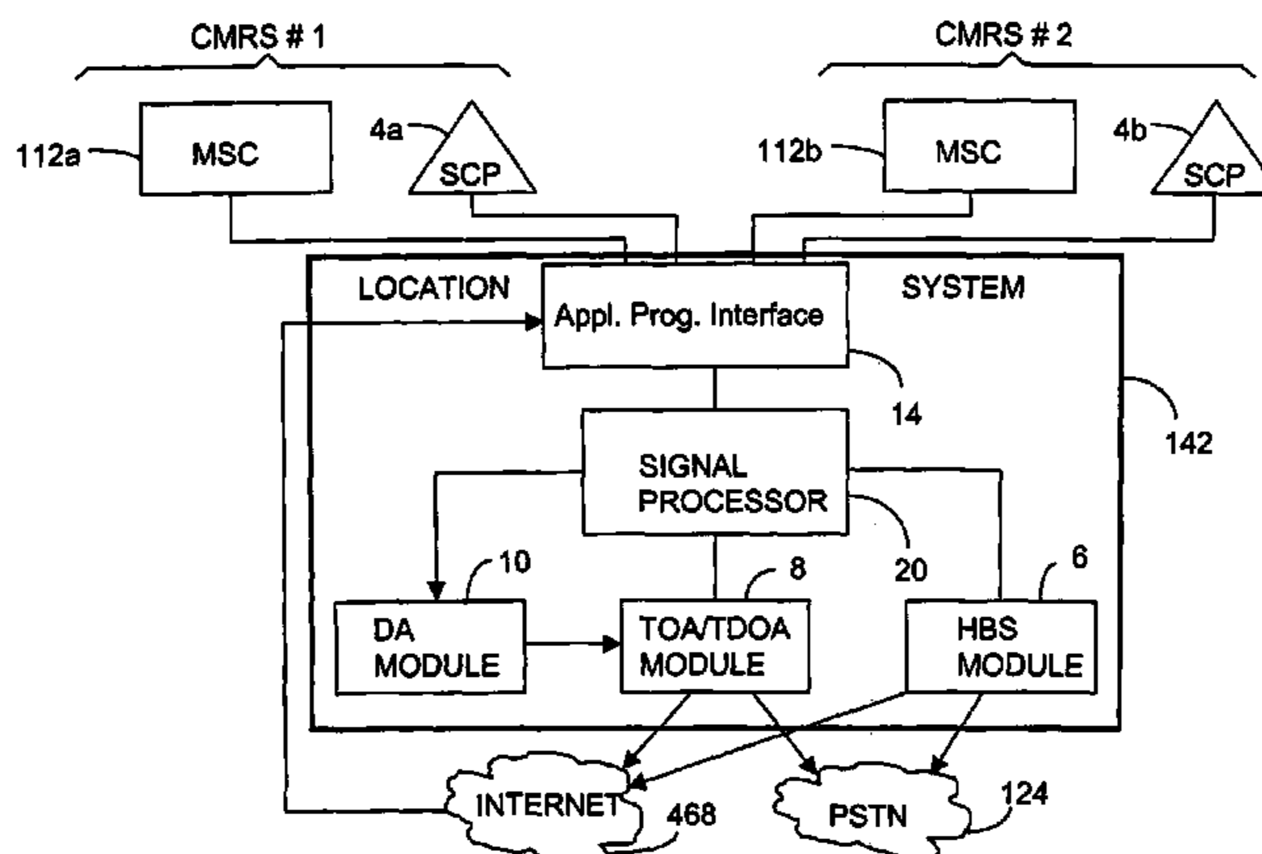
WIRELESS LOCATION USING MULTIPLE CMRSs
