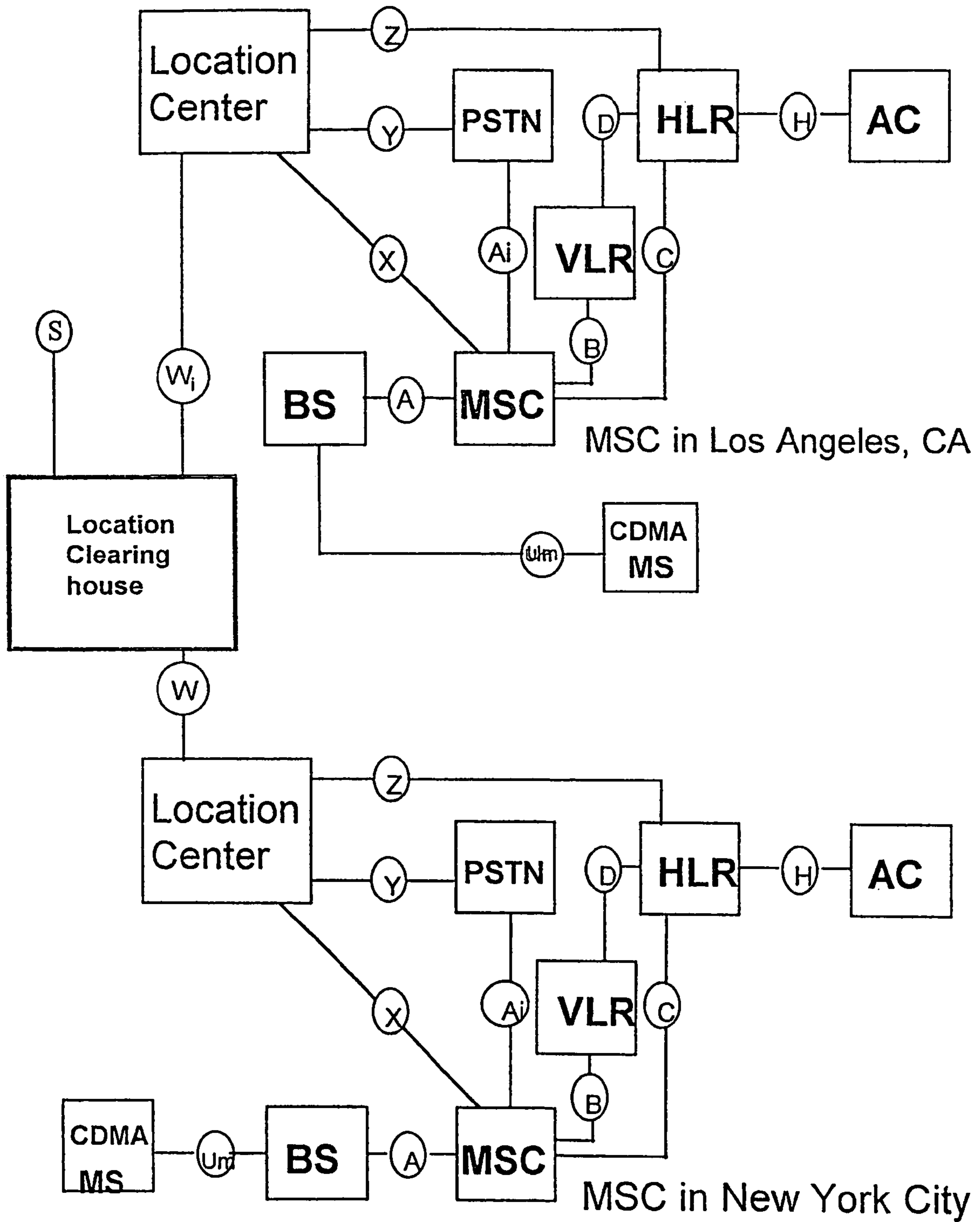
Figure 25: National Location Clearinghouse Structure
