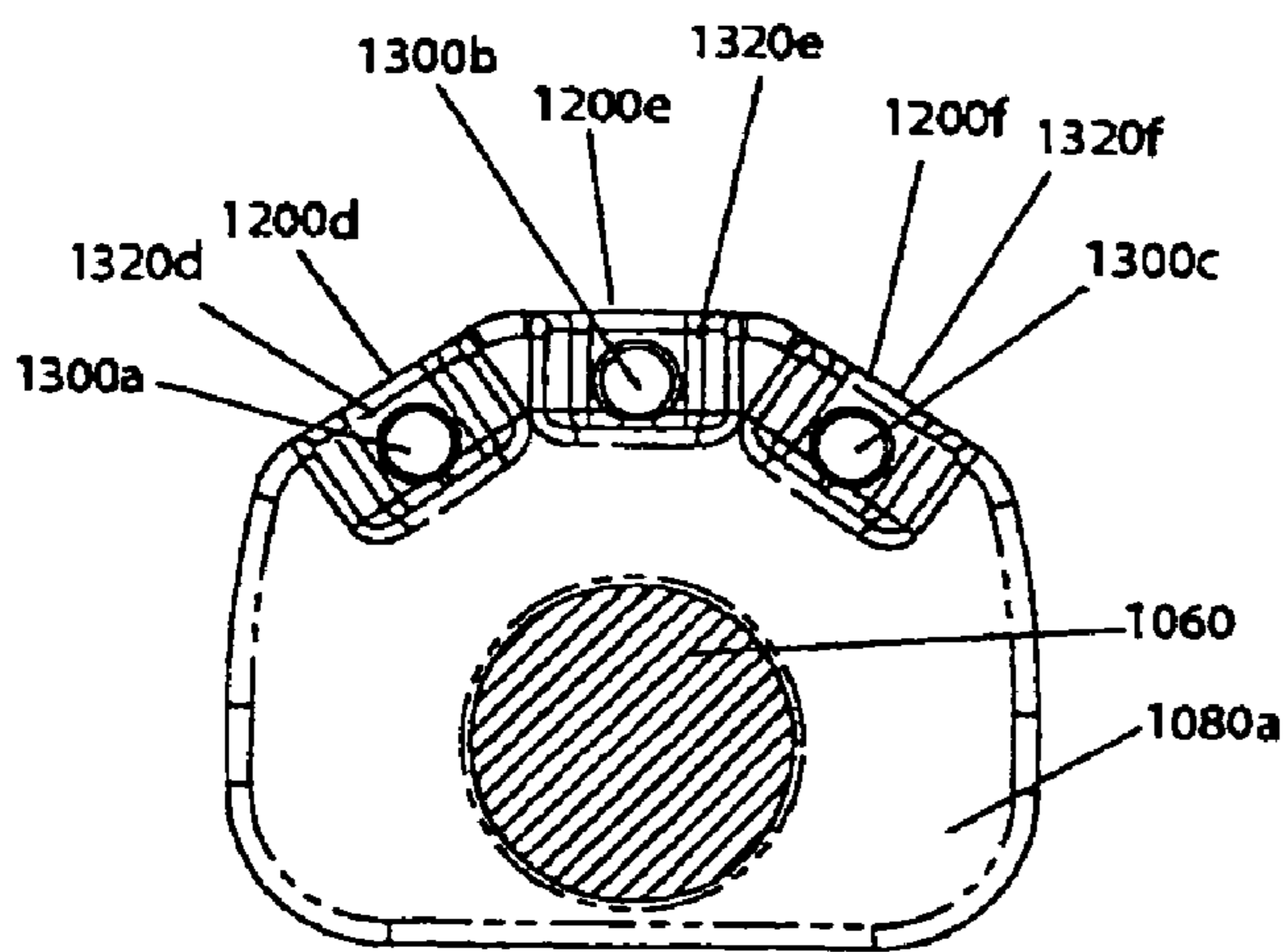
Fig. 11 (Section A-A of Fig. 7 )
