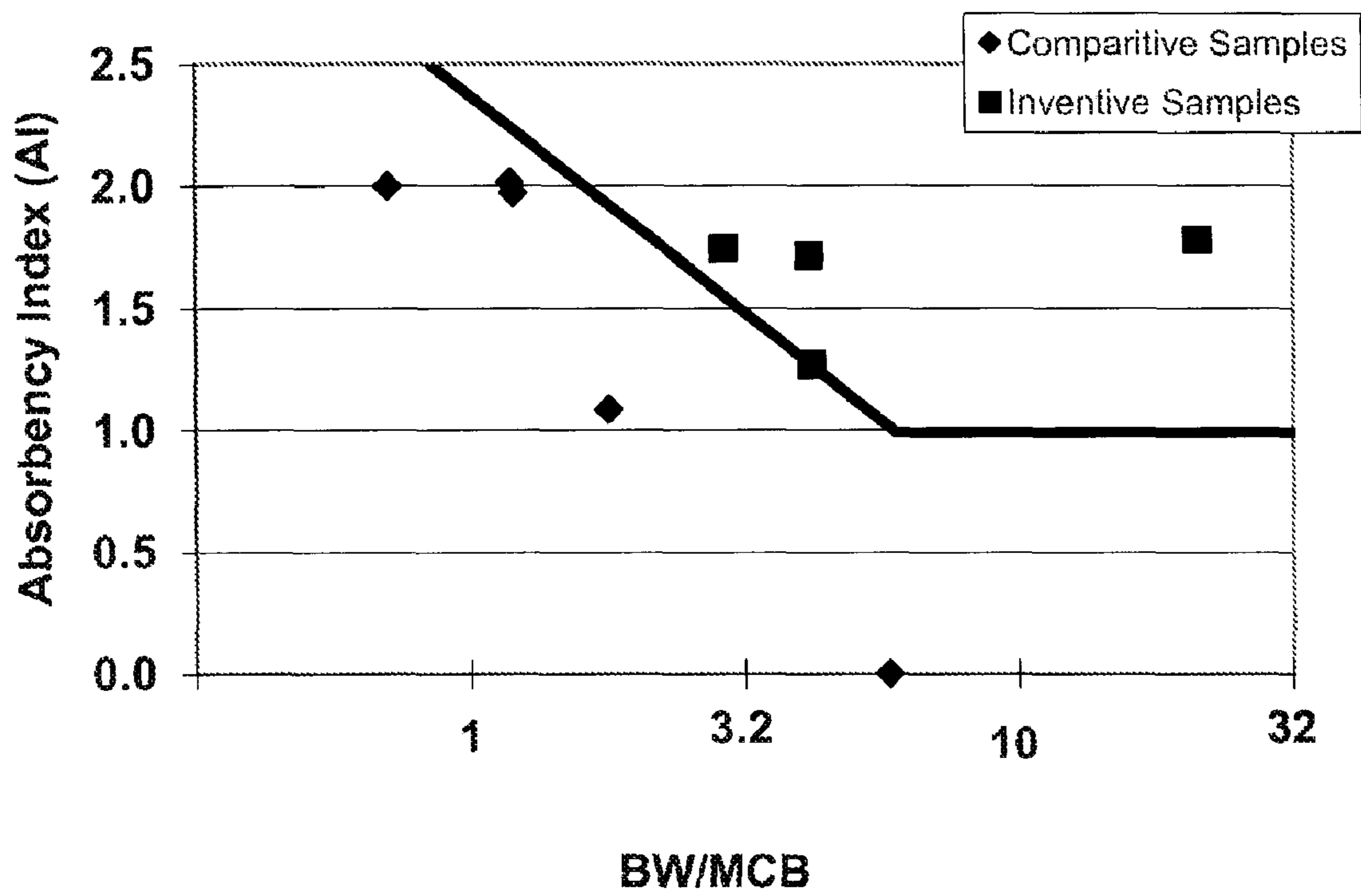
Absorbency vs Drape (thickness \leq 2.5 mm)
