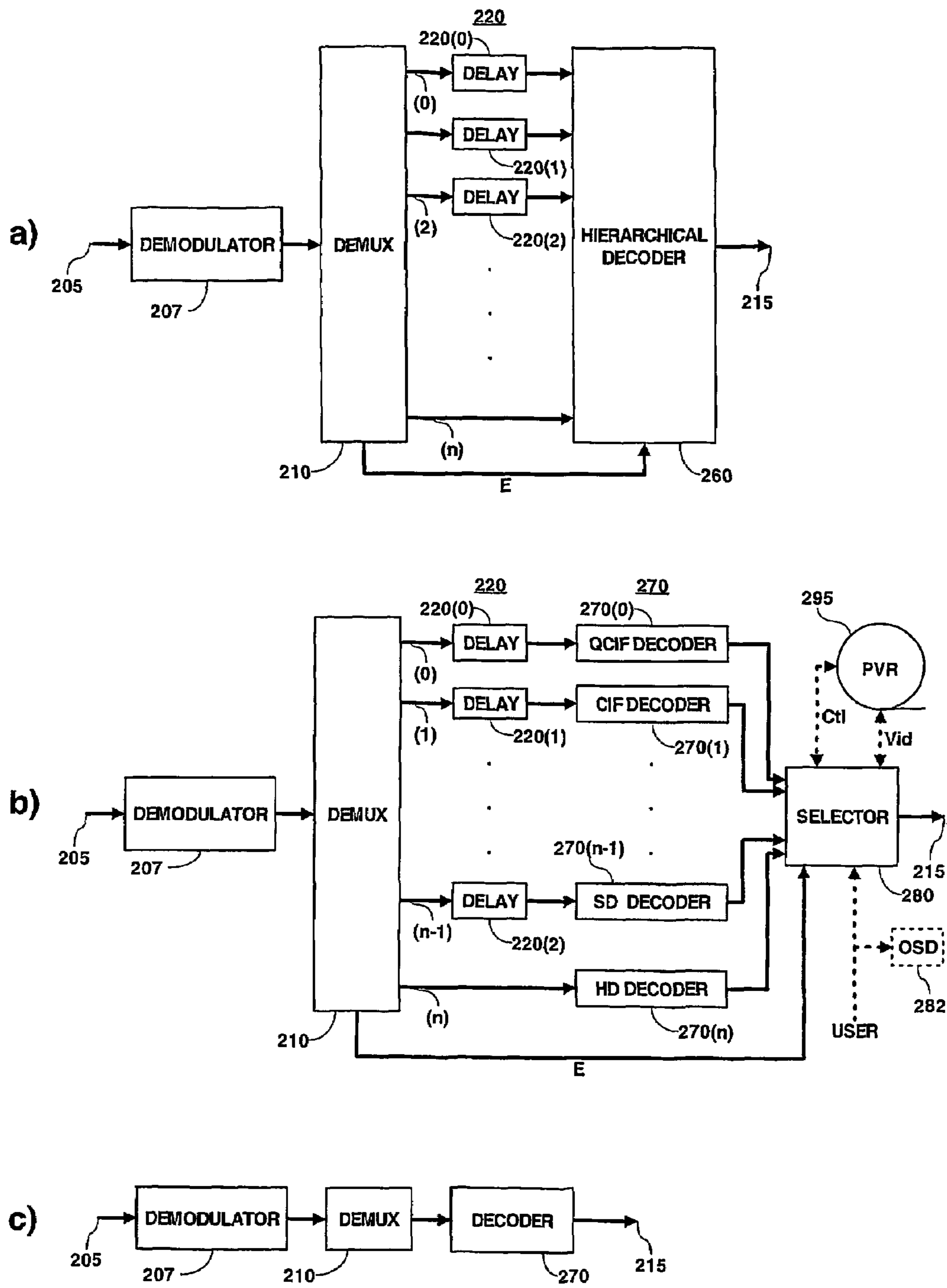
Fig. 10 Multiresolution receiver
