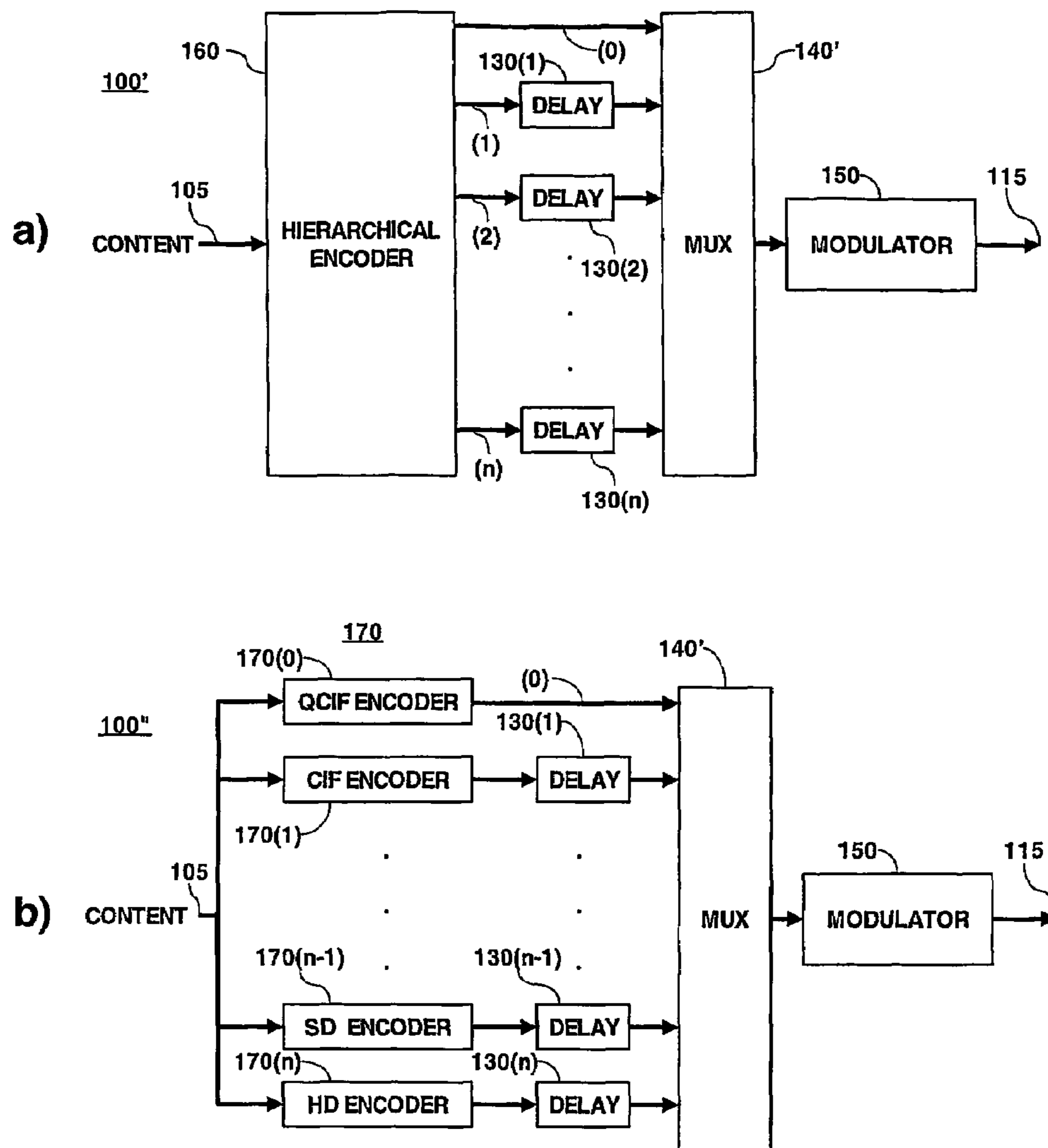
Fig. 9 Multiresolution transmitter
