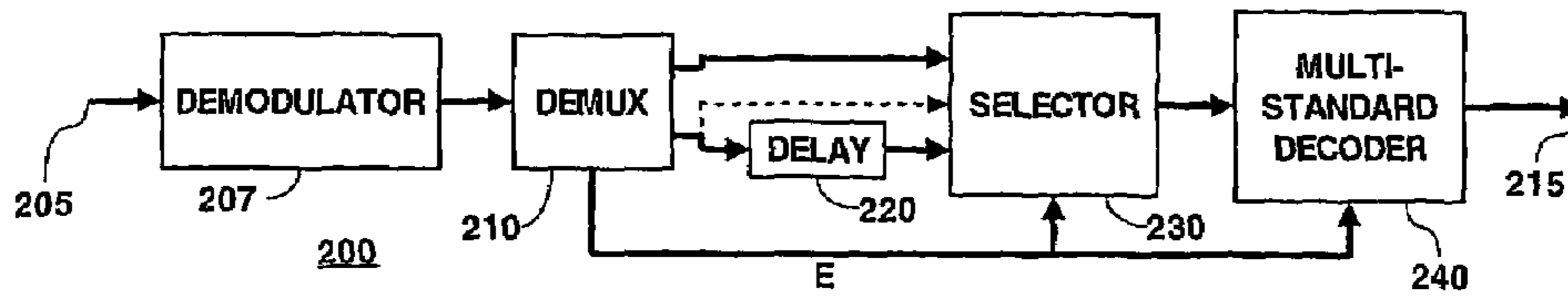
Fig. 2 Receiver
