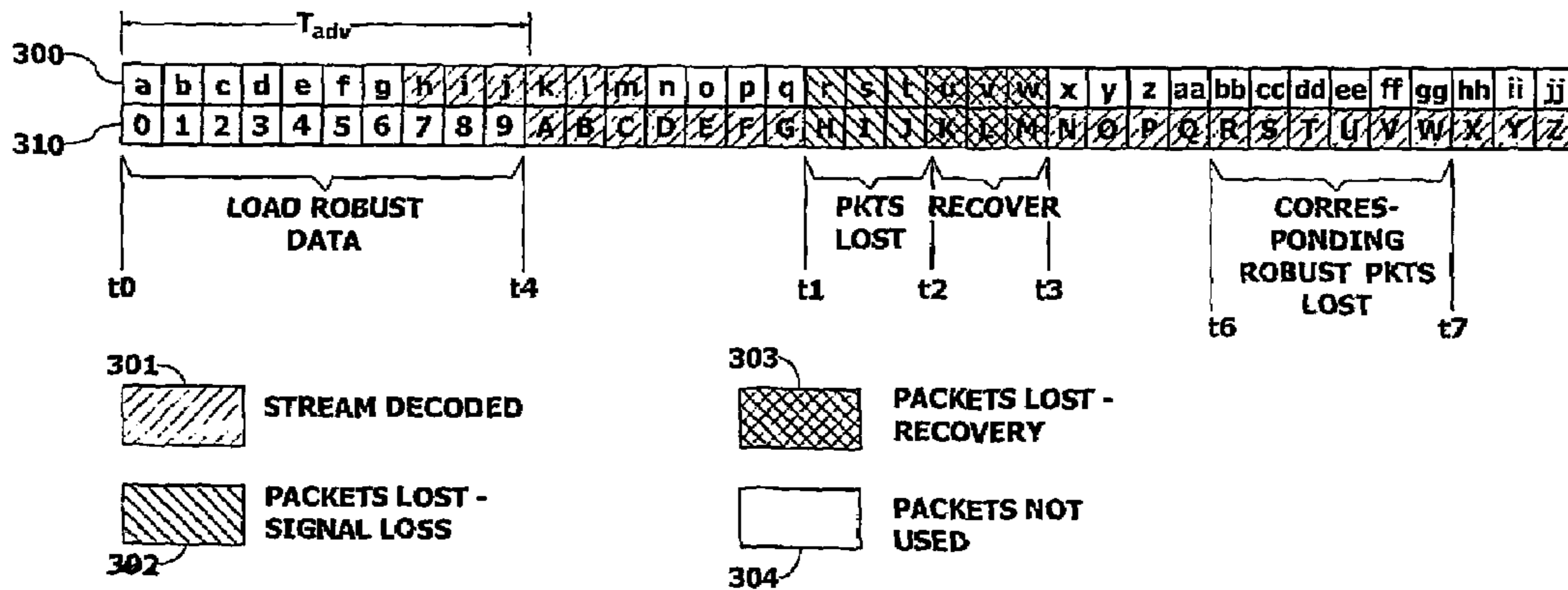
Fig. 3 Packet Streams
