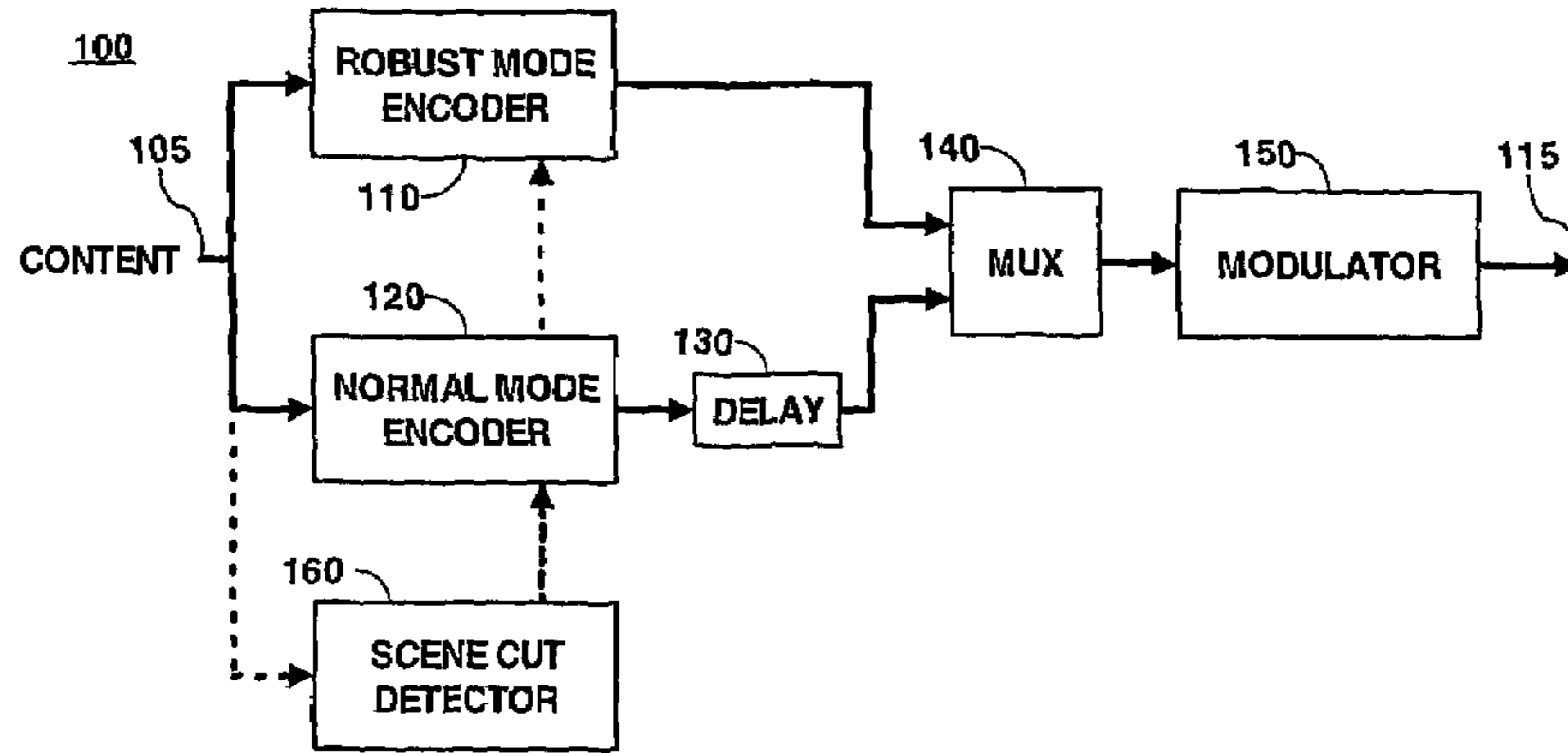
Fig. 1 Transmitter
