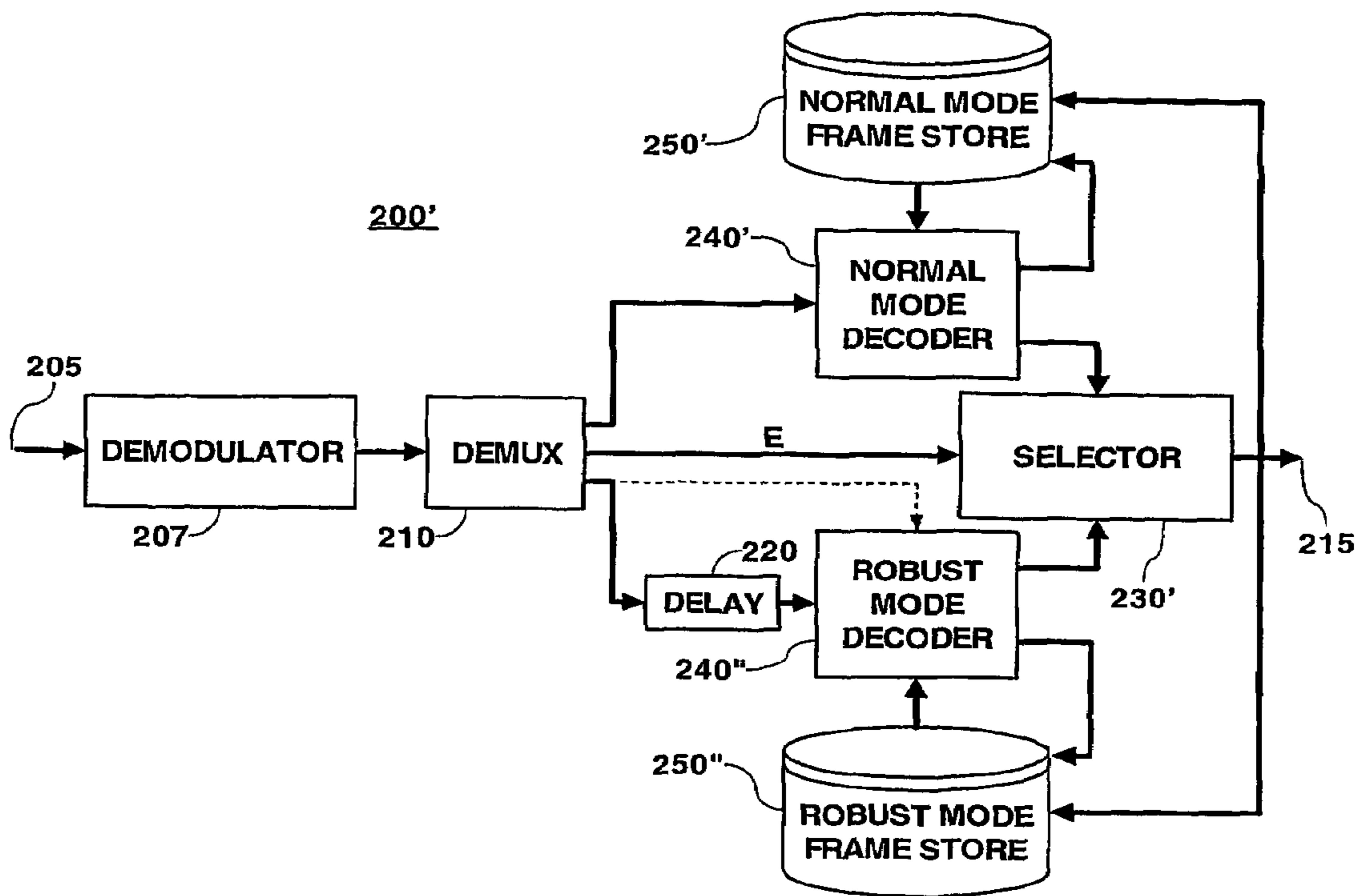
Fig. 6 Picture layer receiver
