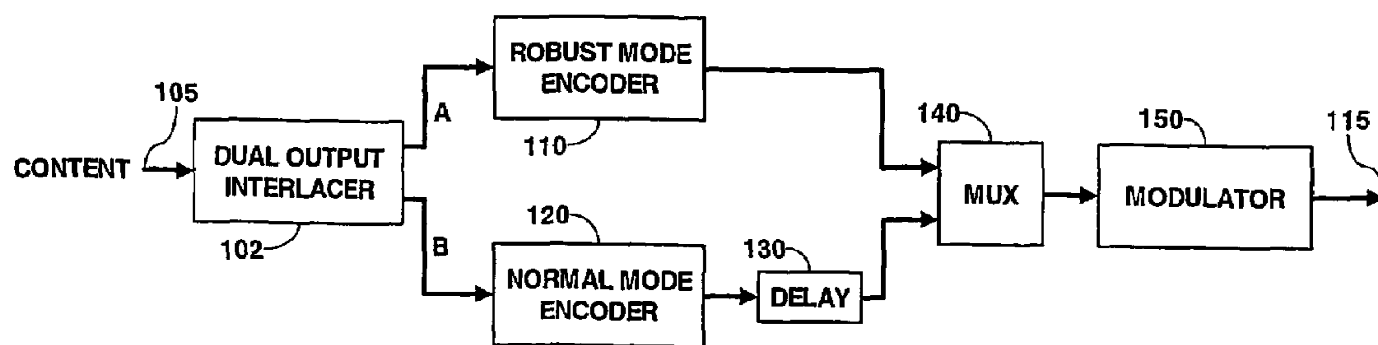
Fig. 11 Dual interlace transmitter
