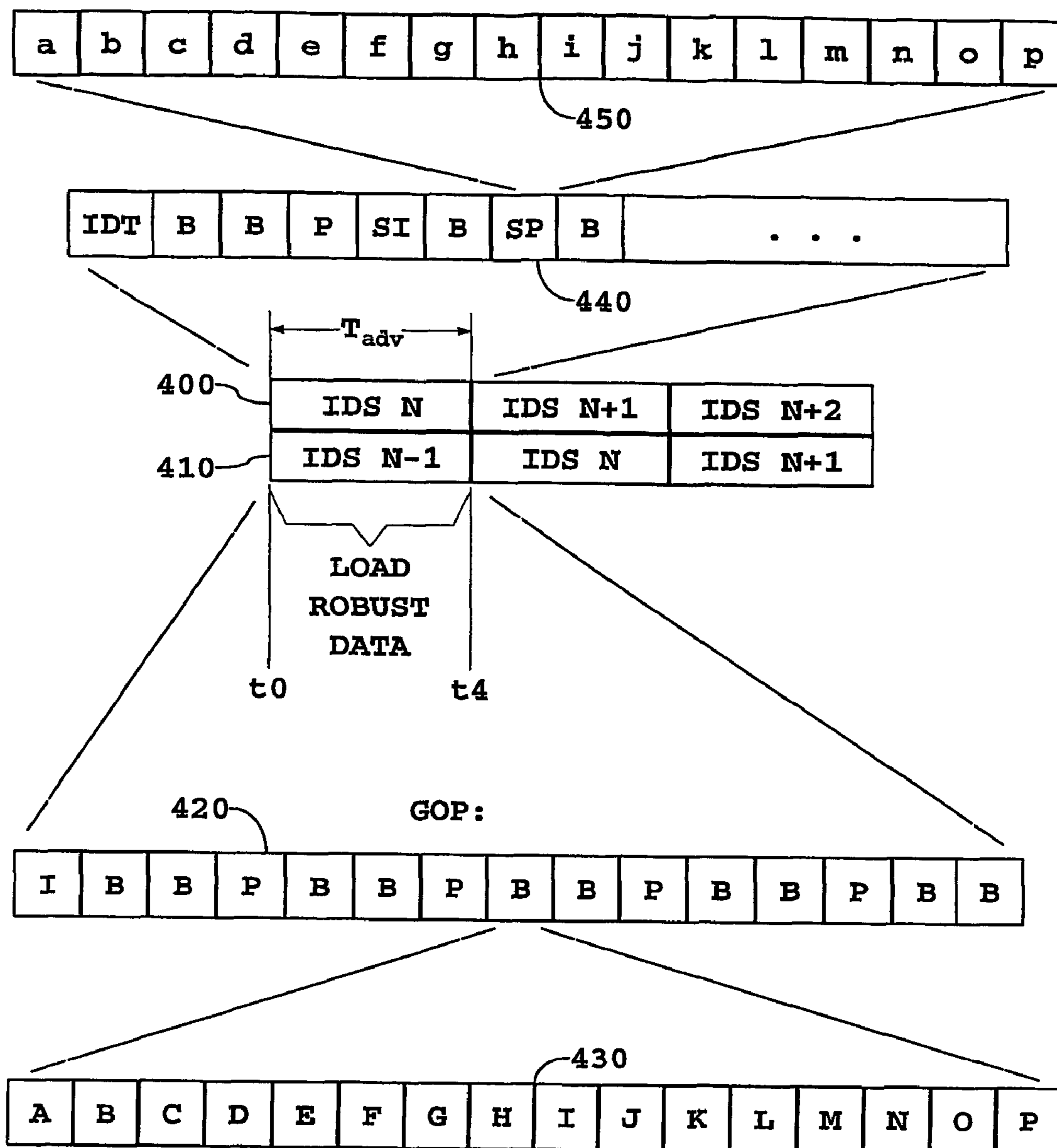
Fig. 4 GOP Streams
