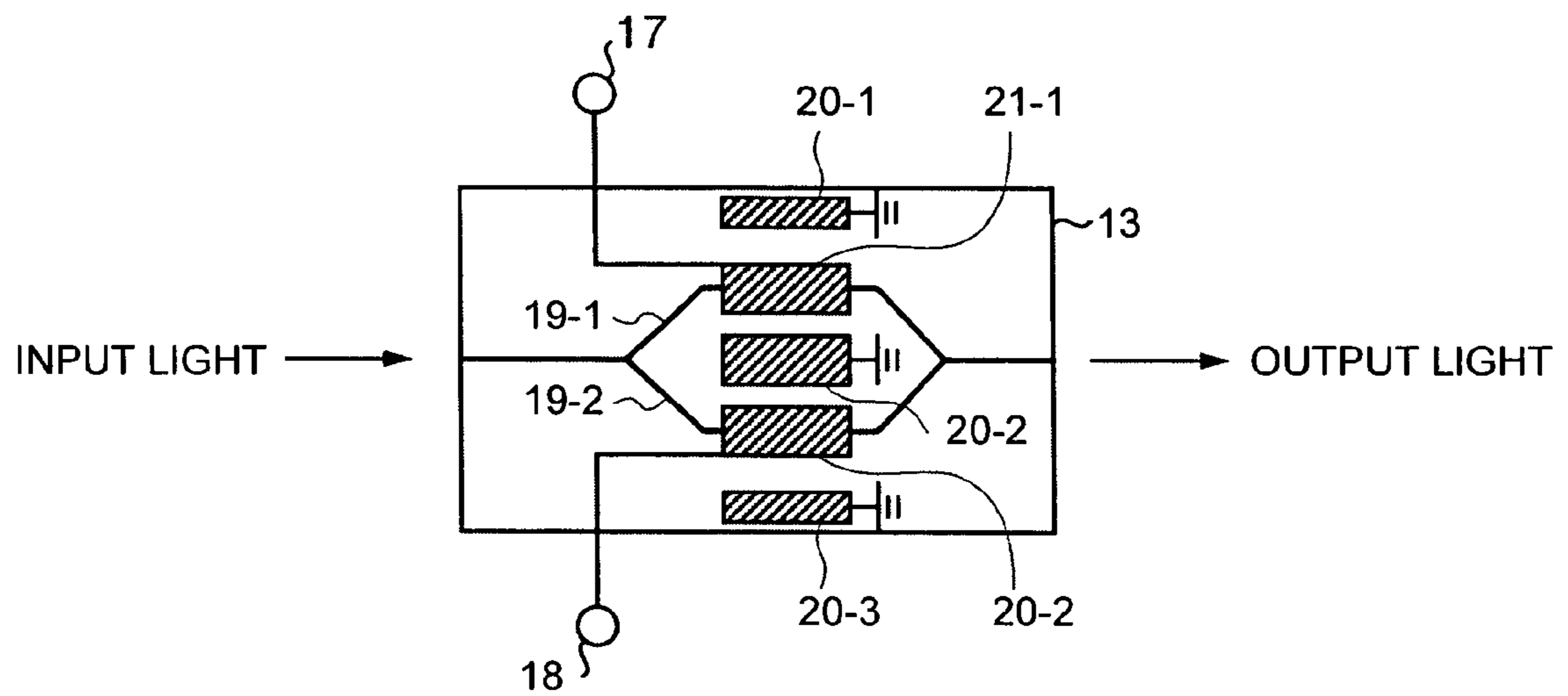
EXAMPLE OF MACH-ZEHNDER INTERFEROMETER TYPE OPTICAL MODULATOR
