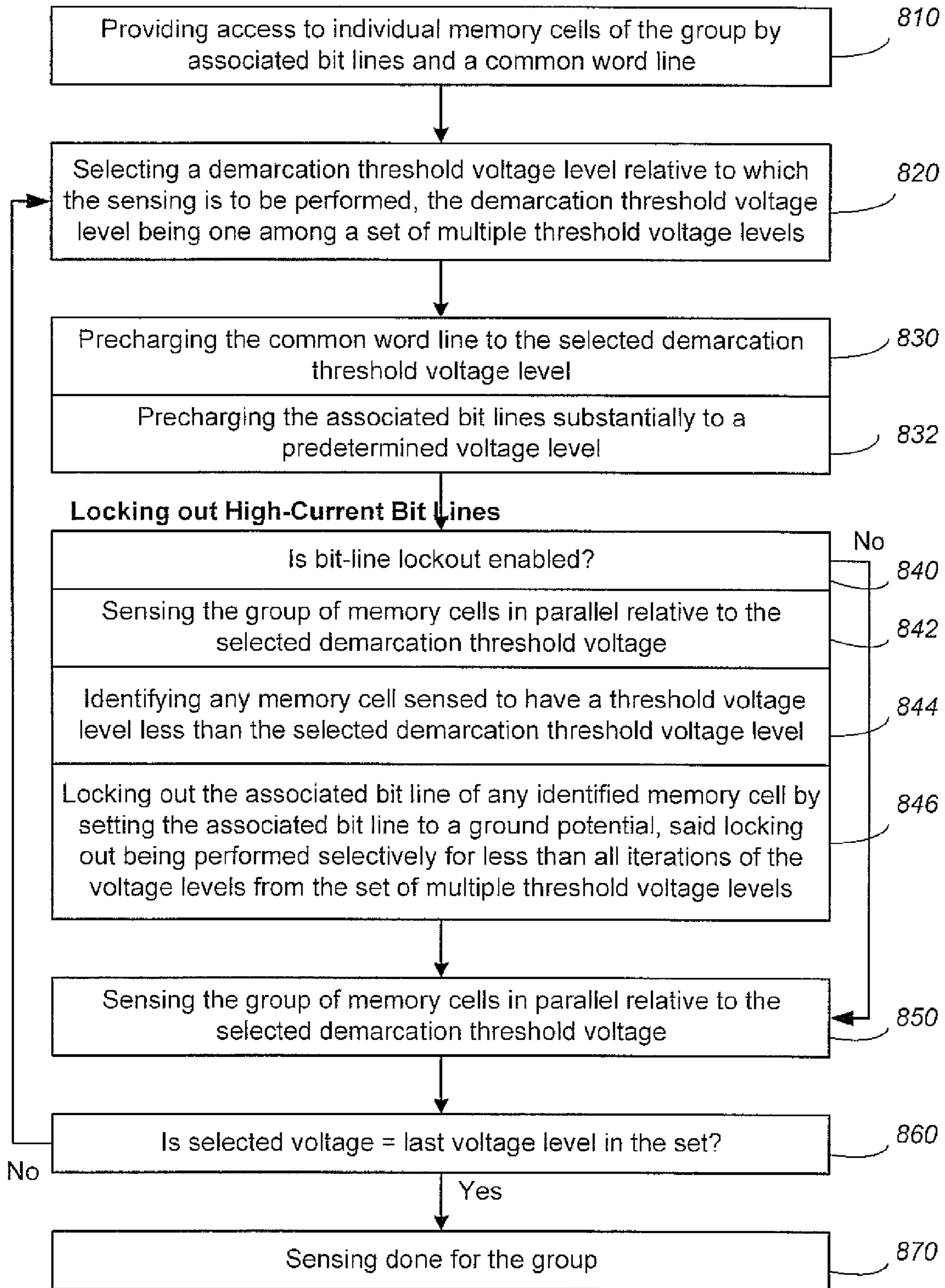
Sensing with Bit-line Lockout Control
