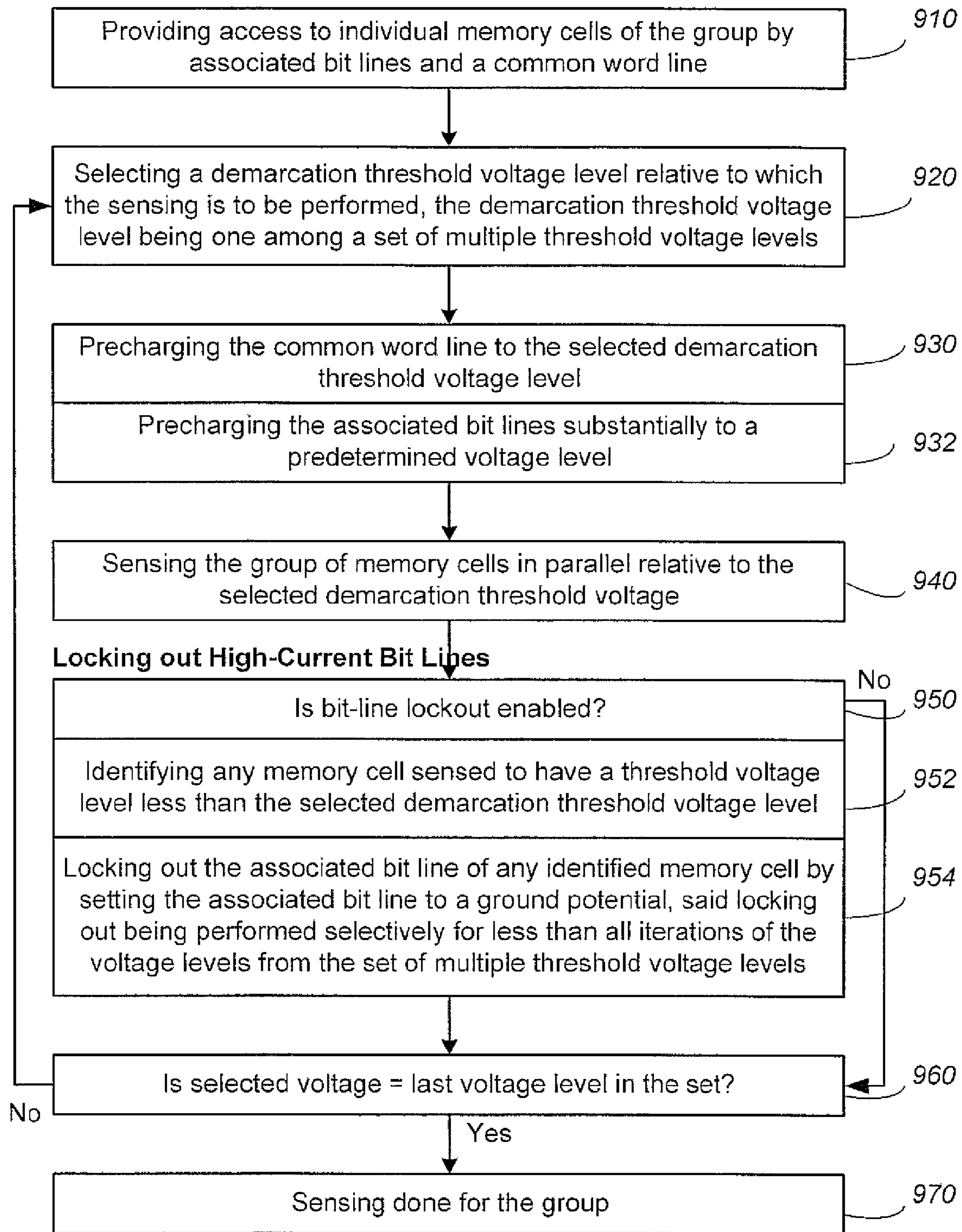
Sensing with Bit-line Lockout Control
