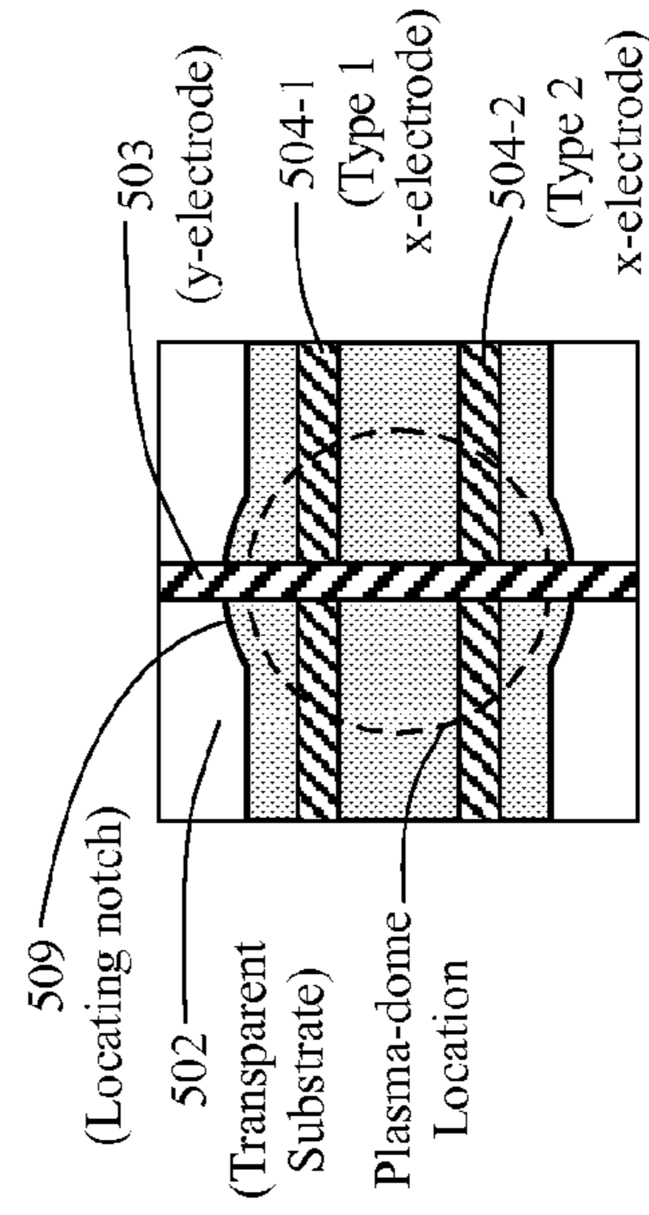
Figure 5C Top View - substrate and electrodes
