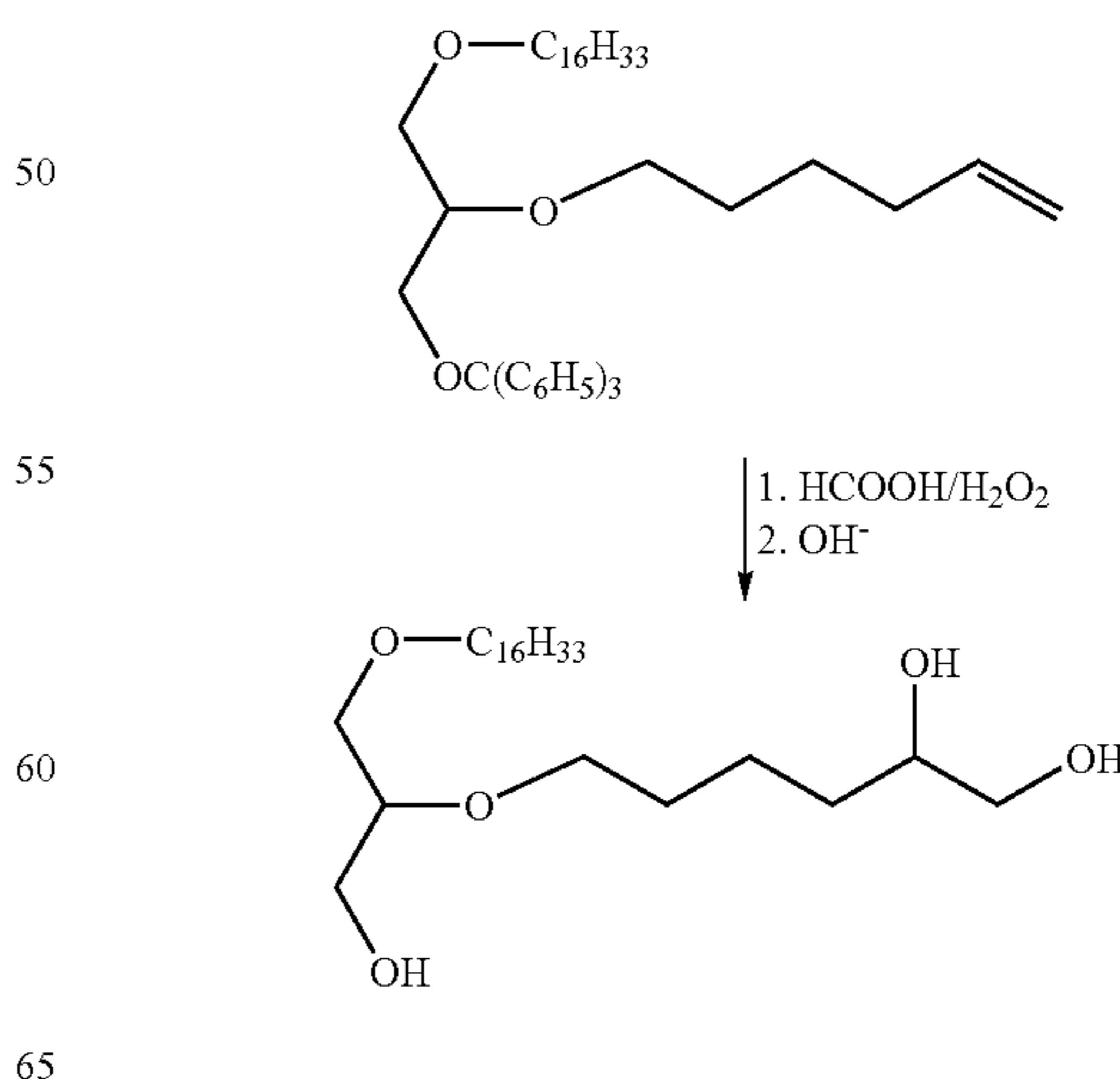
Scheme II
