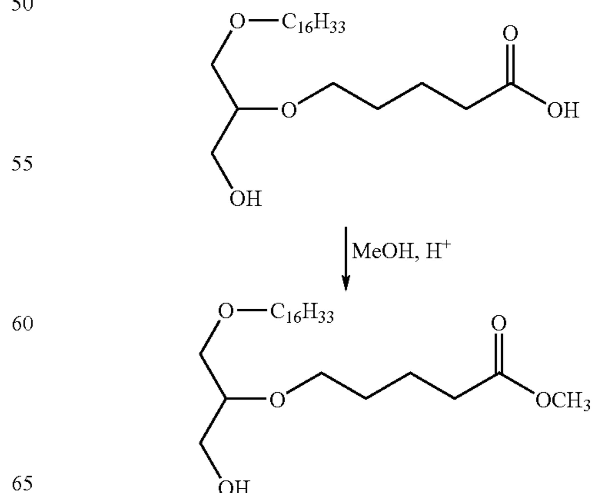
Scheme V
