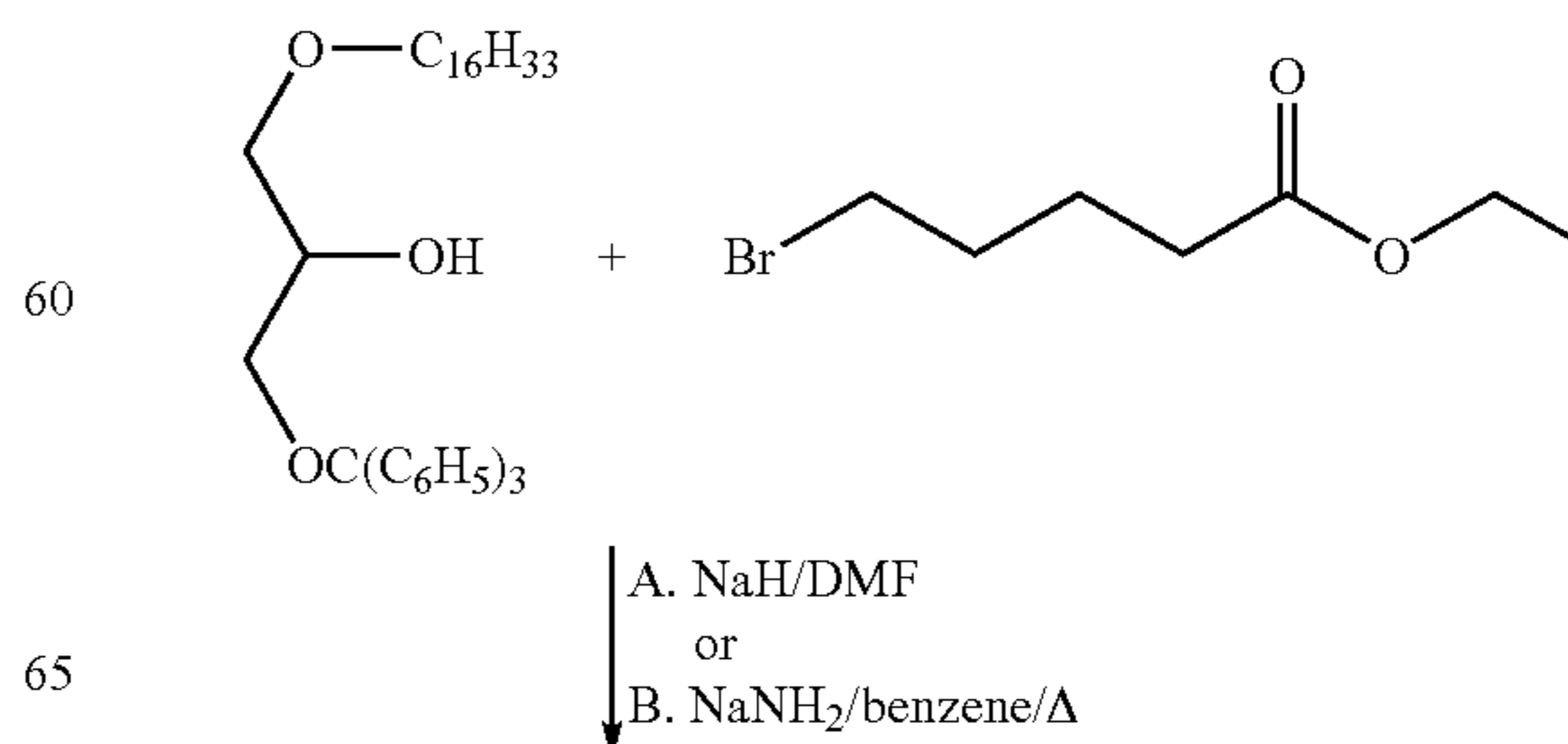
Scheme XI
