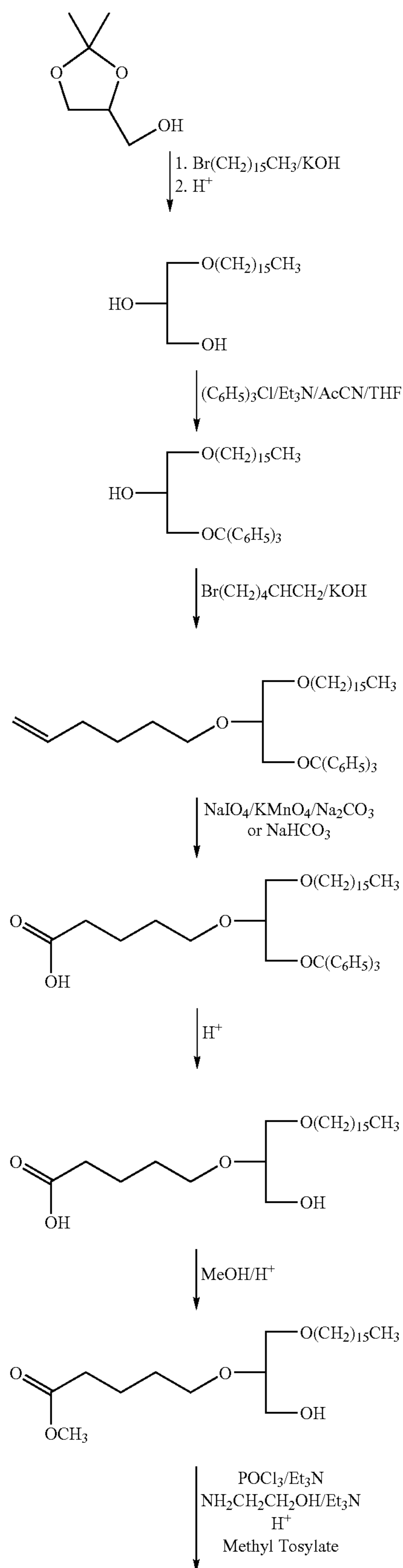
Scheme XV
