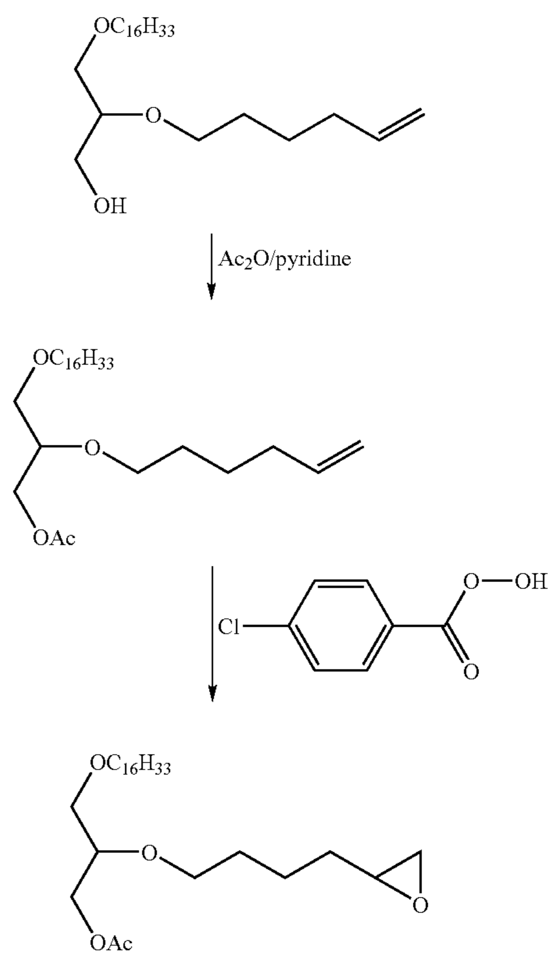
Scheme VII
