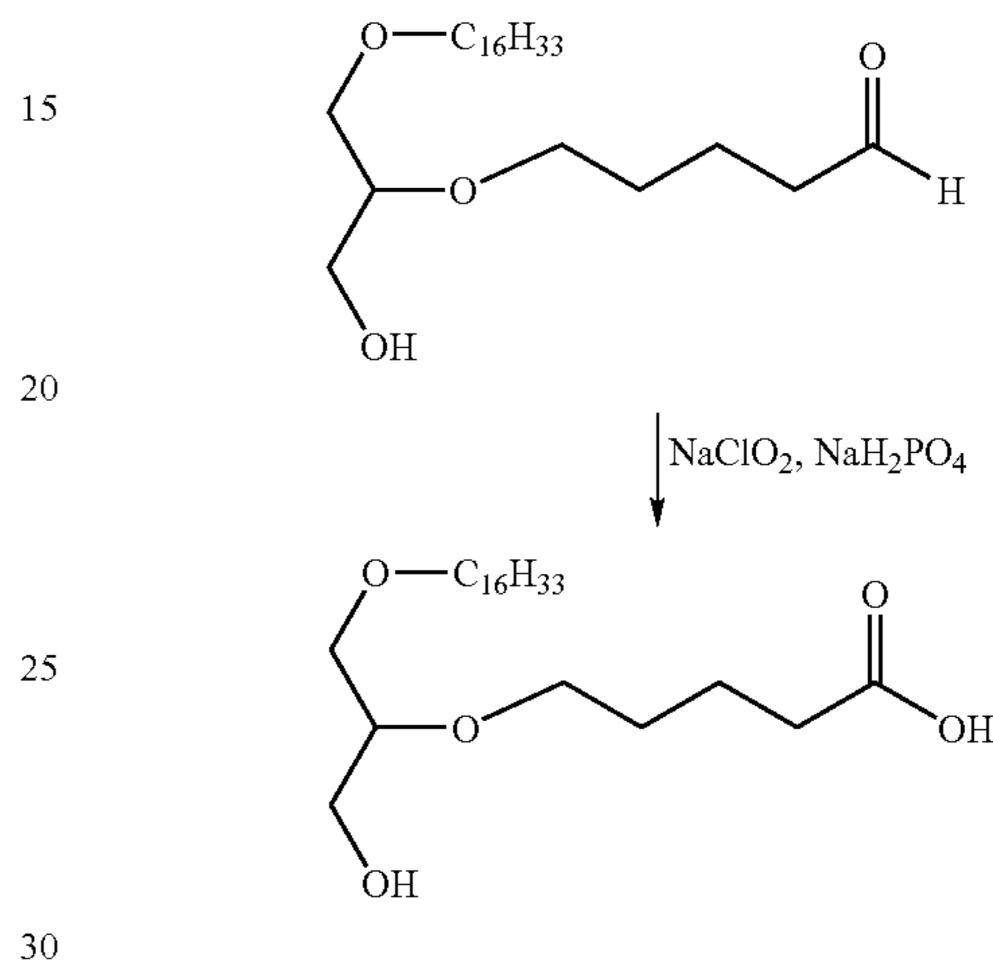
Scheme IV
