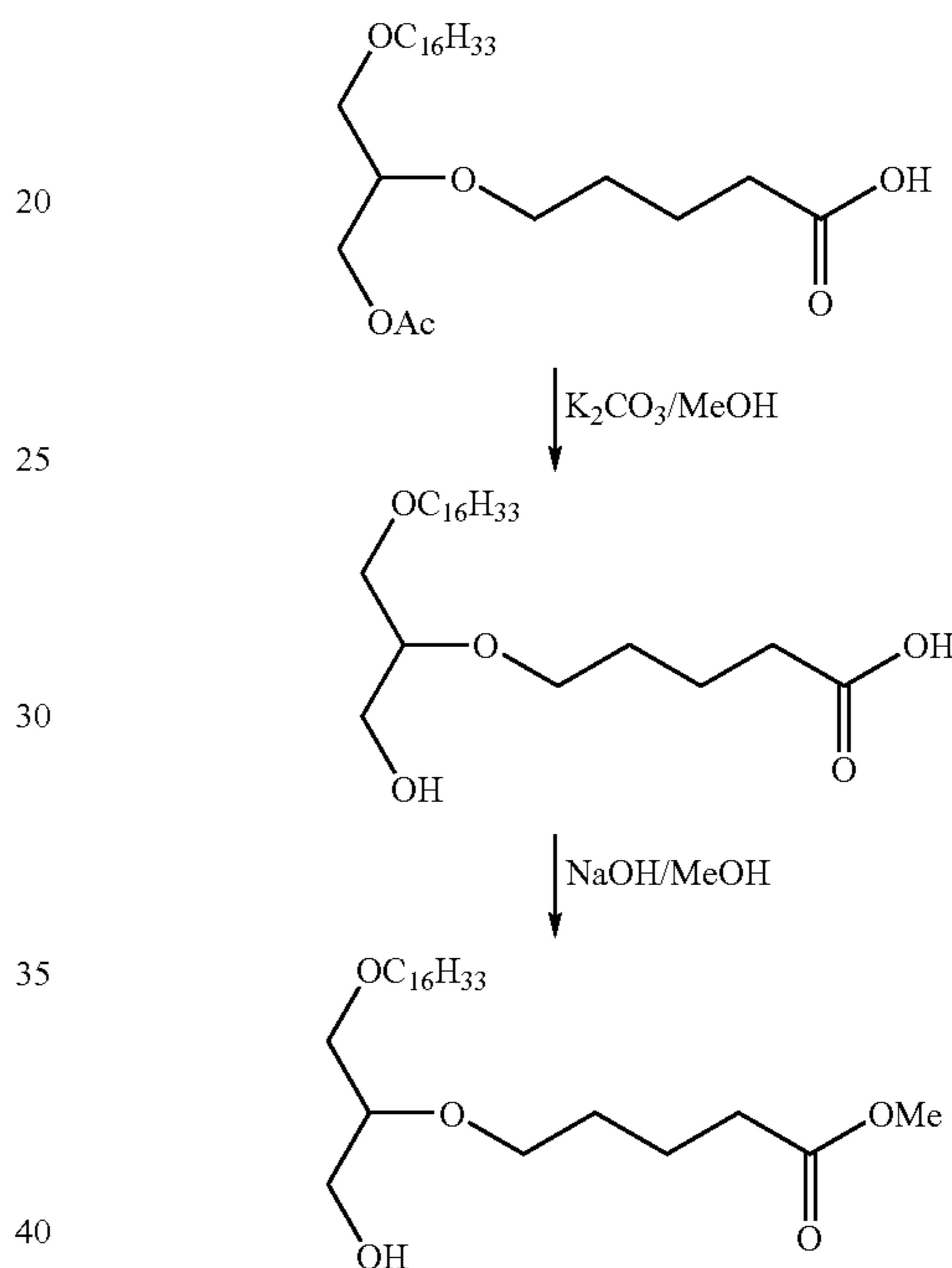
Scheme X
