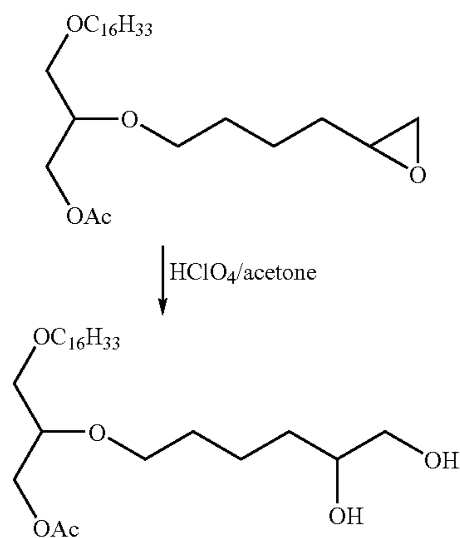
Scheme VIII
