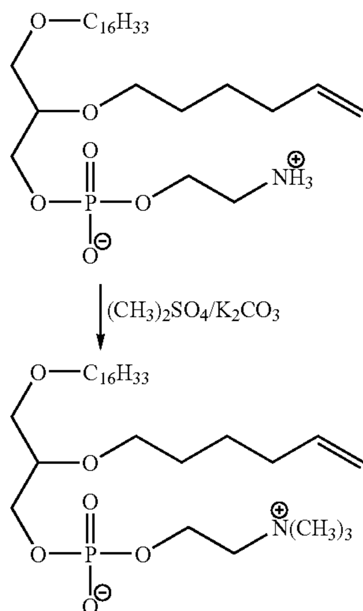
Scheme XIV
