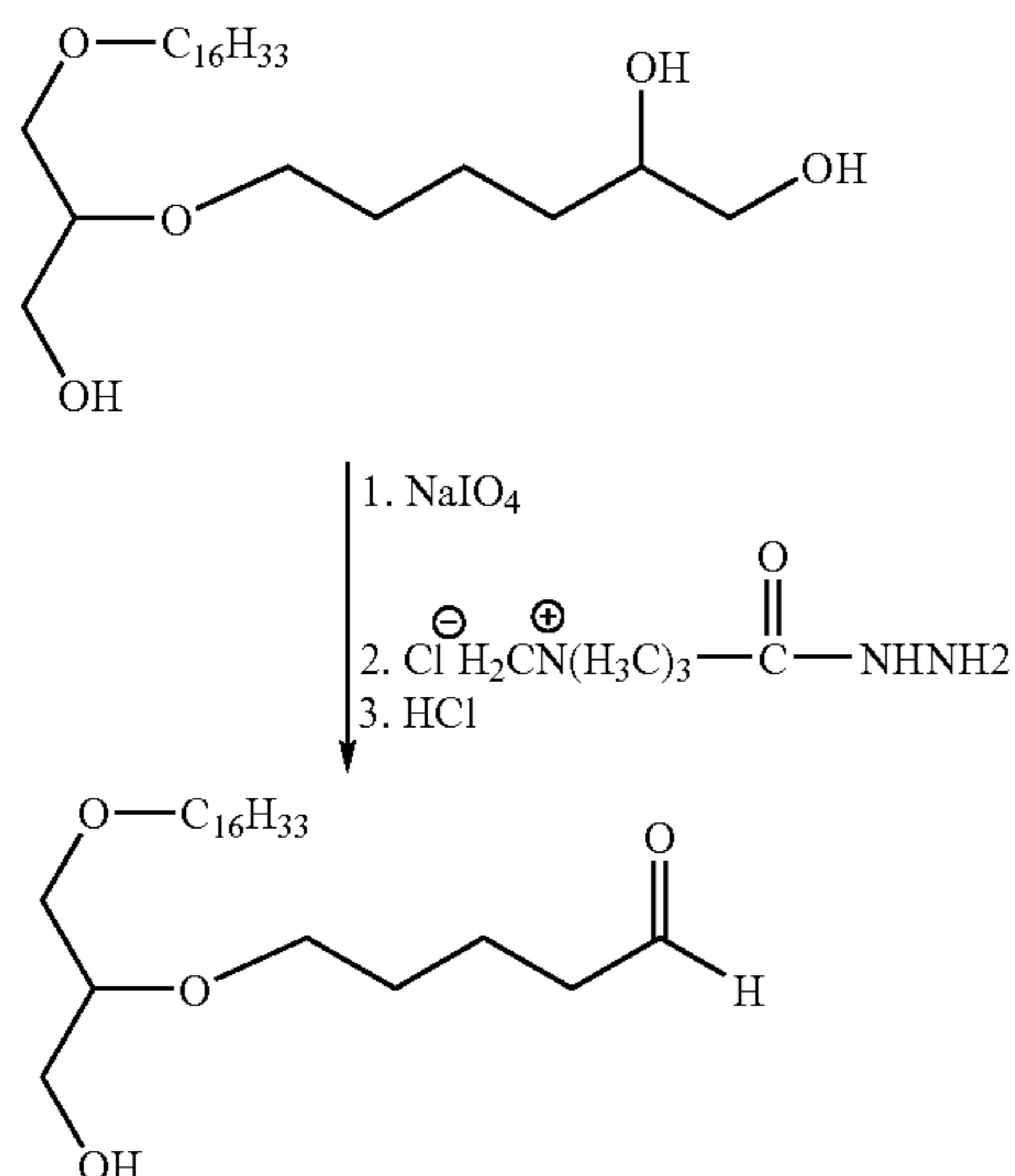
Scheme III
