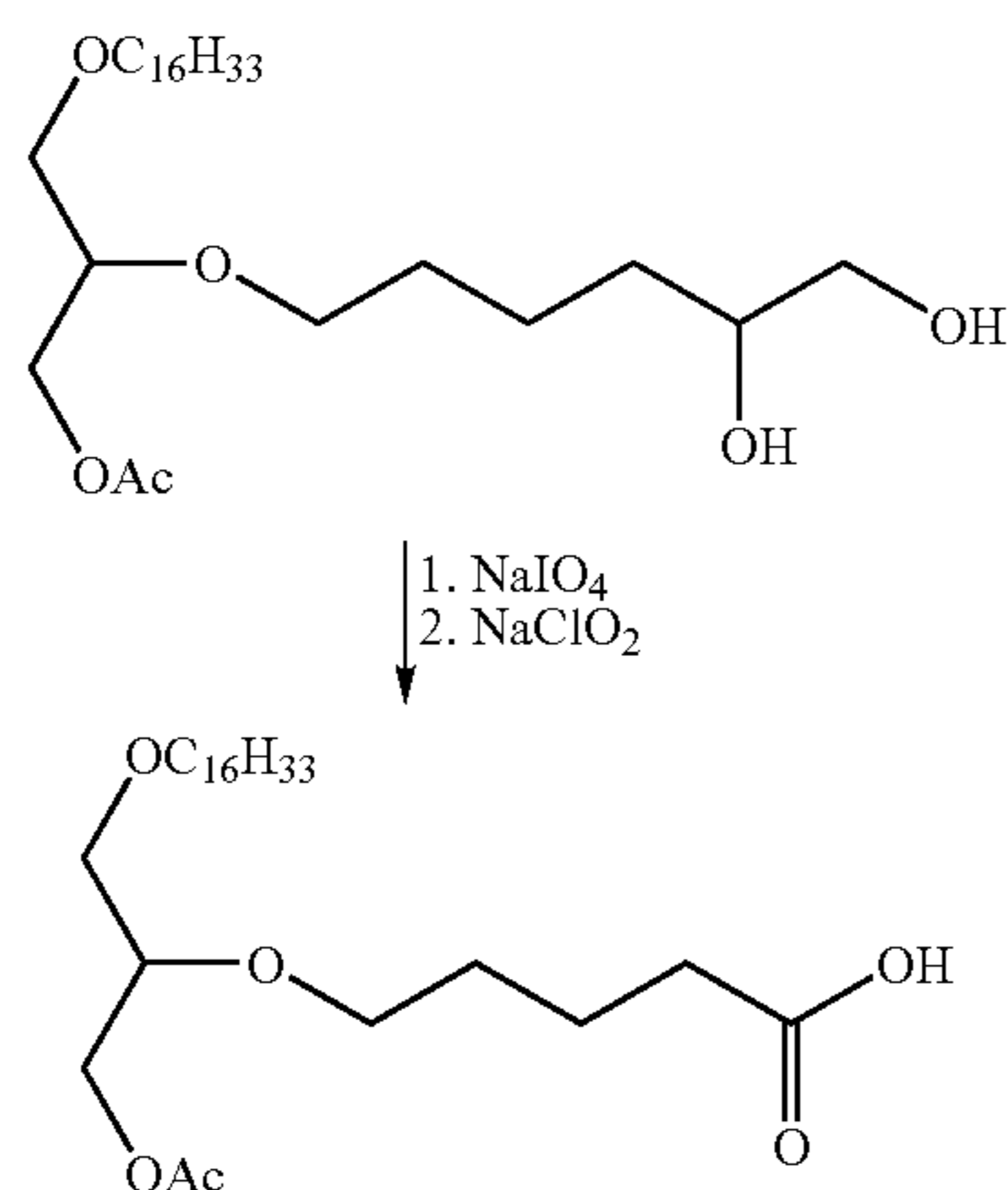
Scheme IX
