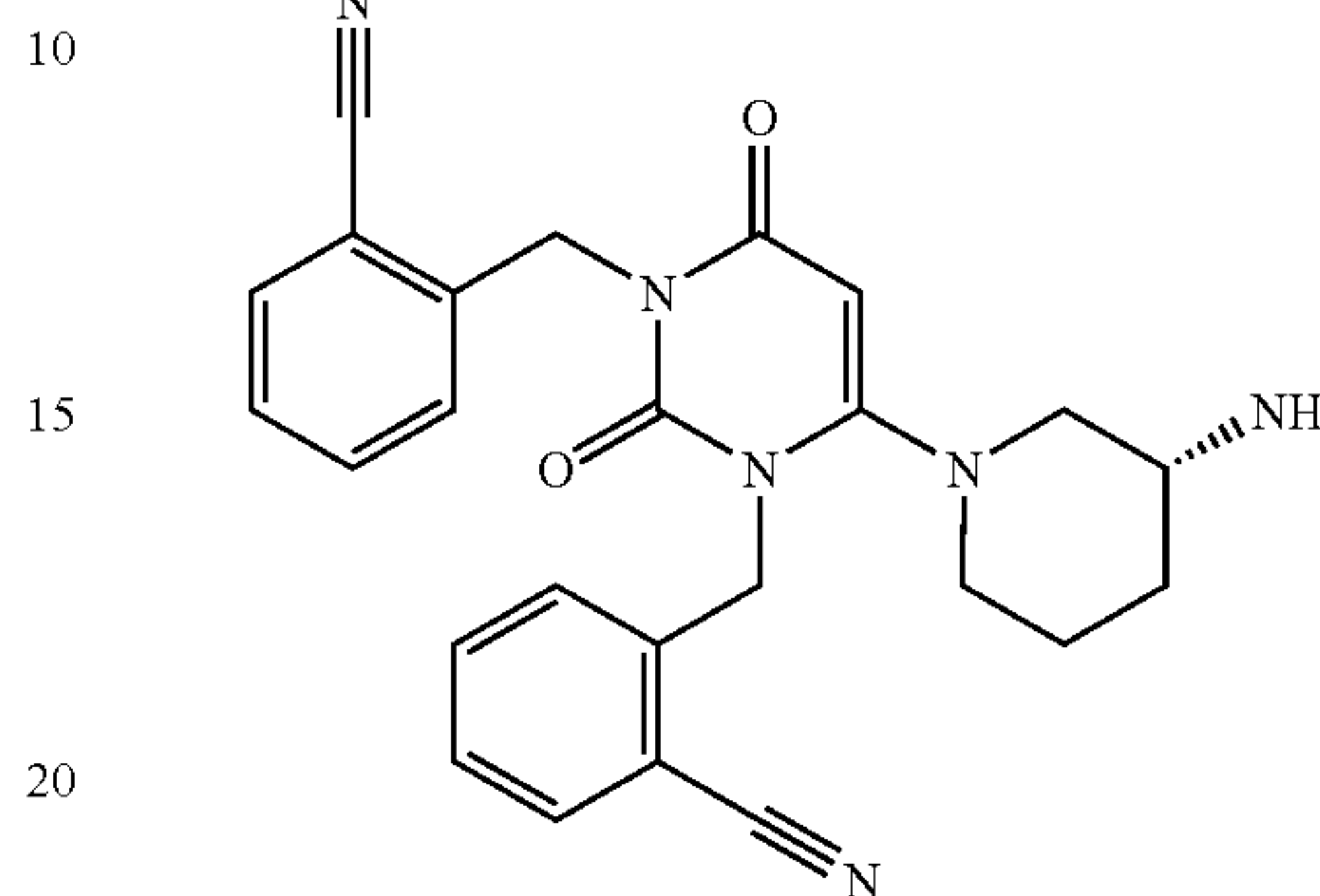
Compound 16
