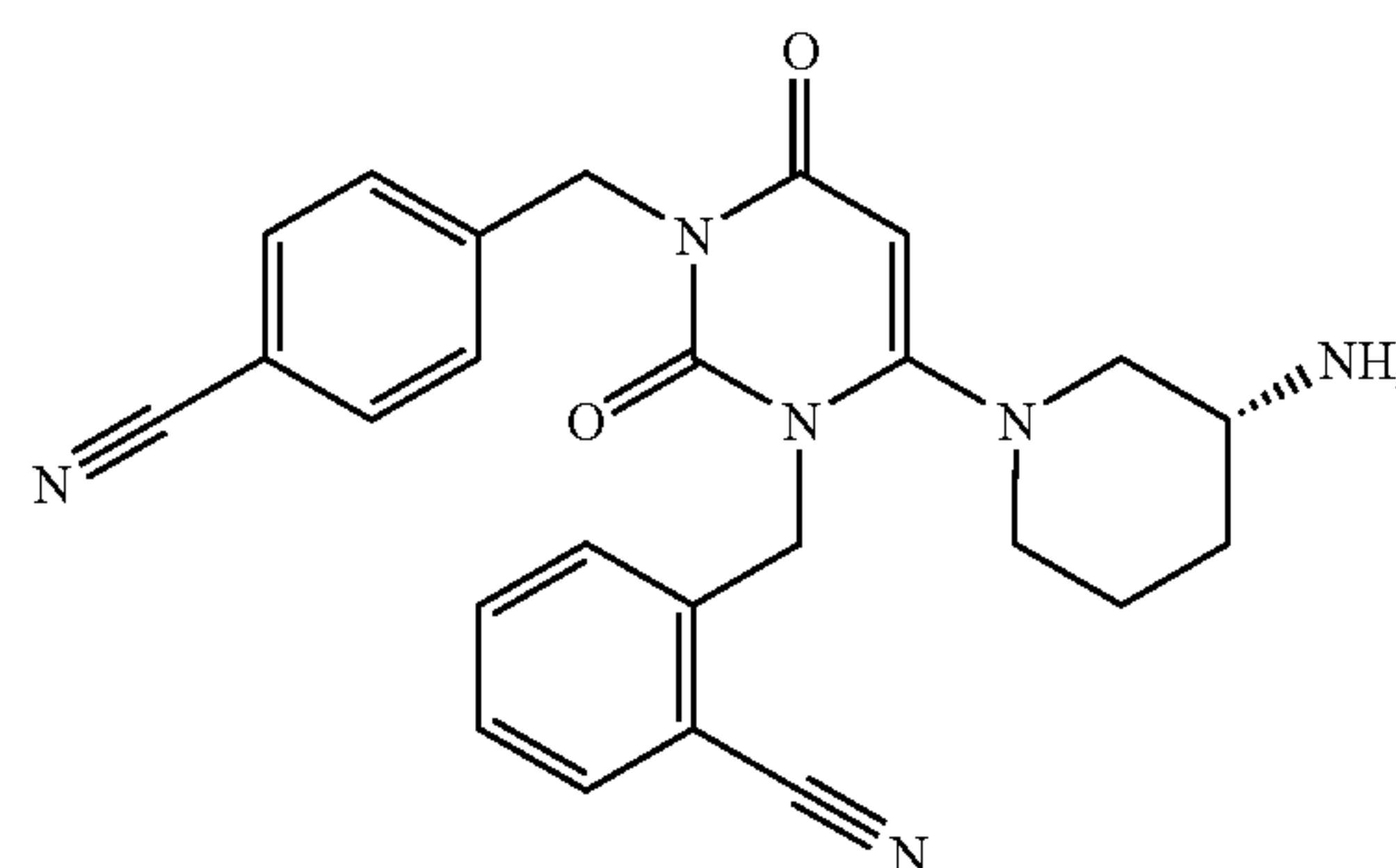
Compound 19
