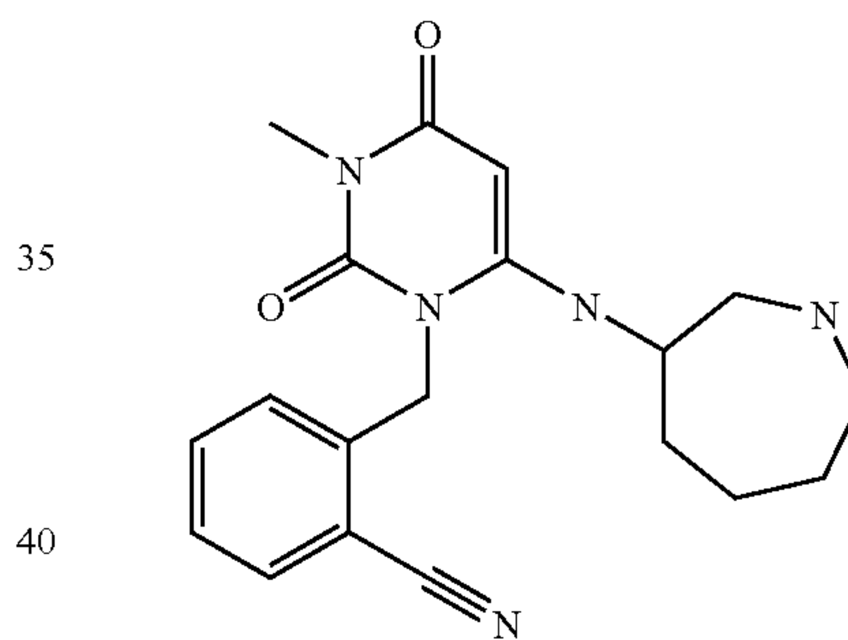
Compound 12
