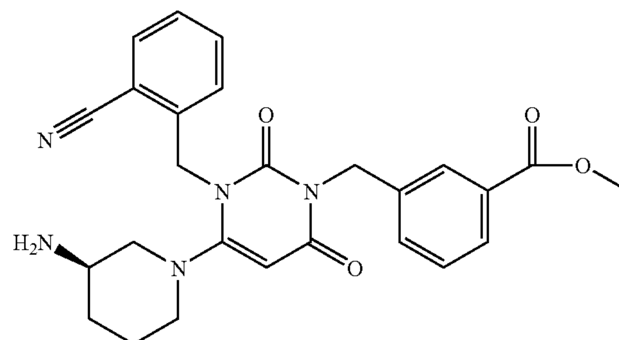
Compound 24
