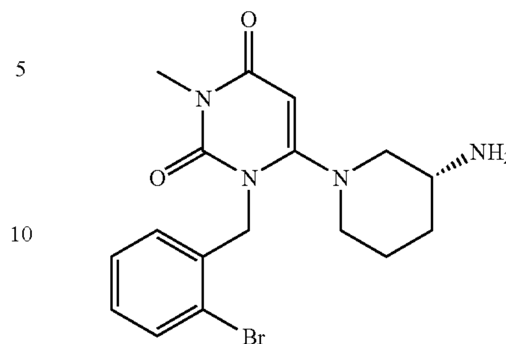
Compound 11
