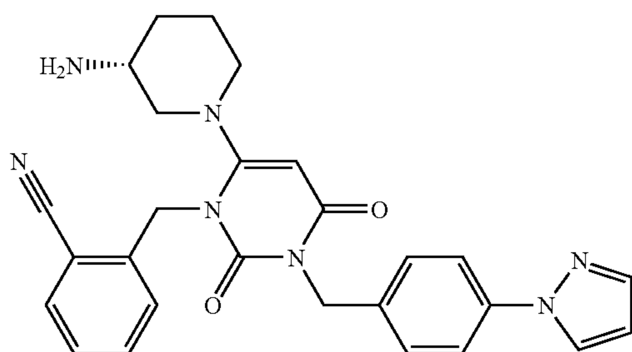
Compound 21
