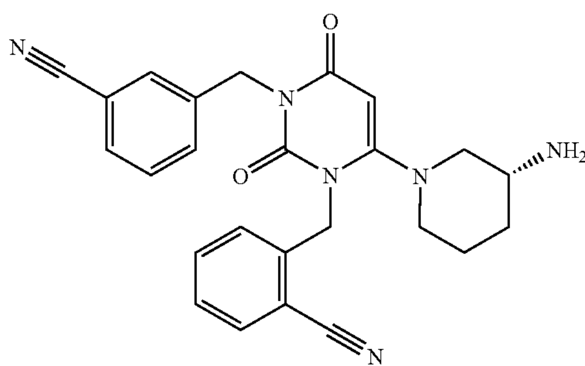
Compound 17
