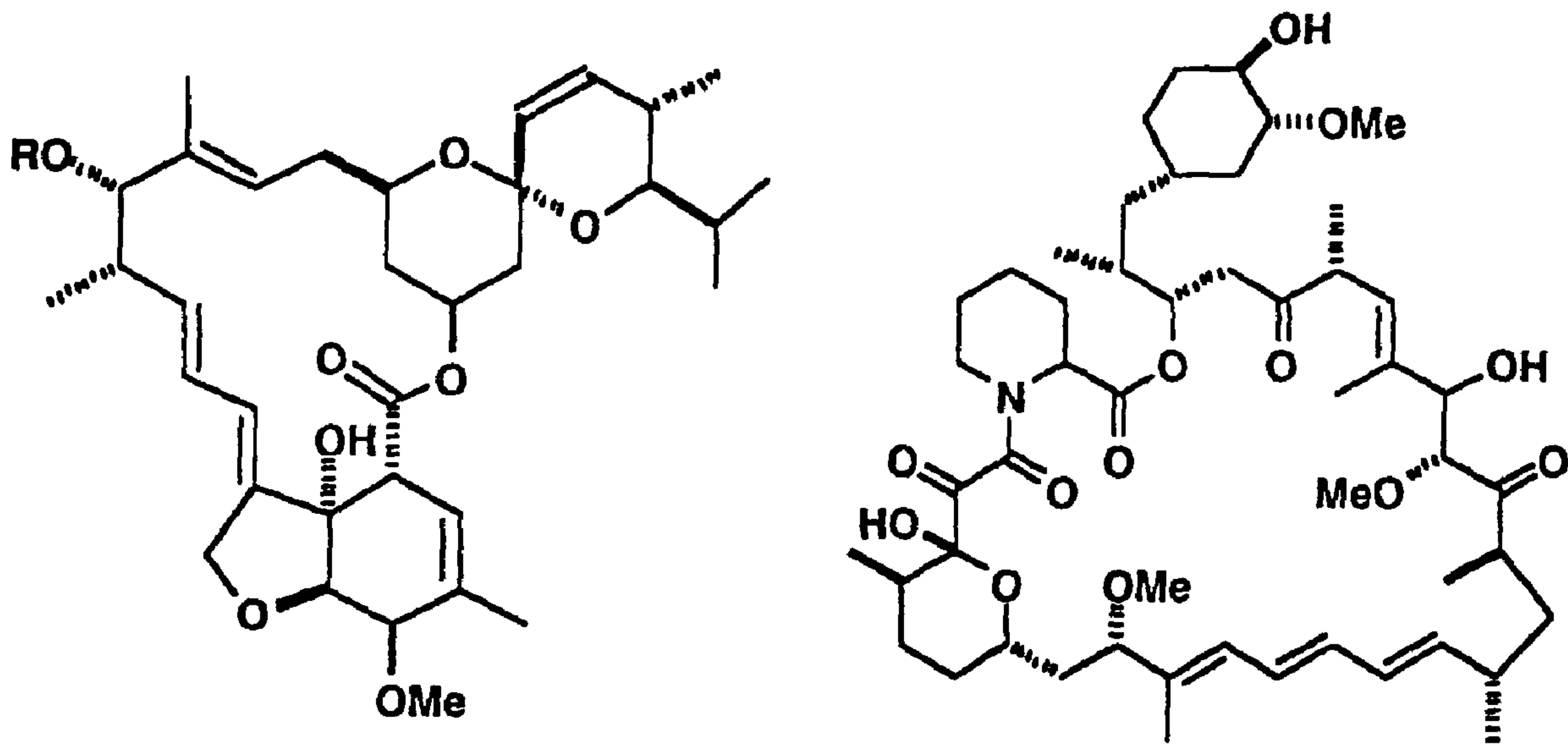
Avermectin A1b
