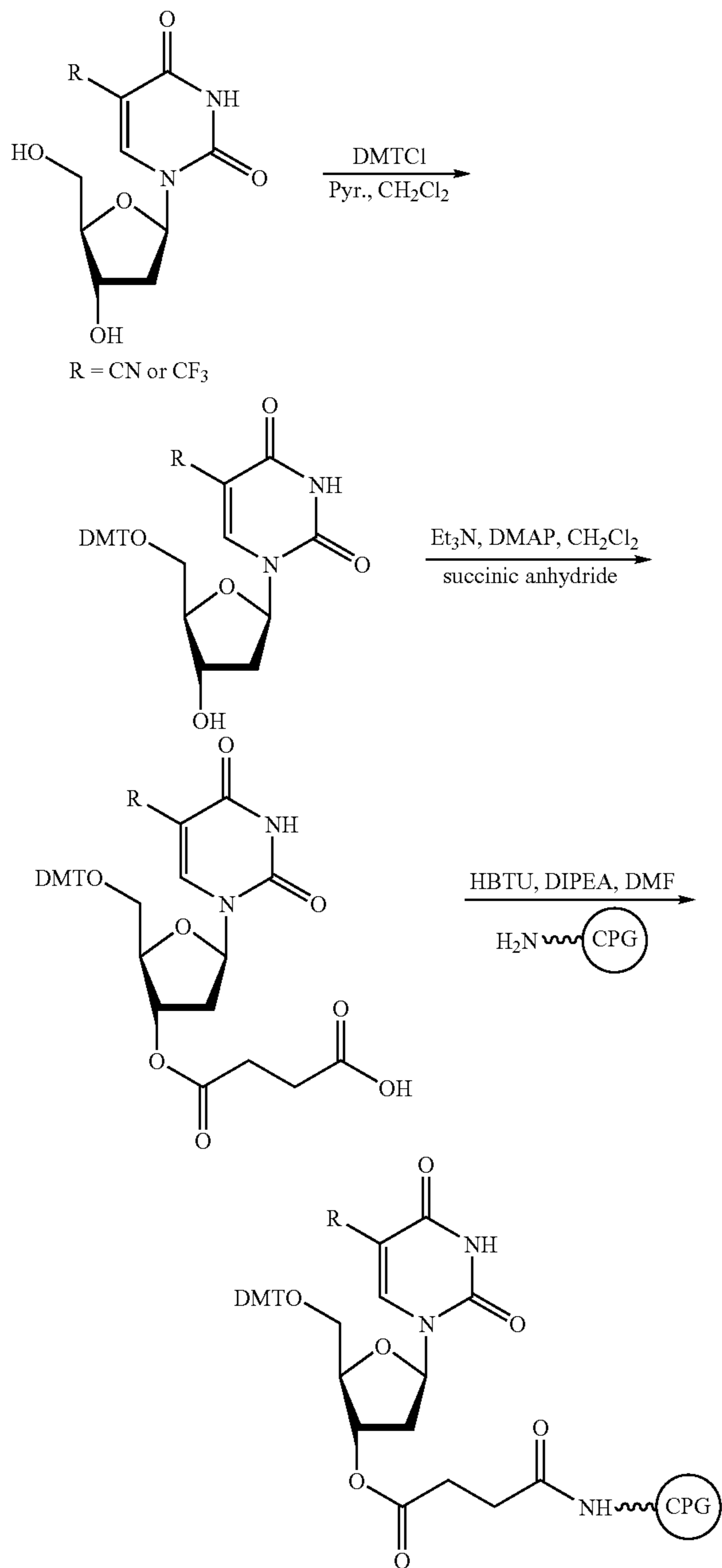
5-Trifluoromethyl-5'-dimethoxytrityl-2'-deoxyuridine
