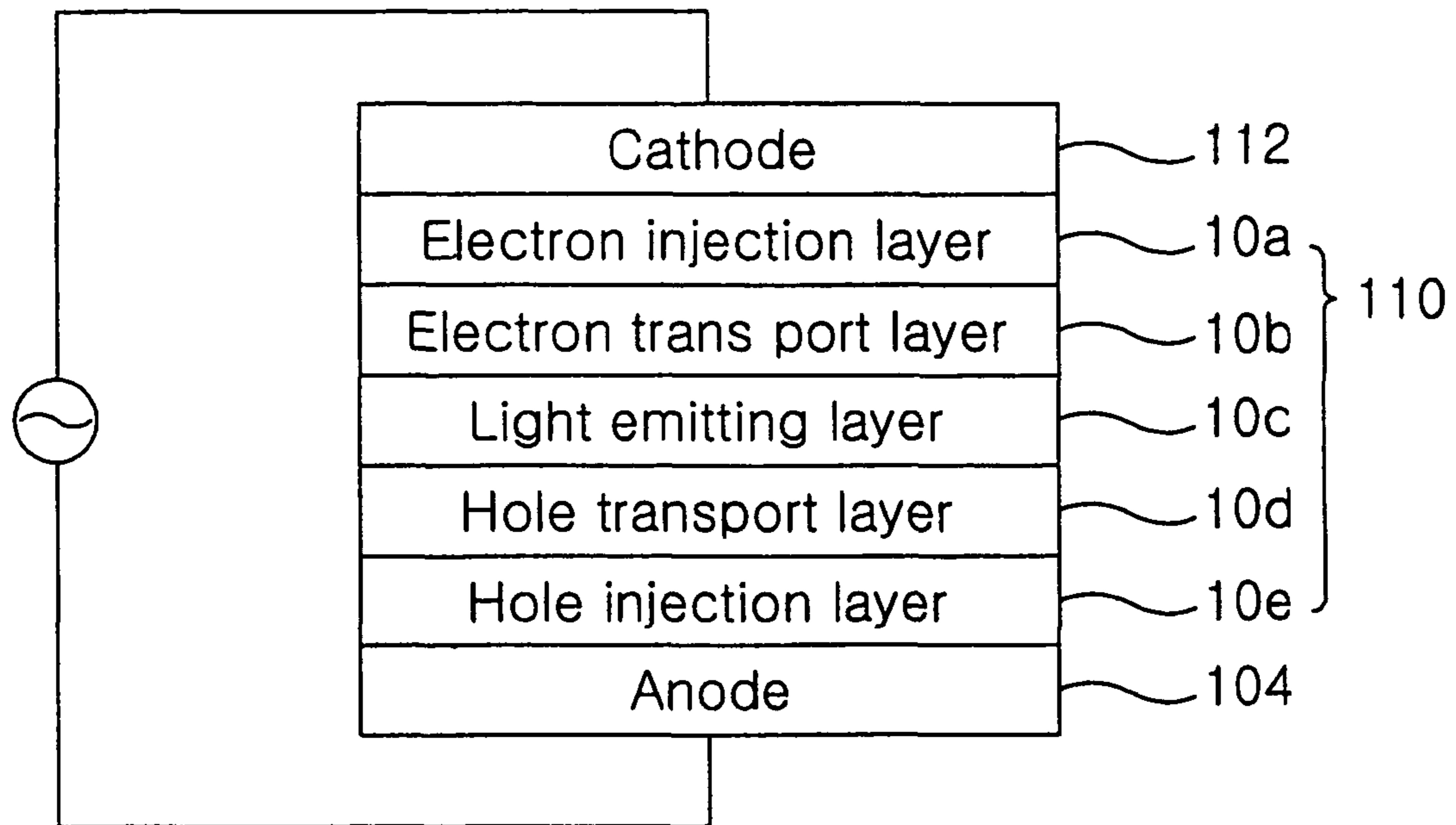
FIG. 1 (RELATED ART)
