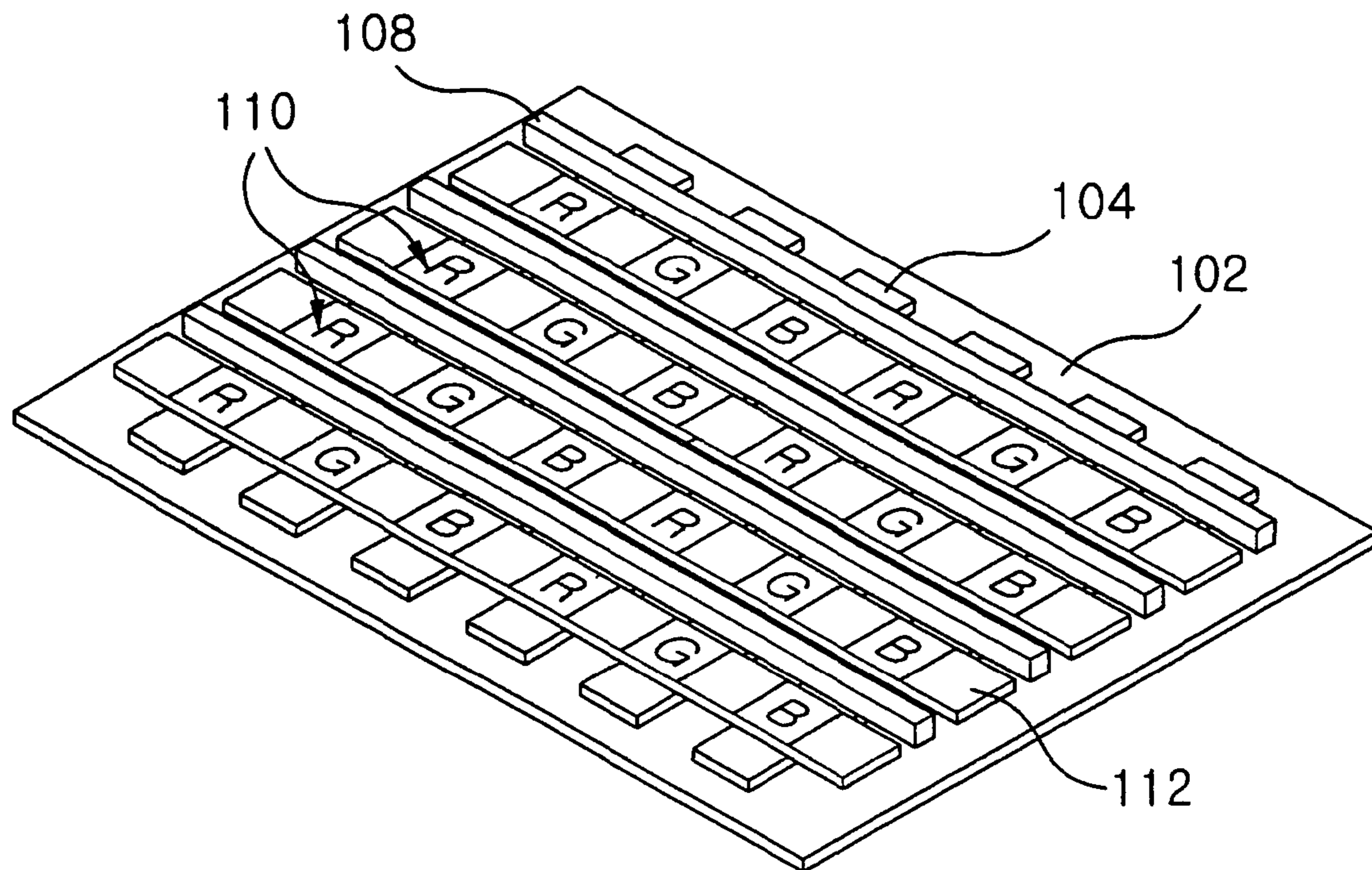
FIG. 2 (RELATED ART)
