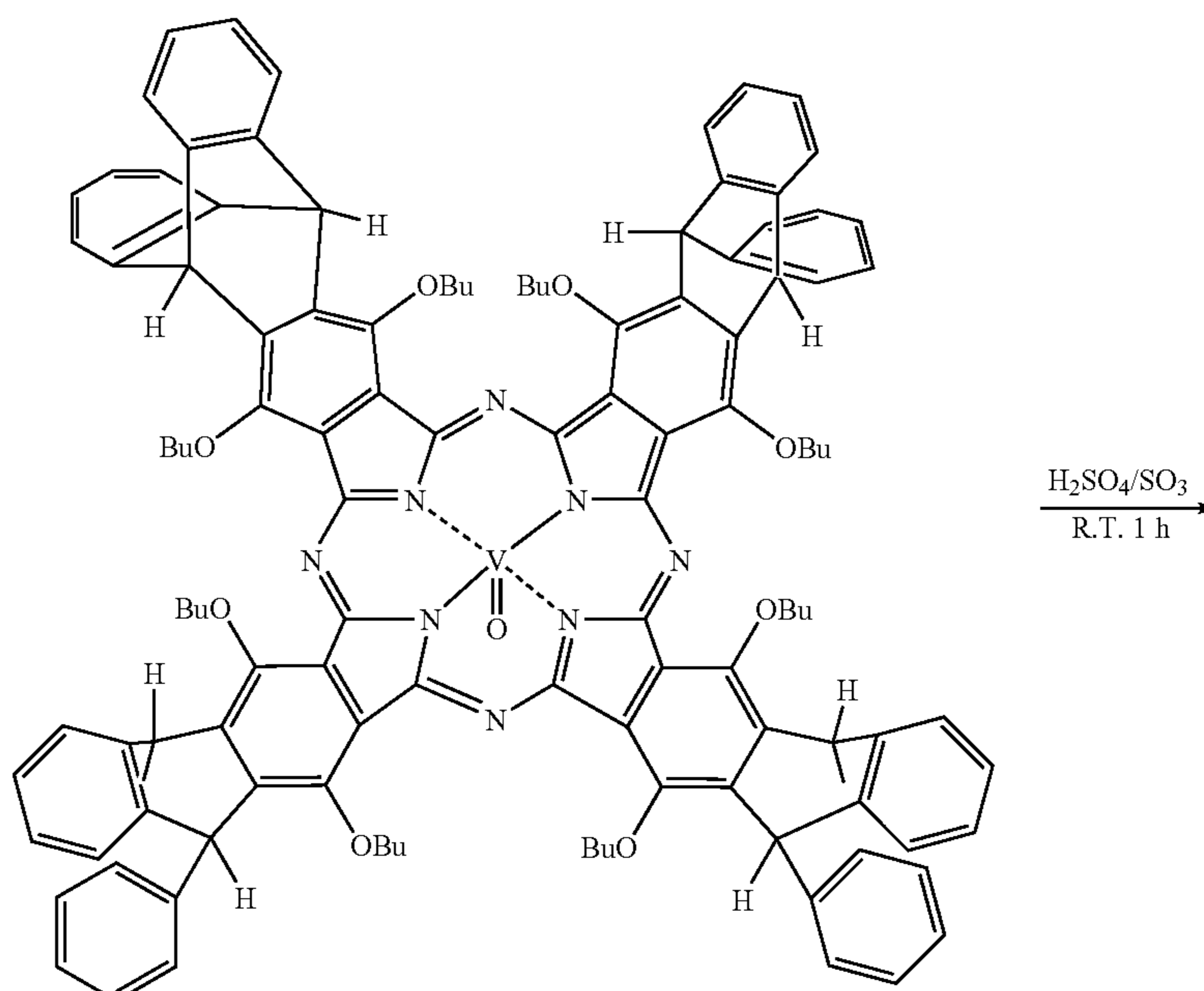
(c) Sulfonation of \text{VOPc}(\text{dib})_4(\text{OBu})_8 to \text{VOPc}(\text{dib})_4(\text{OBu})_8\text{S}_8
