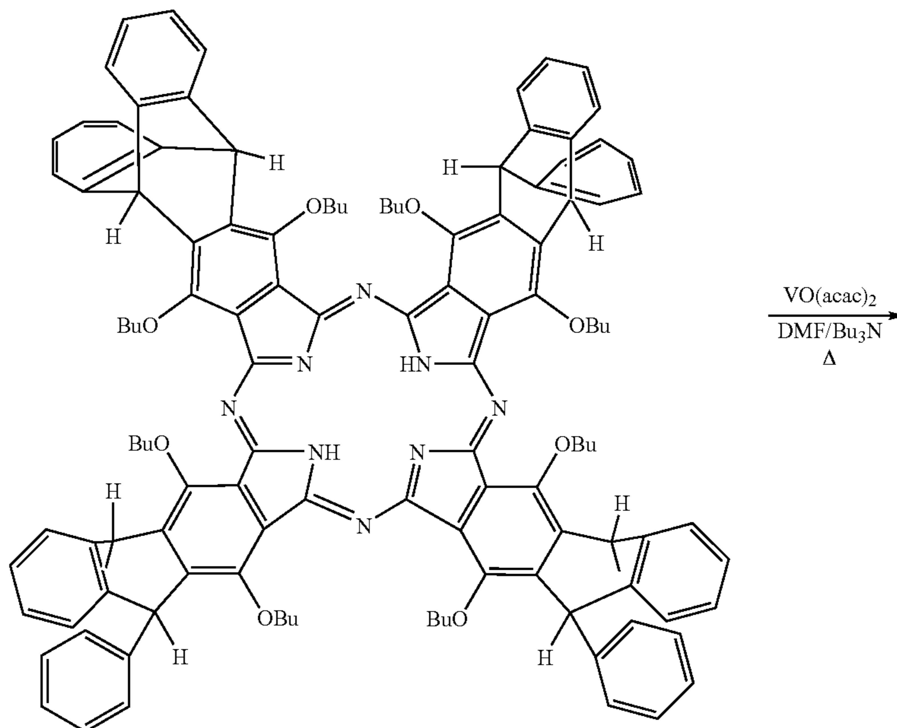
(b) Vanadyl octabutoxyphthalocyanine
