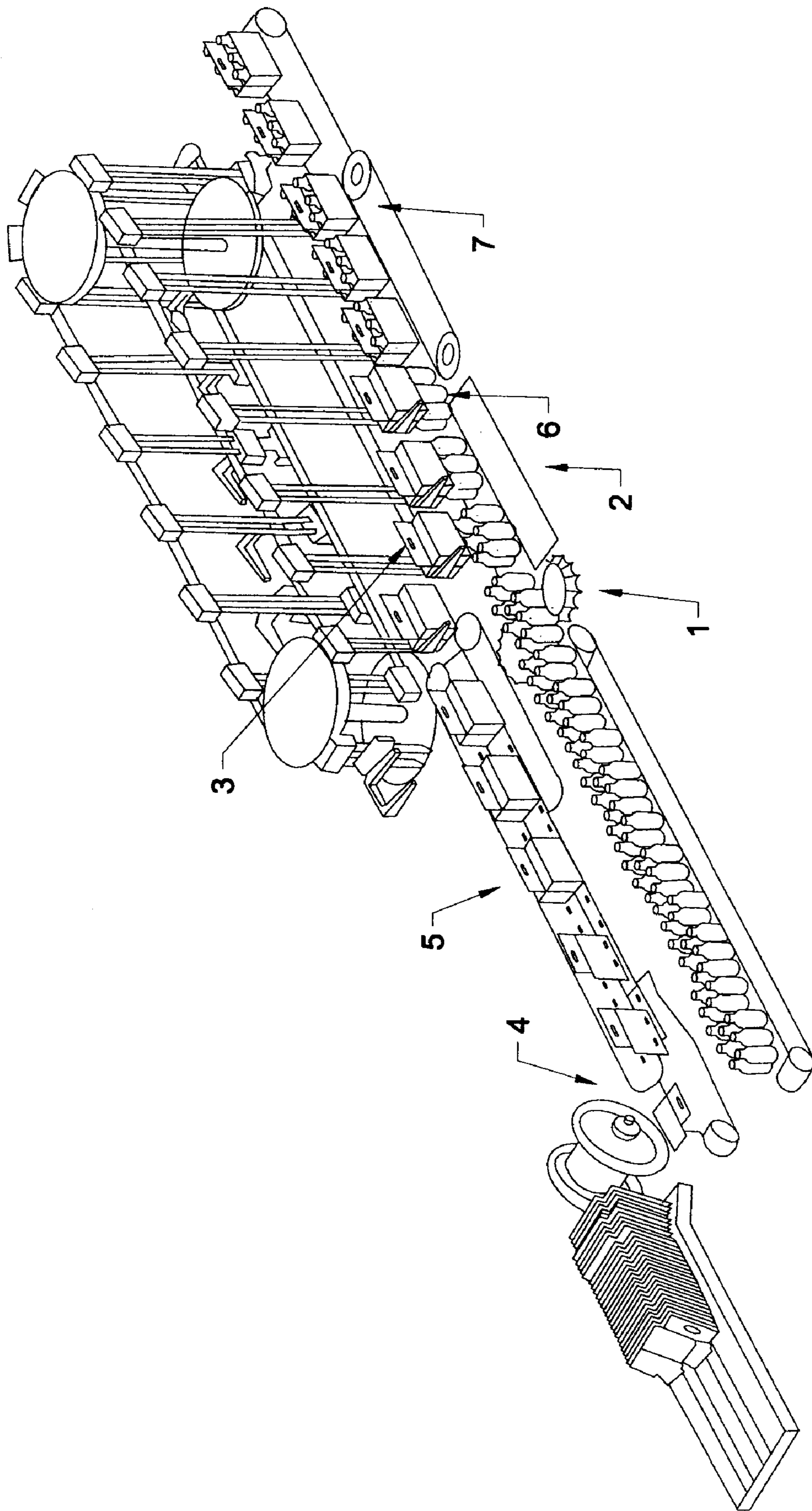
Fig. 1 (PRIOR ART)
