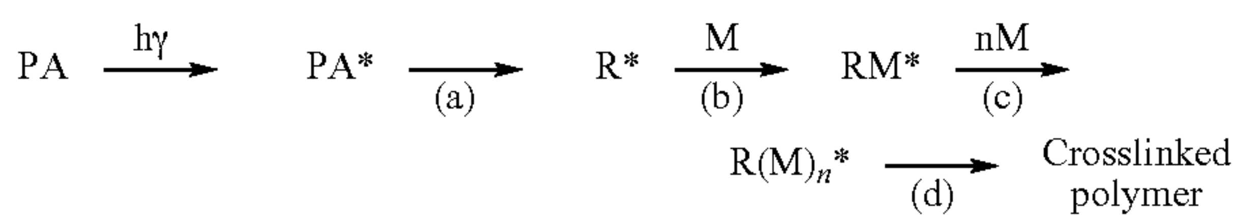
Scheme 1: UV resin radical photopolymerization reactions
