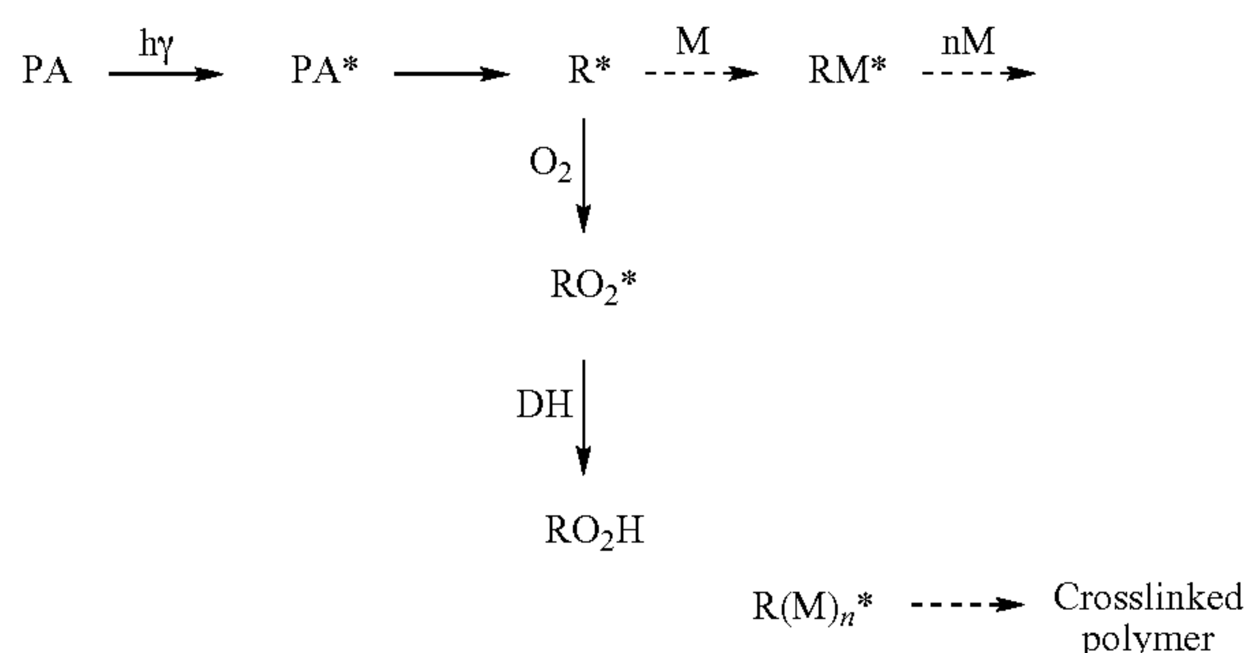
Scheme 2: O 2 inhibition reactions (DH is the diluent or the prepolymer)
