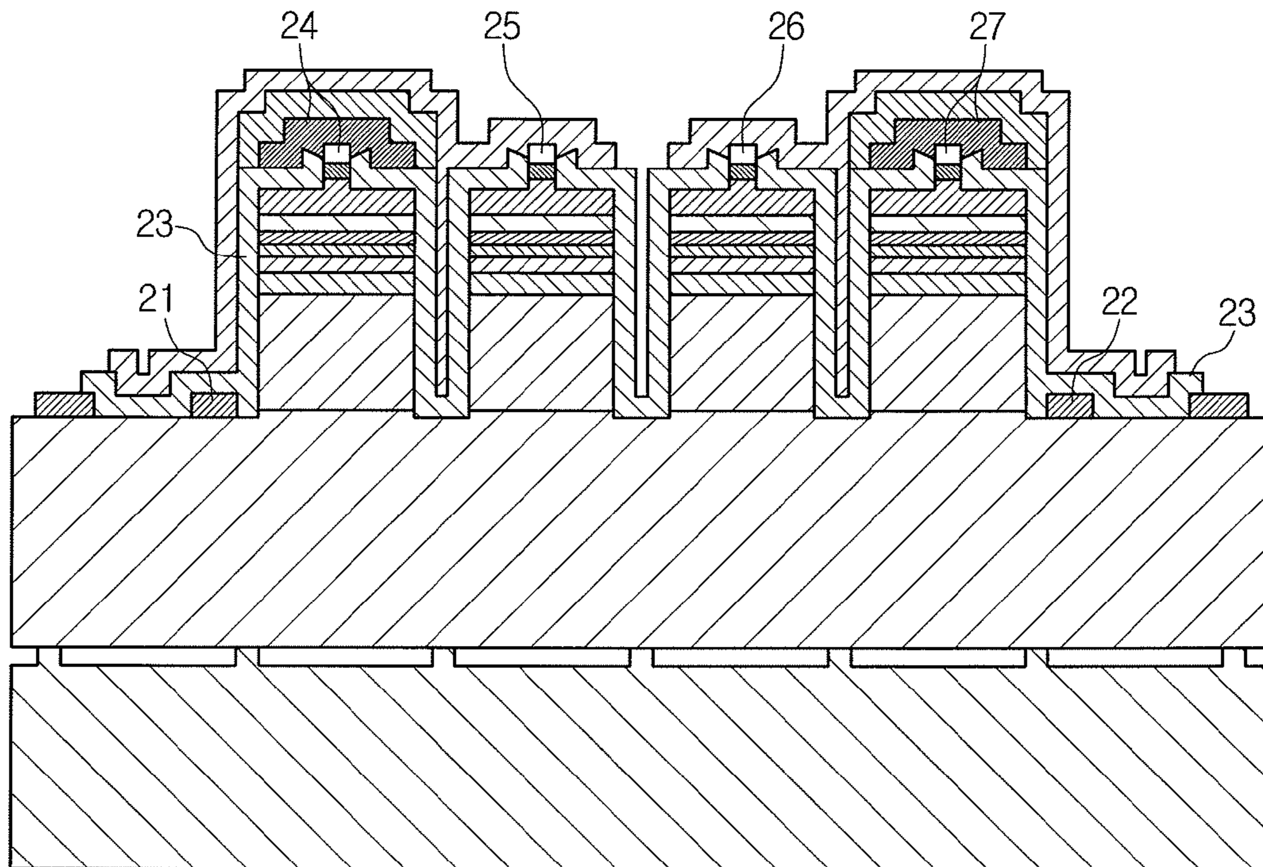
FIG. 2 (PRIOR ART)
