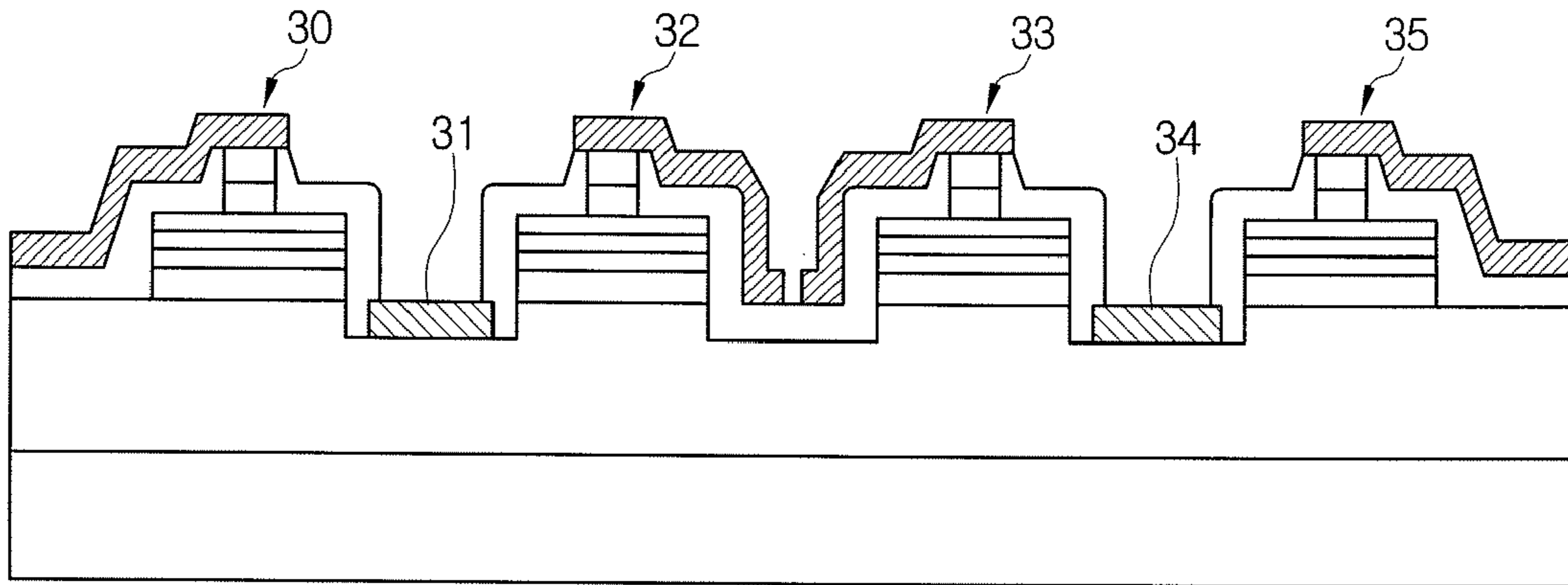
FIG. 3 (PRIOR ART)
