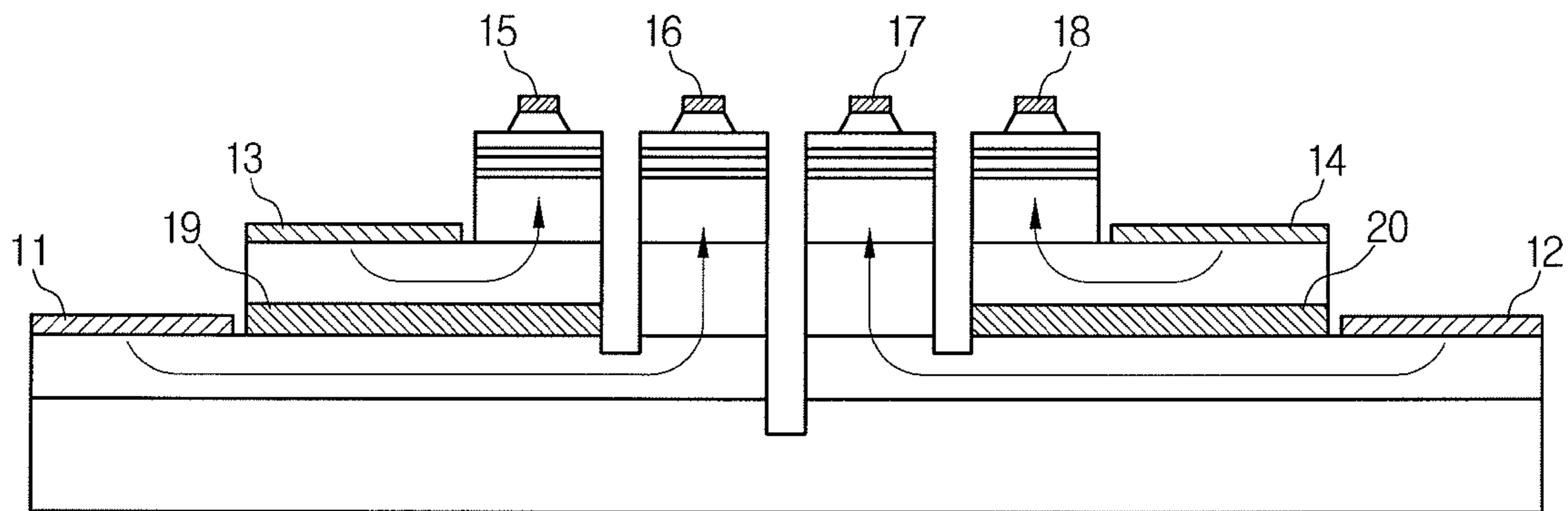
FIG. 1 (PRIOR ART)
