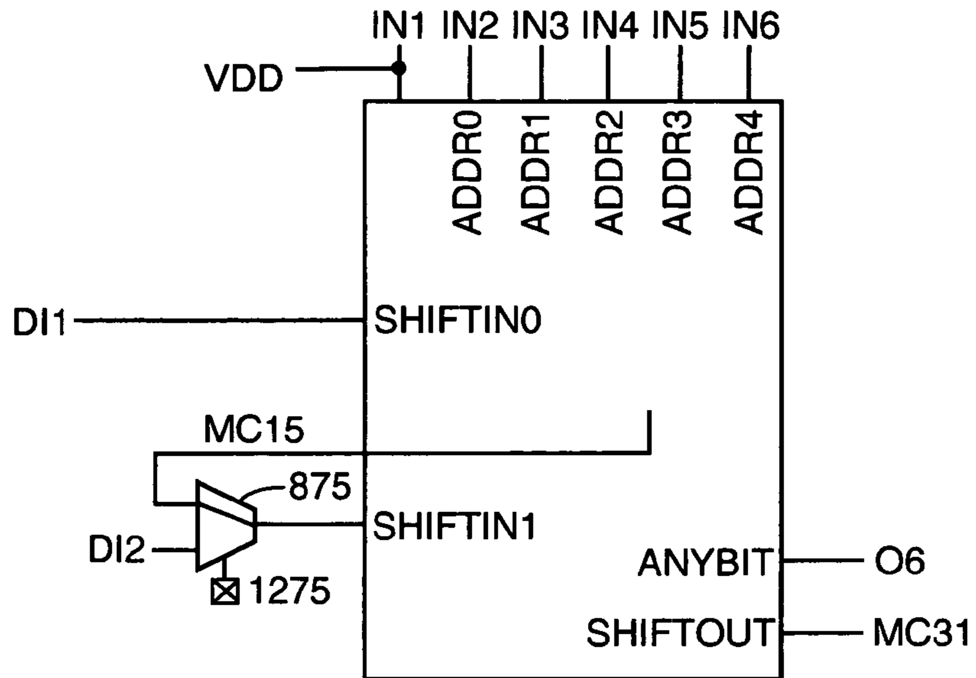
FIG. 12 (32x1 SRL)
