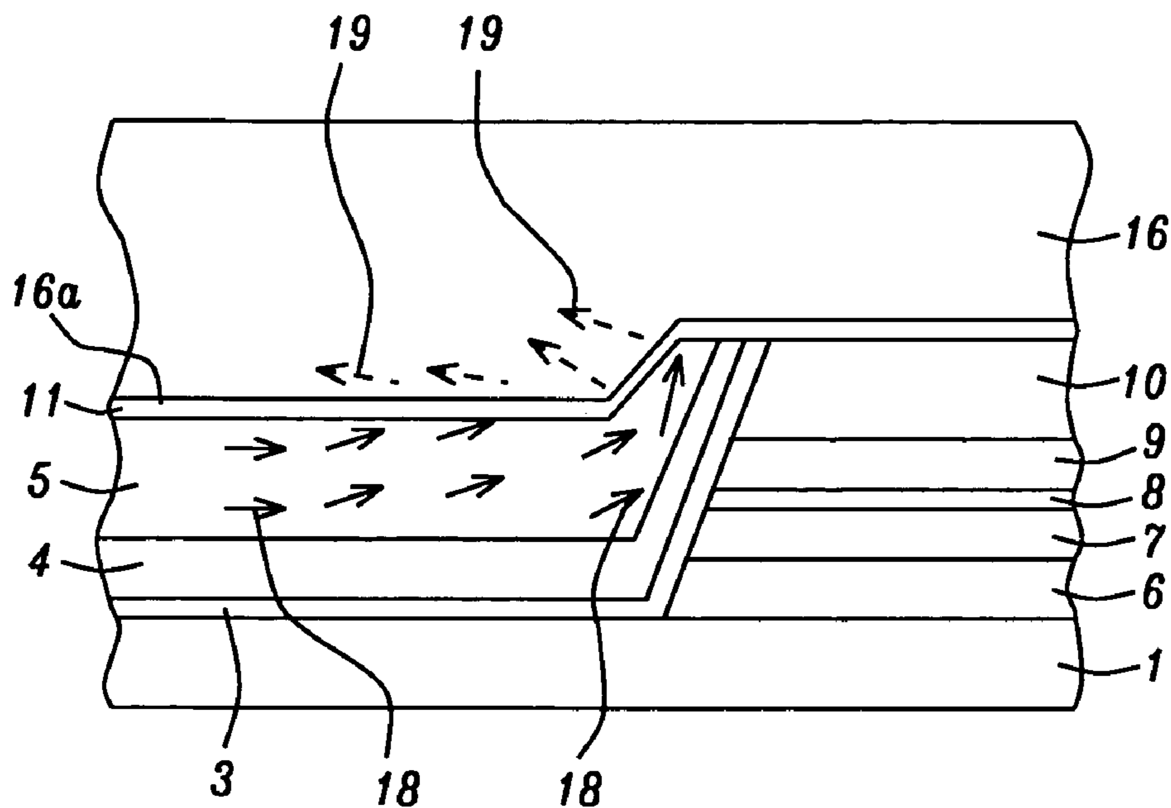
FIG. 4 - Prior Art
