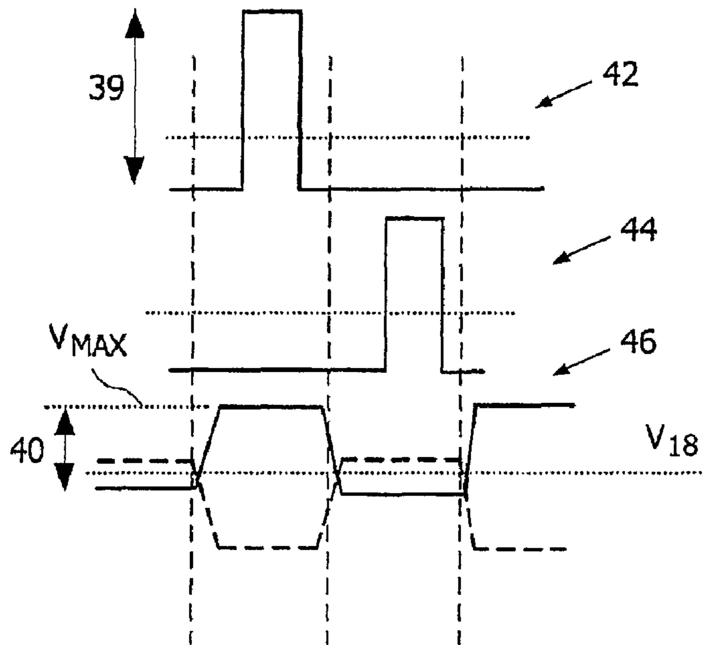
FIG. 3 (PRIOR ART)
