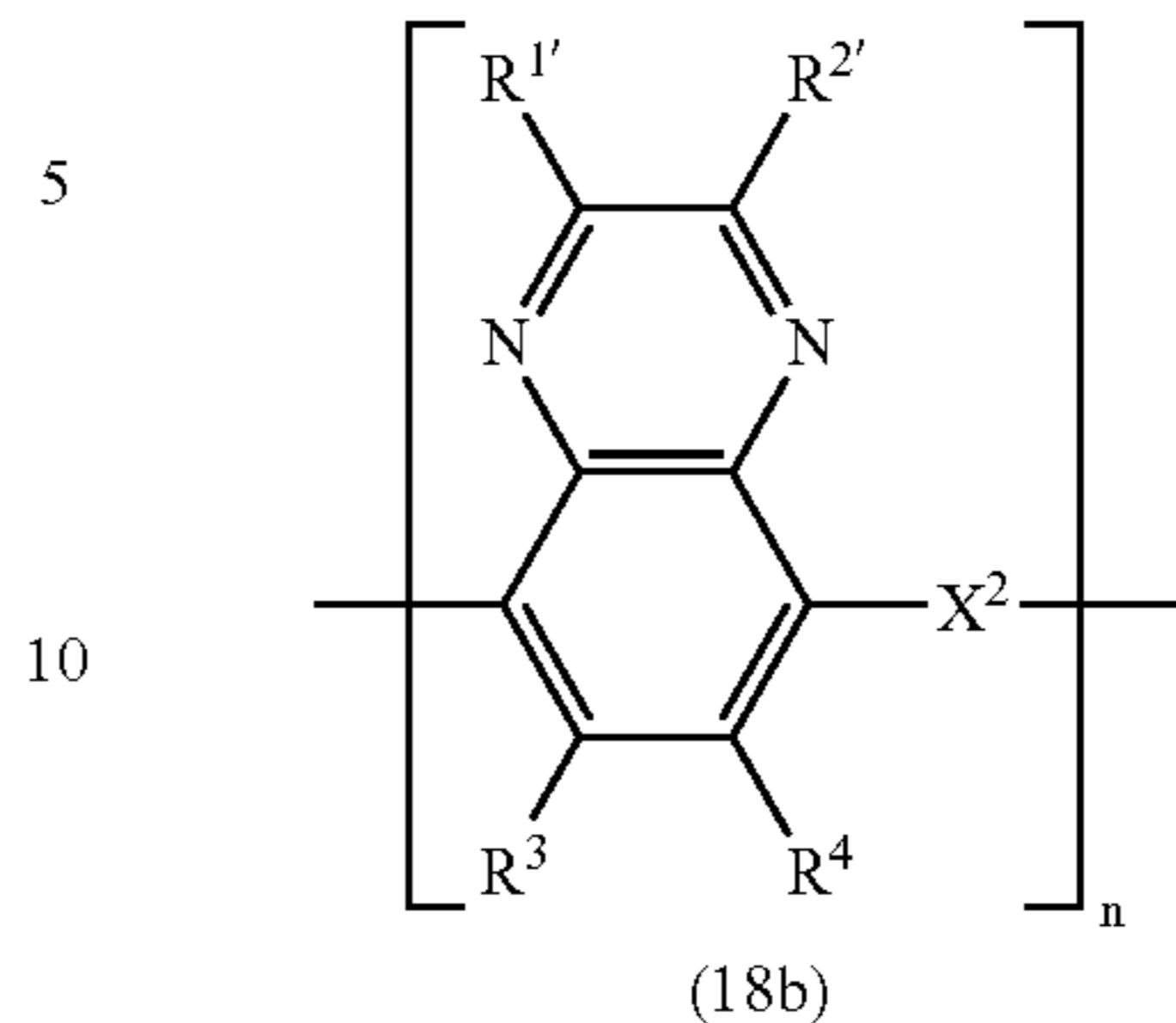
[Chemical Formula 20]
