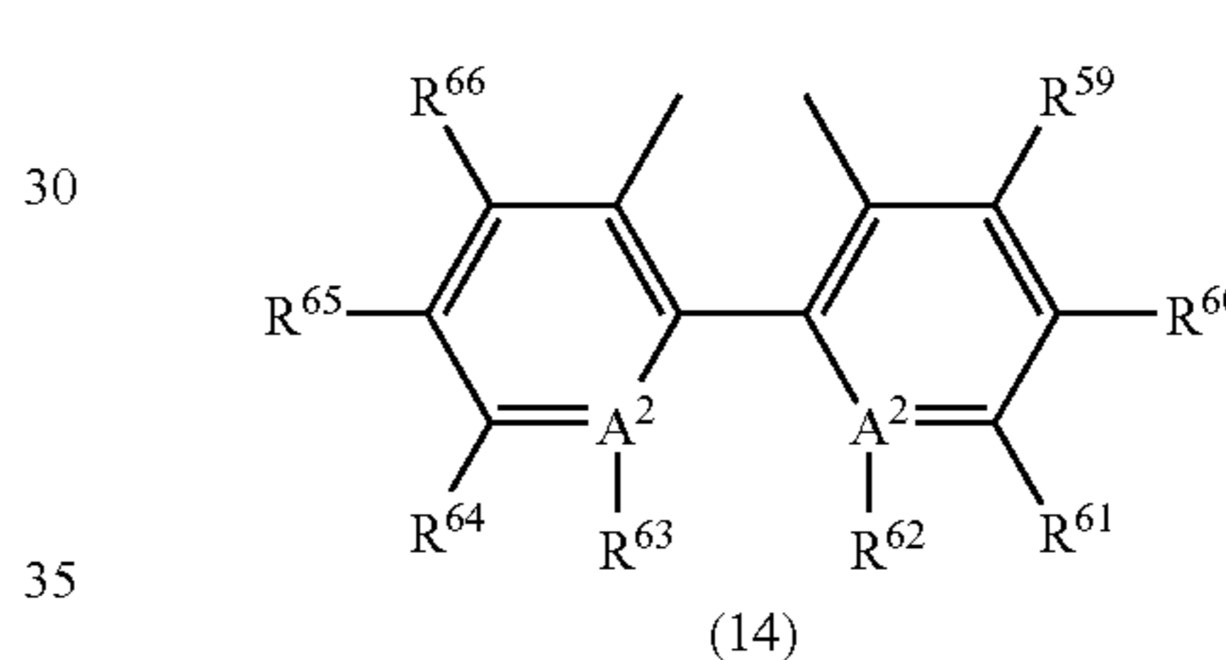
[Chemical Formula 14]
