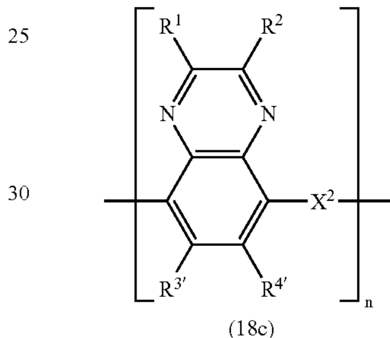
[Chemical Formula 23]
