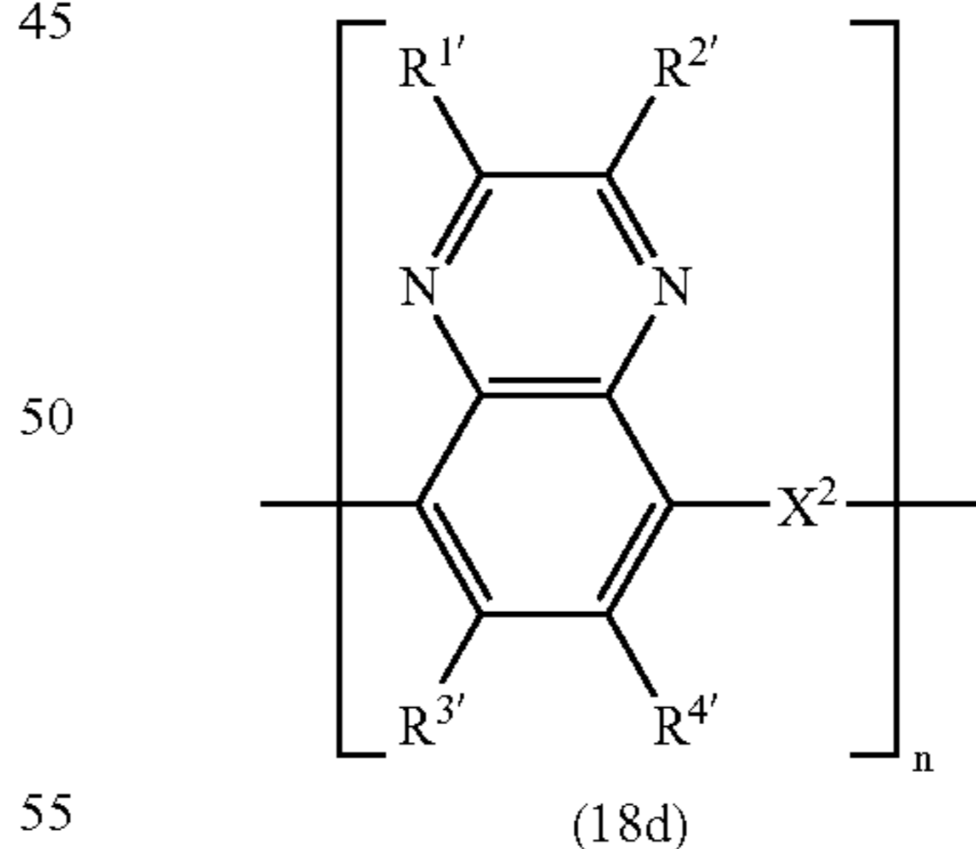
[Chemical Formula 24]
