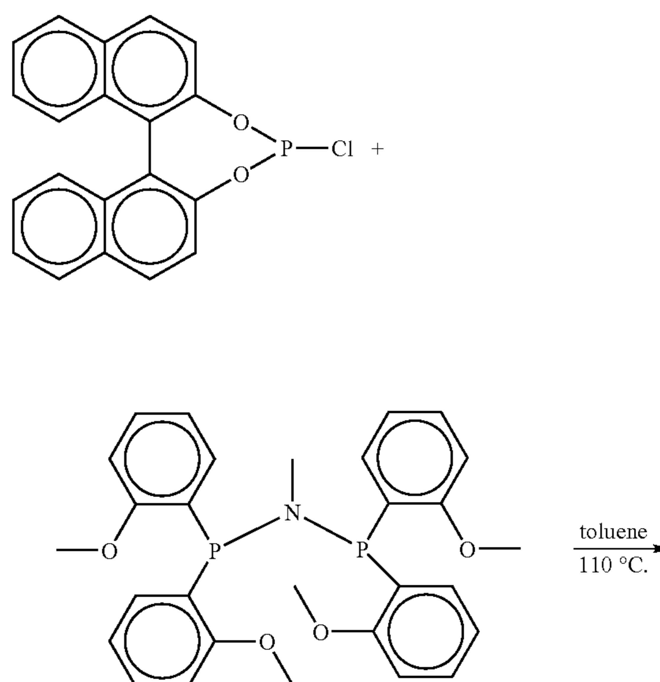
Scheme 1: in situ preparation of ligand composition T'
