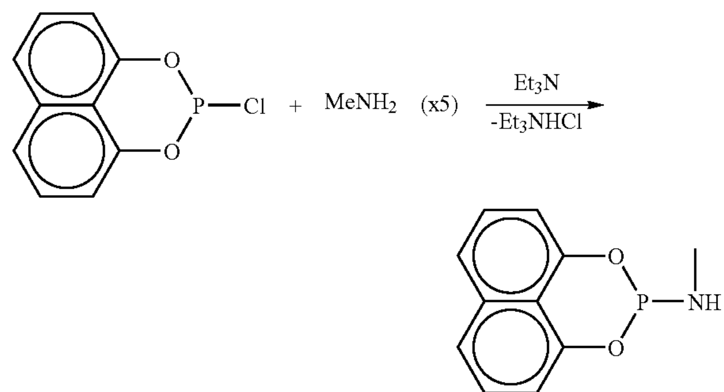
Scheme 2
