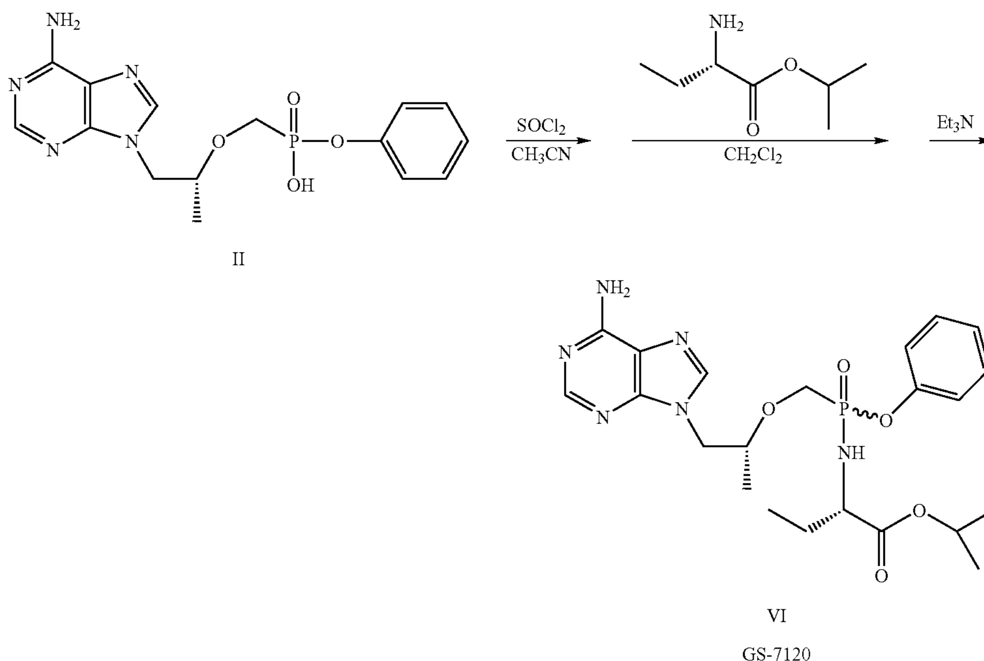
Scheme 3
