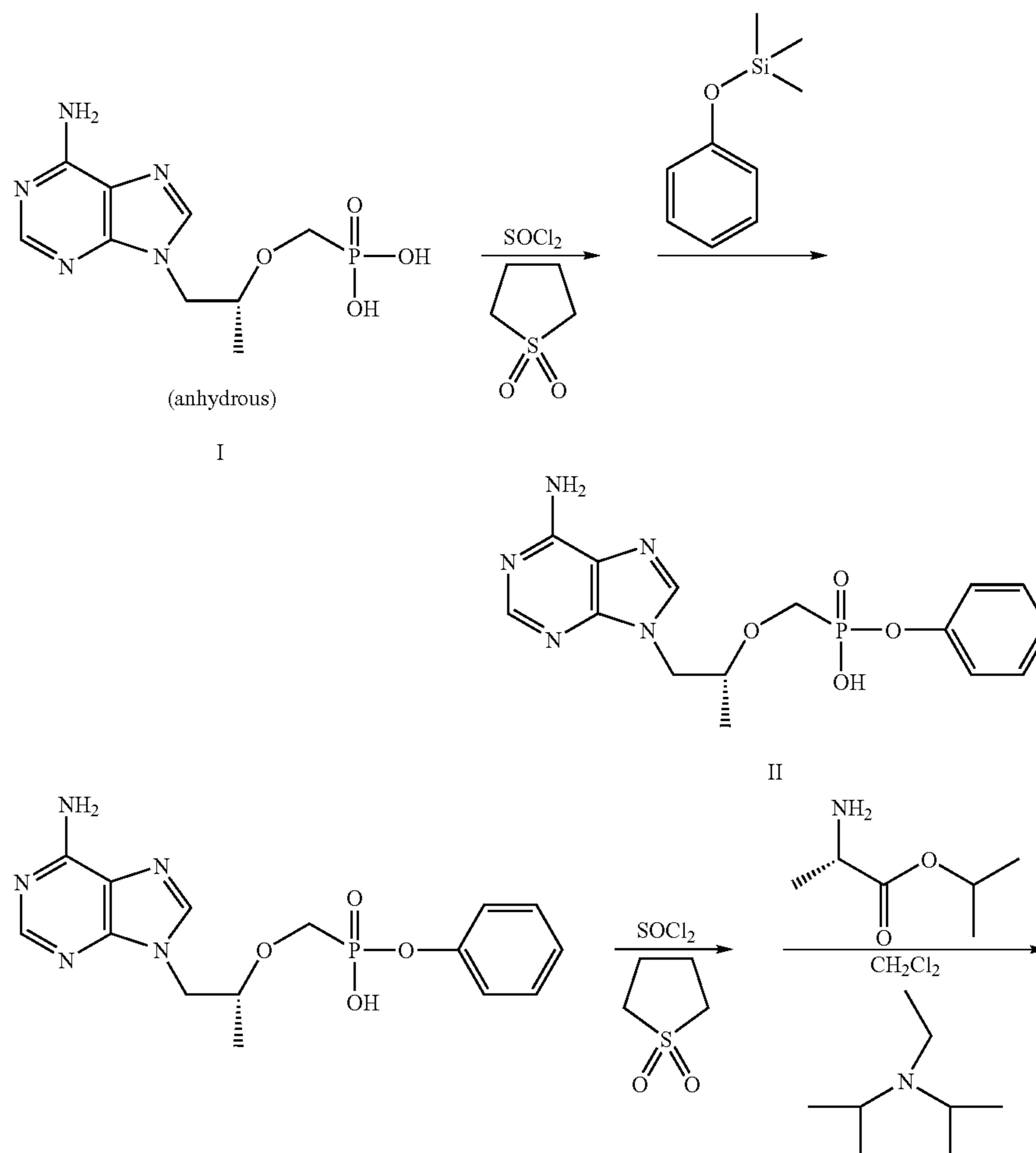
Scheme 2
