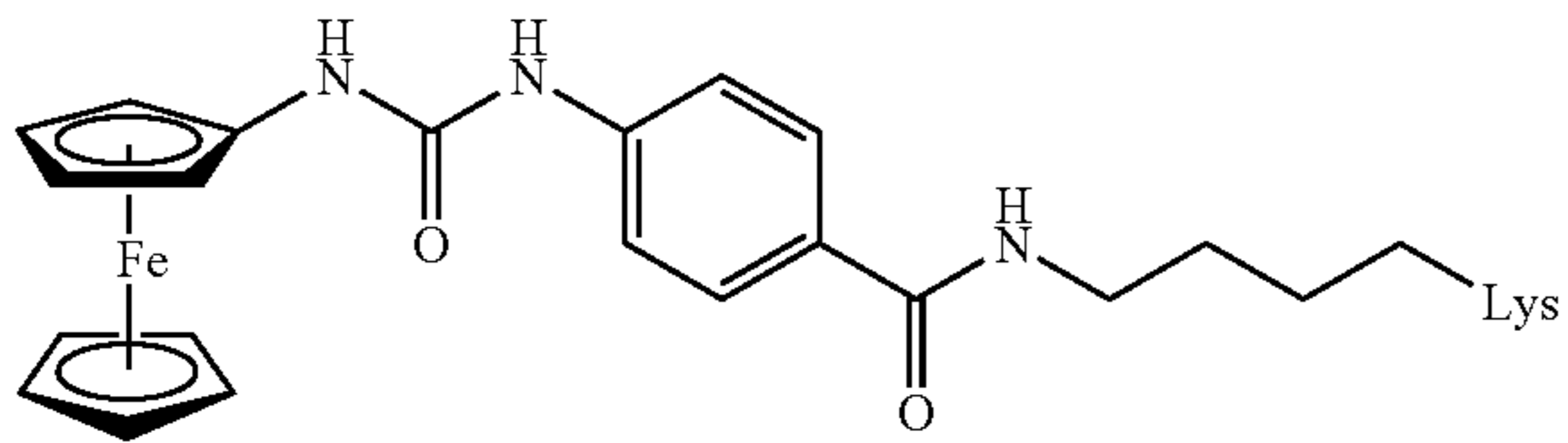
Formula IIIa
