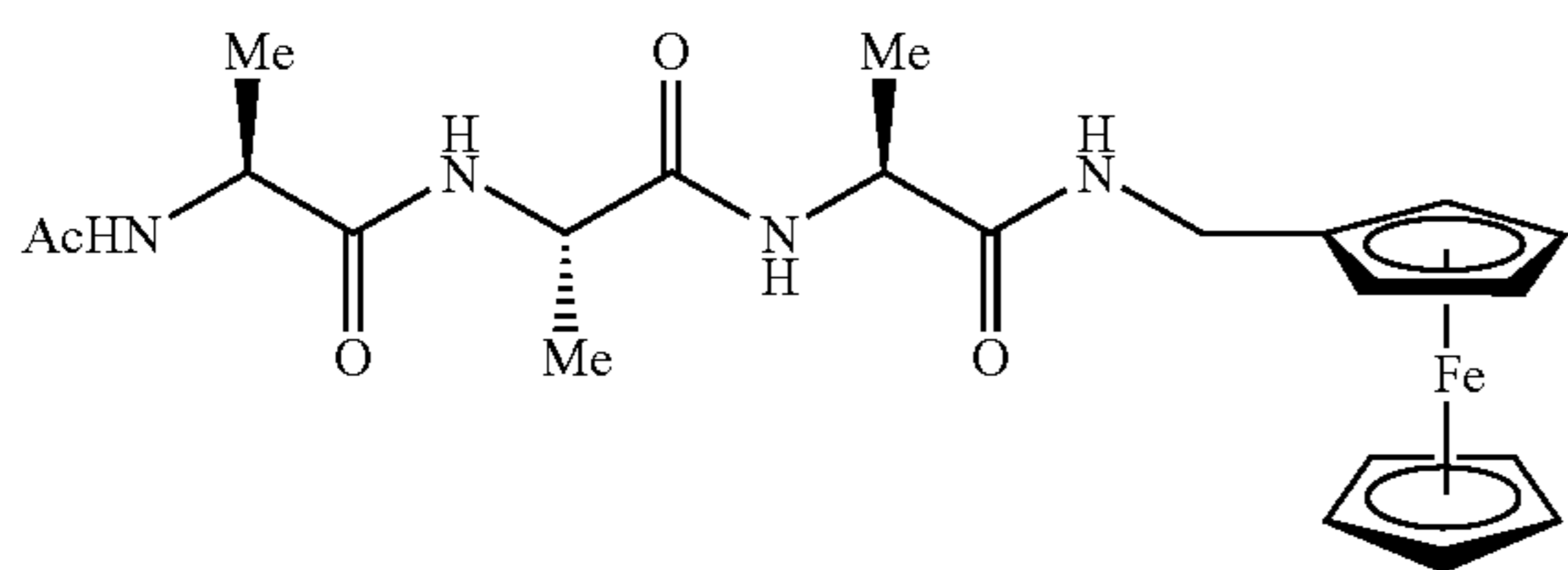
Formula IIIb
