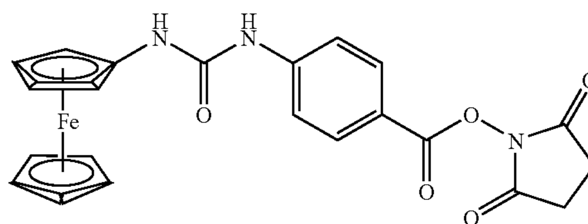
Formula III
